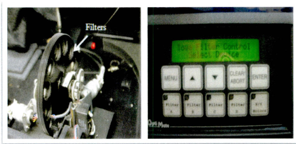
Figure 3.6: The automatic filter control select device and the remote control filter wheel.
