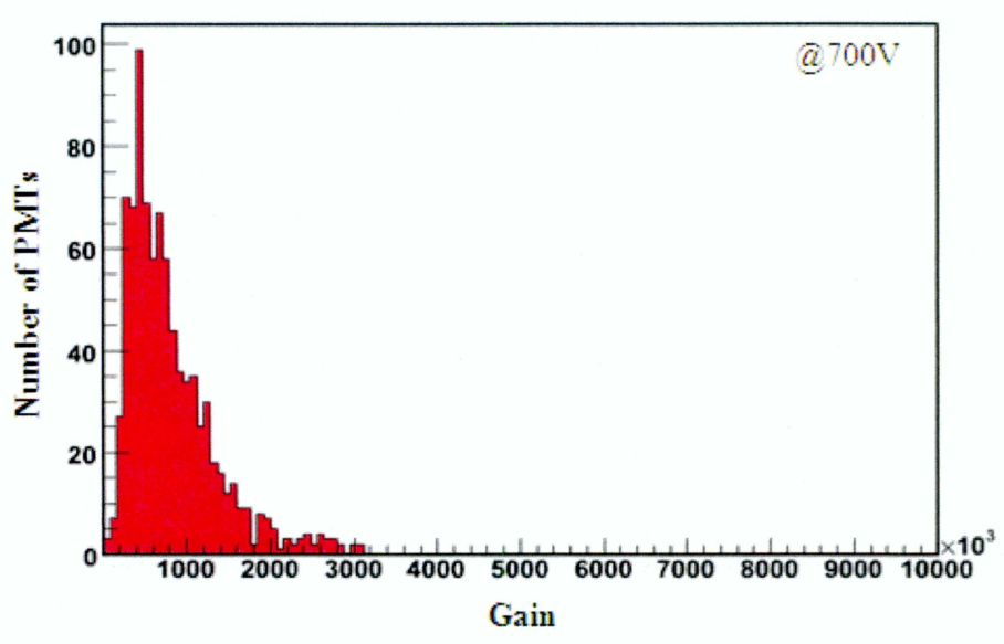
Figure 4.10: Gain Distribution of 900 PMTs at 700 V.
