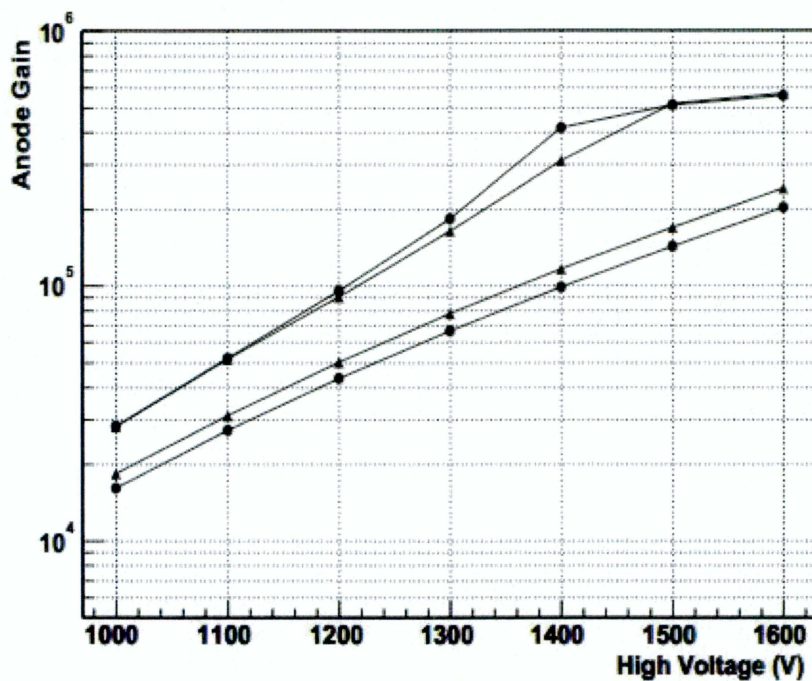
Figure 3.11: The measurement of the gain versus voltage applied before and after the lifetime test [10].
