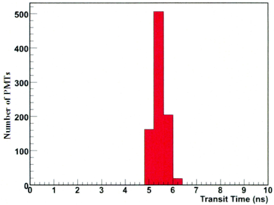
Figure 4.17: Transit time distribution for 900 PMTs.
