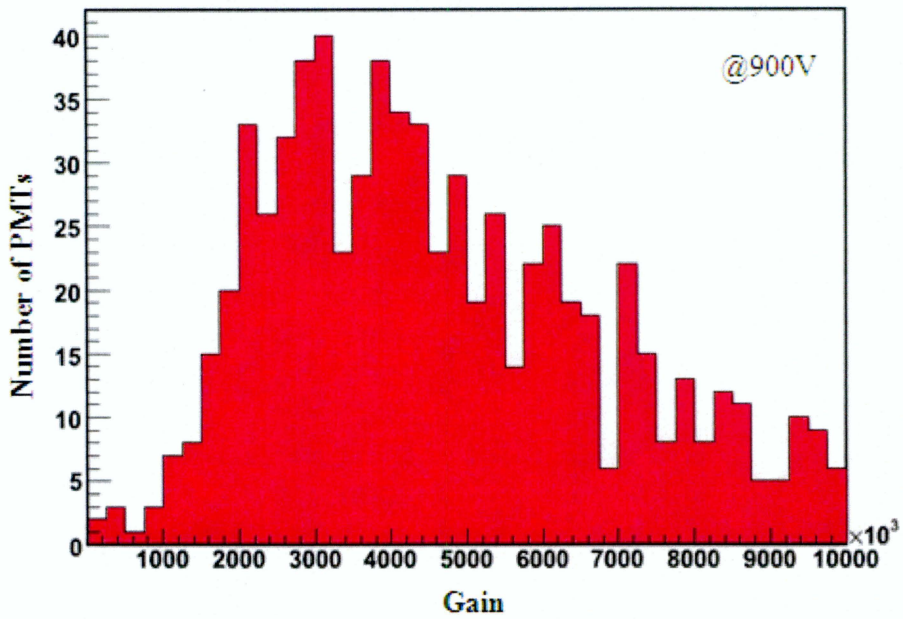
Figure 4.14: Gain Distribution of 900 PMTs at 900 V.
