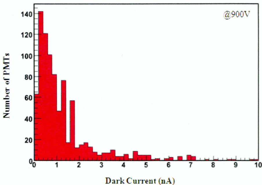
Figure 4.7: Dark current distribution of 900 PMTs at 900 V.
