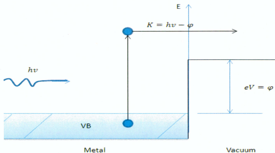
Figure 2.7: The energy level diagram of a metal and the photoelectric effect
