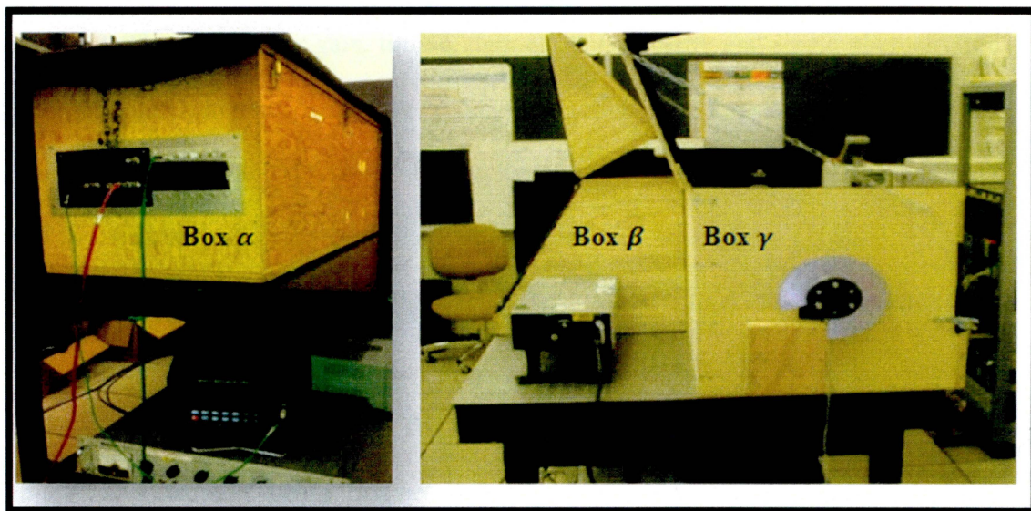
Figure 2.8: Light Tight Boxes: \alpha , \beta and \gamma are aimed to use for measuring different parameters.
