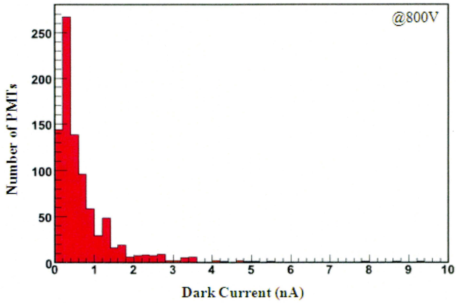
Figure 4.5: Dark current distribution of 900 PMTs at 800 V.
