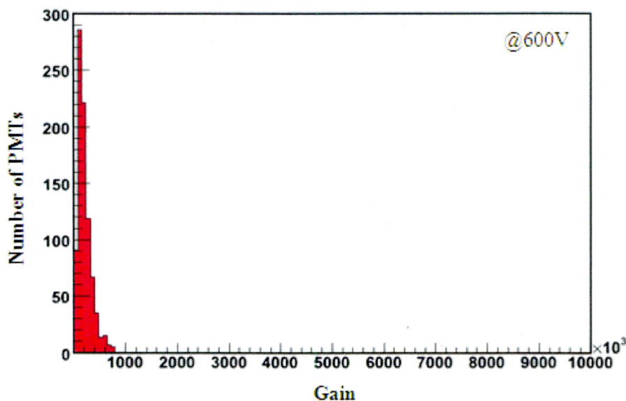
Figure 4.8: Gain distribution of 900 PMTs at 600 V.
