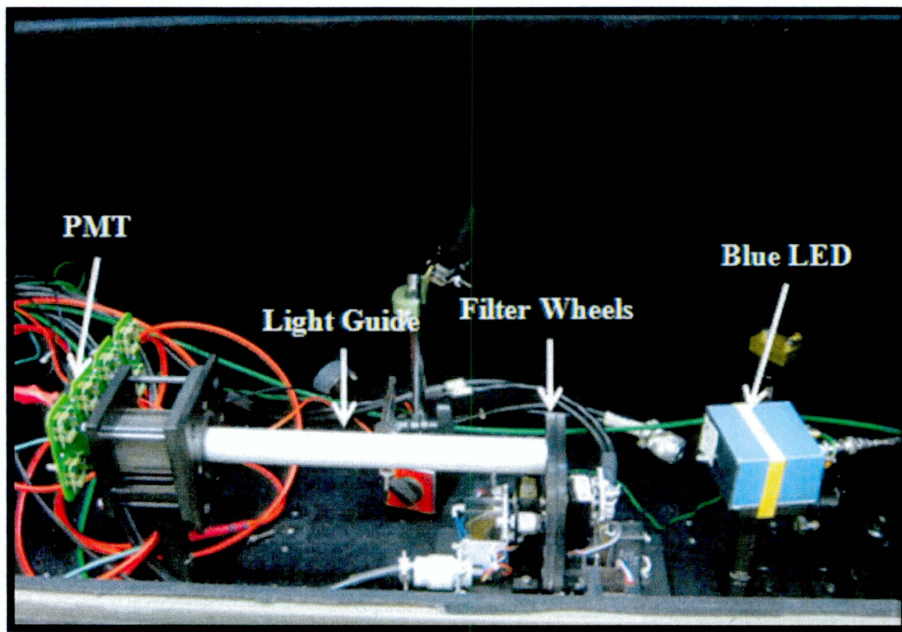
Figure 3.7: The light guide system from the filter wheel to the PMT for D. Pulse test
