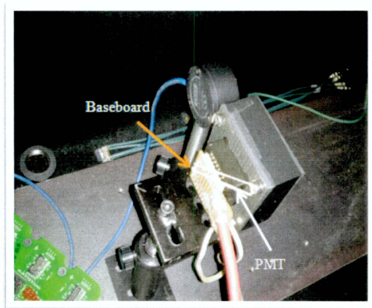
Figure 3.3: The baseboard and the PMT setup for cathode gain test.
