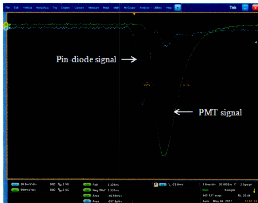
Figure 3.5: The difference between the PMT signal and pin-diode signal on the oscilloscope
