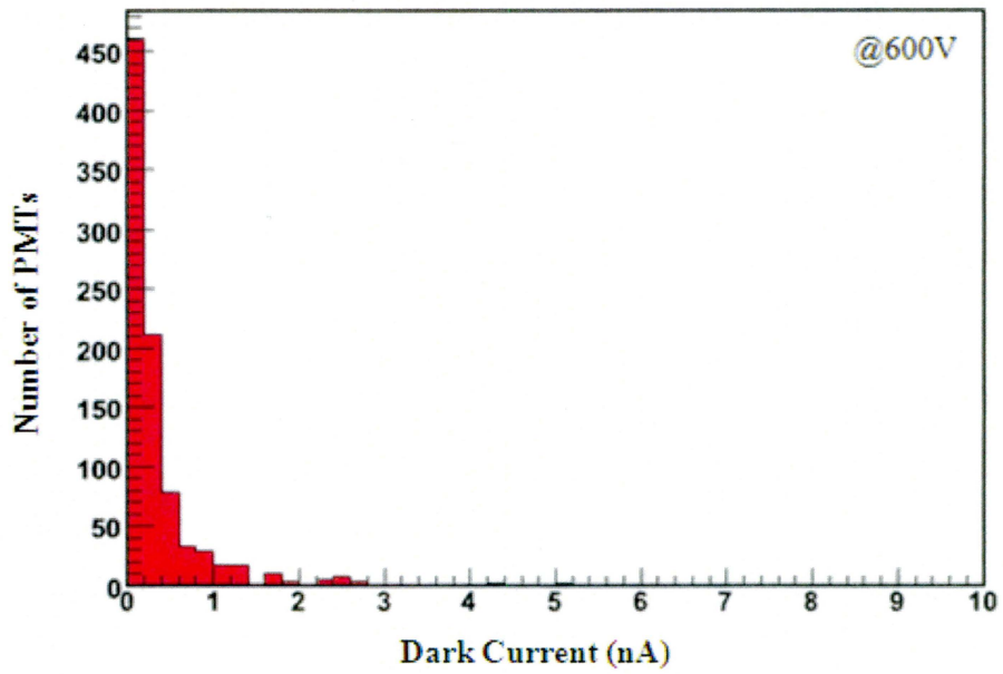
Figure 4.1: Dark current distribution of 900 PMTs at 600 V.
