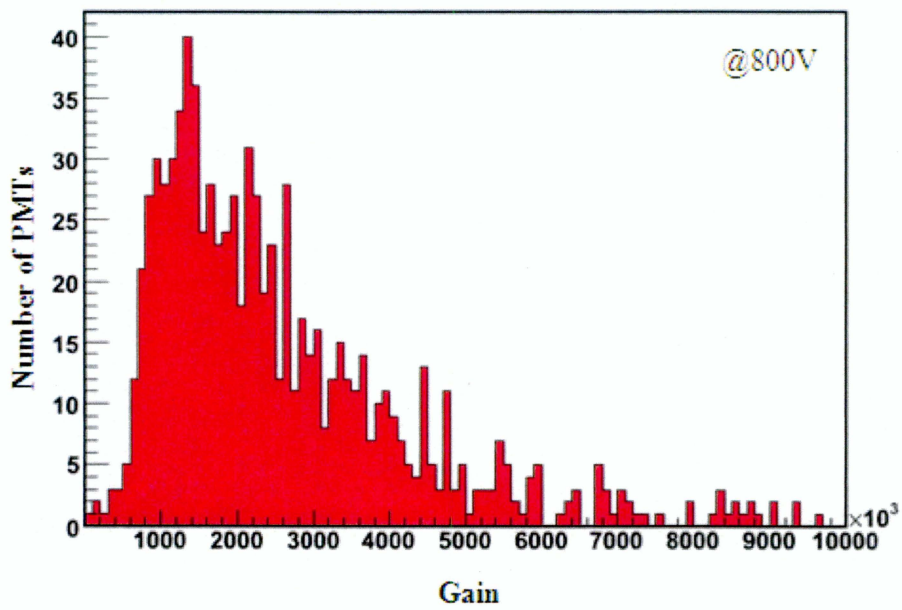
Figure 4.12: Gain Distribution of 900 PMTs at 800 V.
