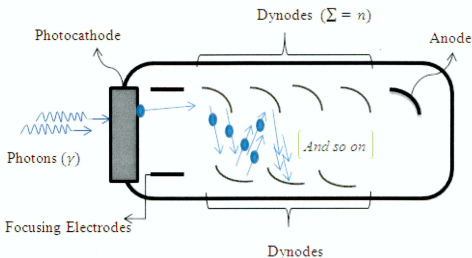
Figure 2.6: Schematic diagram of a linear focused type PMT and the total number of dynode structures ( \Sigma \text{ dynodes} = n ).
