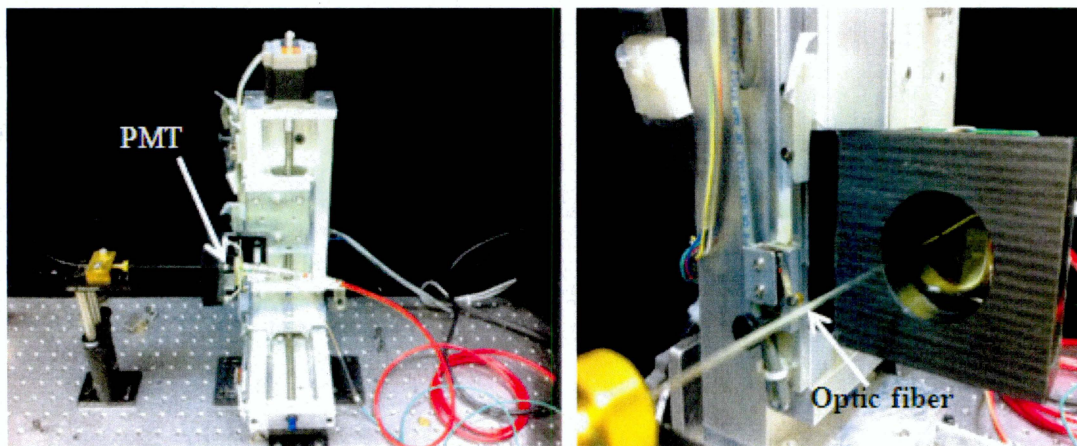
Figure 3.9: The computer controlled X-Y scanner and the fiber controlling each cell of the PMT.
