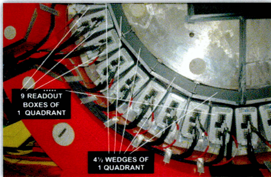
Figure 2.5: In each quadrants of the HF, total 216 PMTs are located equally in 9 identical readout boxes, with 24 PMTs in each box [9].
