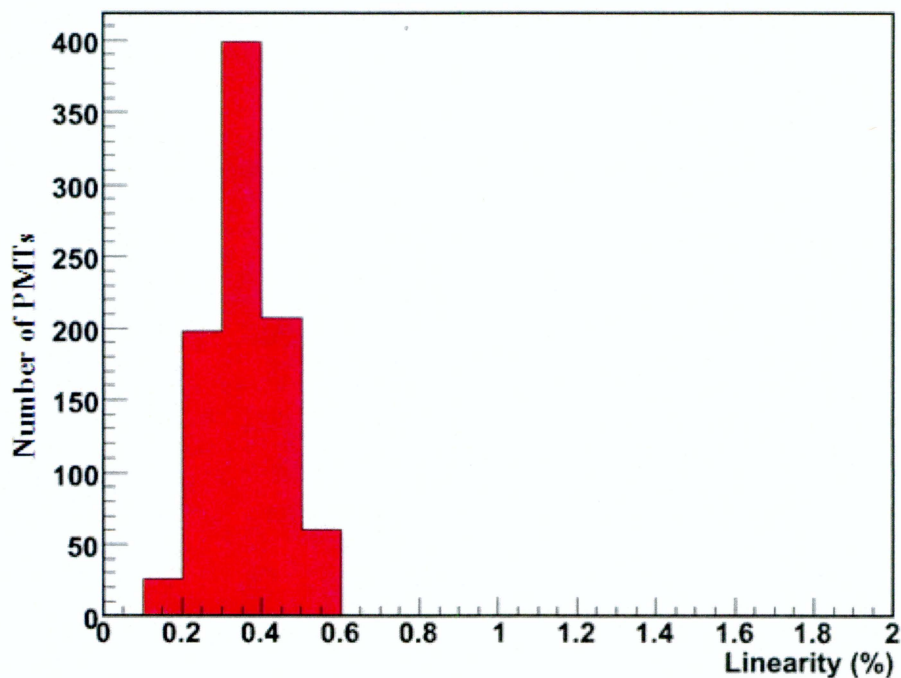
Figure 4.19: Single pulse linearity distribution for 900 PMTs and x-axis shows the percentage deviation.
