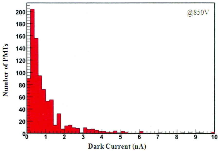
Figure 4.6: Dark current distribution of 900 PMTs at 850 V.
