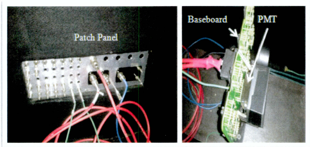
Figure 3.2: The patch panel of the Box- \alpha and PMT baseboard for dark current and anode gain test.
