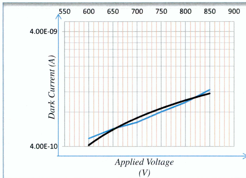
Figure 3.1: Dark Current vs. Supply Voltage for one PMT with serial number JA0883
