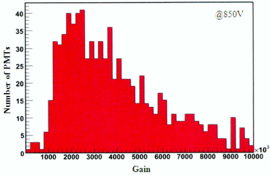
Figure 4.13: Gain Distribution of 900 PMTs at 850 V.
