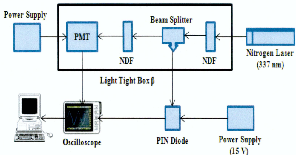
Figure 3.4: Schematic representation of the Box- \beta and the timing set-up.
