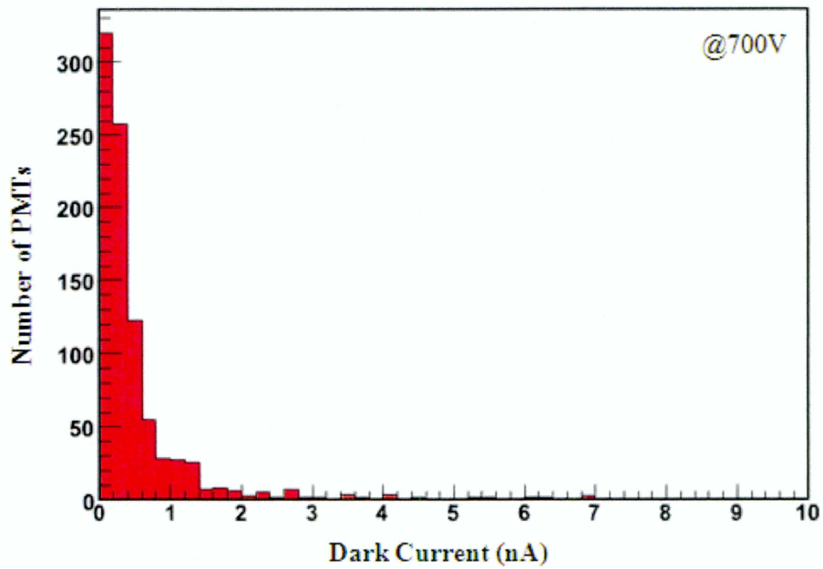
Figure 4.3: Dark current distribution of 900 PMTs at 700 V.
