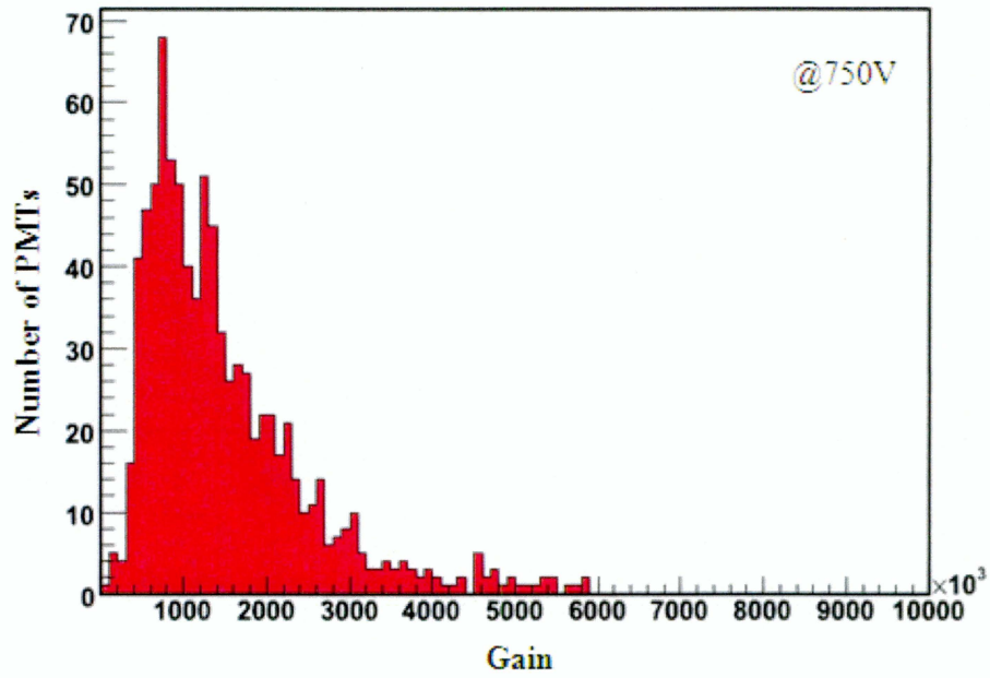
Figure 4.11: Gain Distribution of 900 PMTs at 750 V.
