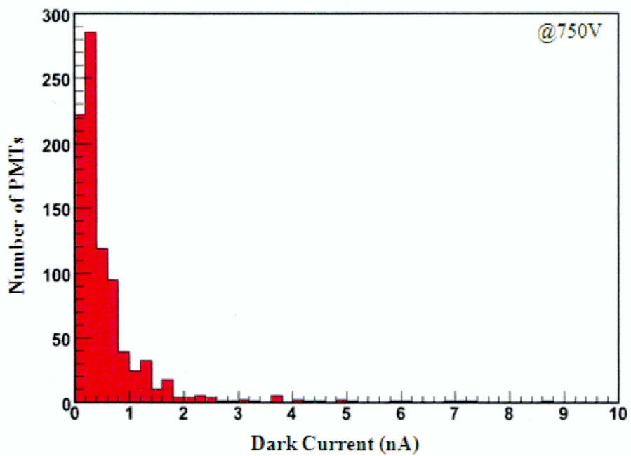
Figure 4.4: Dark current distribution of 900 PMTs at 750 V.
