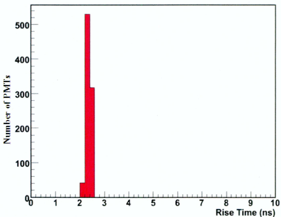
Figure 4.15: Rise time distribution for 900 PMTs.
