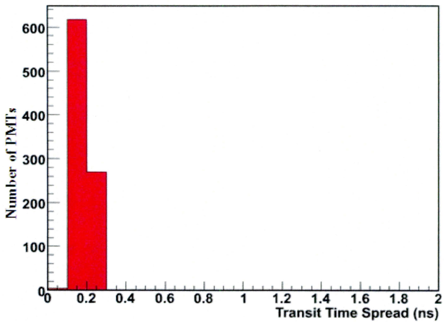
Figure 4.18: Transit time spread distribution for 900 PMTs.
