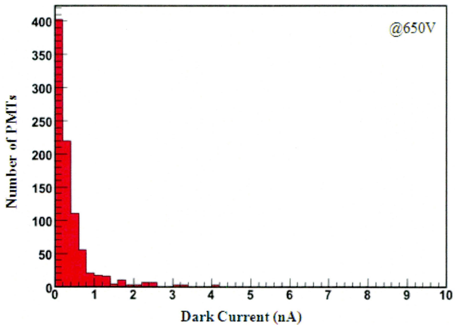
Figure 4.2: Dark current distribution of 900 PMTs at 650 V.
