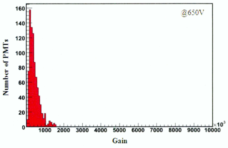
Figure 4.9: Gain Distribution of 900 PMTs at 650 V.
