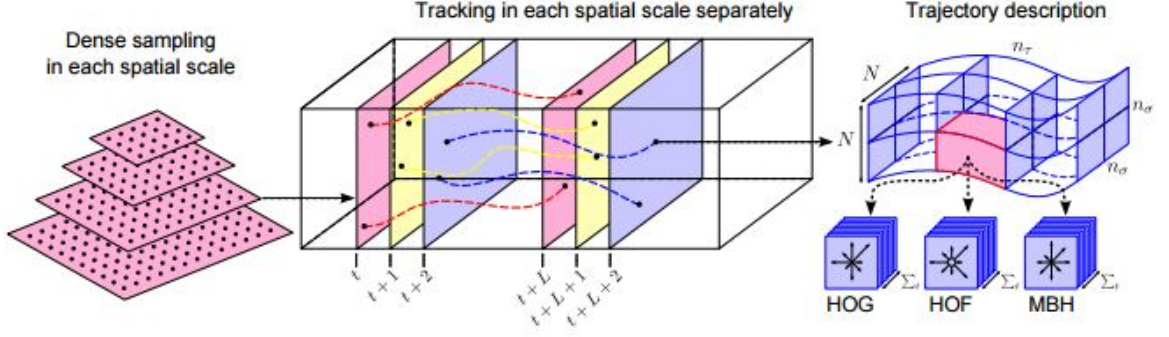
Figure 4.3. Illustration of the approach to extract and characterize dense trajectories.
