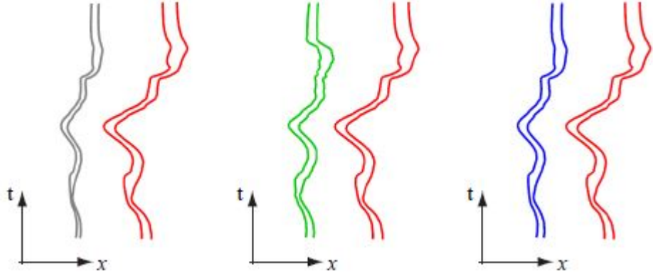
Figure 2.9. The original, linearly scaled, per-frame resized and the optimal motion pathlines are shown in red, gray, green and blue, respectively, projected onto the (x,t) plane. Note that the horizontal offsets between the pathlines are consistently reduced in the linearly scaled and the optimized trajectories. Figure is taken from [4].
