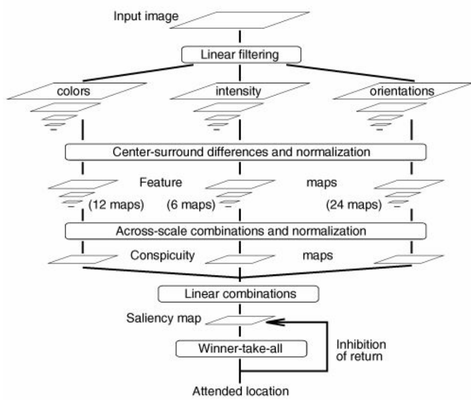
Figure 2.2. The flow of Static saliency algorithm of Itti et al. The general structure of the flow resembles the flow of Figure 2.1. Figure is taken from [20].
