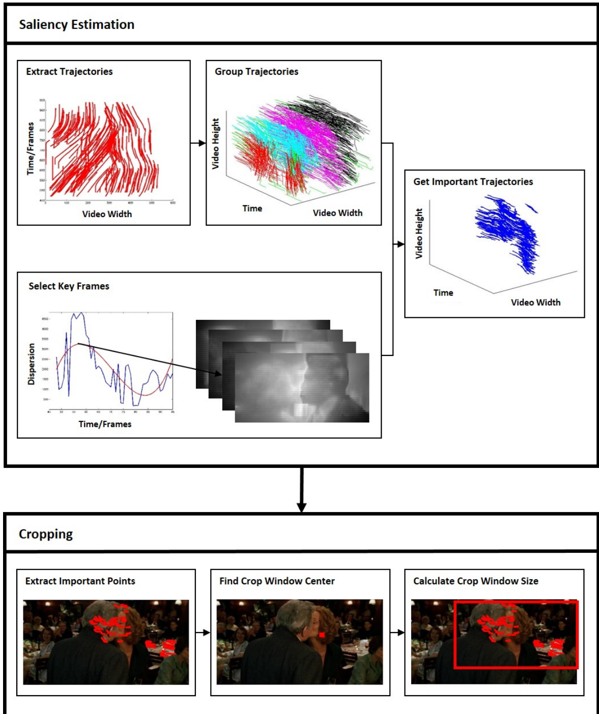
Figure 4.1. Overall flow of the proposed method.
