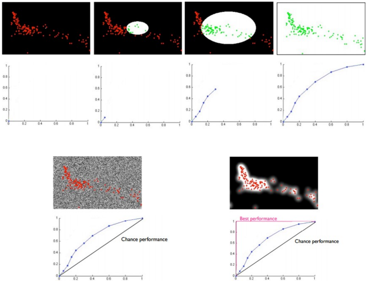
Figure 5.1. The first two row shows the steps while drawing the ROC curve of a selected image. The x axis of the ROC curve is the proportion of covered salient points (calculated) and the y axis is the proportion of the human fixations (green marks). The best possible saliency map and the random saliency map can be seen on the second row, along with their ROC curves.
