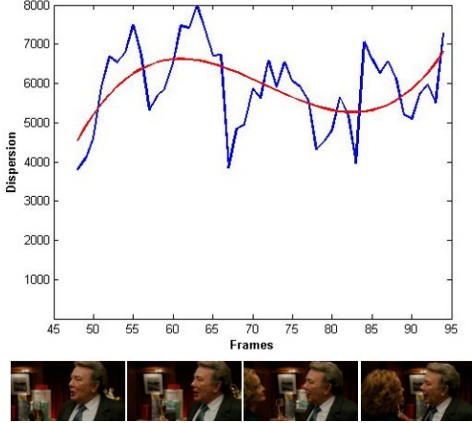
Figure 4.4. An example dispersion graph. Images correspond to the 50 th , 60 th , 70 th and 80 th frames respectively. As the woman enters the scene between 60 th – 70 th frames, the dispersion starts to increase.
