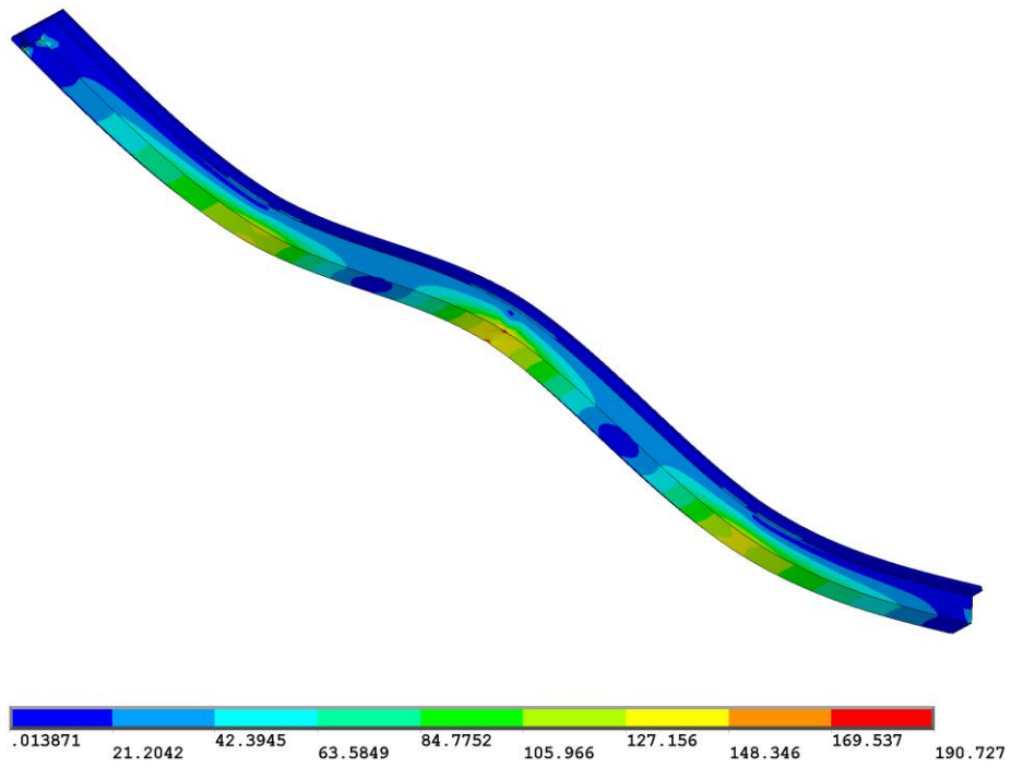
Figure 4.19 the model with dimensions in row (3) in Appendix B for stress.
