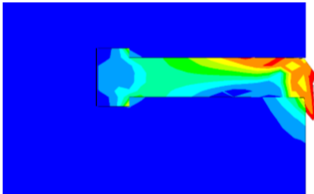
(a) Brick elements at load =127.9 kN
