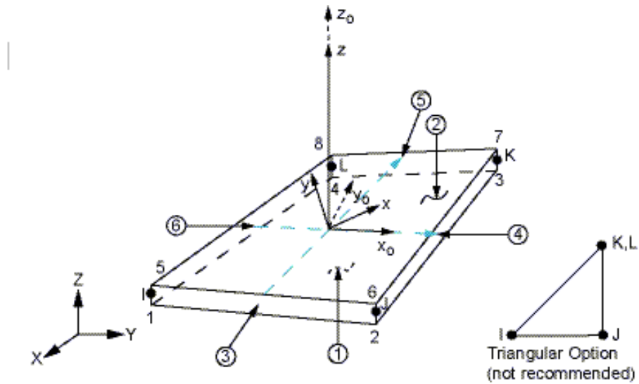
Figure 3.3 SHELL181 geometry [124].
