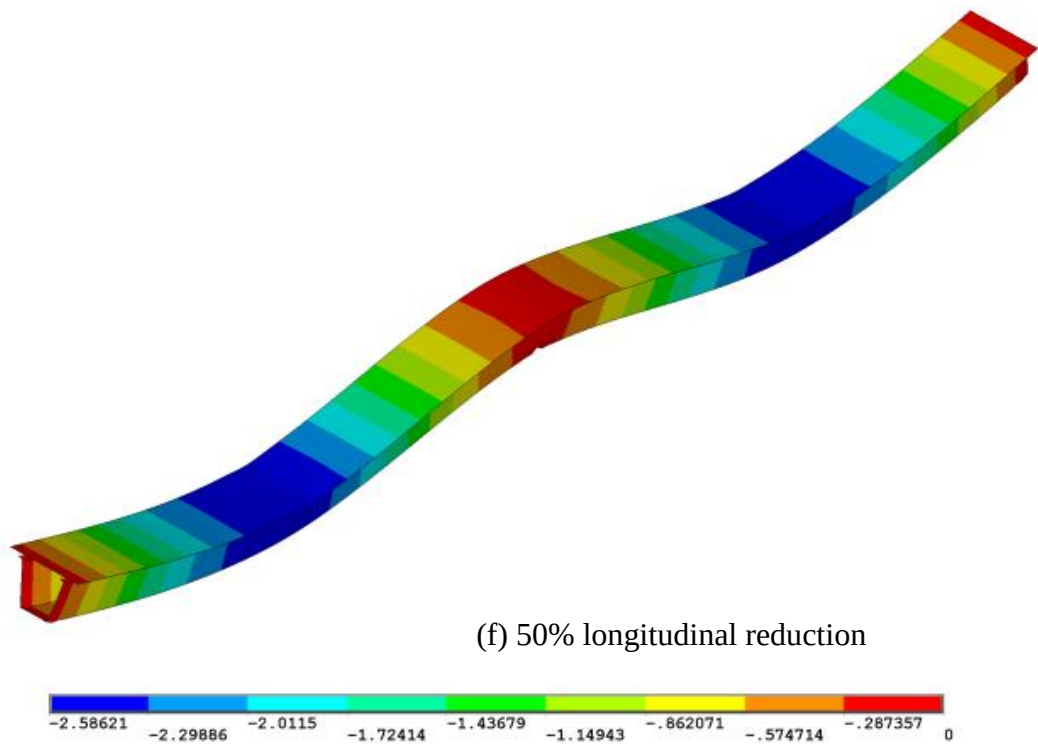
Figure 3.21 (continued) Deflections of numerical Model 2. (Magnification factor 400)
