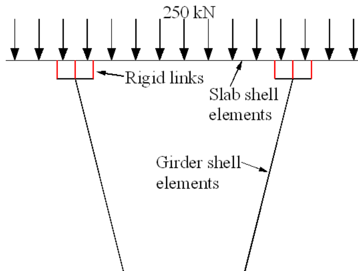
Figure 3.7 FE Model 2.
