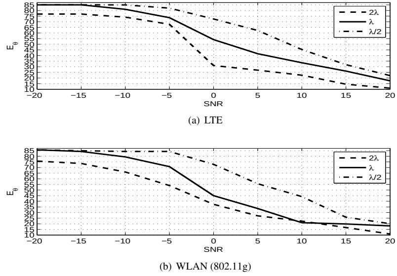
Figure 3.14: NLOS measurements: pt.2
