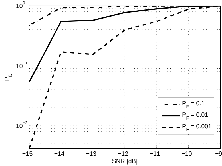
Figure 5.3: Probability of detection vs. SNR for NAC( \alpha )
