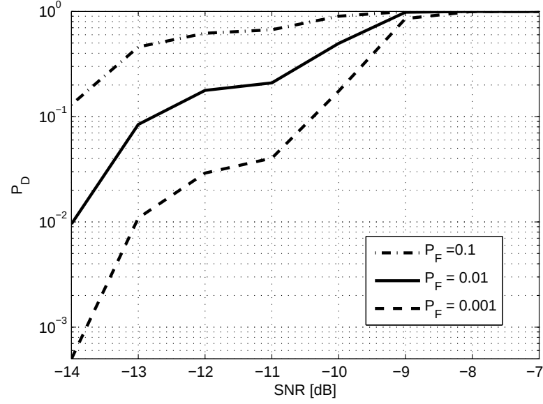
Figure 5.2: Probability of detection vs. SNR for CBD( \alpha )
