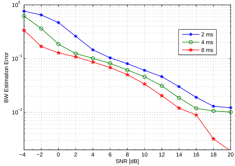
Figure 6.4: Bandwidth estimation performance
