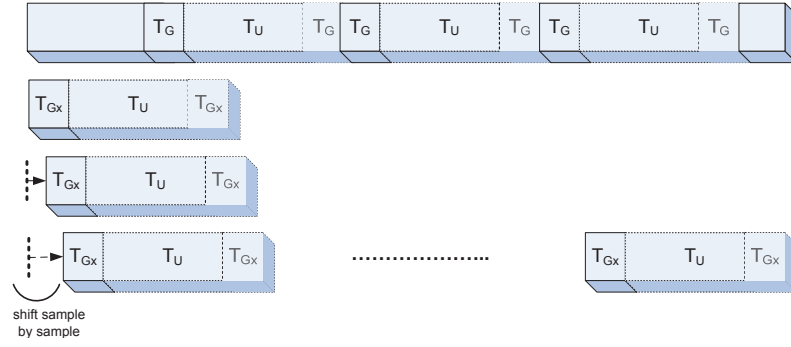
Figure 2.9: Sample by sample correlation
