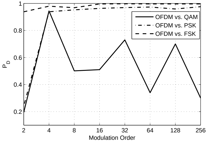
Figure 2.4: OFDM - SC separation: effect of modulation order
