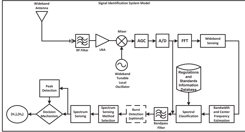
Figure 1.2: Signal identification block diagram
