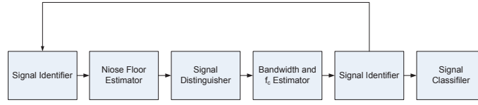
Figure 6.3: Recursive signal detection and parameter estimation block diagram
