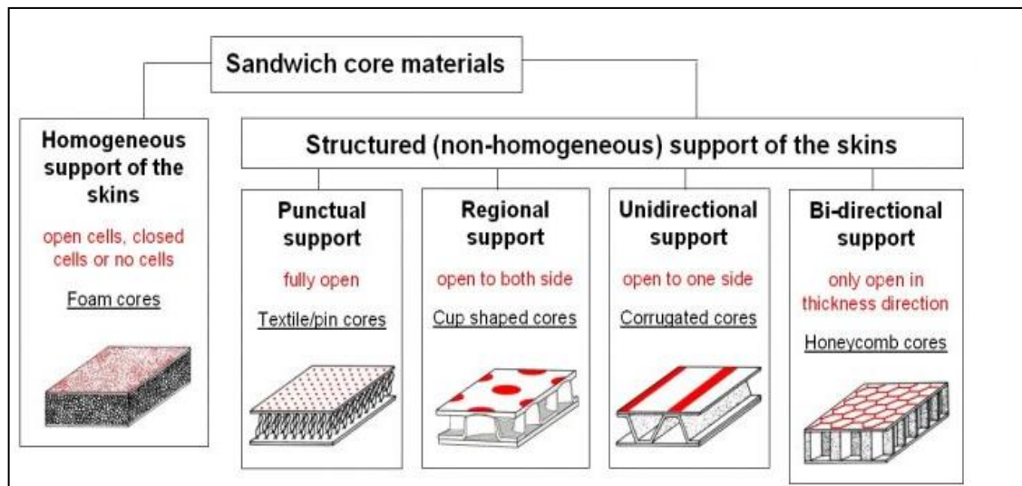
Figure 2.5 The core materials types of sandwich structures [29]
