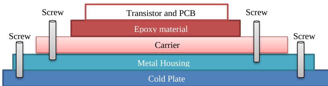
Figure 3.12 Typical thermal stack-up.
