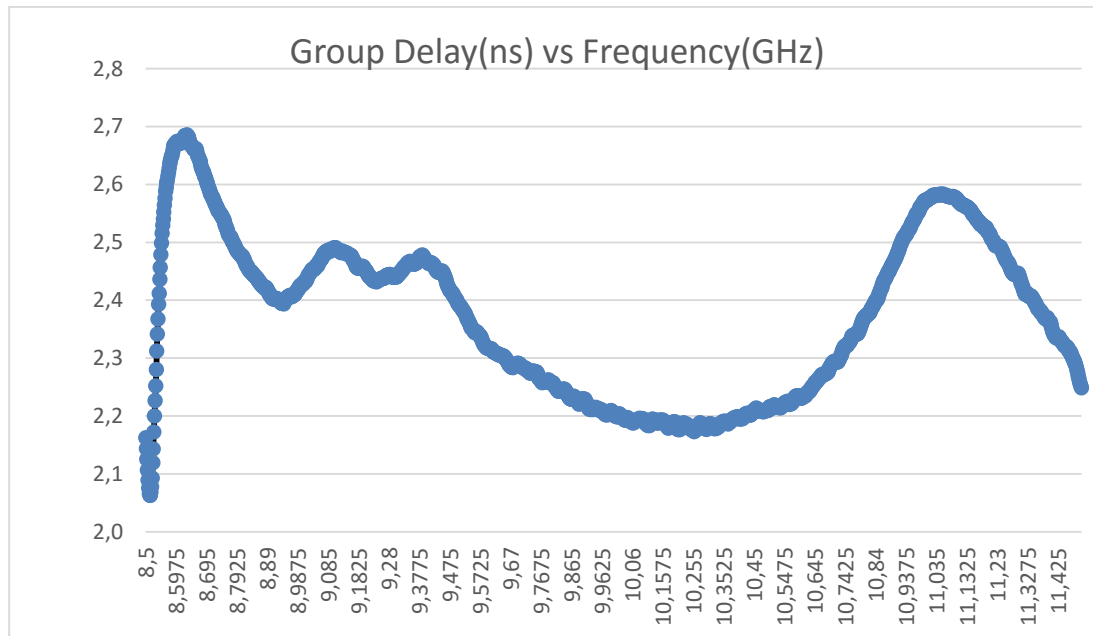
Figure 5.40 Group delay measurement of the constructed PA.
