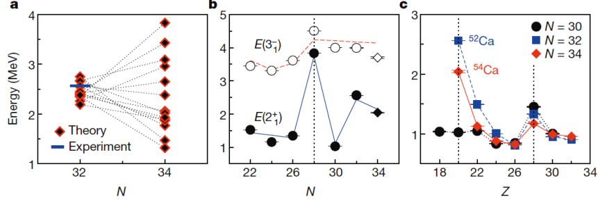
Figure 1.2 Excited-state energies of Ca isotopes and neighboring nuclei. The figure is taken from Ref. [50].
