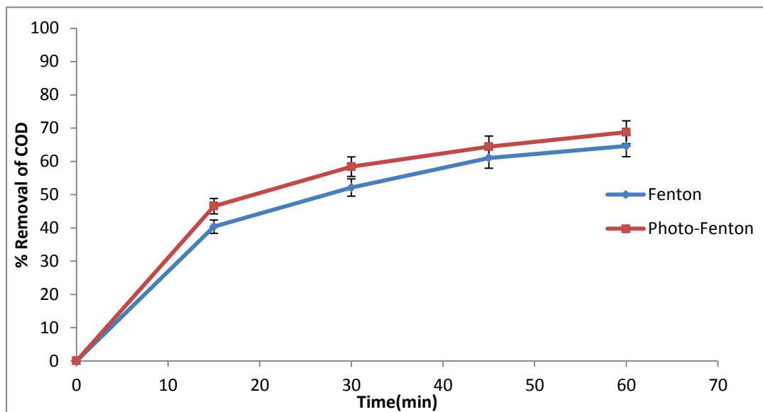
Figure 3.48. Effect of \text{Fe}_2\text{O}_3 particles on removal of COD using Fenton and Photo-Fenton reaction from solution which contain amoxicillin
