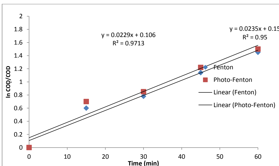
Figure 3.46. Pseudo-first order kinetic model plot of Fenton and Photo-Fenton oxidation for amoxicillin removal
