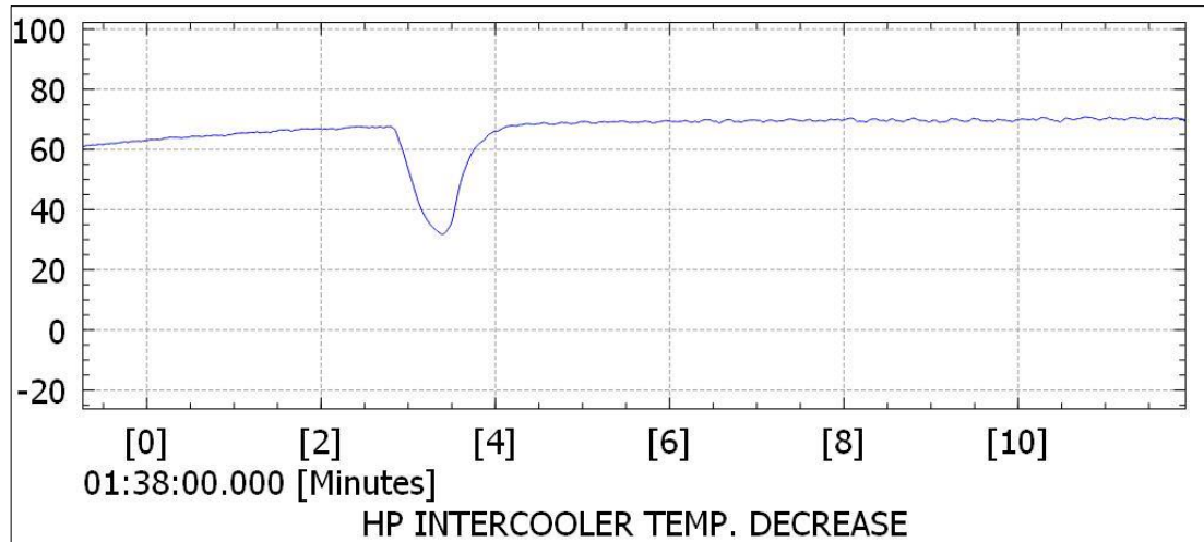
Figure 3.65: Test -3, Take Off – HP Intercooler Temperature Decrease Graph ( ^{\circ}\text{C} -min)
