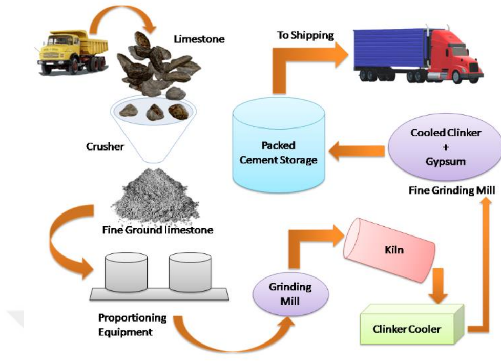
Figure 2. Flow diagram of cement production [3]
