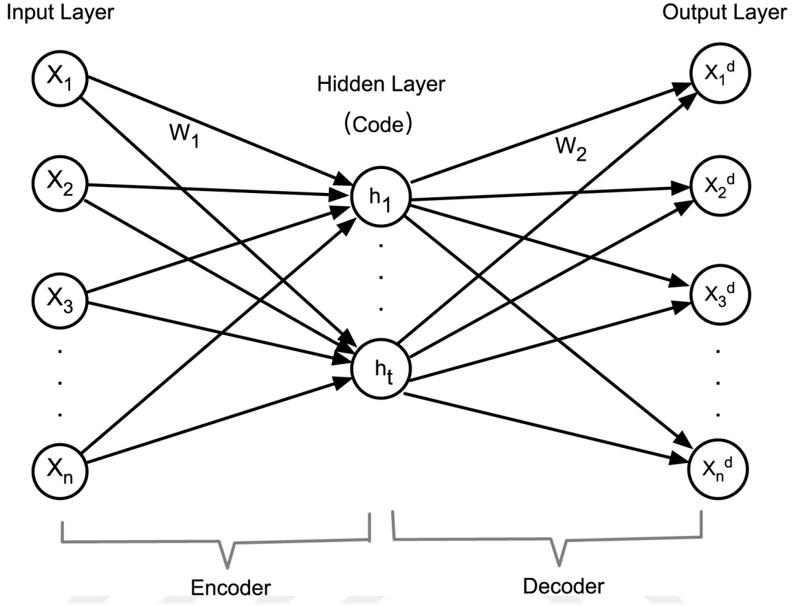
Figure 2.5 Structural diagram of an autoencoder: x represents the input data of the input layer, h denotes the hidden layer's data, and x_1 indicates the reconstructed output data in the output layer [33].
