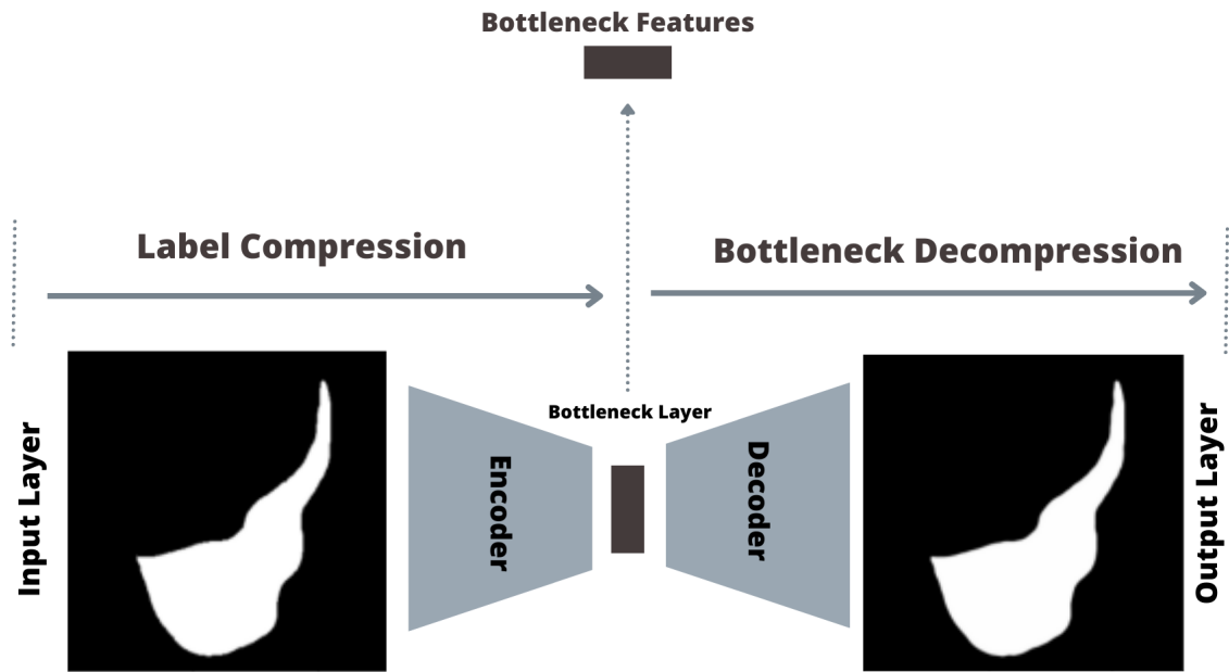
Figure 3.3 Decoder-Net
