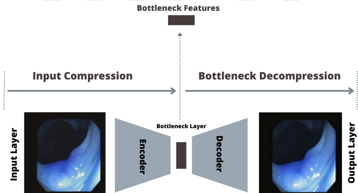
Figure 3.1 Encoder-Net
