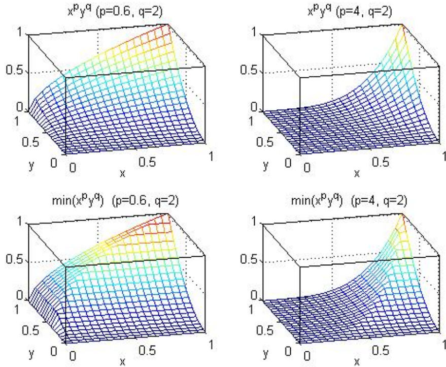
Figure 2.7. The corresponding surfaces for parameterized conjunctions T(x,y)=x^p y^q and T(x,y)=\min(x^p, y^q)
