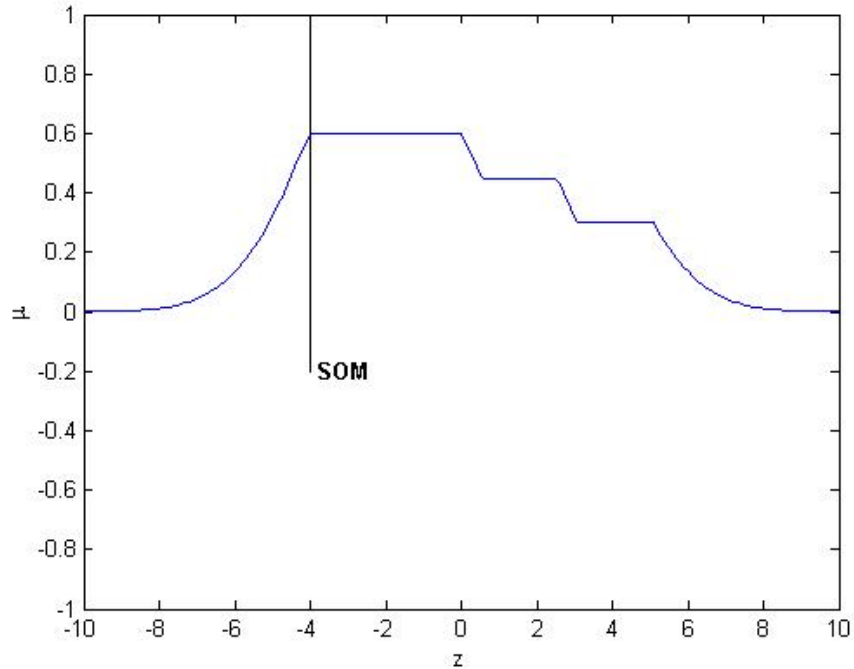
Figure 2.10. Smallest of Maximum (SOM) defuzzification method
