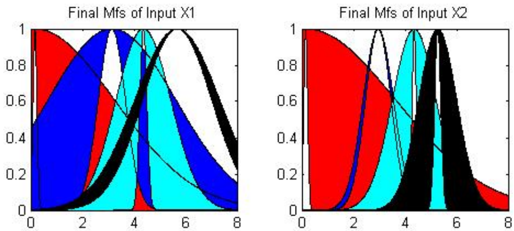
Figure 5.12. The interval type-2 gaussian membership functions with uncertain deviation after tuning with 0.40 uncertainty bound
