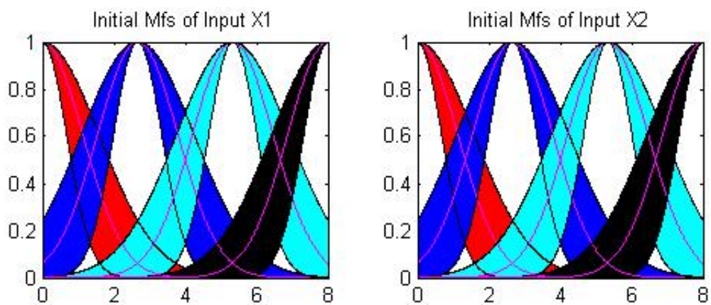
Figure 5.11. Initial interval type-2 Gaussian membership functions with uncertain standard deviation
