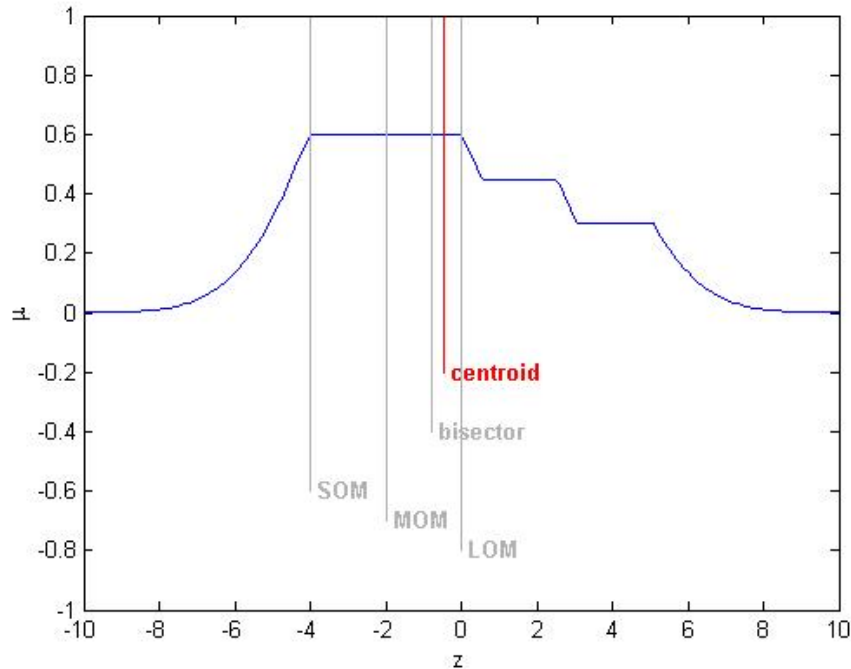
Figure 2.13. Five defuzzification methods
