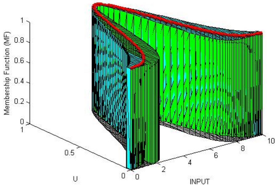
Figure 2.16. Interval Type-2 Gaussian membership function with uncertain standard deviation
