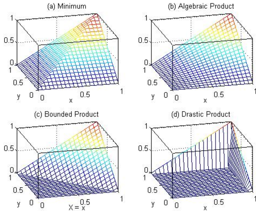
Figure 2.5. The corresponding surfaces of t-norms (a) Minimum, (b) Algebraic Product, (c) Bounded Product, (d) Drastic Product
