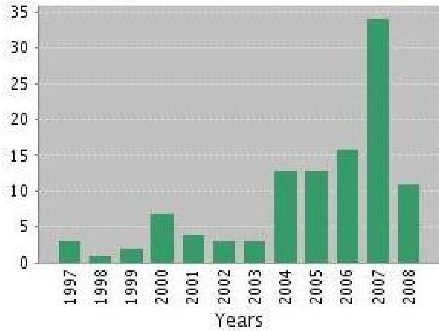
Figure 1.2. Citations in each year
