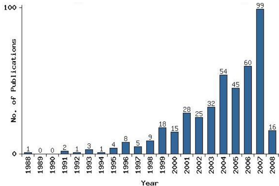
Figure 1.1. Number of publications in each year
