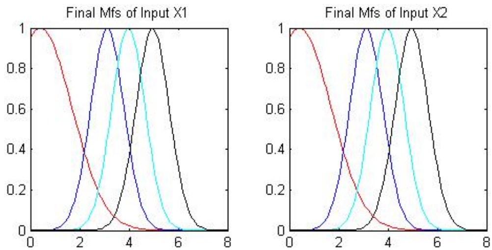
Figure 5.5. The membership functions after tuning CFSs
