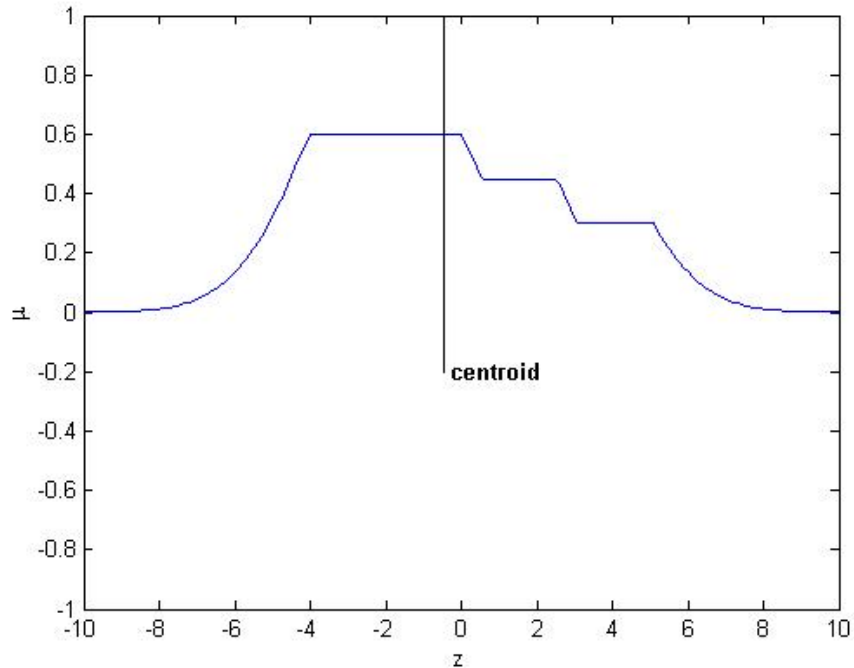
Figure 2.8. Center of area (Centroid) defuzzification method
