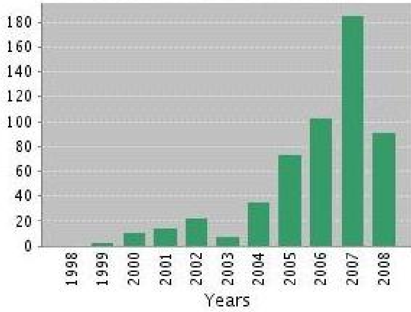
Figure 1.2. Citations in each year
