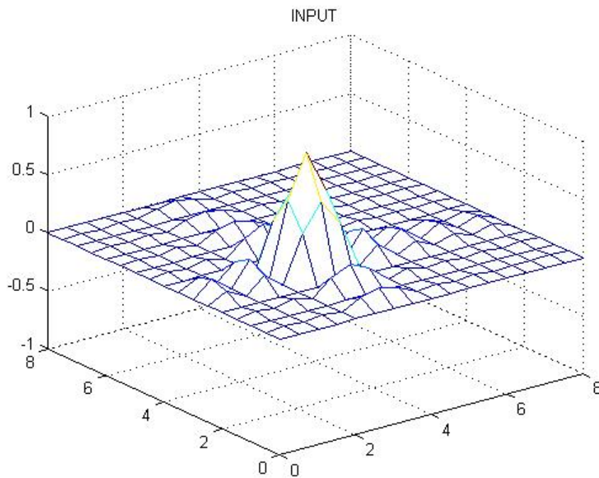
Figure 5.1. The sinc function that has global maximum at x_1 = 3.0, x_2 = 3.0
