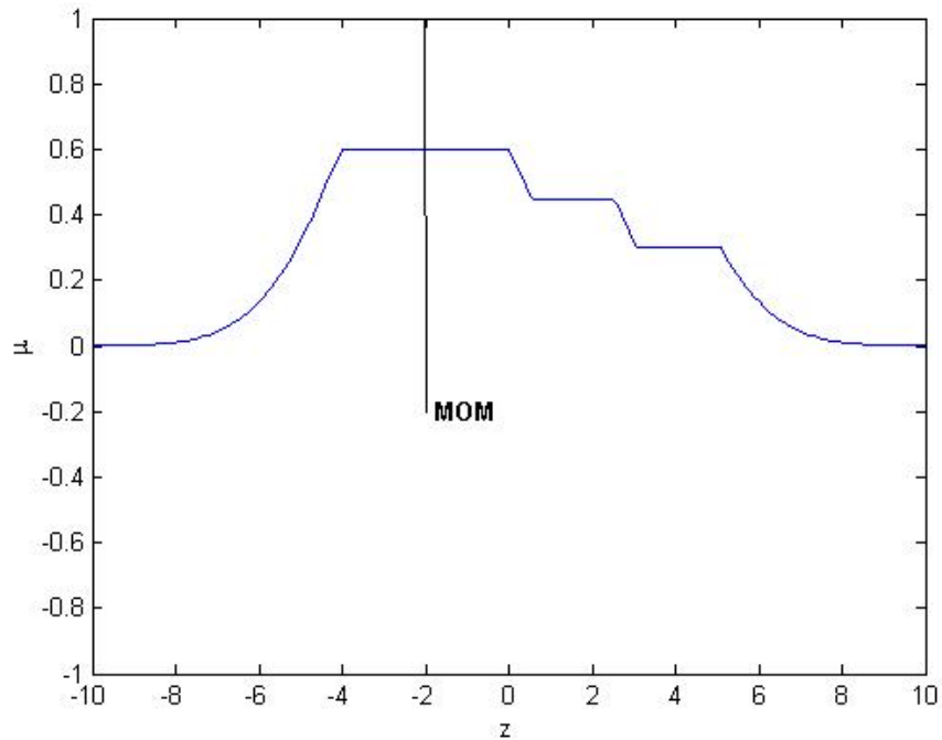
Figure 2.12. Mean of Maximum (MOM) defuzzification method
