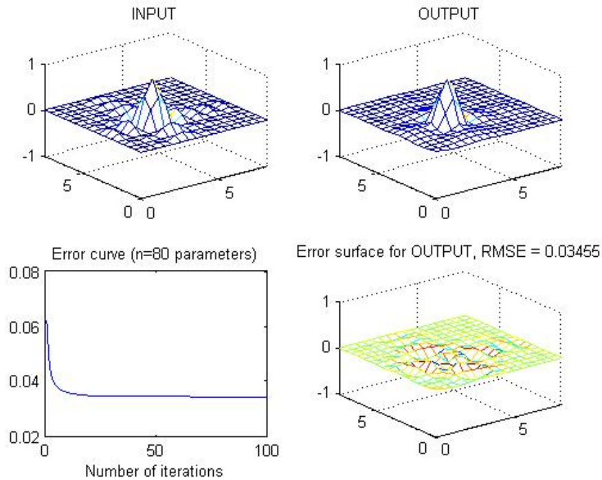
Figure 5.3. The result of approximating two input sinc function by using parameterized conjunction
