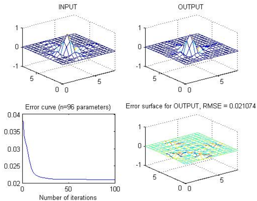
Figure 5.9. The result of approximating two input sinc function by using CFSs with parameterized conjunctions
