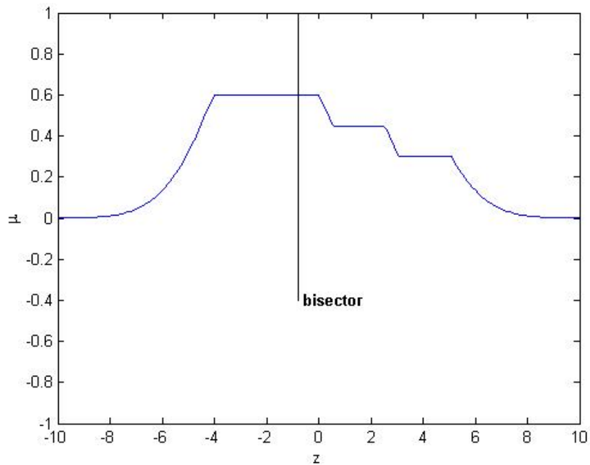
Figure 2.9. Bisector of area defuzzification method
