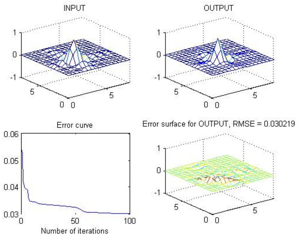
Figure 5.13. The result of approximating two input sinc function by using IT2 TSK Unnormalized Fuzzy Logic
