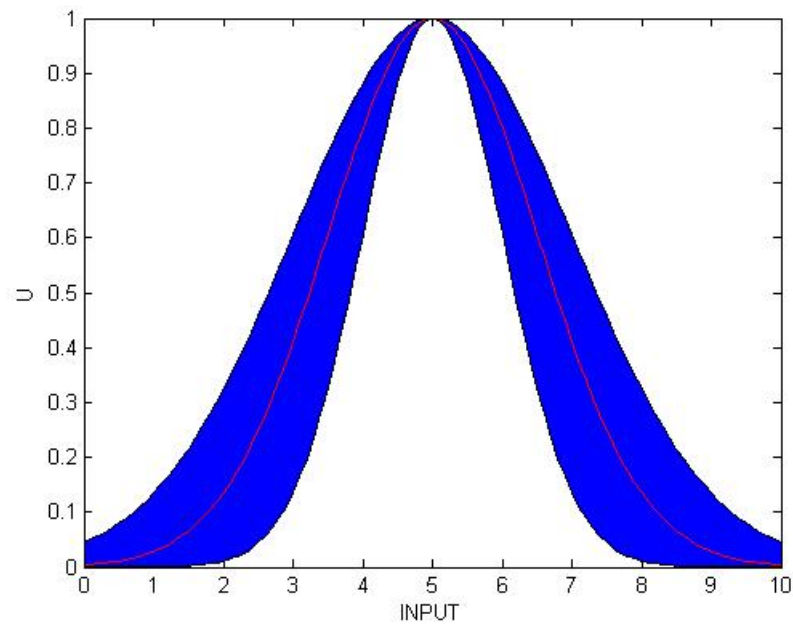
Figure 2.15. Diagram of Footprint of Uncertainty (FOU)
