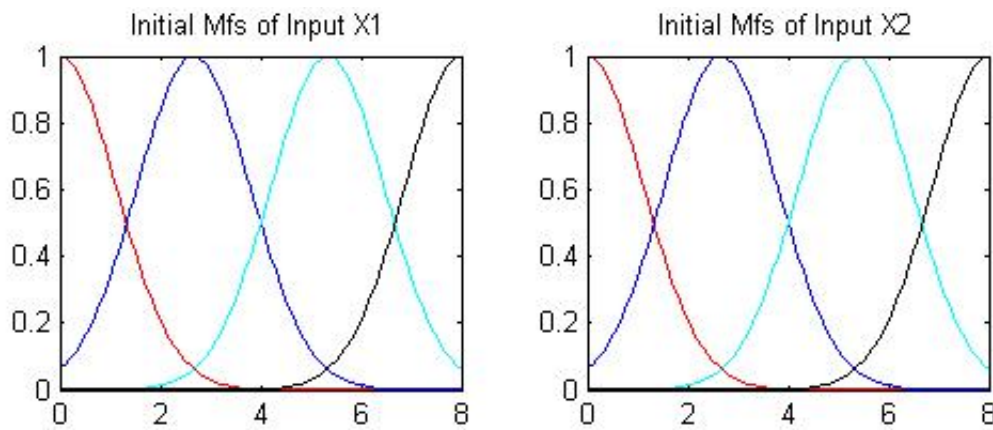
Figure 5.7. The Initial membership functions before tuning CFSs with parameterized conjunctions
