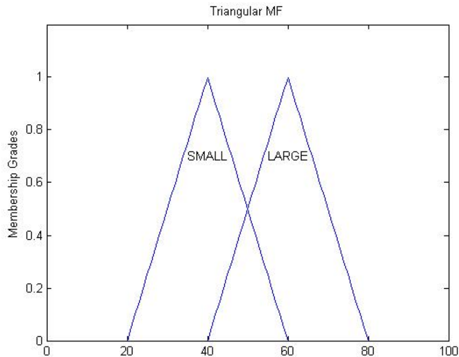
Figure 2.3. Triangular membership functions with linguistic values “Small”, “Large”
