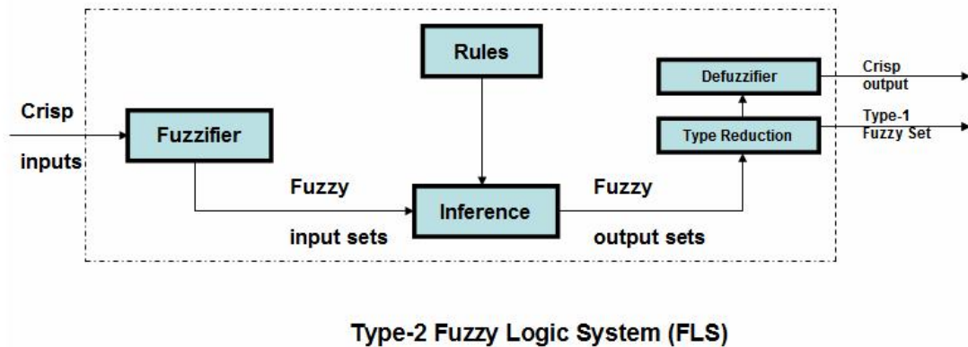
Figure 2.17. Block Diagram of Type-2 Fuzzy Logic Systems (T2FLSs)
