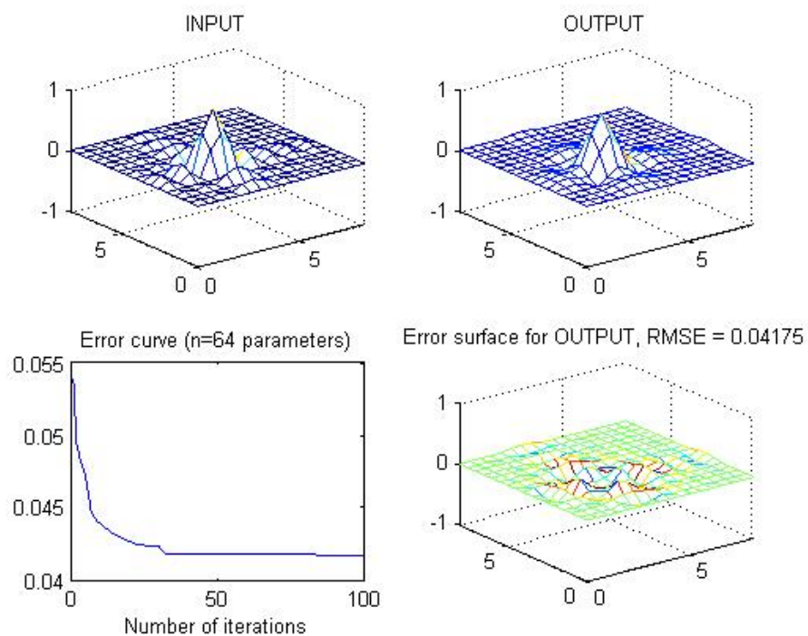
Figure 5.6. The result of approximating two input sinc function by using CFSs
