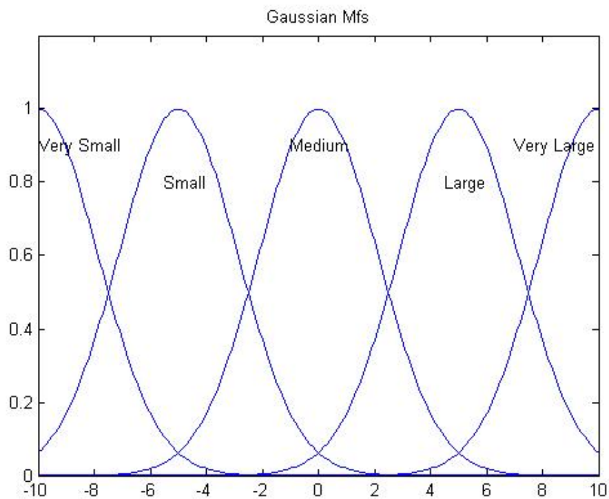
Figure 2.2. Gaussian membership functions with linguistic values “Very Small”, “Small”, “Medium”, “Large”, “Very Large”
