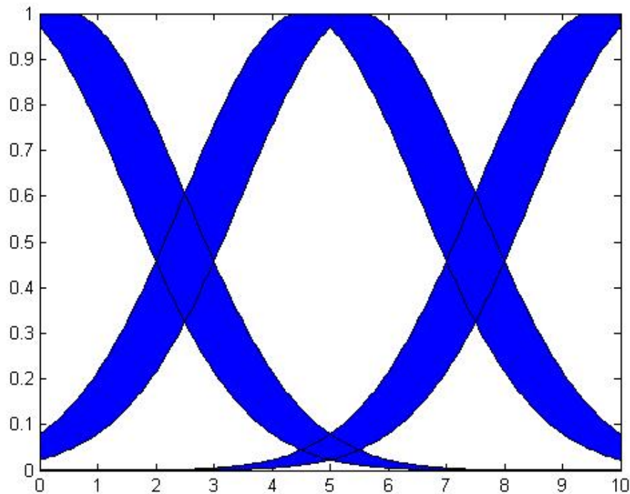
Figure 2.19. Gaussian primary membership function with uncertain mean
