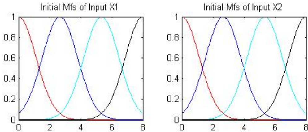
Figure 5.2. The membership functions that carry the expert knowledge
