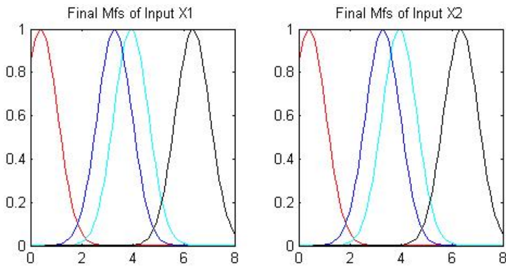
Figure 5.8. The membership functions after tuning CFSs with parameterized conjunctions
