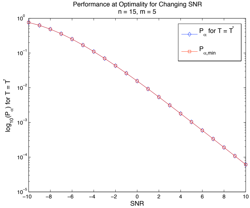
Figure 3.7. Performance of \mathbf{T}^* for changing SNR, P_\alpha indicates eigenvalue bound on P_\alpha .
