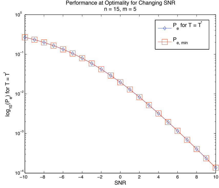
Figure 3.2. Performance of T^* for changing SNR, P_e indicates Chernoff bound on expected probability of error here. Also, SNR is in dB.
