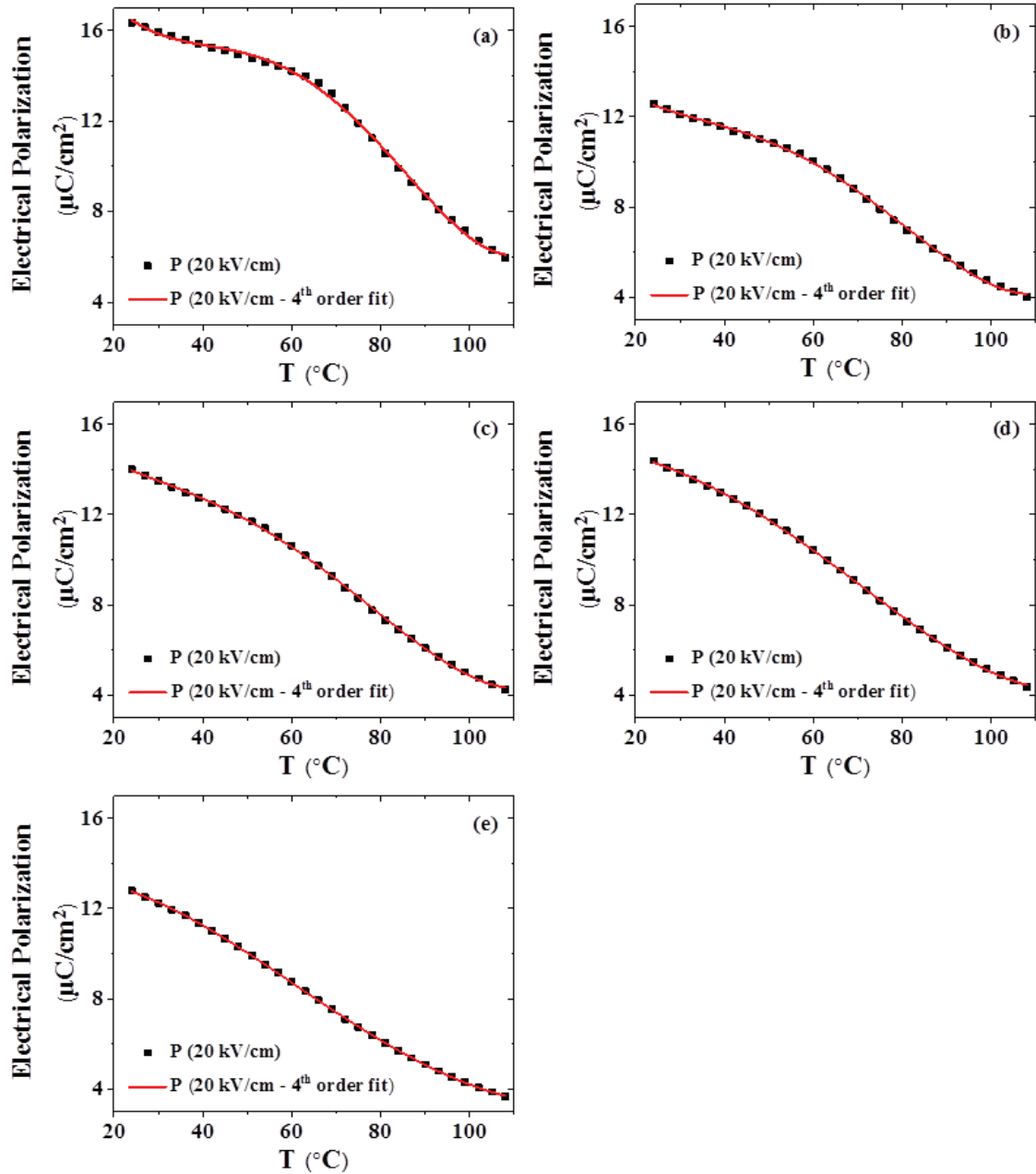
Figure 3.14. Fitted P-T curves of BSTZ x with (a) x=0 , (b) x=0.03 , (c) x=0.05 , (d) x=0.07 , (e) x=0.10 at 20 kV/cm electric field and 1 Hz.
