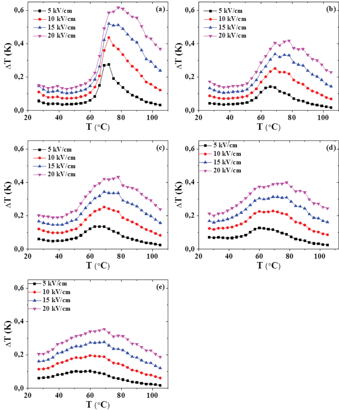
Figure 3.12. Numerically calculated \Delta T - T curves of \text{BSTZ}_x with (a) x=0 , (b) x=0.03 , (c) x=0.05 , (d) x=0.07 , (e) x=0.10 at various electric fields and 1 Hz.
