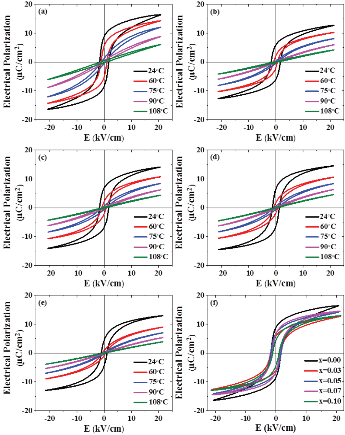
Figure 3.10. The P-E loops of BSTZ x ceramics for (a) x=0, (b) x=0.03, (c) x=0.05, (d) x=0.07, (e) x=0.10 and (f) comparison of all ceramics at 24°C and 1 Hz.
