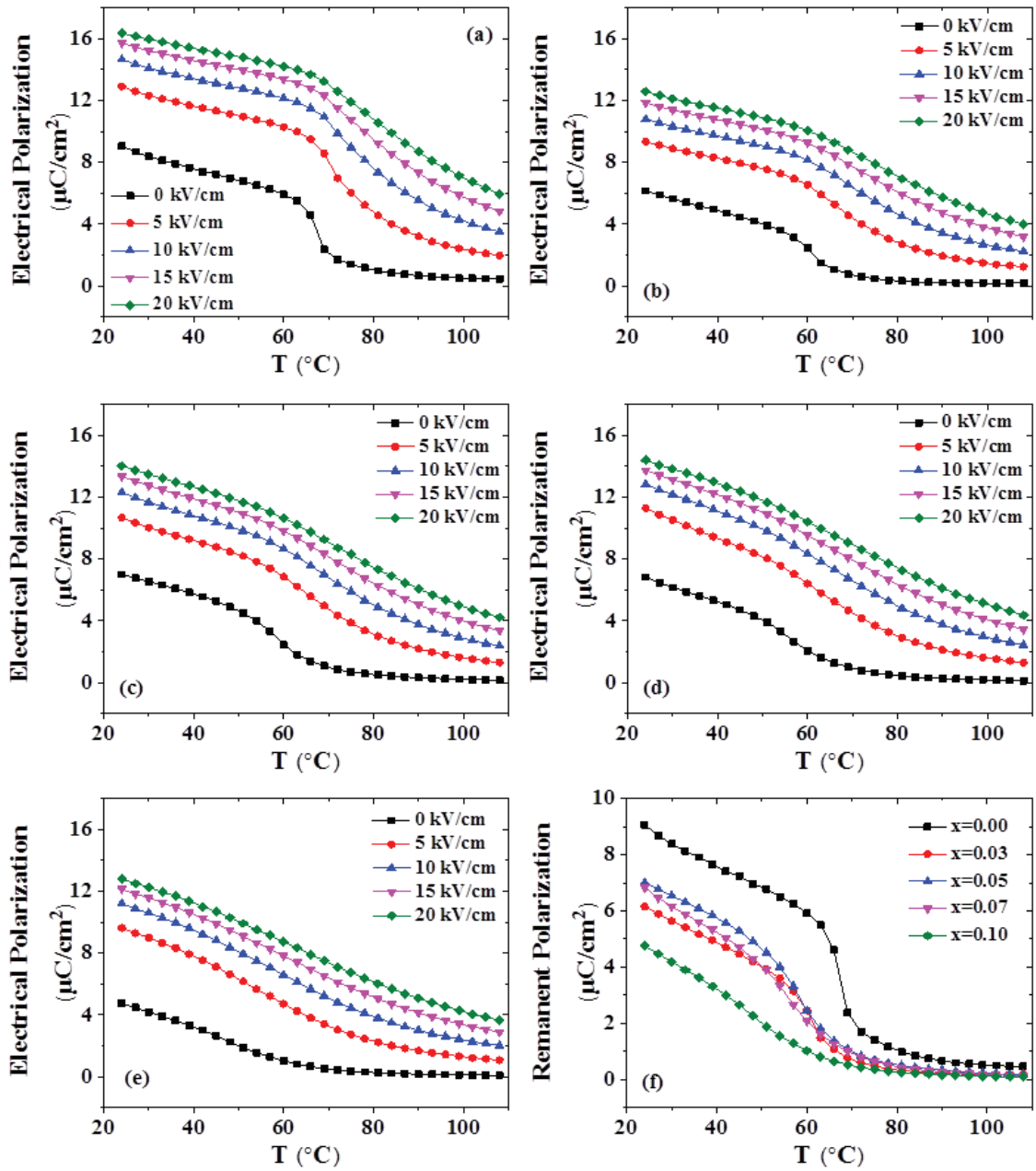
Figure 3.11. The P-T curves of BSTZ x with (a) x=0 , (b) x=0.03 , (c) x=0.05 , (d) x=0.07 , (e) x=0.10 at various electric fields and 1 Hz and (f) comparison of remanent polarization of all compositions.
