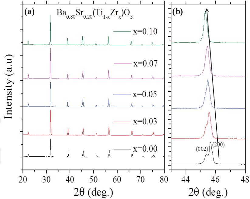
Figure 3.2. XRD patterns of sintered BSTZ x samples for 0 \leq x \leq 0.10 in the range of 2\theta (a) from 20^\circ to 80^\circ and (b) close examination between 43^\circ - 48^\circ .
