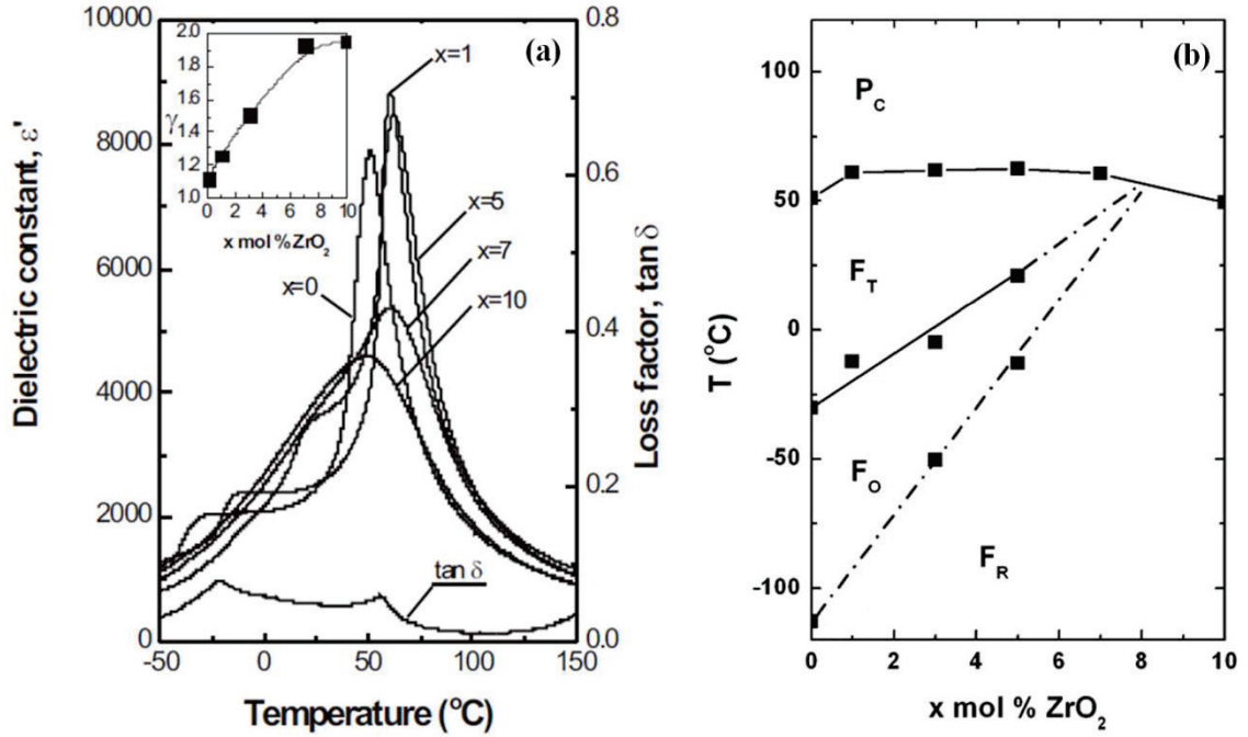
Figure 1.12. (a) Dielectric constant values for BSTZ x ceramics ( 0 \leq x \leq 0.10 ) and dielectric loss for x=0.01 as a function of temperature at 1 kHz. Inset shows diffuseness exponent, \gamma and Zr content. (b) Temperature-Composition (T-x) phase diagram of BSTZ x ceramics for 0 \leq x \leq 0.10 . 39
