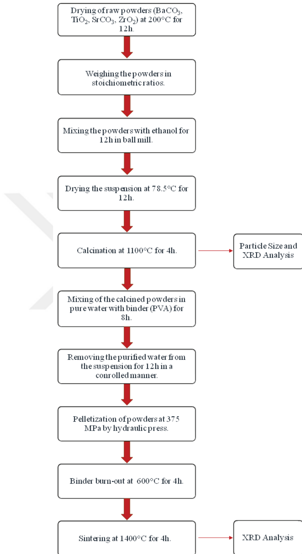
Figure 2.1. Flow chart of the synthesis.
