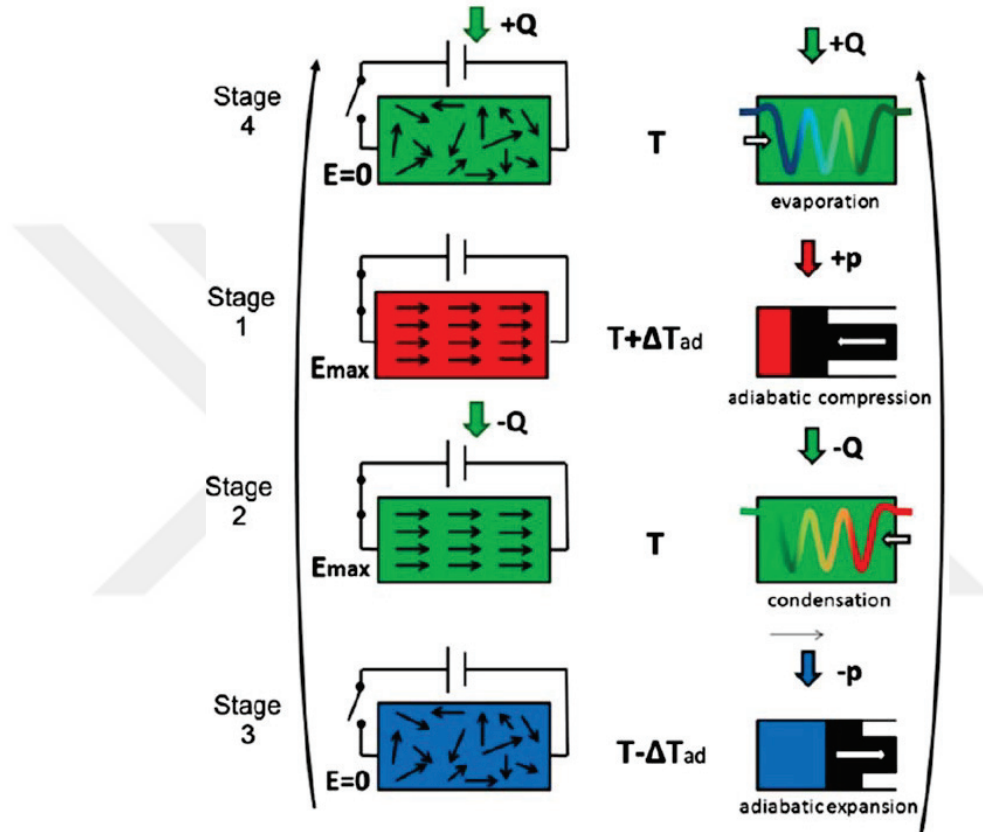
Figure 1.2. Schematic presentation of the EC solid-state cooling cycle (left) and traditional vapor-compression cooling cycle (right). 1
