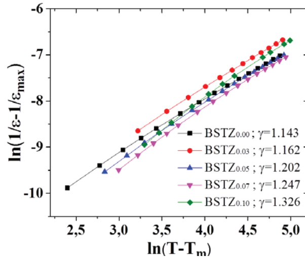
Figure 3.8. Diffuseness constants ( \gamma ) of BSTZ x ceramics.
