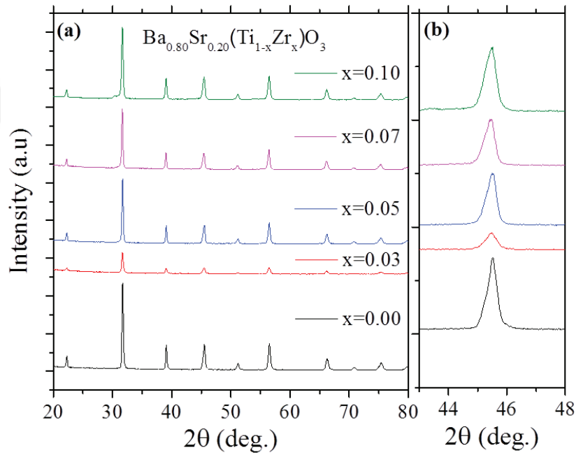
Figure 3.1. XRD patterns of calcined BSTZ x samples for 0 \leq x \leq 0.10 in the range of 2\theta (a) from 20° to 80° and (b) close examination between 43°-48°.
