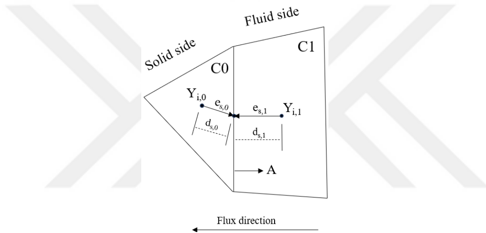
Figure 3.8: Schematic representation of adapted conjugated boundary
