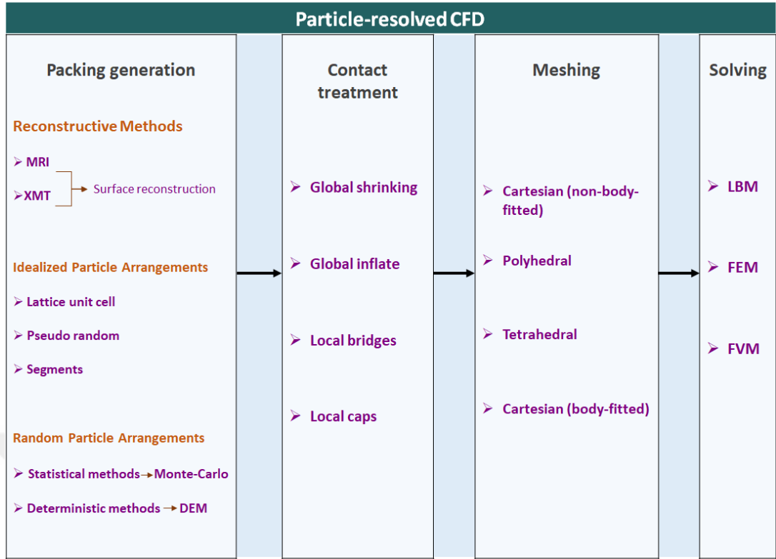
Figure 2.4: General workflow of particle-resolved CFD methodology. Adapted from [1].
