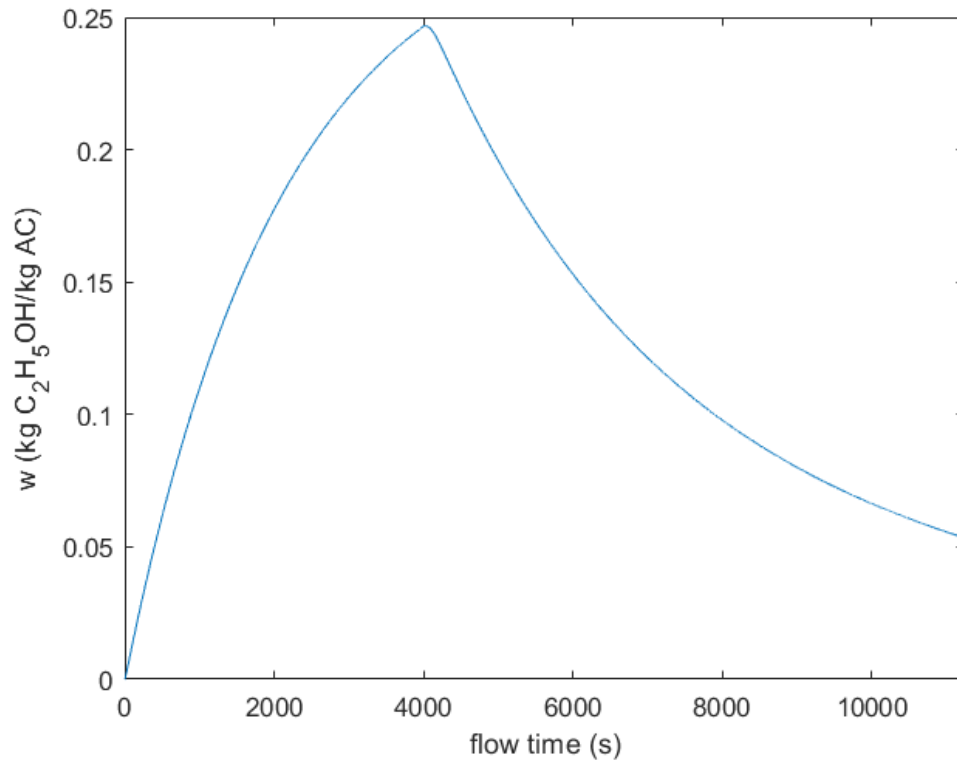
Figure 4.12: Volume-averaged adsorbed amount ( w ) profile during adsorption-desorption cycle at 30°C.
