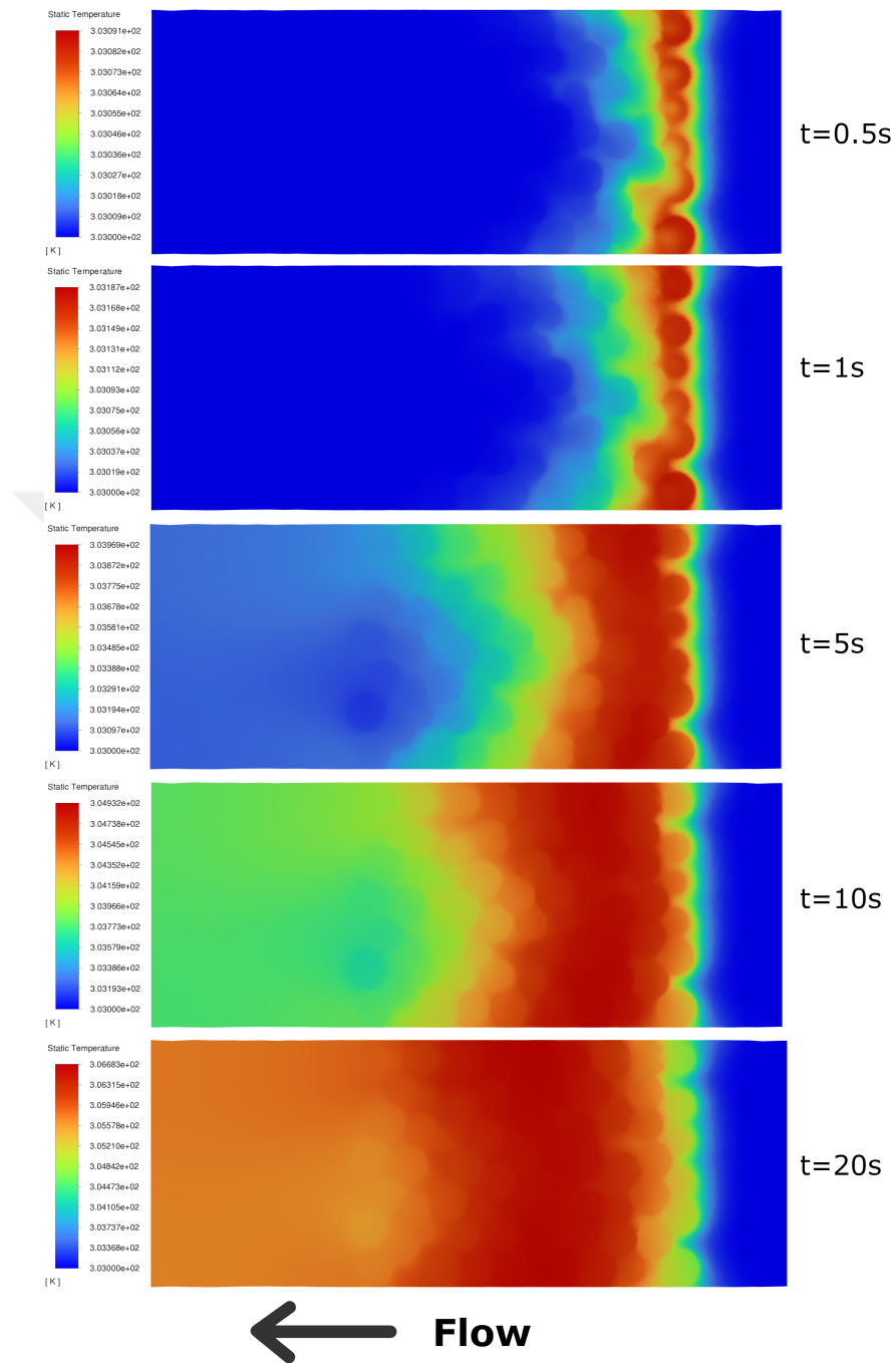
Figure 4.7: Temperature contours along the bed at the mid-plane ( x=0 ) during start-up at 30^\circ\text{C} .
