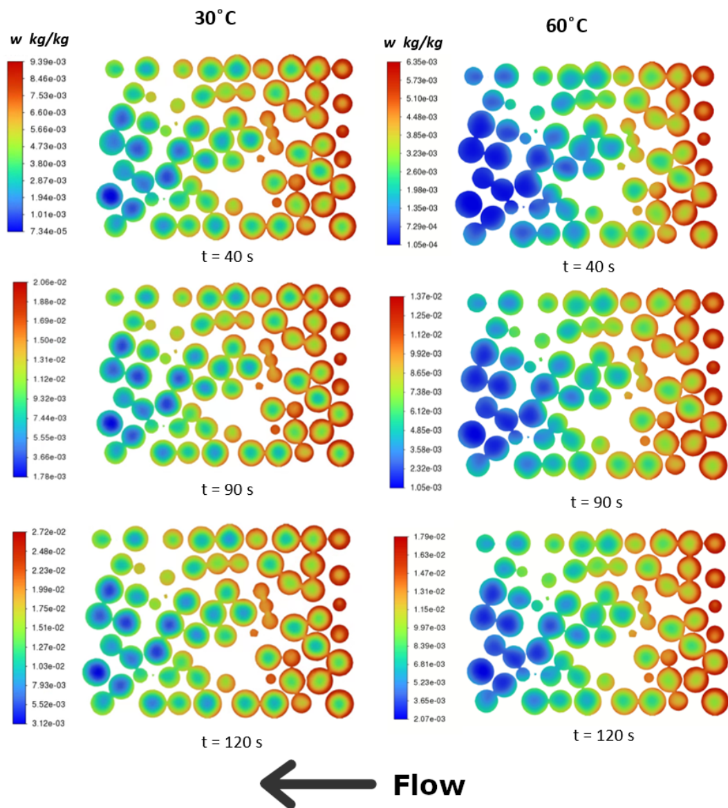
Figure 4.8: Amount adsorbed w (kg \text{C}_2\text{H}_5\text{OH} /kg activated carbon) contours along the bed at the mid-plane ( x=0 ) at different times for 30^\circ\text{C} and 60^\circ\text{C} .
