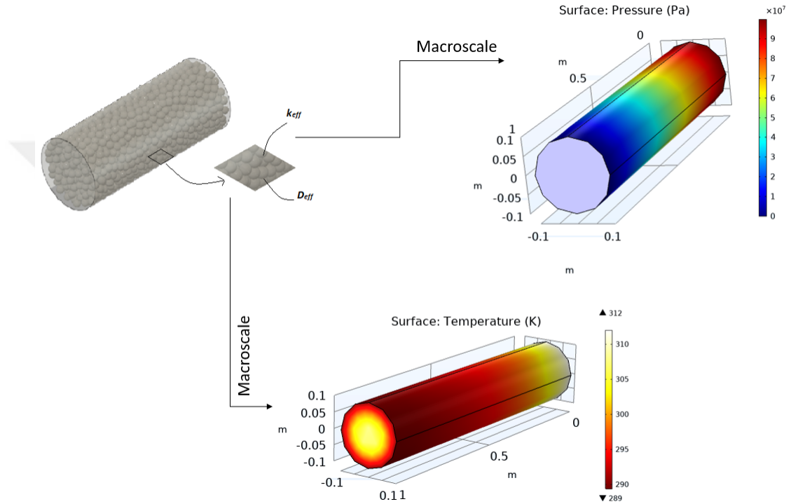
Figure 2.2: Contour plots of pressure and temperature resulting from homogeneous model utilization.
