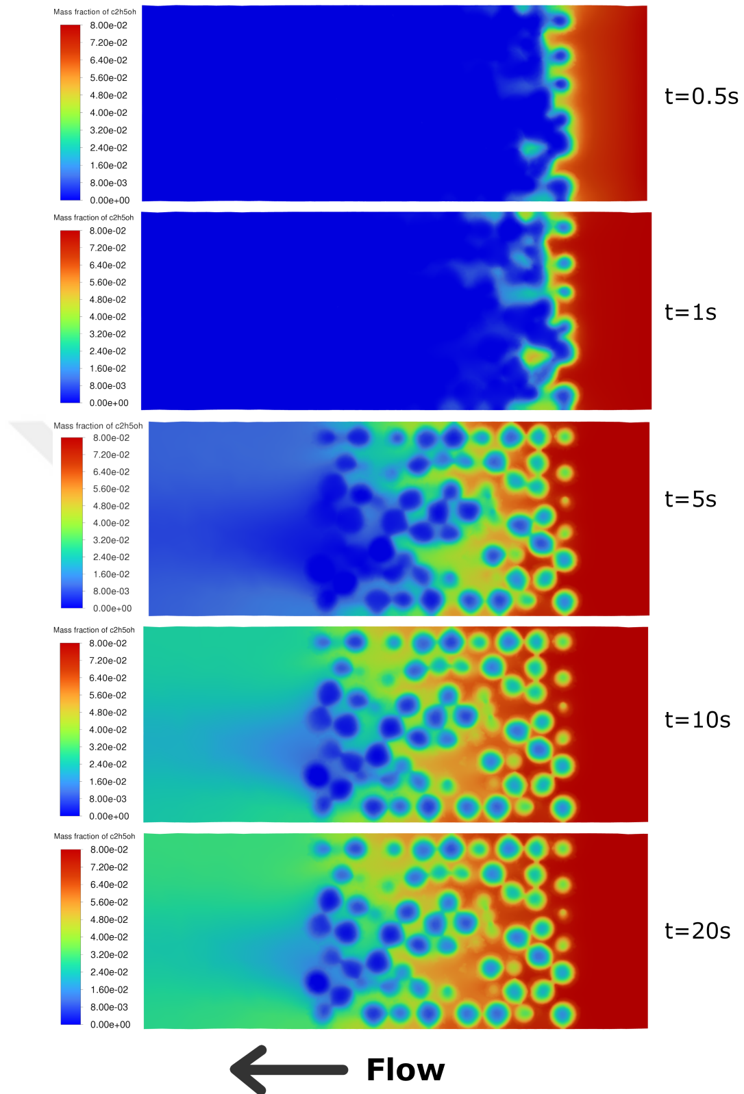
Figure 4.6: Mass fraction contours of ethanol along the bed at the mid-plane ( x=0 ) during start-up at 30°C.
