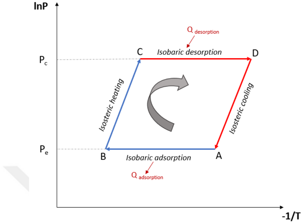
Figure 1.1: Clapeyron diagram of an adsorption heat pump.
