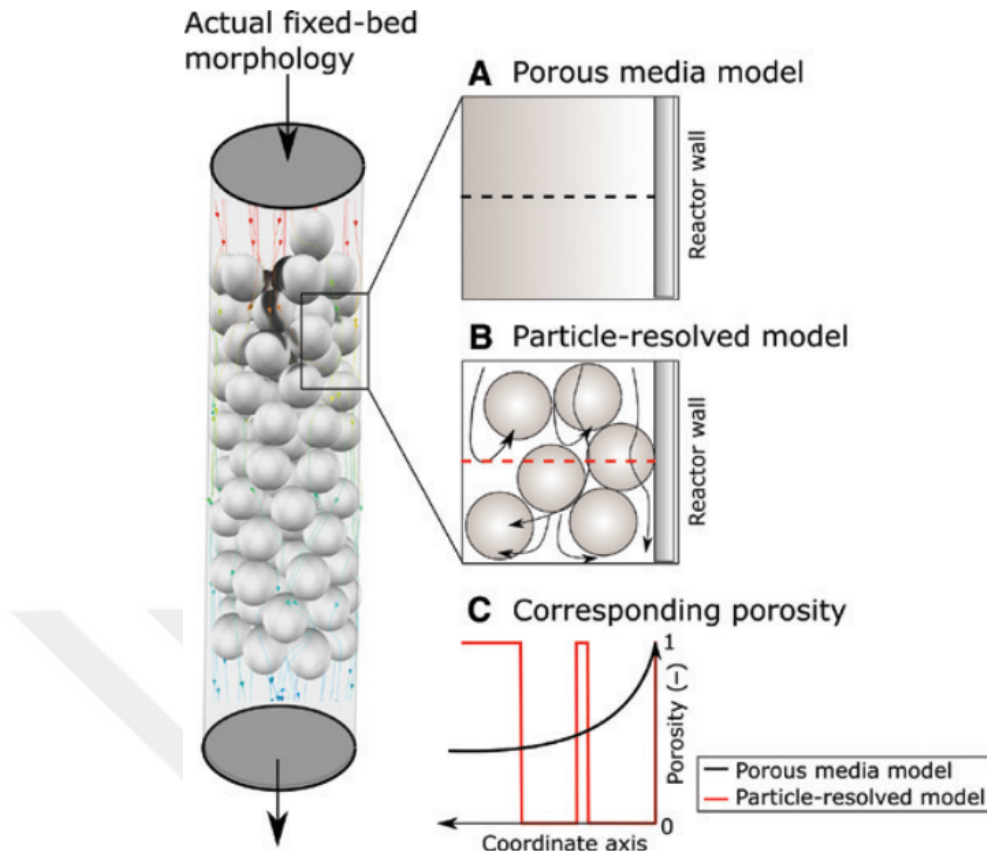
Figure 2.3: Porosity variations in particle-resolved model and porous media model [1].
