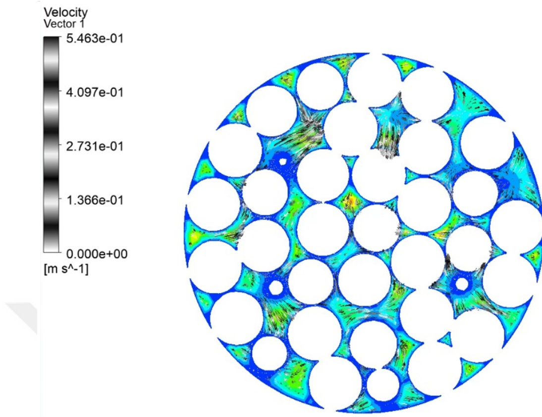
Figure 4.4: (a) Velocity vector and contour at an arbitrary radial plane.
