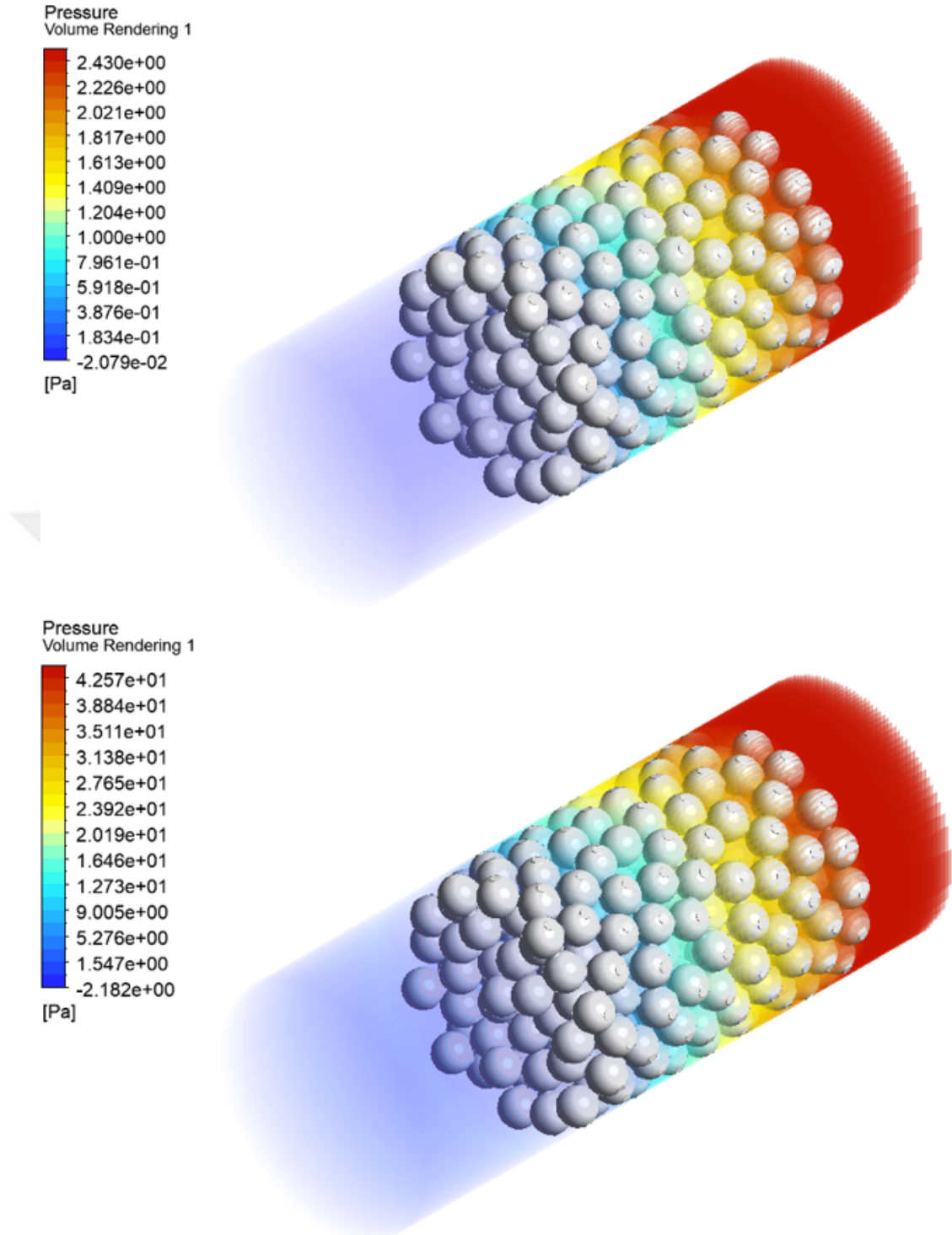
Figure 4.2: Static pressure volume rendering along the bed for (a) v_{in} = 0.05 m/s, Re_p = 12 (b) v_{in} = 0.05 m/s, Re_p = 120 .
