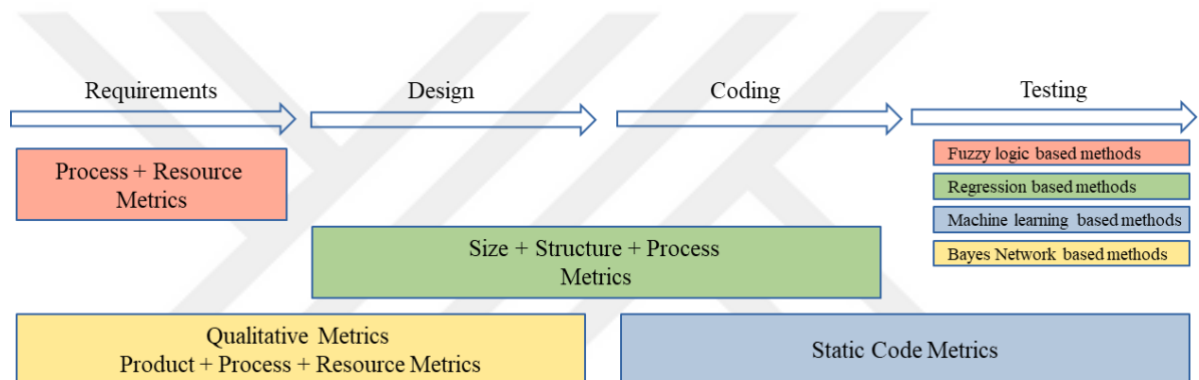
Figure 6.1. Recommended methods related to Waterfall phases with the most successful metric suites
