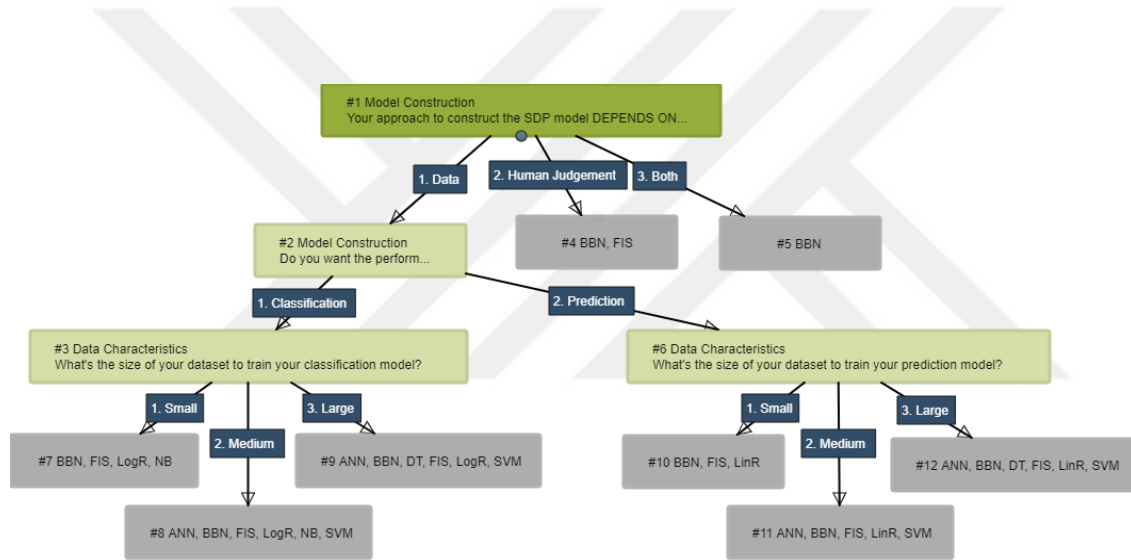
Figure 4.3. Decision tree for the phase–1 of the decision analysis process
