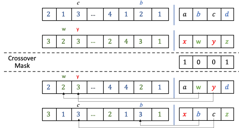
Figure 6.6: An example for Crossover Exception II
