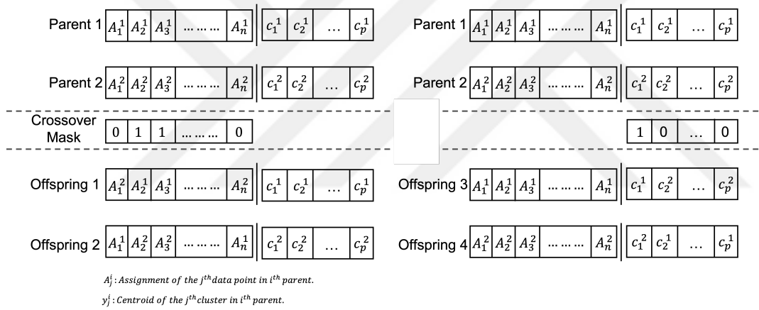
Figure 6.4: Uniform Crossover Operator for CCBFS-H
