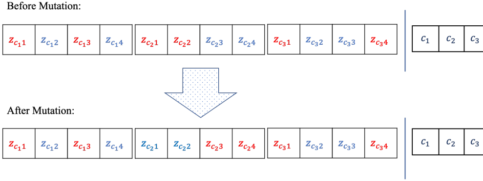
Figure 4.9: An example for Mutation - Type 2
