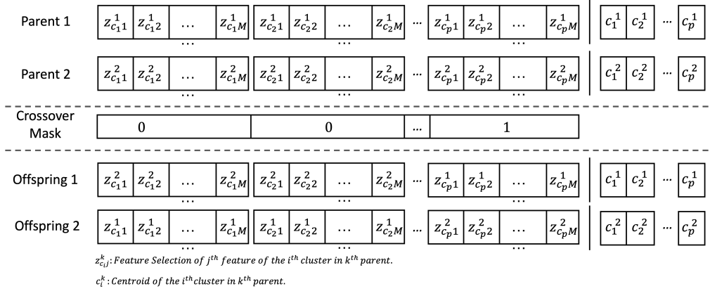
Figure 4.6: Uniform Crossover Operator to Create First Two Offsprings
