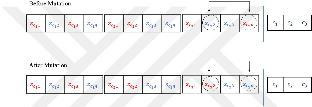
Figure 4.8: An example for Mutation - Type 1
