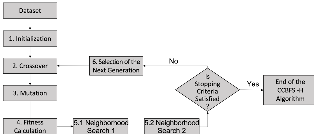
Figure 6.1: Flowchart of the CCBFS-H Algorithm
