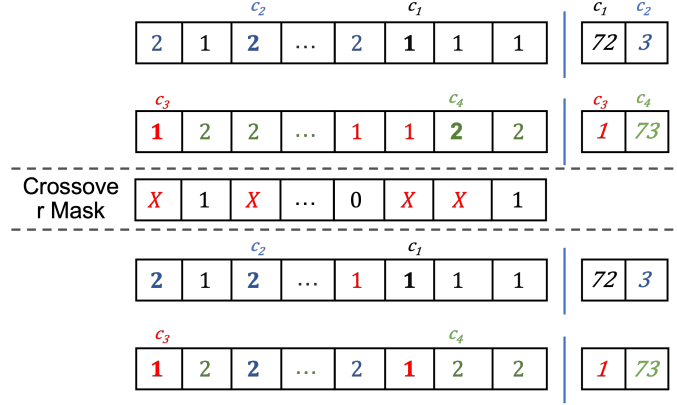
Figure 6.5: An example for Crossover Exception I
