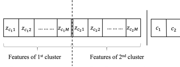
Figure 4.5: Desirable chromosome split
