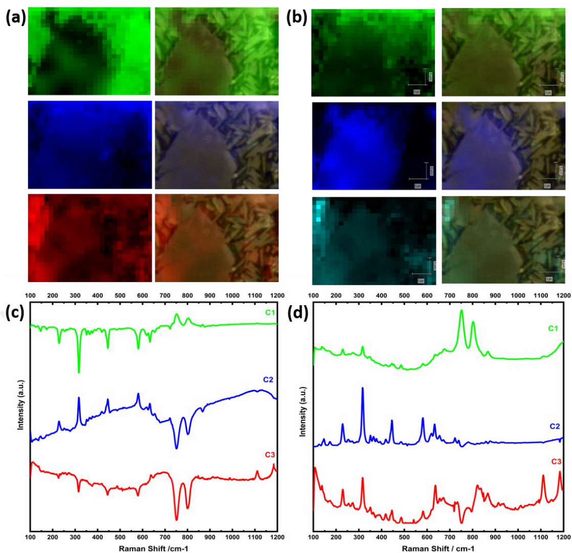
Figure 5.12 Comparison of PCA and MCR-ALS method for the S4A7ED 30 mol% B 2 O 3 .
