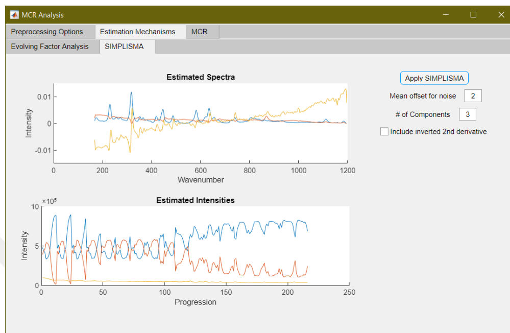
Figure 5.20 SIMPLISMA subtab of the Estimation Mechanisms (From Ahmet Alper Özkan graduation Project).
