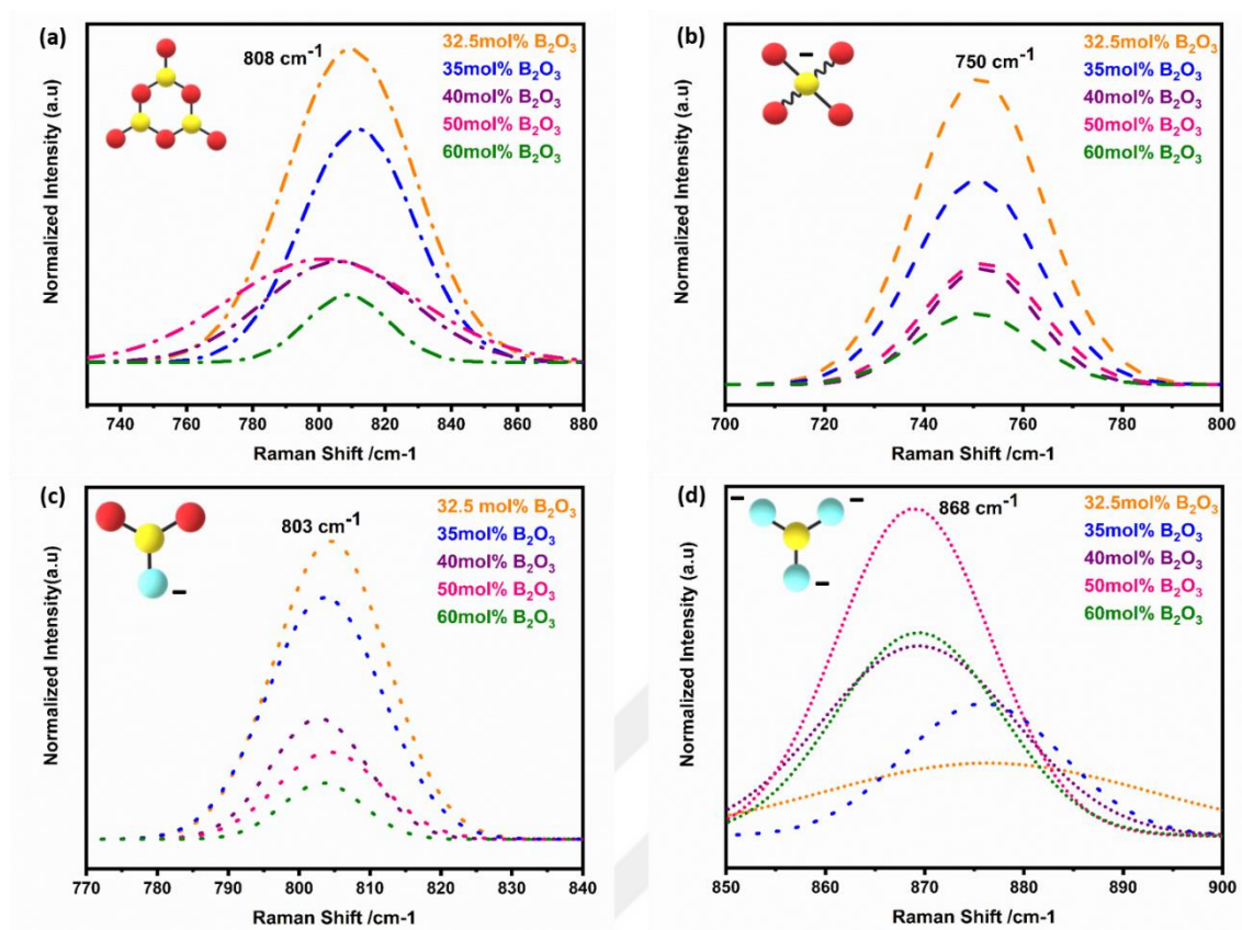
Figure 3.8 Deconvoluted Raman-shift spectra for S4A7ED x B ( 30 \leq x \leq 60 mol% B 2 O 3 ) for vibrations of a) boroxyl rings of corner-sharing [BØ 3 ]; b) [BØ 4 ]; c) metaborate [BØ 2 O]; d) orthoborate (monomers of [BO 3 ] 3- ).
