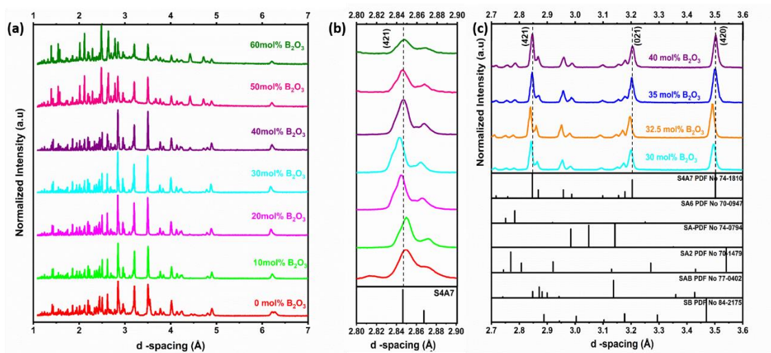
Figure 3.2 X-ray diffractograms of S4A7EDxB ( 0 \leq x \leq 60 mol% B 2 O 3 ) a) full range; b) magnified around the (421) diffraction peak; c) diffractograms for S4A7EDxB ( 30 \leq x \leq 40 mol% B 2 O 3 ).
