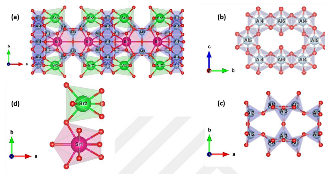
Figure 1.1 a) Components of the \text{Sr}_4\text{Al}_{14}\text{O}_{25} unit cell viewed along the [001]; b) 6 oxygen-coordinated alumina scaffold; c) 4 oxygen-coordinated alumina scaffold; d) the coordination polyhedra of Sr (1) site (Wyckoff 4j) and Sr (2) site (Wyckoff 4i).
