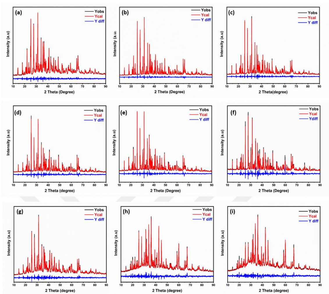
Figure 3.4 Rietveld refinement from the X-ray powder diffraction data plots of a) S4A7ED 0 mol% B 2 O 3 ; b) S4A7ED 10 mol% B 2 O 3 ; c) S4A7ED 20 mol% B 2 O 3 ; d) S4A7ED 30 mol% B 2 O 3 ; e) S4A7ED 32.5 mol% B 2 O 3 ; f) S4A7ED 35 mol% B 2 O 3 ; g) S4A7ED 40 mol% B 2 O 3 ; h) S4A7ED 50 mol% B 2 O 3 ; i) S4A7ED 60 mol% B 2 O 3 . Observed (black solid line); calculated (red solid line) and difference (blue solid line) patterns data taken at room temperature.
