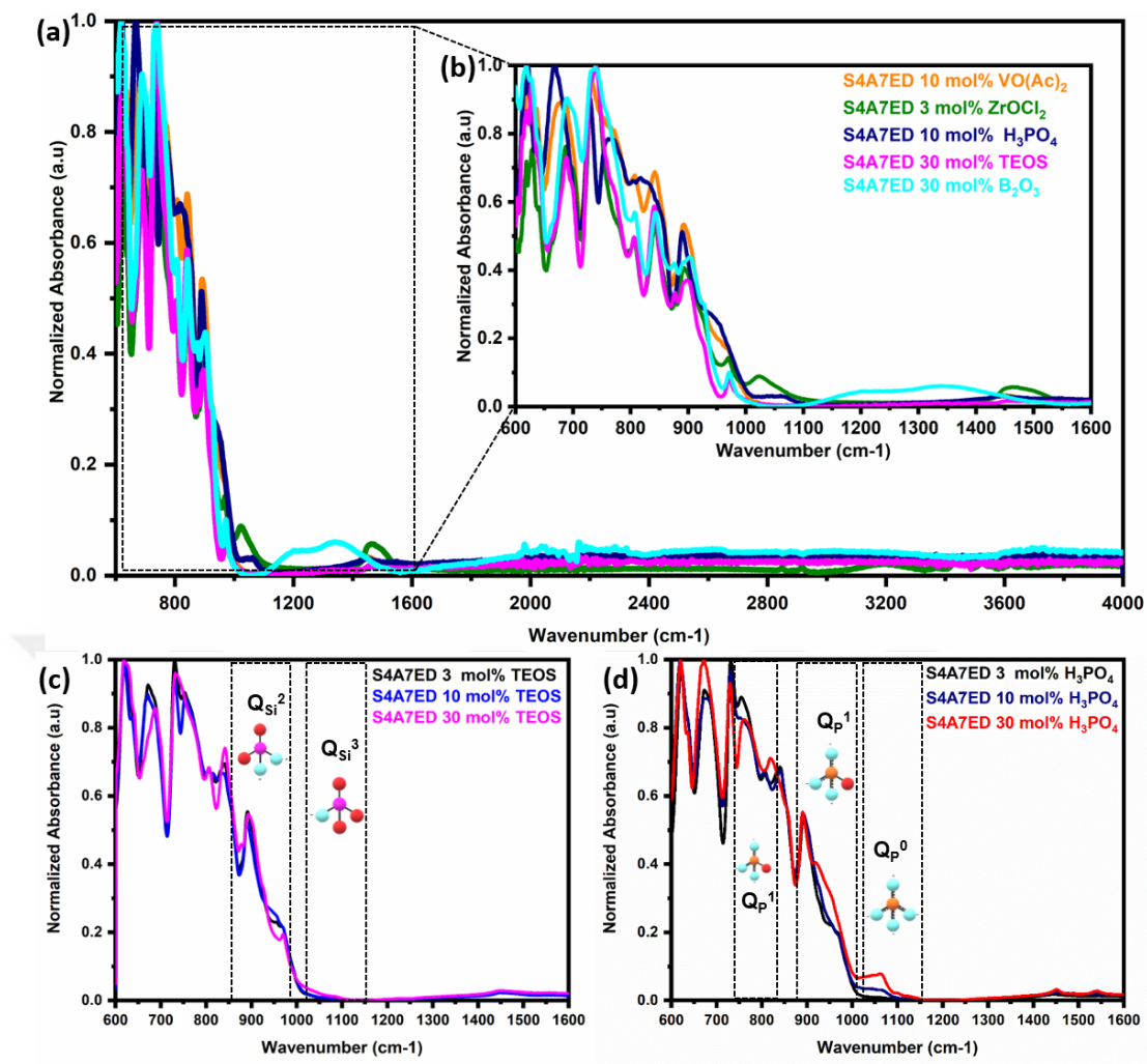
Figure 4.5 a) Full range FTIR spectra for S4A7EDmX compounds; b) 600-1600 \text{cm}^{-1} magnified; c) FTIR spectra for S4A7EDmX with 3, 10 and 30 mol% TEOS and d) FTIR spectra for S4A7EDmX with 3, 10 and 30 mol% \text{H}_3\text{PO}_4 .
