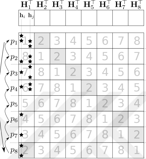
Figure 5.2: The numbers identify the sub-matrix blocks that constitute a stratum in a ring strata with seed=1 . Stratum \mathcal{S}_2 is highlighted. Side arrows show the processor update order of \mathbf{h}_i and \mathbf{h}_j .
