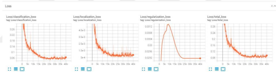
Figure 4.20. TF2 Result Graph
