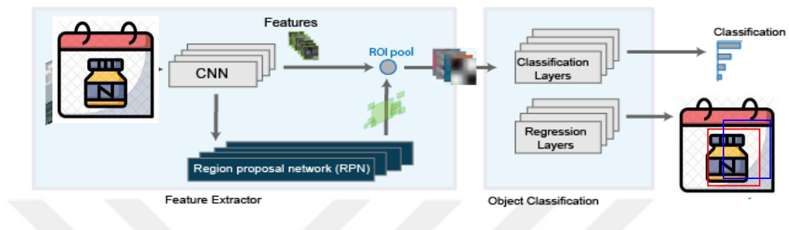
Figure 3.3. Faster R-CNN Architecture
