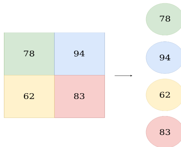
Figure 2.5. Flattening
