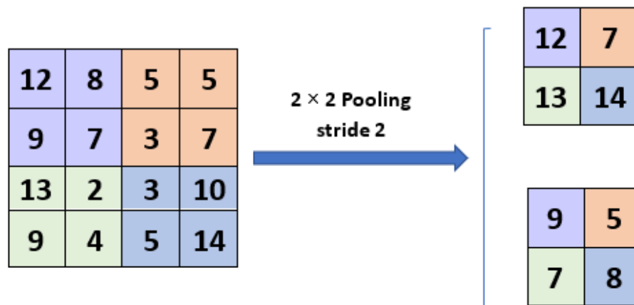
Figure 2.3. Pooling Layer
