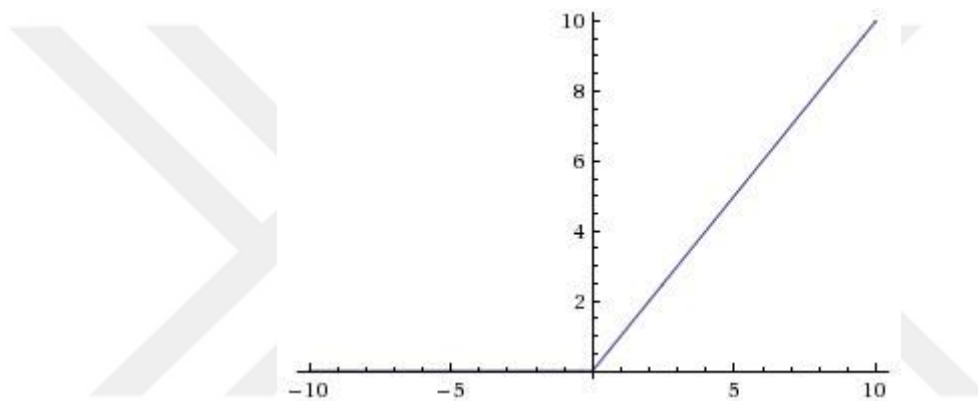
Figure 2.7. ReLU Function
