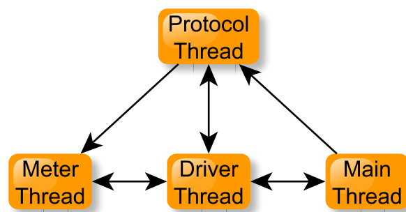
Figure 5.1: Thread Hierarchy
