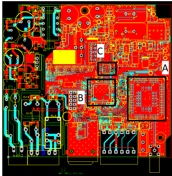
Figure 4.2: Final Gerber Design, A: GSM Module, B: Microcontroller, C: Flash Memory
