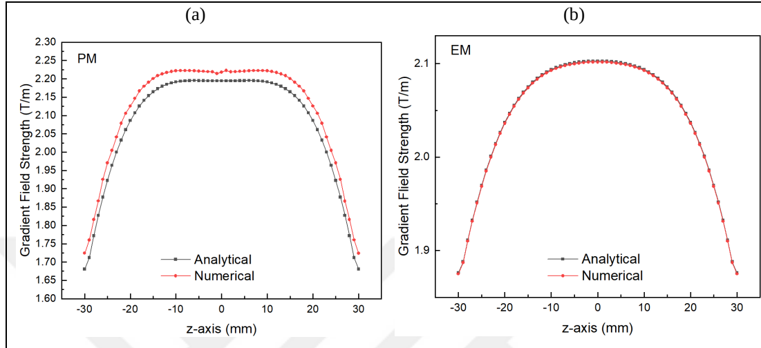
Figure 4.12: Gradient field strength along the z-axis. (a) The gradient of the selection field produced with the permanent magnets, (b) Gradient of the selection field produced with the electromagnets.
