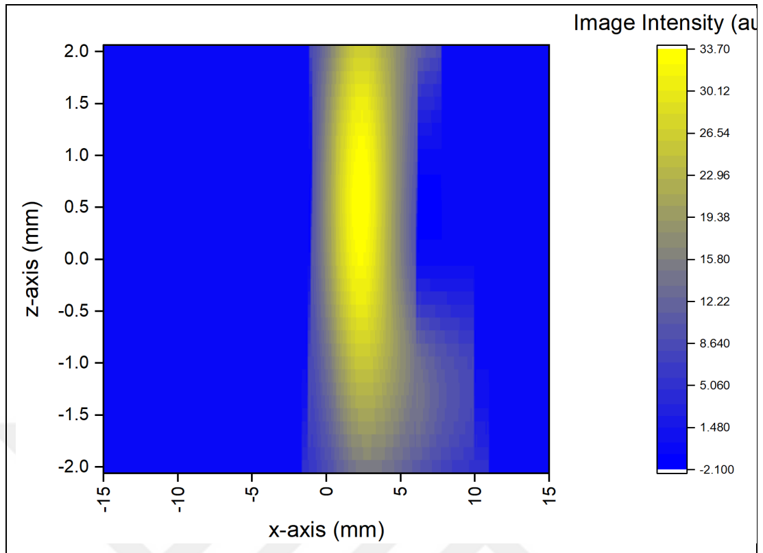
Figure 6.12: MPI image of the Perimag sample of 40 \mu l in a cylindrical phantom.
