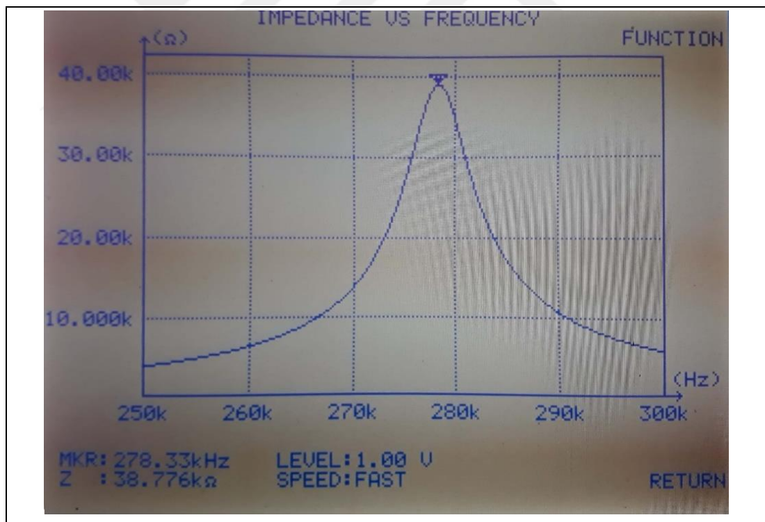
Figure 5.10: Self-resonance of the drive coil.
