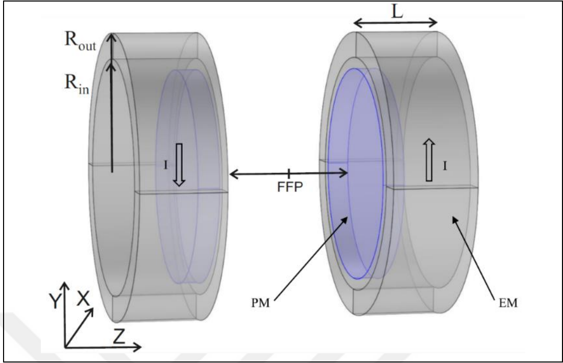
Figure 4.11: 3D transparent view of the combined topology of the disc type permanent magnet and ring-shaped electromagnetic coils. The current ( I ) direction of the electromagnets is represented with arrow directions. The permanent magnets (PM) are kept inside the electromagnets (EM) for effective usage.
