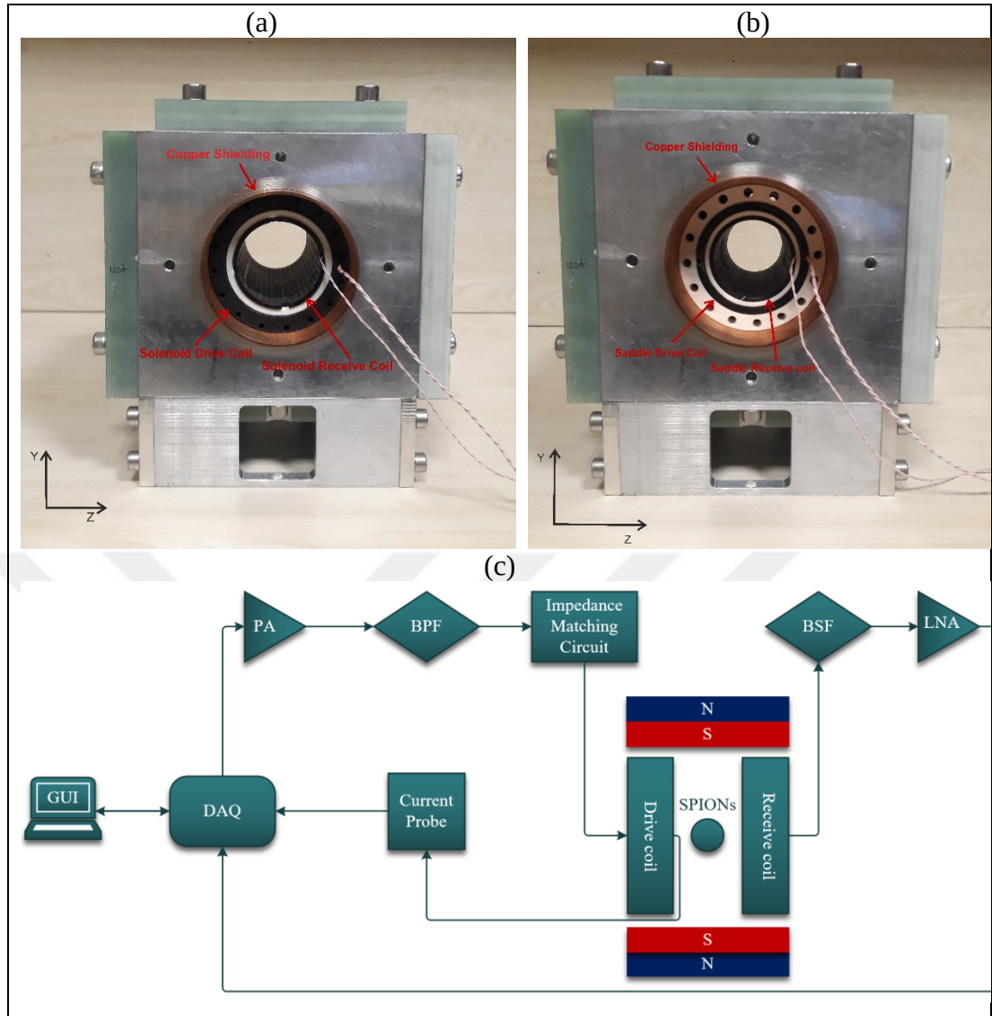
Figure 7.1: MPI scanner with 2D FOV; (a) MPI scanner with 2D FOV with solenoid drive and receive coils, (b) MPI scanner with 2D FOV with saddle-shaped drive and receive coils, (c) Generalized signal chain for two pairs of drive and receive coils (solenoid and saddle).
