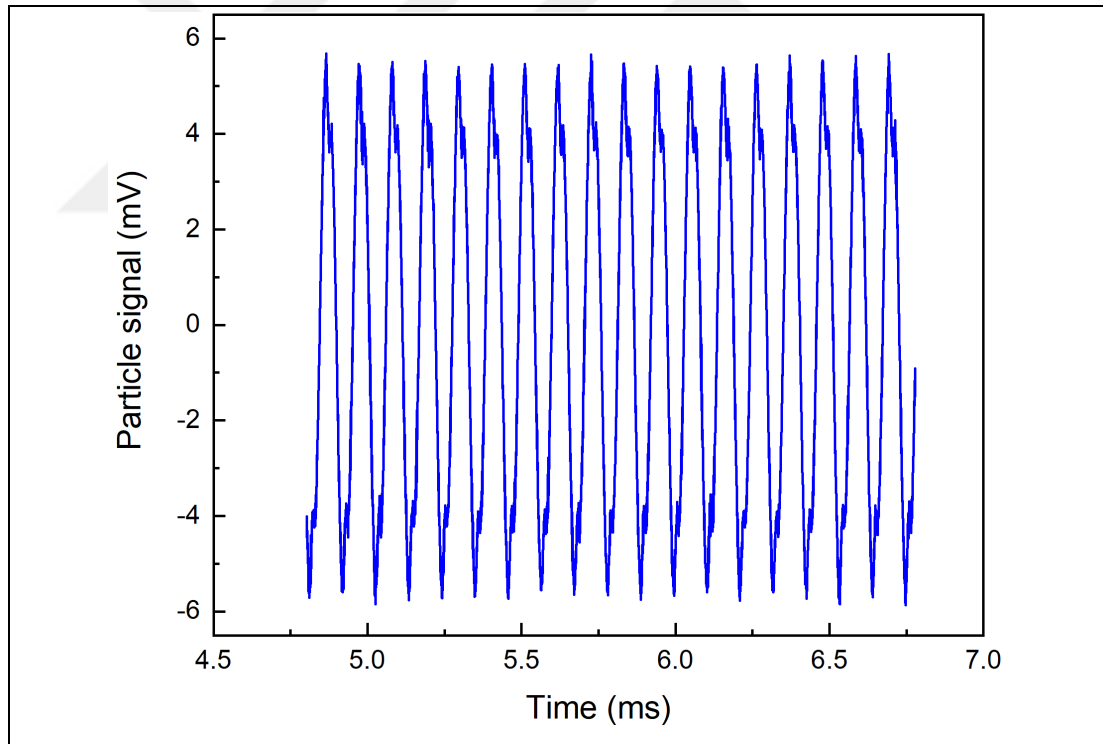
Figure 6.3: Particle signal of the 40 \mu\text{l} Perimag ® at the midpoint of the 4.3 T/m MPI scanner. An excitation field of 15 mT was applied to acquire the background signal before the sample scanning.
