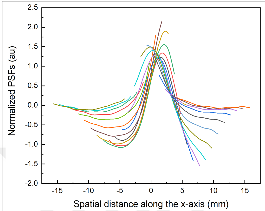
Figure 6.9: Overlapped view of the partial PSFs at z = 0 line.
