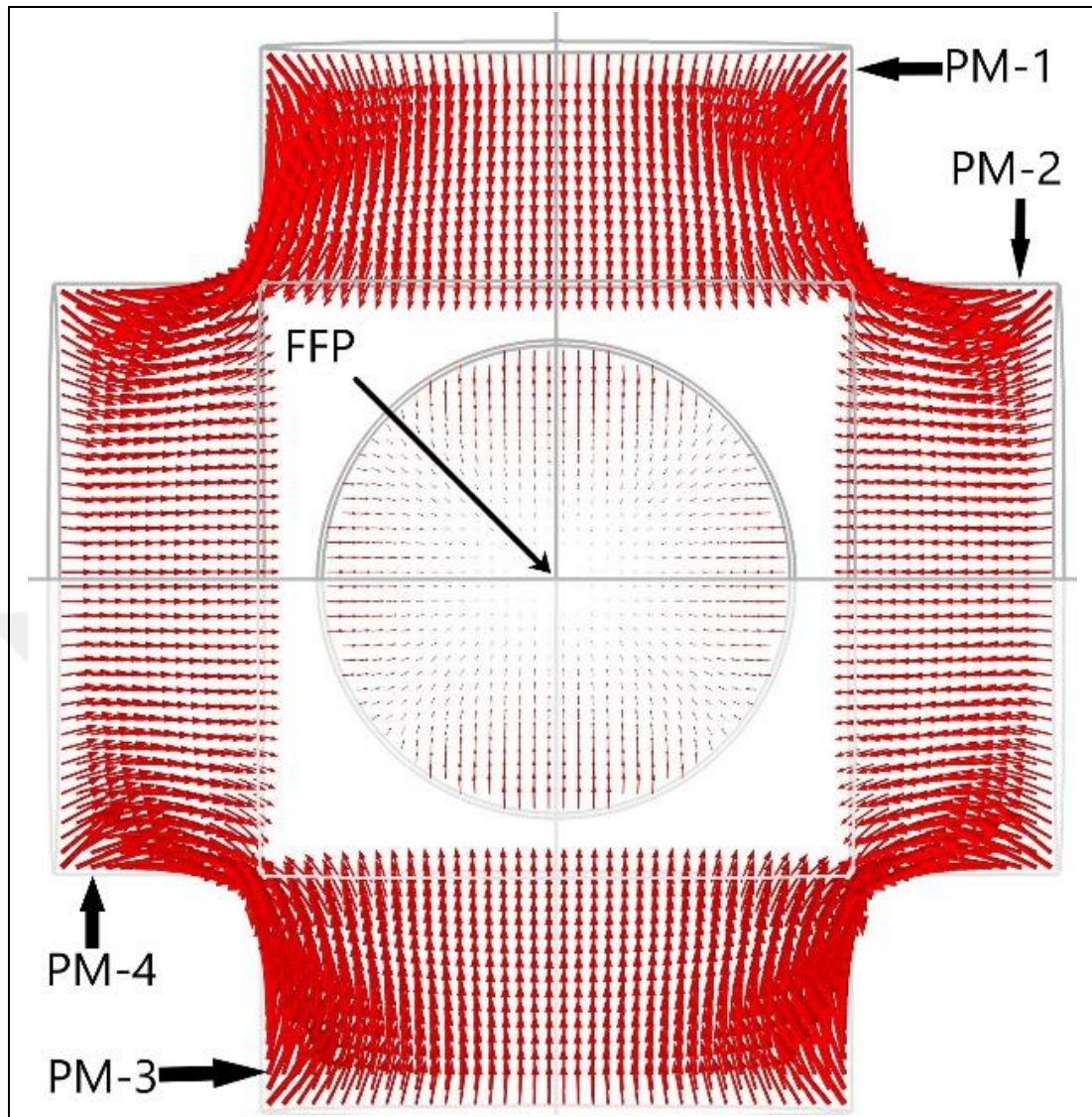
Figure 7.6: Magnetic flux density of the two pairs system in YZ plane; pole magnets of PM-1 and PM-3 are oppositely placed. Similarly, pole magnets of PM-2 and PM-4 are also oppositely placed. No magnetic field exists at the center of the system.
