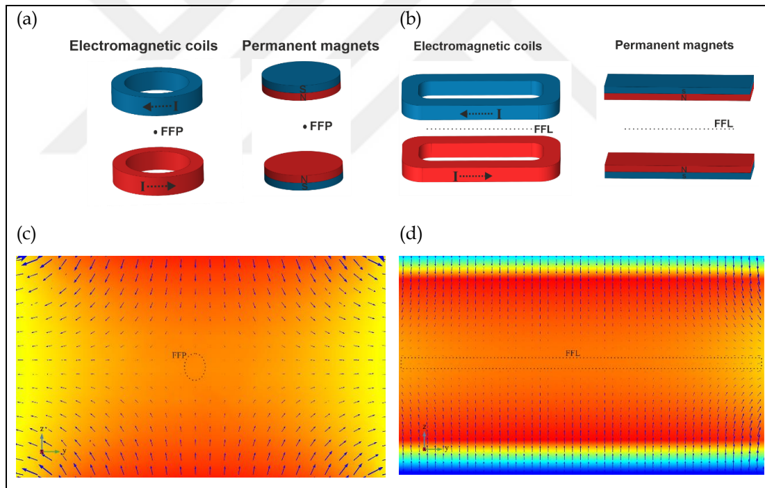
Figure 4.1: Selection fields for MPI scanners; (a) Disc-shaped permanent magnets and ring-shaped electromagnetic coils are commonly used to generate FFP, (b) Rectangular shaped permanent magnets and electromagnetic coils are usually used to achieve FFL, (c) Magnetic field strength pattern of FFP spatial encoding, (d) Magnetic field strength pattern of FFL spatial encoding.
