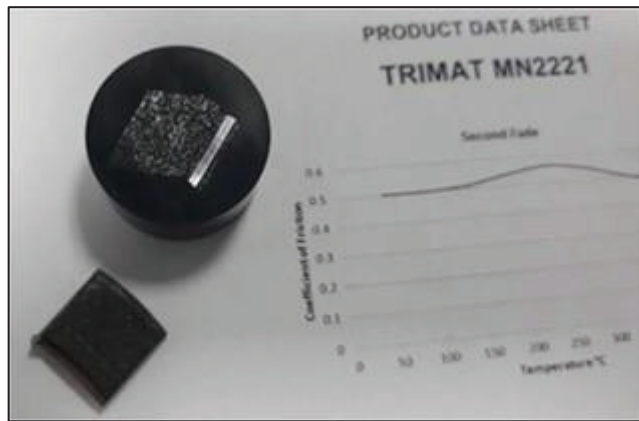
Figure 3.1. Prepared by Taking the Surface and Cross Section of Commercial Friction Facing
