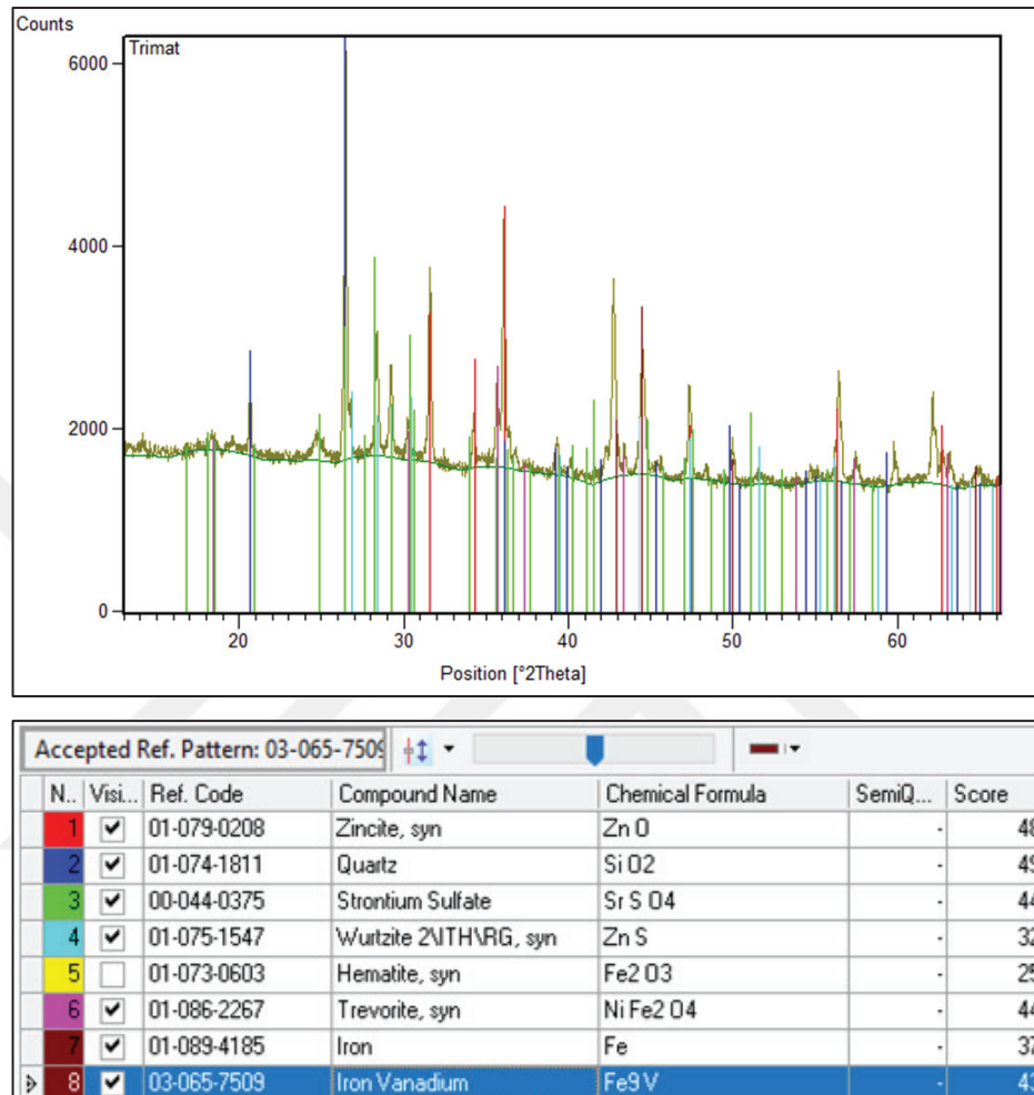
Figure 4.1. XRD Phase Analysis Result
