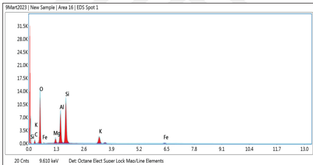
Figure 4.7. EDS Result of the Sample in the Spot1 Region
