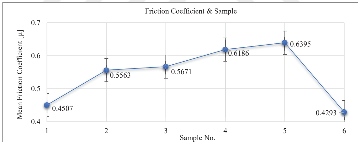
Figure 4.10. Mean Friction Coefficient- Sample
