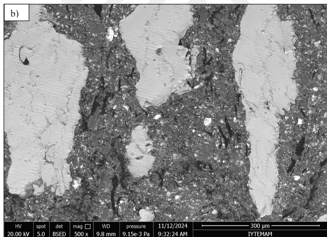
Figure 4.25. SEM Images of Sample6, a) From the Worn Surface, b) From the Sectioned Surface
