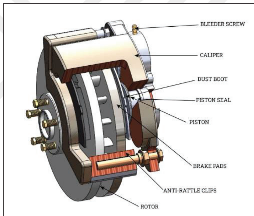
Figure 2.1. Disc Brake Used in Vehicles (Source: Zhang et al. 2022)
