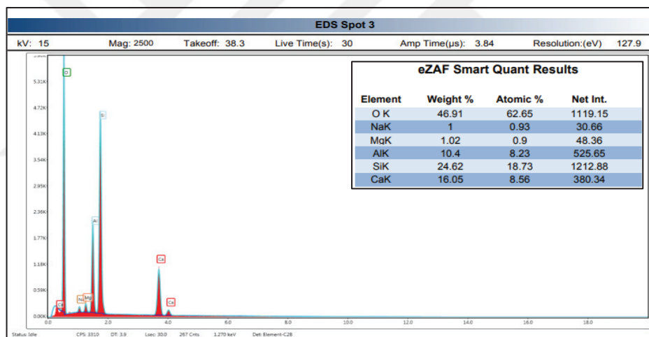
Figure 4.27. EDS Images of Sample2 Taken from Spot
