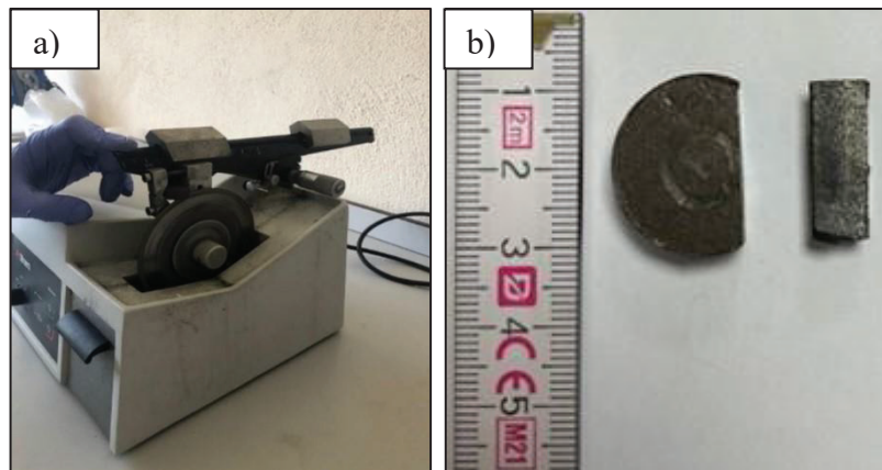
Figure 3.8. The Process of Sectioning with a) Wire Saw, b) Sectioned Sample
