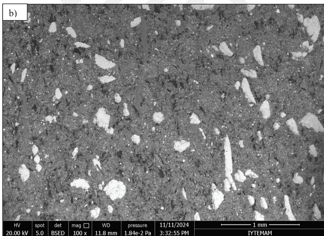
Figure 4.22. SEM Images of Sample3, a) From the Worn Surface, b) From the Sectioned Surface
