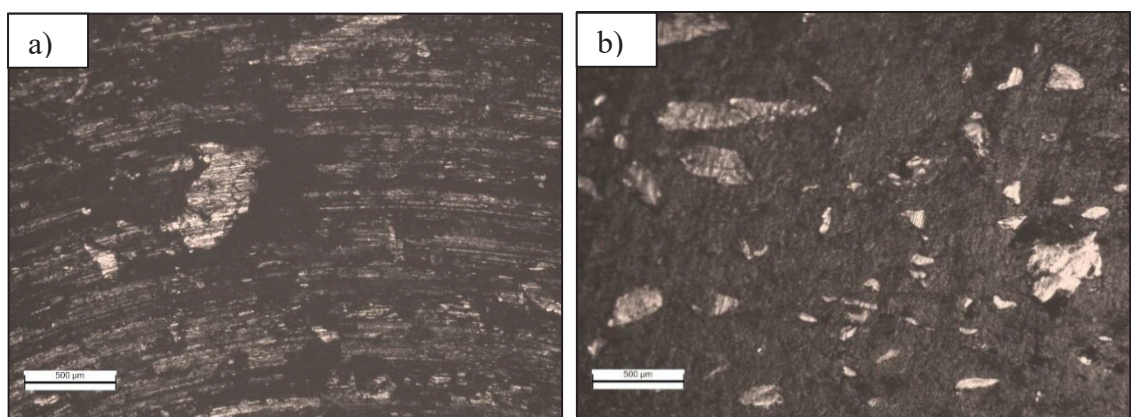
Figure 4.16. Optical Microscope Images of Sample3, a) From the Worn Surface, b) From the Sectioned Surface
