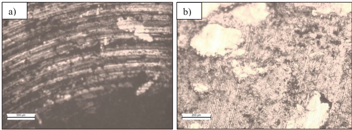
Figure 4.17. Optical Microscope Images of Sample4, a) From the Worn Surface, b) From the Sectioned Surface
