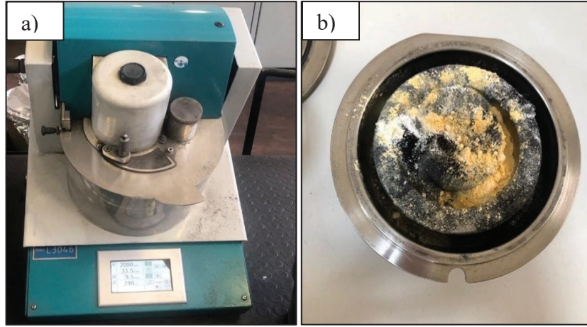
Figure 3.3. a) L3046 Mixer Device, b) Homogeneous Raw Material Mixture
