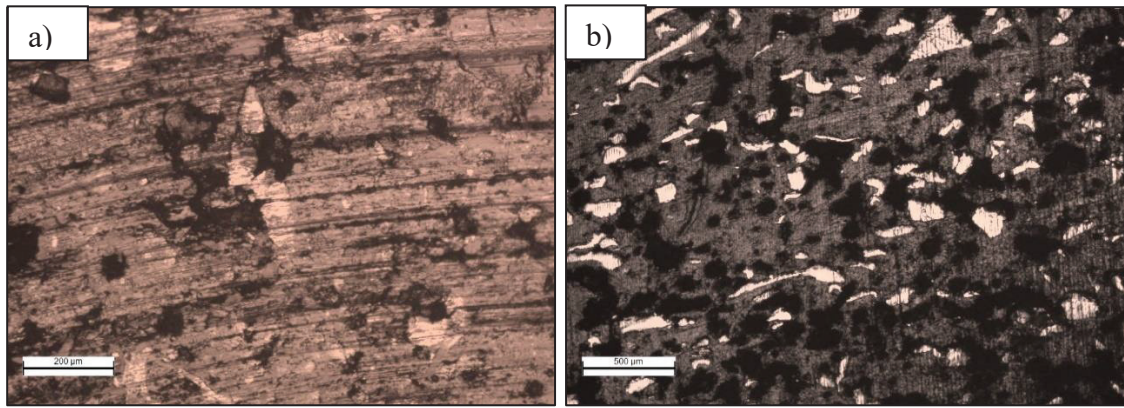
Figure 4.14. Optical Microscope Images of Sample1, a) From the Worn Surface, b) From the Sectioned Surface
