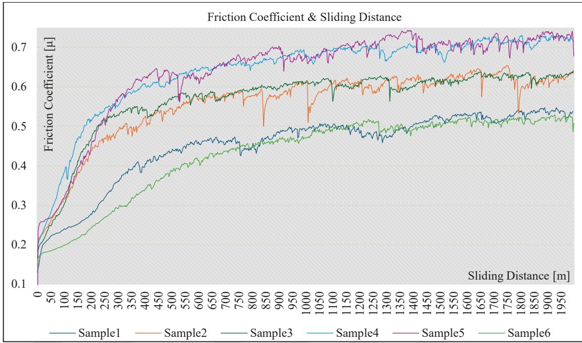
Figure 4.11. Comparative Friction Coefficient vs. Distance Result of Samples
