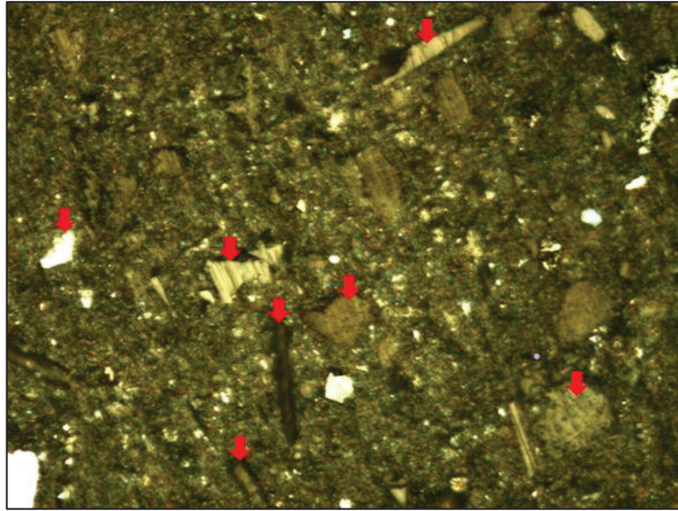
Figure 4.4. Sectional Image of the Sample Under an Optical Microscope Taken at 500X Magnification
