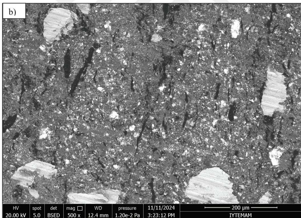
Figure 4.21. SEM Images of Sample2, a) From the Worn Surface, b) From the Sectioned Surface
