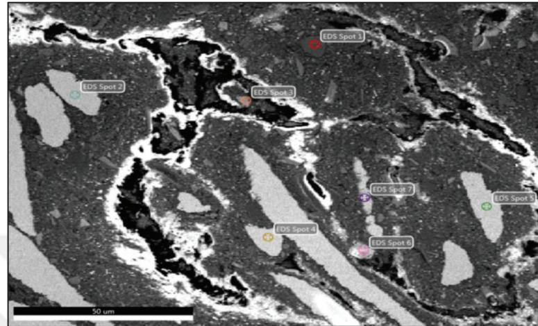
Figure 4.6. SEM Image of Sample Taken at 50 \mu\text{m} Magnification
