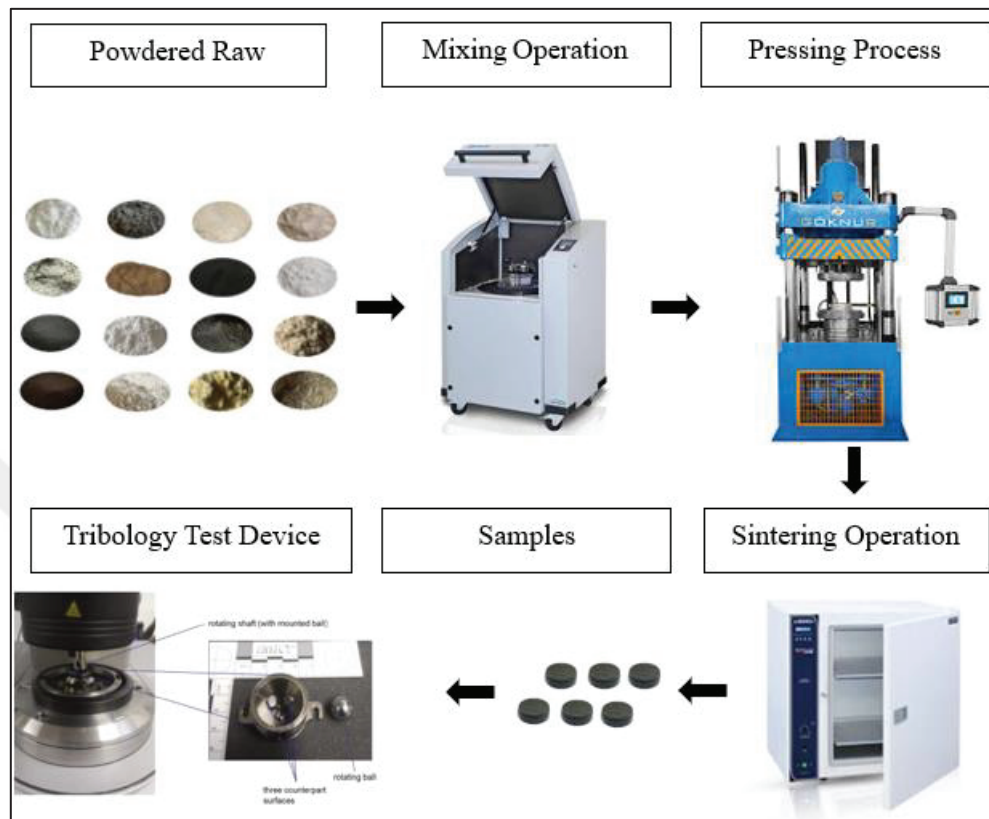
Figure 3.5. Production Flow Chart (Source: Di Gianfrancesco 2017)
