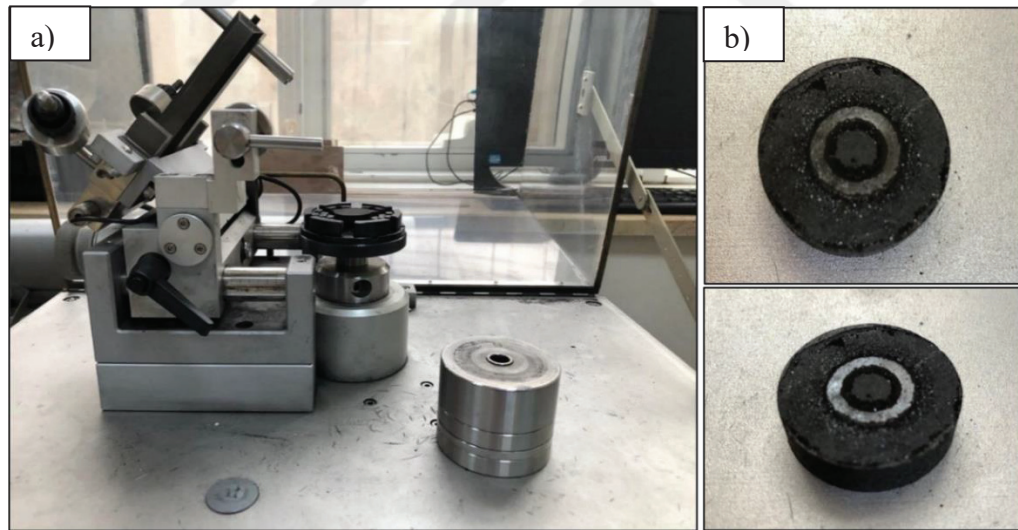
Figure 3.6. a) Tribology Test Device, b) Worn Test Specimen Used in the Experiments
