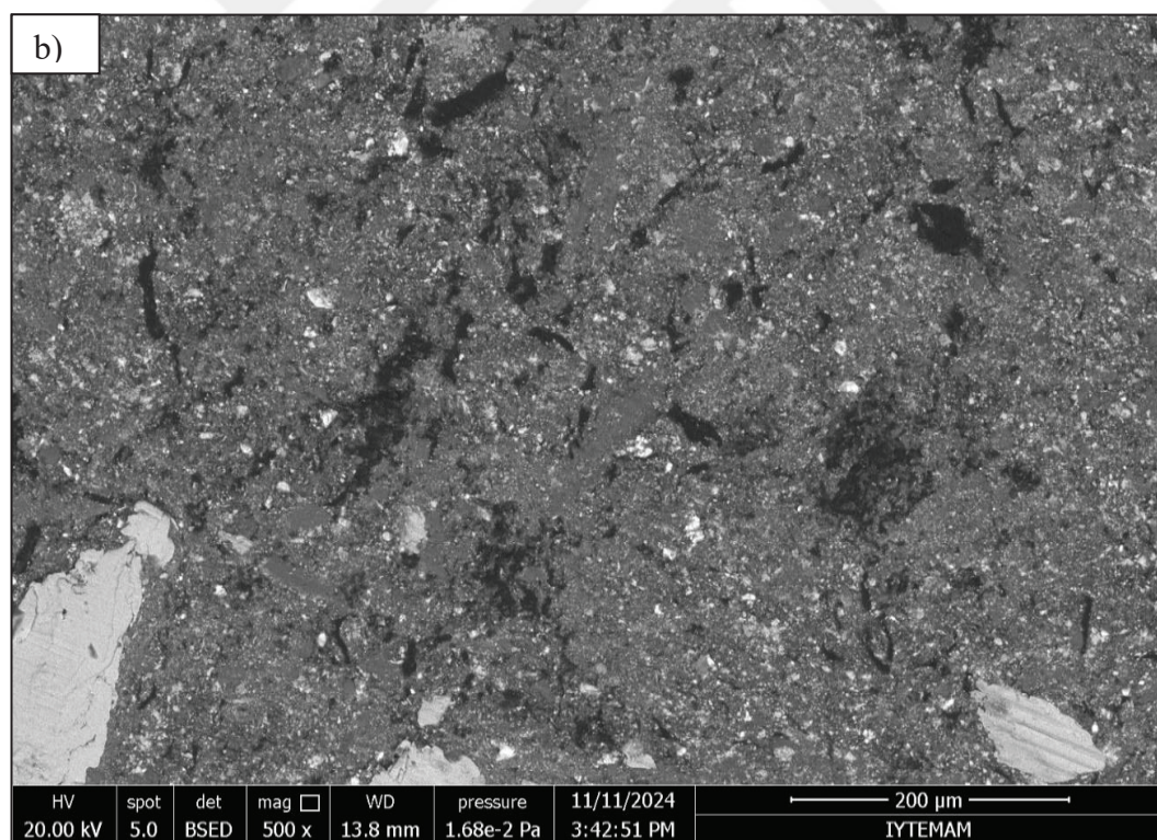
Figure 4.23. SEM Images of Sample4, a) From the Worn Surface, b) From the Sectioned Surface
