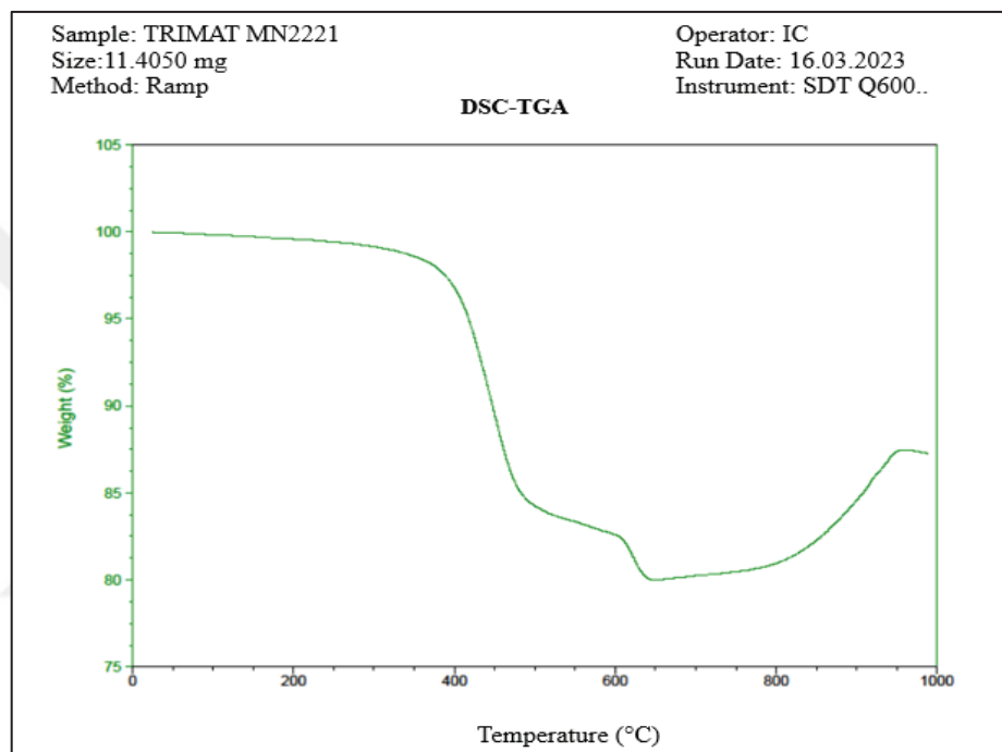
Figure 4.9. TG/DTA Analysis Results
