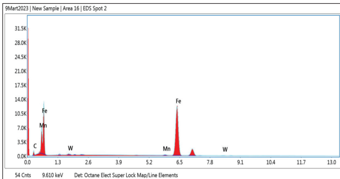
Figure 4.8. EDS Result of the Sample in the Spot2 Region
