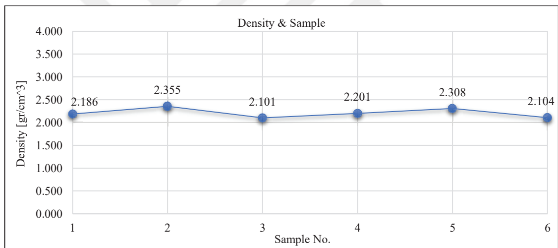
Figure 4.13. Density & Sample Graph
