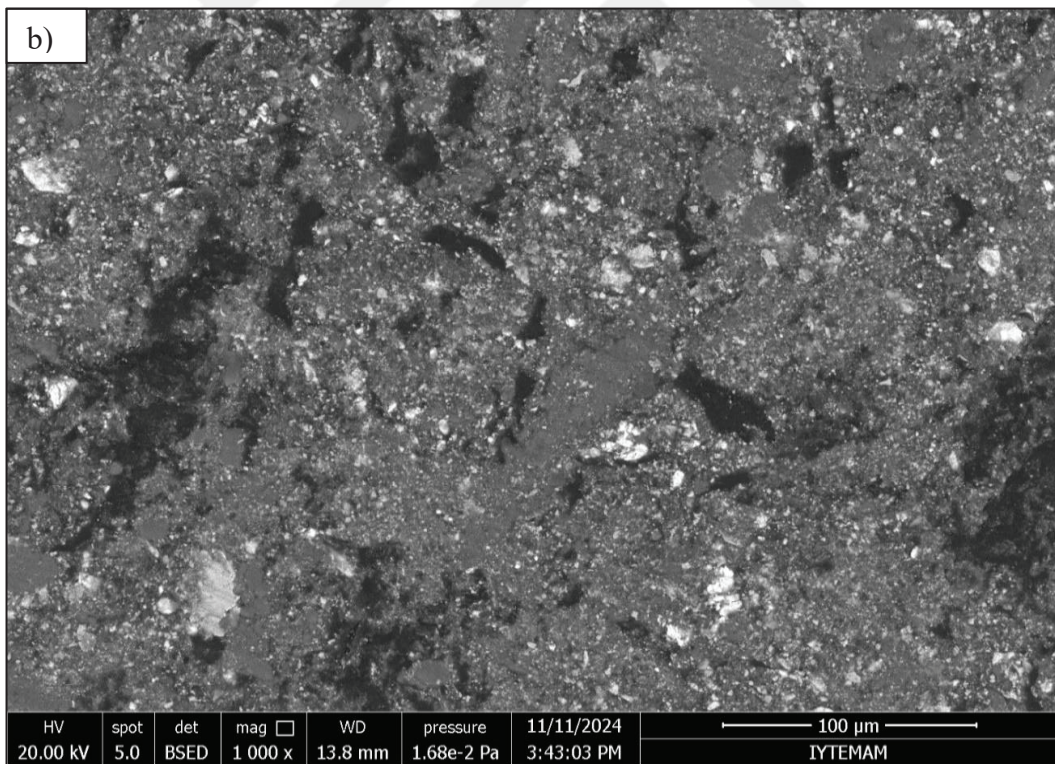
Figure 4.24. SEM Images of Sample5, a) From the Worn Surface, b) From the Sectioned Surface
