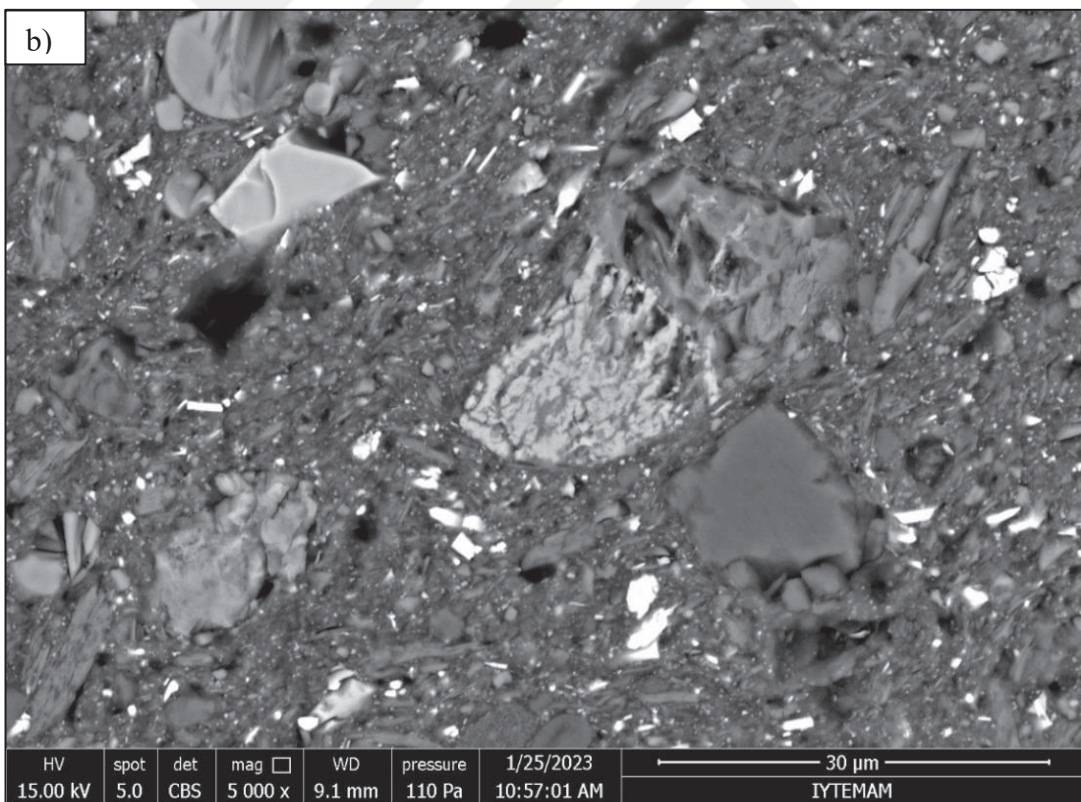
Figure 4.5. SEM Images Acquired from the Slice at Various Magnifications, a) at 500X Magnification, b) at 5000X Magnification
