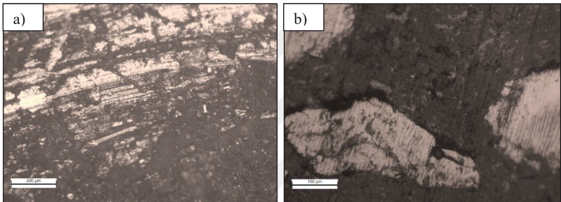
Figure 4.18. Optical Microscope Images of Sample5, a) From the Worn Surface, b) From the Sectioned Surface
