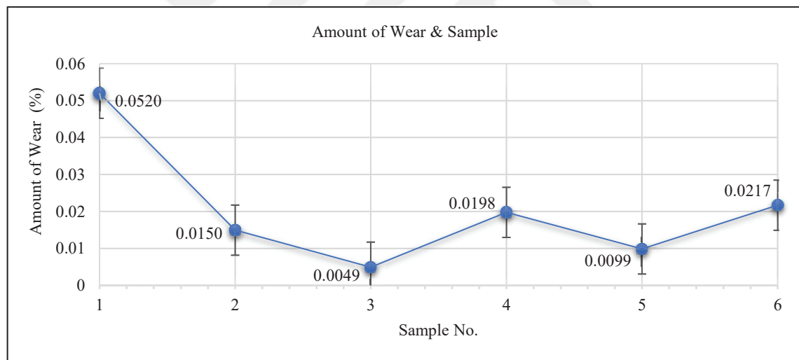
Figure 4.12. Amount of Wear -Sample Graph
