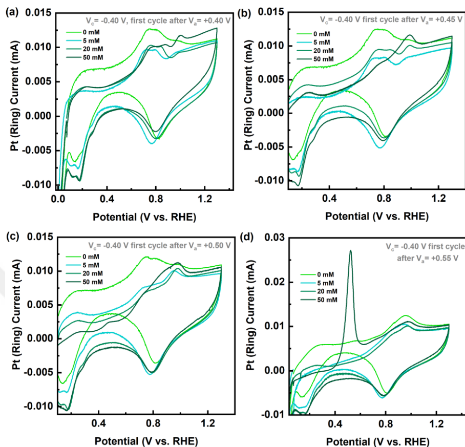
Figure D-5. CVs recorded at the Pt ring while the Cu disk is held at a cathodic potential of -0.40 V after (a) 0.40 V, (b) 0.45 V, (c) 0.50 V, and (d) 0.55 V anodic potential steps in \text{CO}_2 -purged 0.1 M \text{KHCO}_3 with x mM KCl (x = 0, 5, 20, and 50) electrolytes.
