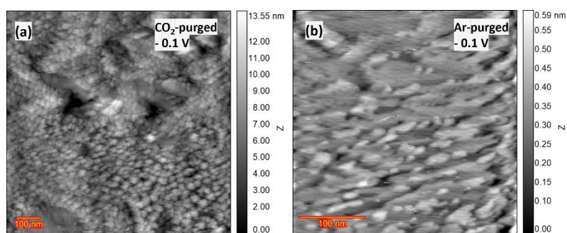
Figure D-9. In-situ EC-STM imaging of the Cu (111) surface at -0.1 V after application of cathodic potentials of (a) -0.8 V in CO 2 -purged 0.1 M KHCO 3 electrolyte and (b) -0.4 V in Ar-purged 0.1 M KHCO 3 electrolyte.
