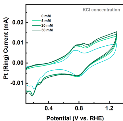
Figure D-6. Effect of KCl concentration on the Pt ring, in \text{CO}_2 -purged 0.1 M \text{KHCO}_3 with x mM KCl (x = 0, 5, 20, and 50) electrolytes, in the absence of the Cu disk.
