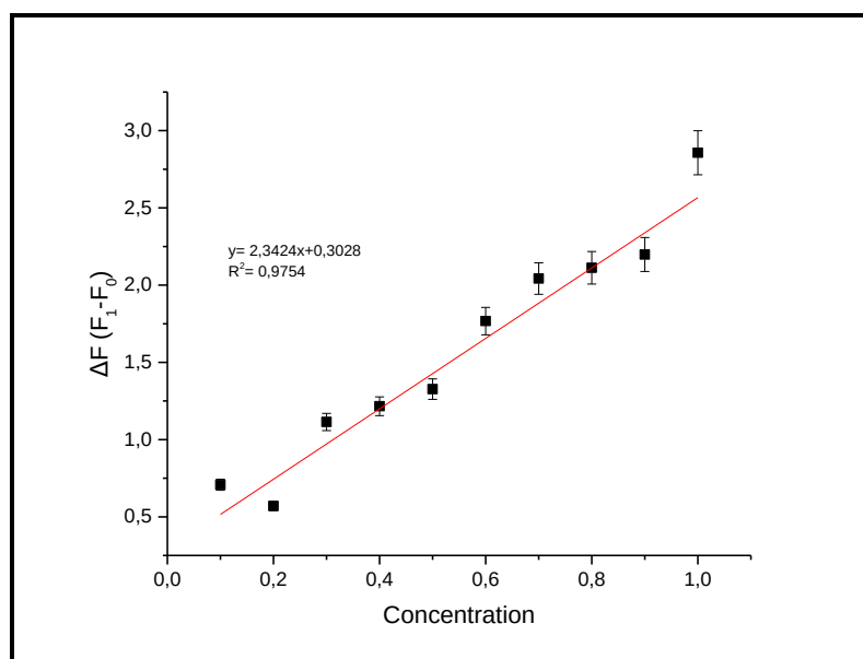
Figure 4.33. Fluorescence changes of 1c (5 \mu M) upon addition of CORM-2 (0.1 to 1 \mu M) in 0.01 M PBS (pH 7.4), ( \lambda_{\text{ex}} : 460 nm).
