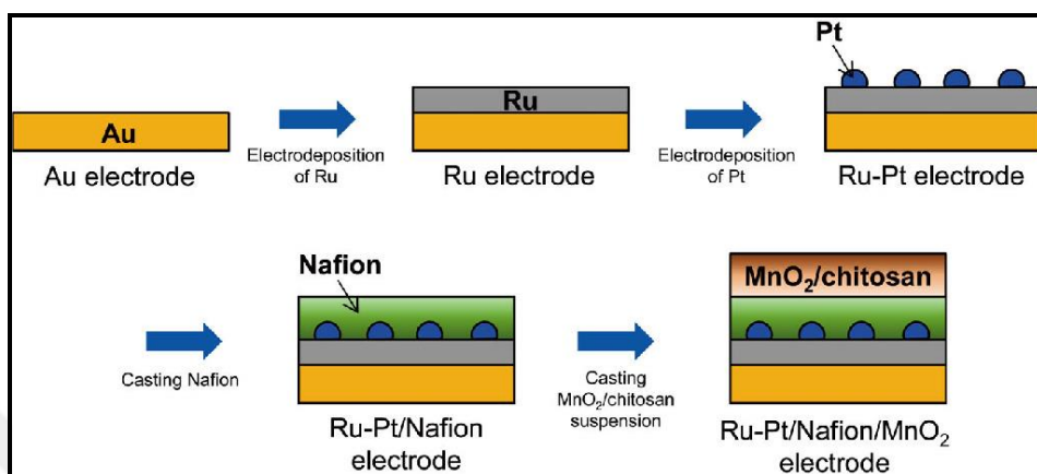
Figure 2.6. Preparation of Pt-Ru/Nafion/ \text{MnO}_2 electrode (Source: Seto et al., 2012).
