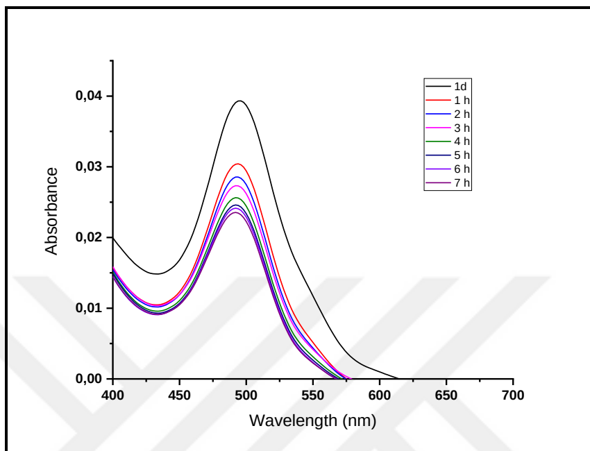
Figure 4.51. Absorbance change of 1d over time under green led.
