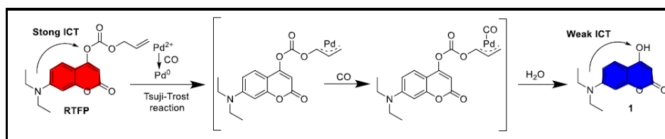
Figure 2.31. Sensing mechanism of the probe (Source: Tang et al., 2023).
