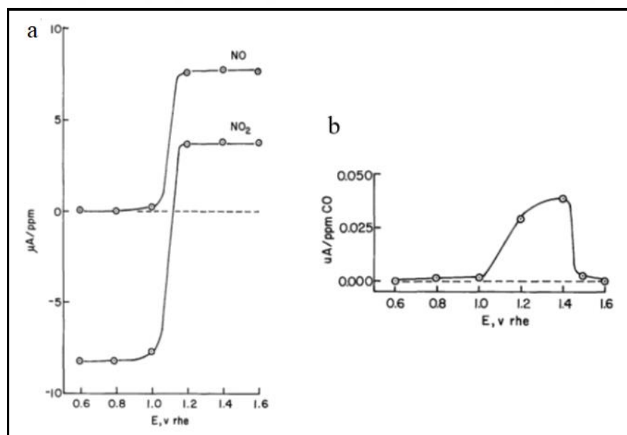
Figure 2.2. a) NO oxidation and NO 2 oxidation-reduction currents; b) CO oxidation currents (Source: Sedlak and Blurton, 1976).
