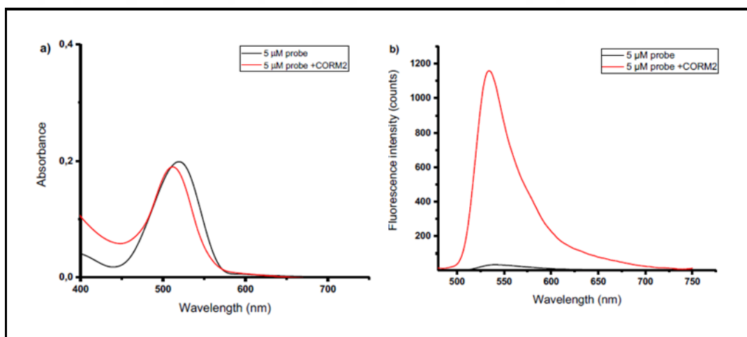
Figure 4.5. a) Absorbance and b) fluorescence spectra of 1a (5 \mu M) in the absence and presence of CORM-2 (250 \mu M) in 0.01 M PBS/CH 3 CN (pH 7.4, v/v,8:2), ( \lambda_{\text{ex}} : 460 nm).
