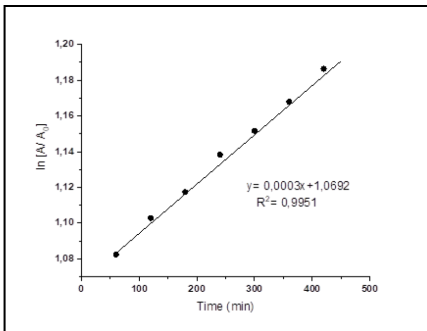
Figure 4.52. \ln (A_t/A_0) /time graphic of 1d .
