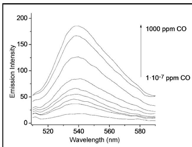
Figure 2.20. Fluorescence intensities of complex 7 vs. increasing CO concentrations (Source: Toscani et al., 2015).
