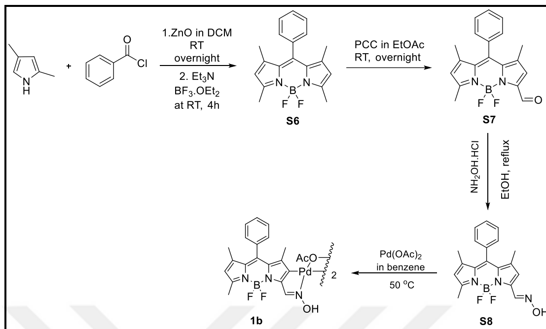
Figure 3.3. Synthesis of 1b .
