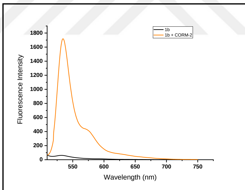
Figure 4.14. Fluorescence spectra of 1b (5 \mu M) in the absence and presence of 40 eq. CORM-2 in 0.01 M PBS/EtOH (pH 7.4, v/v, 1:1), ( \lambda_{\text{ex}} : 500 nm).
