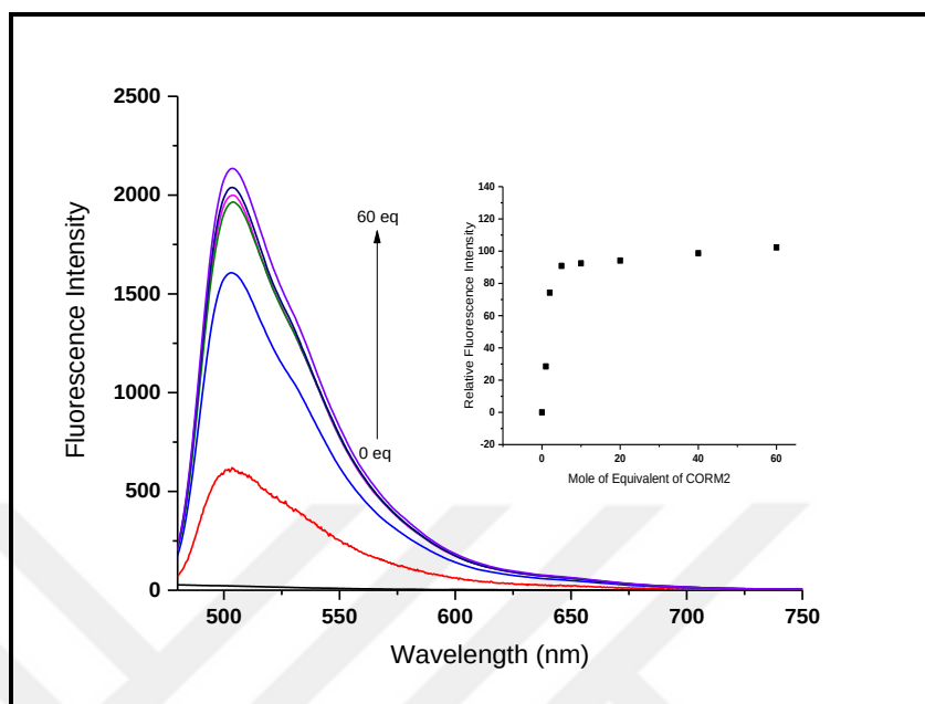
Figure 4.29. Emission spectra of 1c (5 μM) with increasing amount CORM-2 in 0.01 M PBS (pH 7.4), ( \lambda_{\text{ex}} : 460 nm).
