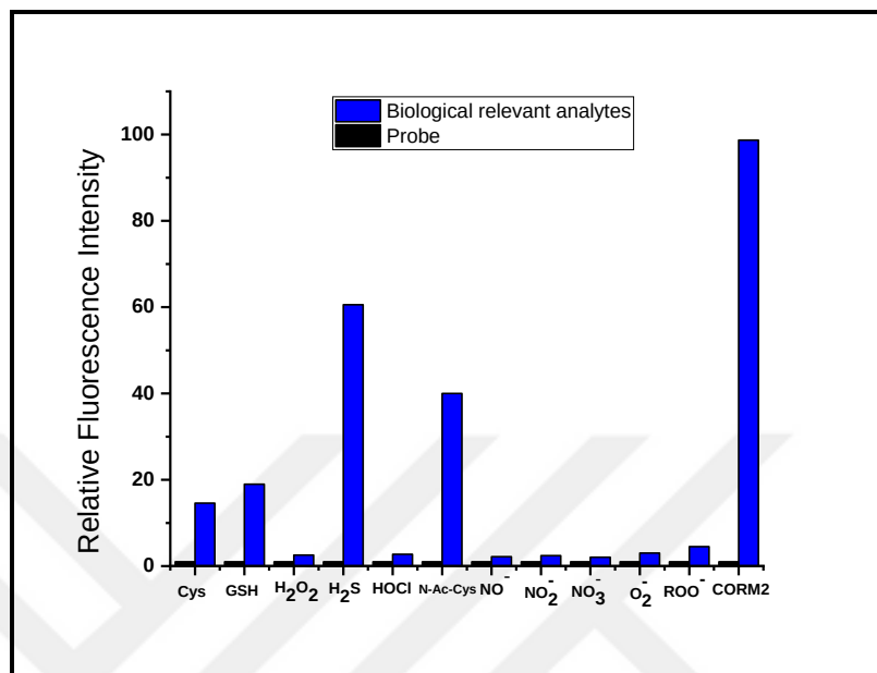
Figure 4.32. Fluorescence responses of 1c (5 \mu M) in the presence of biologically relevant analytes, reactive oxygen species, and CORM-2 (5 eq.) in 0.01 M PBS (pH 7.4), ( \lambda_{\text{ex}} : 460 nm).
