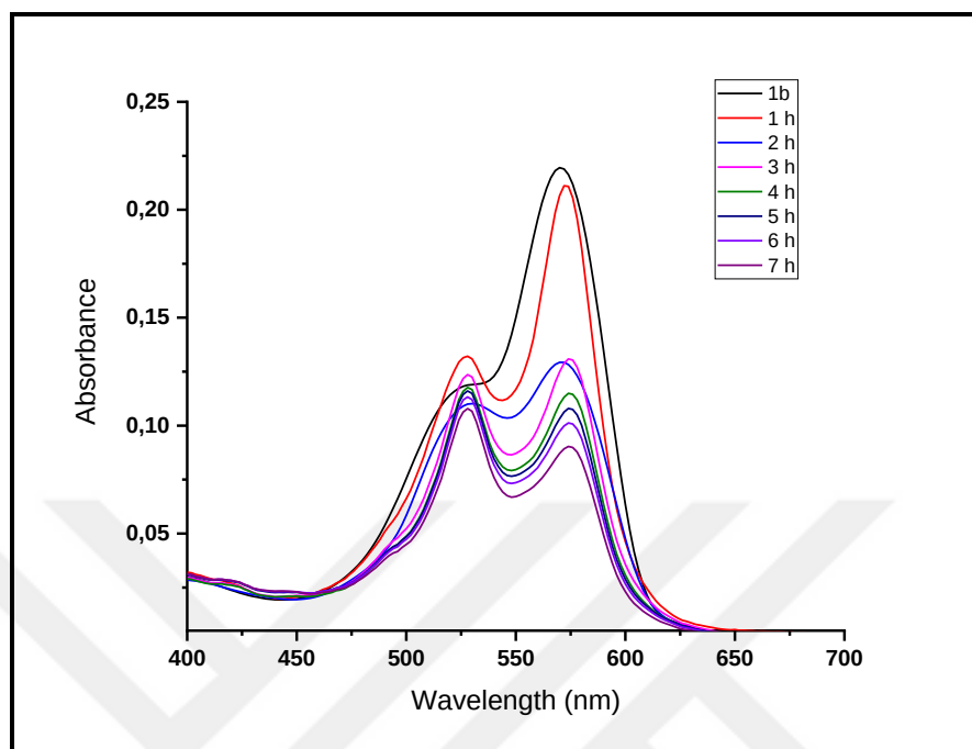
Figure 4.19. Absorbance change of 1b over time under green led.
