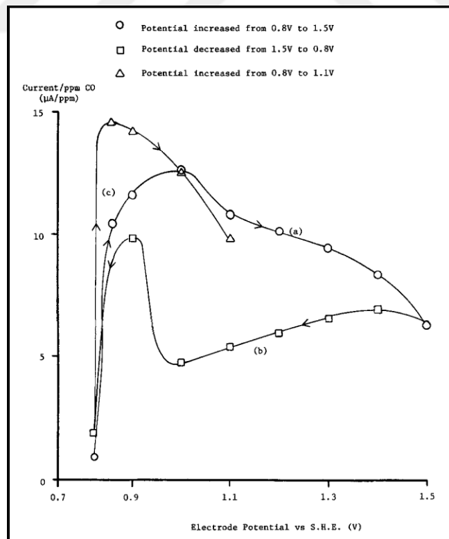
Figure 2.1. The CO oxidation current vs. the potential of the Pt electrode (Source: Blurton and Sedlak, 1974).
