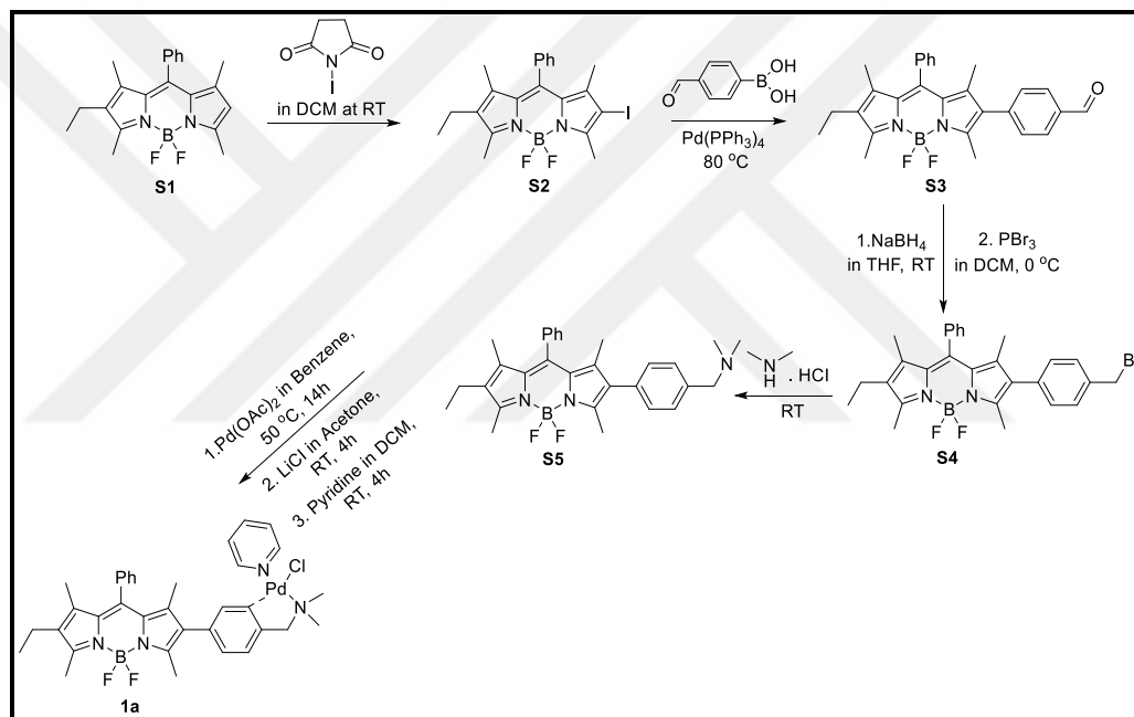
Figure 3.2. Synthesis of 1a .
