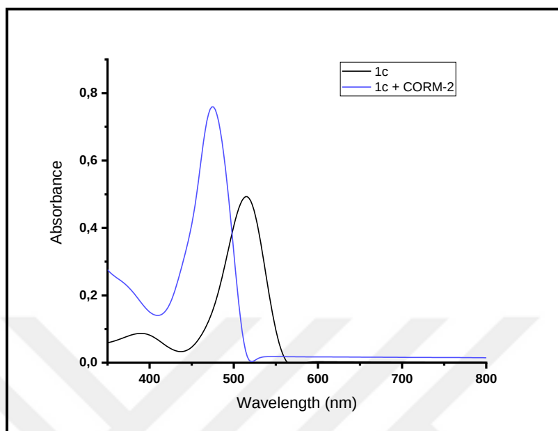
Figure 4.26. Absorbance spectra of 1c (5 μM) in the absence and presence of CORM-2 (5 eq.) in 0.01 M PBS (pH 7.4).
