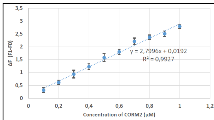
Figure 4.11. Fluorescence changes of 1a with the addition of CORM-2 at increasing concentrations in 0.01 M PBS/CH 3 CN (pH 7.4, v/v, 8:2), ( \lambda_{\text{ex}} : 460 nm).
