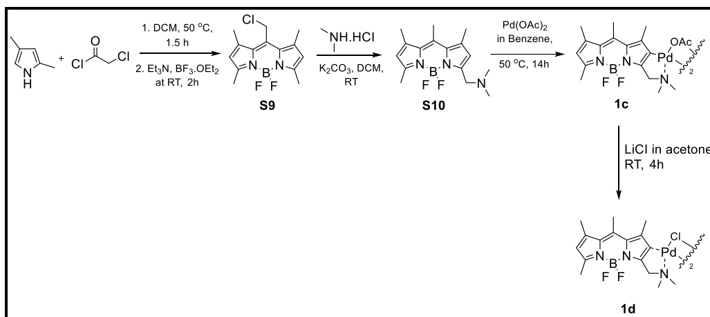
Figure 3.4. Synthesis of 1c and 1d
