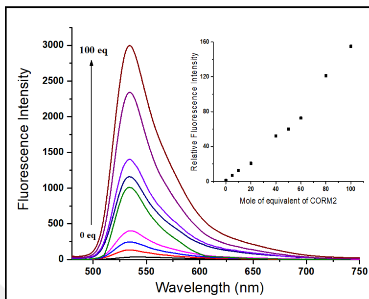
Figure 4.6. Fluorescence spectra of 1a (5 \mu\text{M} ) in the presence of increasing amount of CORM-2 (0-500 \mu\text{M} ) in 0.01 M PBS/CH 3 CN (pH 7.4, v/v,8:2), ( \lambda_{\text{ex}} : 460 nm). Inset: Calibration curve.
