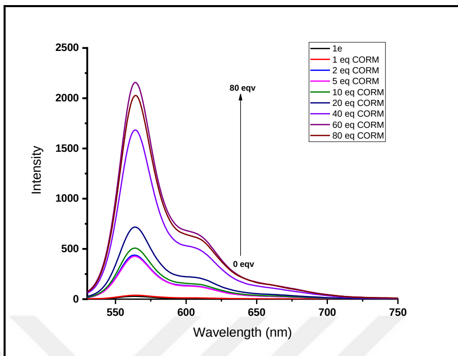
Figure 4.57. Fluorescence intensity of 1e (5 \mu M) in the presence of increasing amount of CORM-2 in 0.01 M PBS/DMF (pH 7.4, v/v,8:2), ( \lambda_{\text{ex}} : 520 nm).
