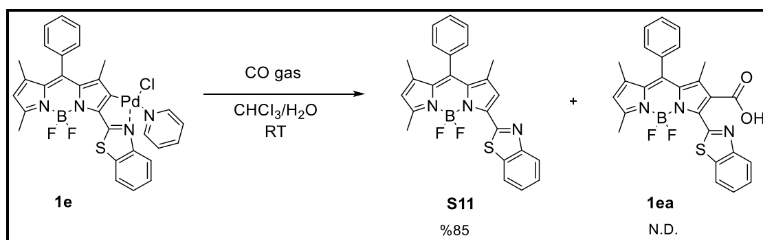
Figure 4.4. Reaction with carbon monoxide gas of the probe 1e .
