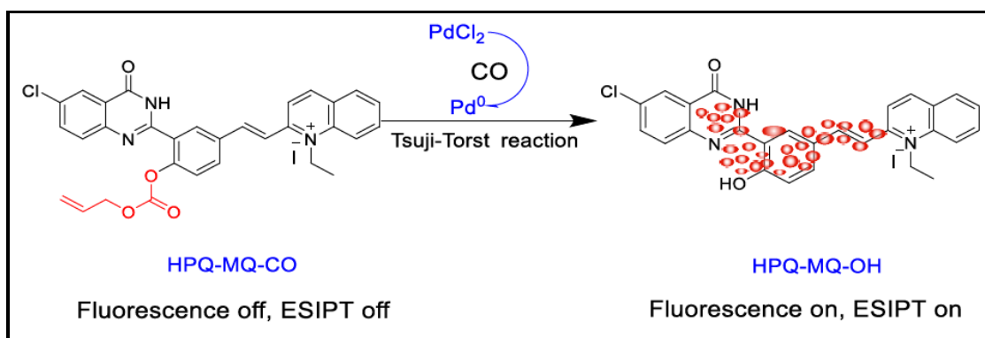
Figure 2.30. Schematic illustration of the probe with CO (Source: Fu et al., 2022).
