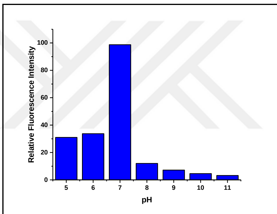
Figure 4.28. Effect of pH on the 1c (5 \mu M) in the presence of CORM-2 (5 eq.) in 0.01 M PBS (pH 7.4), ( \lambda_{\text{ex}} : 460 nm).
