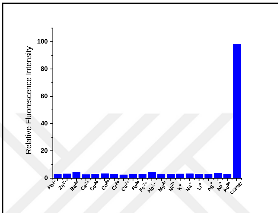
Figure 4.31. Fluorescence intensity of 1c (5 \mu M) in the presence of CORM-2 and other metal ions (5 eq.) in 0.01 M PBS (pH 7.4), ( \lambda_{\text{ex}} : 460 nm).
