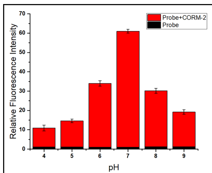
Figure 4.9. Performance of 1a (5 \mu M) with CORM-2 (50 eq) at various pH levels in 0.01 M PBS/CH 3 CN (pH 7.4, v/v, 8:2), ( \lambda_{\text{ex}} : 460 nm).
