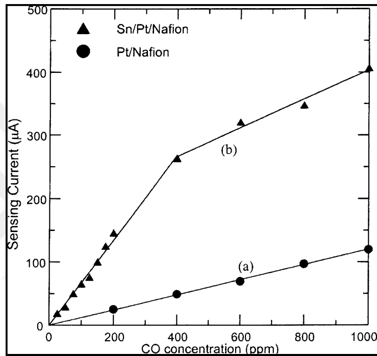
Figure 2.3. CO concentration vs. Current. a) Pt/Nafion at 0.8 V vs. Ag/AgCl; b) Sn/Pt/Nafion at 0.5 V vs. Ag/AgCl (Source: Tsceng and Yang, 2003).
