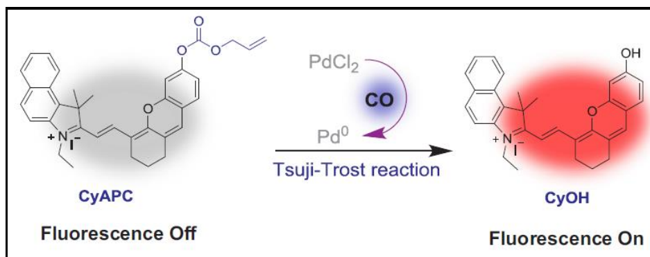
Figure 2.26. Response mechanism of the probe (Source: Li et al., 2018).
