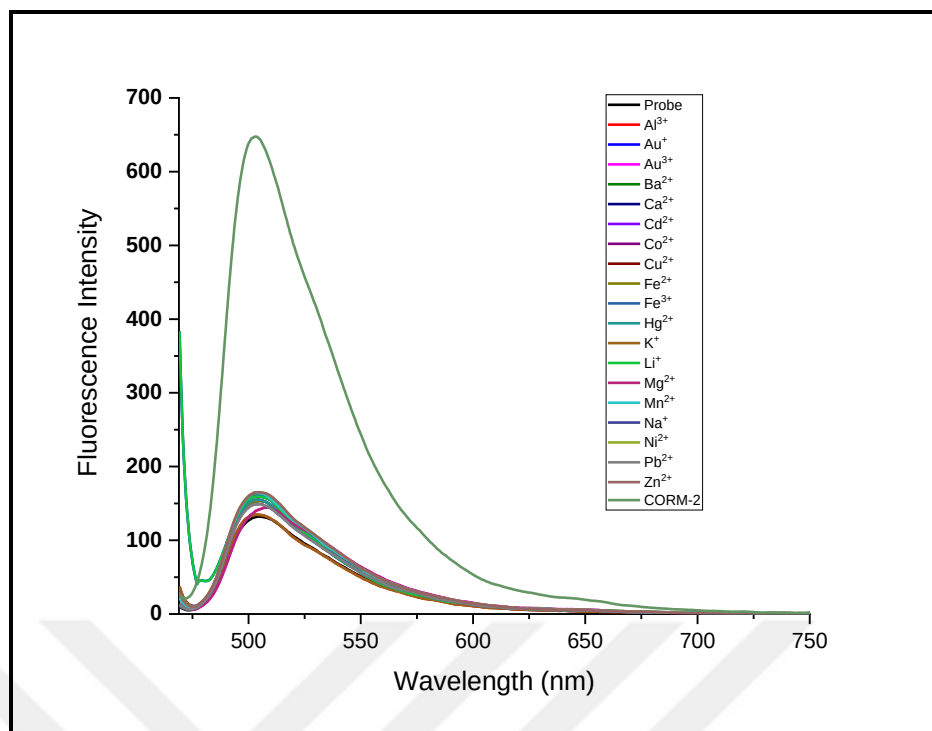
Figure 4.45. Fluorescence intensity of 1d (5 \mu M) in the presence of CORM-2 and other metal ions (2 eq.) in 0.01 M PBS/EtOH (pH 7.4, v/v,9:1), ( \lambda_{\text{ex}} : 460 nm).
