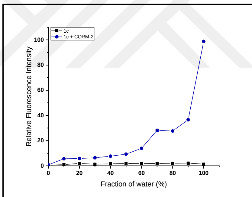
Figure 4.25. Fluorescence performance of 1c (5 \mu M) at increasing water ratios with CORM-2 (5 eq.) in 0.01 M PBS/DMF (pH 7.4), ( \lambda_{\text{ex}} : 460 nm).
