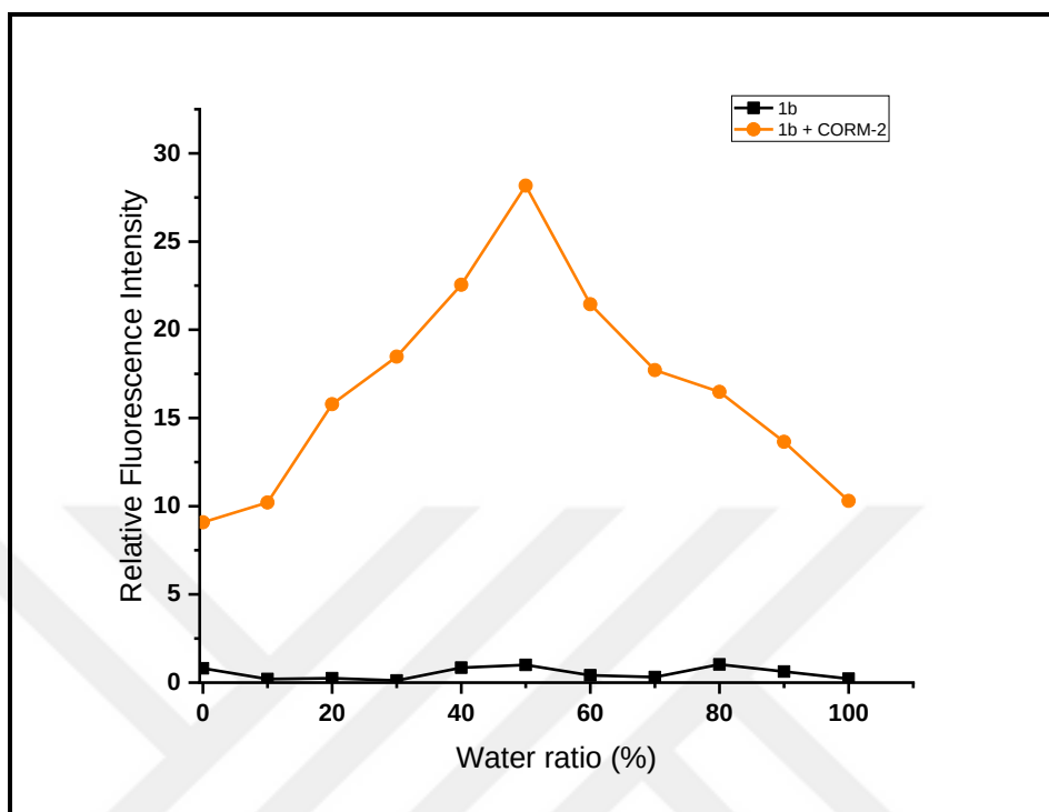
Figure 4.15. Fluorescence performance of 1b (5 \mu M) at increasing water ratios with CORM-2 (40 eq.) in 0.01 M PBS/EtOH (pH 7.4 v/v, 1:1), ( \lambda_{\text{ex}} : 500 nm).
