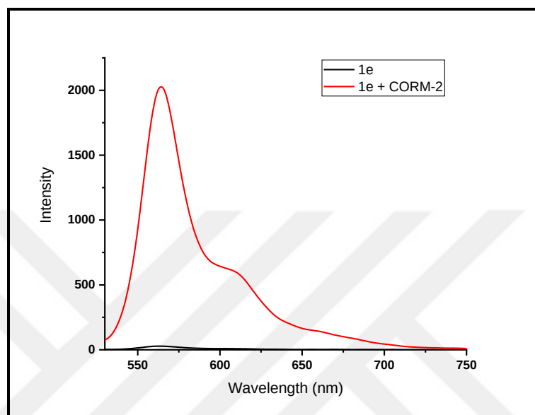
Figure 4.55. Fluorescence spectra of 1e (5 \mu M) in the absence and presence of 50 eq. CORM-2 in 0.01 M PBS/DMF (pH 7.4, v/v, 8:2), ( \lambda_{\text{ex}} : 520 nm).
