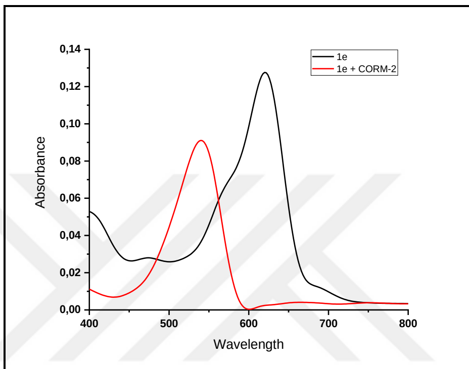
Figure 4.54. Absorbance spectra of 1e (5 \mu M) in the absence and presence of 50 eq. CORM-2 in 0.01M PBS/DMF (pH 7.4, v/v, 8:2).
