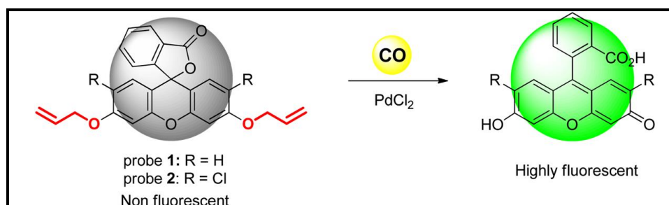
Figure 2.25. Probe 1 and probe 2 sensing mechanisms (Source: Feng et al., 2017).
