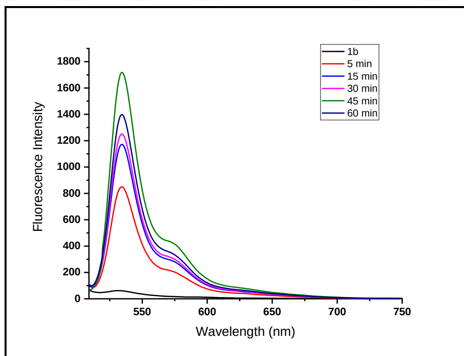
Figure 4.17. Reaction time profiles of 1b (5 \mu\text{M} ) in the presence of CORM-2 (40 eq.) in 0.01 M PBS/EtOH (pH 7.4, v/v,1:1), ( \lambda_{\text{ex}} : 500 nm).
