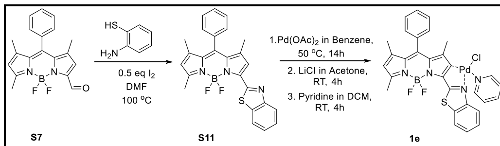
Figure 3.5. Synthesis of 1e
