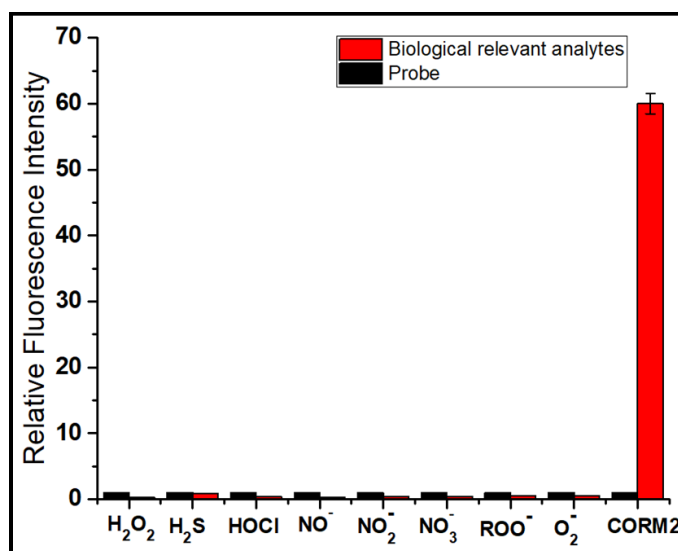
Figure 4.8. Fluorescence intensities of 1a (5 \mu\text{M} ) towards other biologically relevant analytes and reactive oxygen species (50 eq) along with CORM-2 in 0.01 M PBS/CH 3 CN (pH 7.4, v/v, 8:2) ( \lambda_{\text{ex}} : 460 nm).
