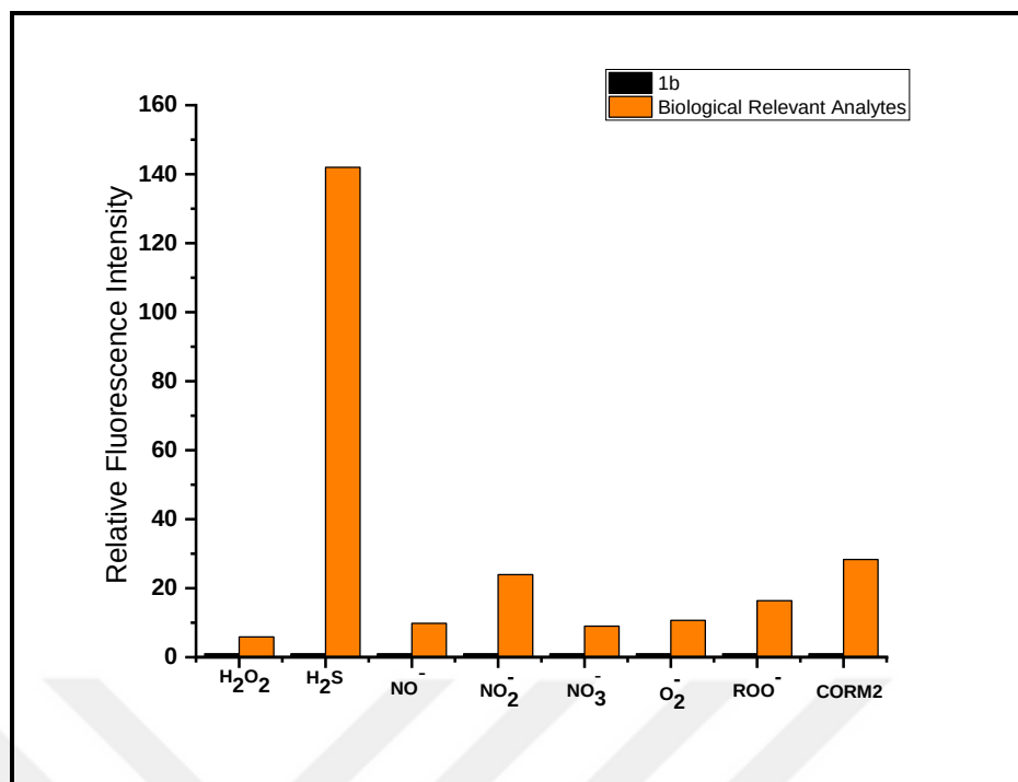
Figure 4.18. Fluorescence intensities of 1b (5 \mu M) towards other biologically relevant analytes and reactive oxygen species (40 eq) along with CORM-2 in 0.01 M PBS/EtOH (pH 7.4, v/v, 1:1), ( \lambda_{\text{ex}} : 500 nm).
