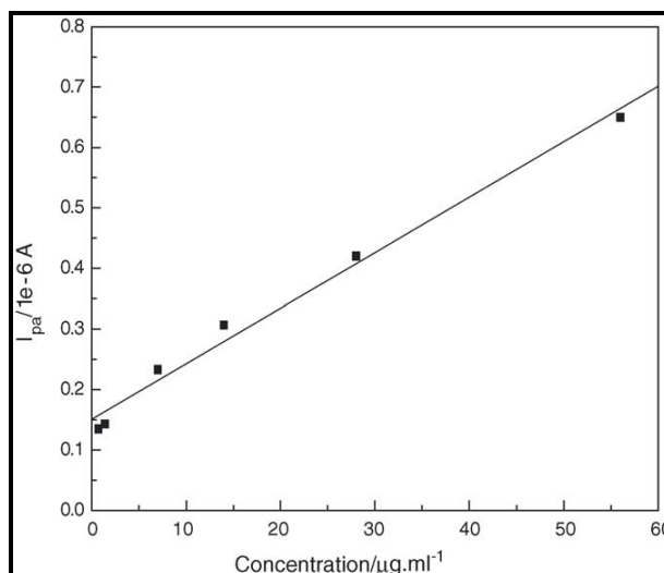
Figure 2.4. The linear relationship between current and the concentration of CO (Source: Chen et al., 2005).
