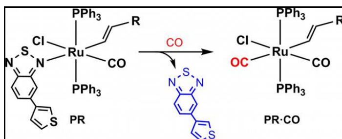
Figure 2.16. Reaction of the probes with CO (Source: Toscani et al., 2018).
