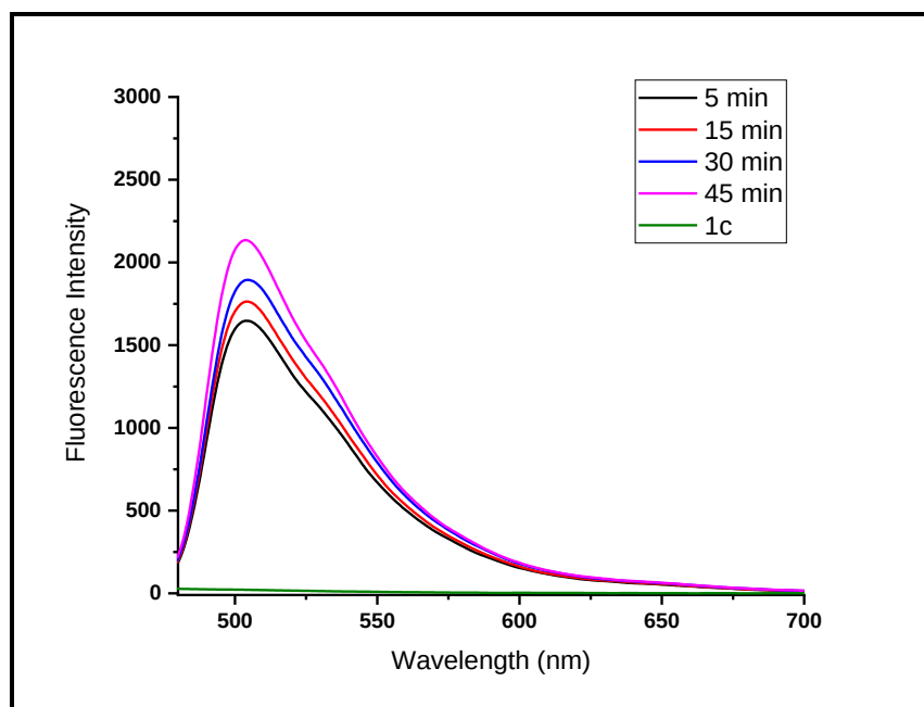
Figure 4.30. Reaction time profiles of 1c (5 μM) in the presence of CORM-2 (5eq.) in 0.01 M PBS (pH 7.4), ( \lambda_{\text{ex}} : 460 nm).
