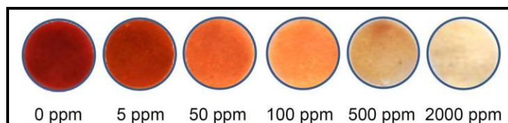
Figure 2.17. Color change of the complex adsorbed with silica according to increasing CO concentration (Source: Toscani et al., 2018).
