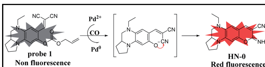
Figure 2.29. Sensing mechanism of the probe (Source: Chen et al., 2021).
