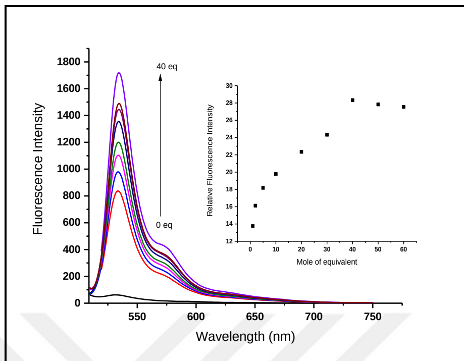
Figure 4.16. Fluorescence spectra of 1b (5 \mu\text{M} ) in the presence of the increasing amount of CORM-2 (0-40 eq.) in 0.01 M PBS/EtOH (pH 7.4, v/v,1:1), ( \lambda_{\text{ex}} : 500 nm).
