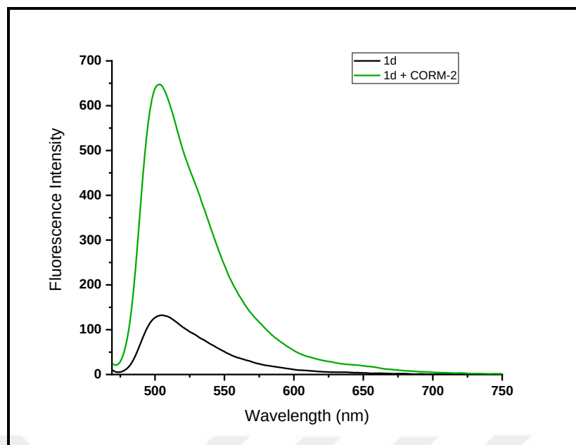
Figure 4.40. Fluorescence spectra of 1d (5 \mu M) in the absence and presence of 2 eq. CORM-2 in 0.01 M PBS/EtOH (pH 7.4, v/v, 9:1), ( \lambda_{\text{ex}} : 460 nm).
