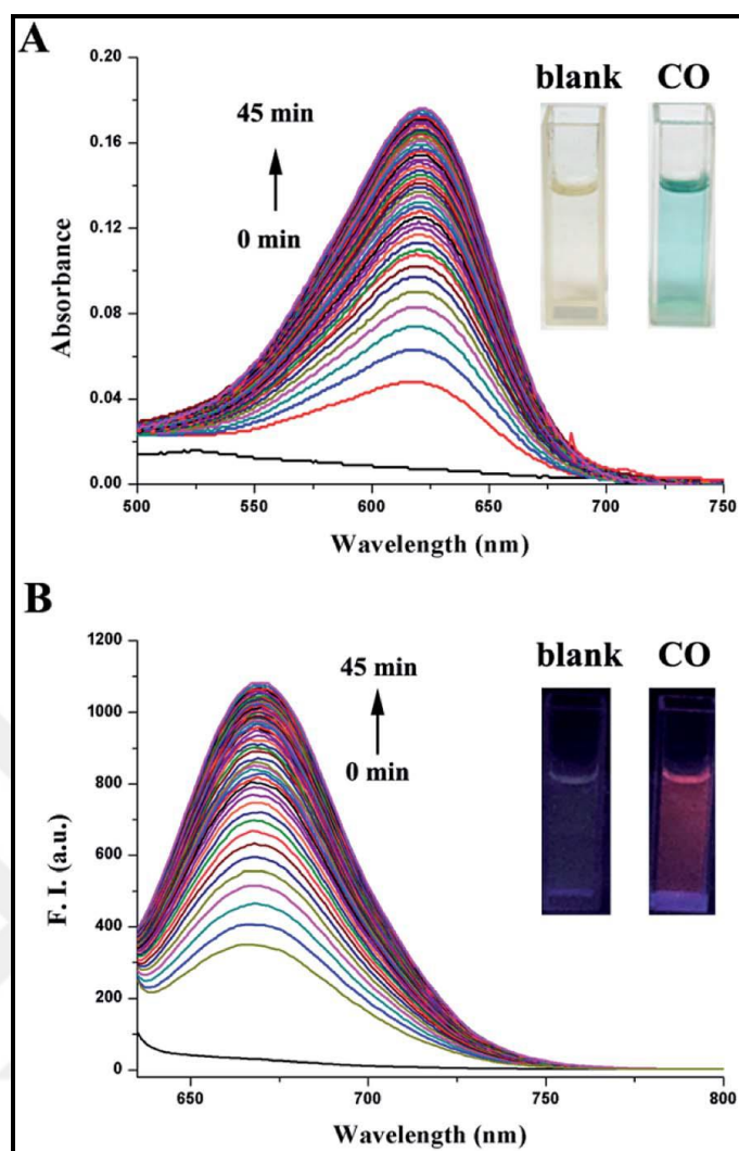
Figure 2.15. A) Absorbance and B) fluorescence spectra of the probe in the absence and presence of CORM (Source: Yan et al., 2016).
