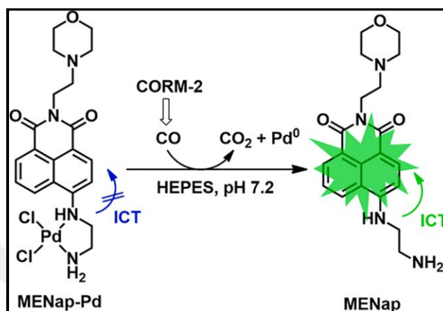
Figure 2.36. Probe response mechanism in CO environment (Source: Saha and Saha, 2020).
