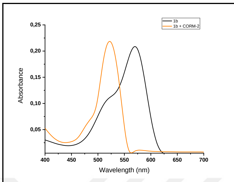
Figure 4.13. Absorbance spectra of 1b (5 \mu M) in the absence and presence of CORM-2 in 0.01 M PBS/EtOH (pH 7.4, v/v, 1:1).
