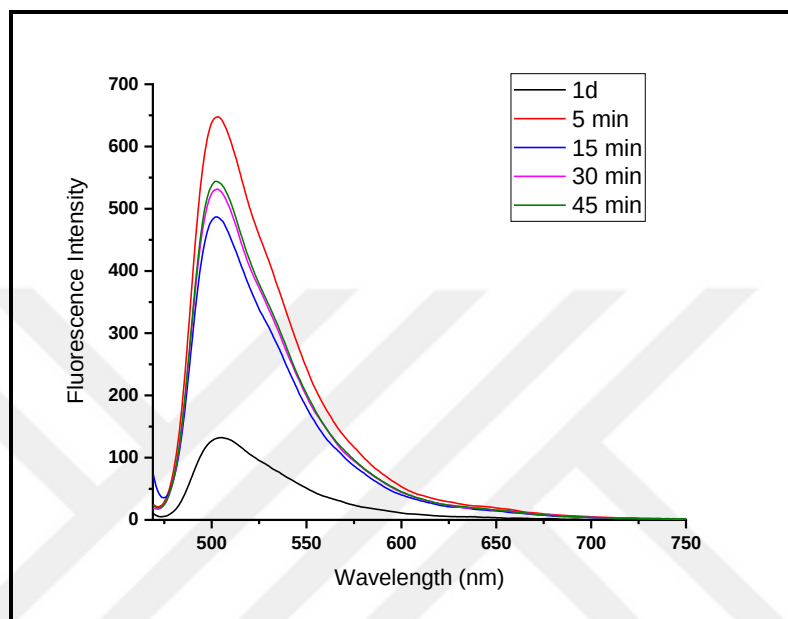
Figure 4.44. Reaction time profiles of 1d (5 \mu M) in the presence of CORM-2 (2 eq.) in 0.01 M PBS/EtOH (pH 7.4, v/v,9:1), ( \lambda_{\text{ex}} : 460 nm).
