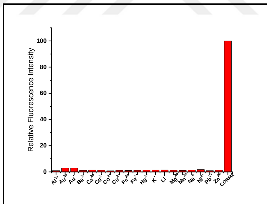
Figure 4.61. Bar graph notation of fluorescence intensities of 1e (5 \mu M) with metal species and CORM-2 (250 \mu M, 50 eq.) in 0.01 M PBS/DMF (pH 7.4, v/v, 8:2), ( \lambda_{\text{ex}} : 520 nm).
