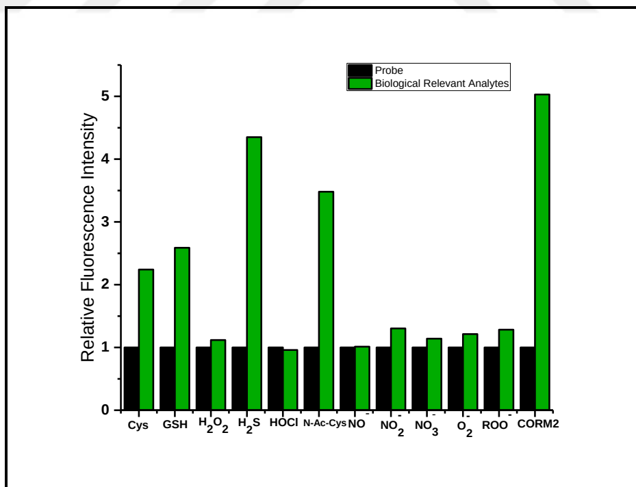
Figure 4.46. Fluorescence intensity of 1d (5 \mu M) in the presence of biologically relevant analytes, reactive oxygen species, and CORM-2 (2eq.) in 0.01 M PBS/EtOH (pH 7.4, v/v,9:1), ( \lambda_{\text{ex}} : 460 nm).
