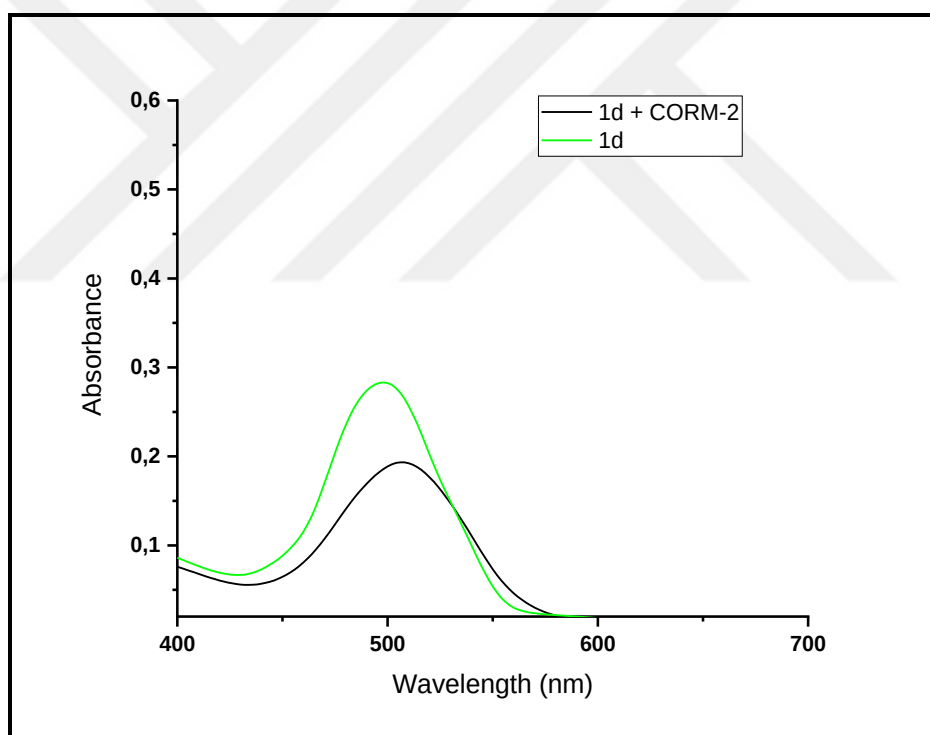
Figure 4.39. Absorbance spectra of 1d (5 \mu M) in the absence and presence of 2eq. CORM-2 in 0.01 M PBS/EtOH (pH 7.4, v/v, 9:1).
