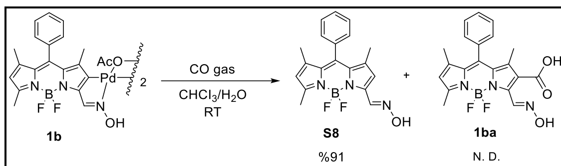
Figure 4.2. Reaction with carbon monoxide gas of the probe 1b .
