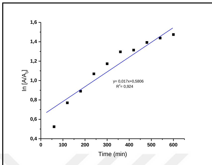
Figure 4.35. \ln (A_t/A_0) /time graphic of 1c .
