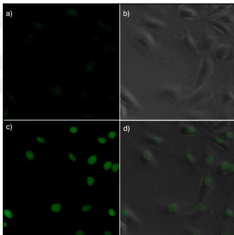
Figure 4.38. Fluorescence images of A549 cells. (a) fluorescence image of cells treated with only 1c (1 \mu\text{M} ) (control); (b) bright field image of cells treated with 1c (1 \mu\text{M} ) in CO environment; (c) fluorescence image of cells treated with 1c (1 \mu\text{M} ) in CO environment; (d) merged images of frames (b and c). ( \lambda_{\text{ex}} :460 nm), scale bar: 100 \mu\text{m} .
