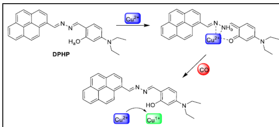
Figure 2.22. Sensing mechanism of the probe (Source: Bai et al., 2022).
