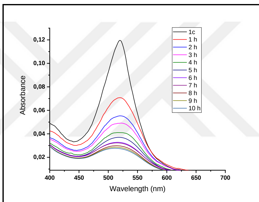
Figure 4.34. Absorbance change of 1c over time under green led.
