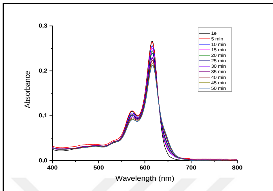
Figure 4.65. Absorbance change of 1e over time under red led.
