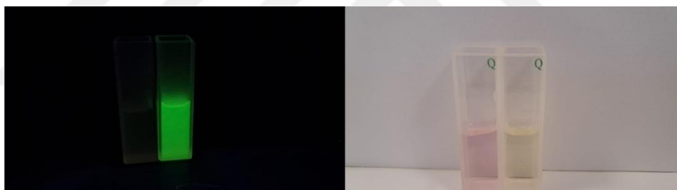
Figure 4.36. 1c photographs in UV (left) and daylight (right) in the absence (left ones) and presence (right ones) of CORM-2.
