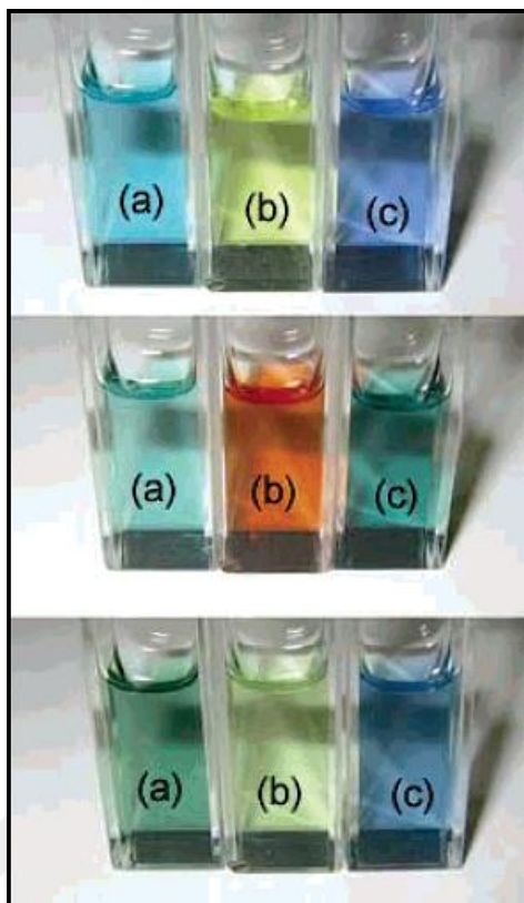
Figure 2.10. Color changes of ruthenium complexes. a) A ruthenium complex; b) One electron reduced ruthenium complex; c) CO exchange ruthenium complex with three different ligands (Source: Itou et al., 2006).
