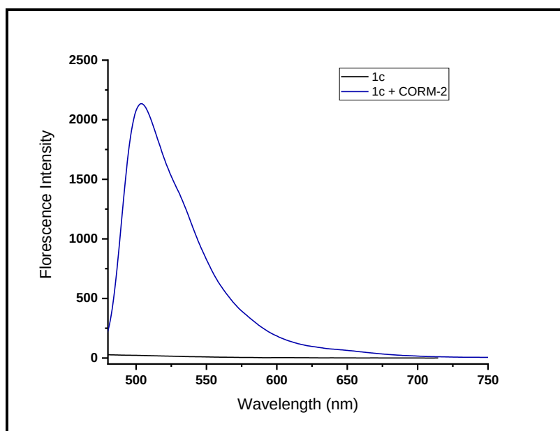
Figure 4.27. Emission spectra of 1c (5 μM) in the absence and presence of CORM-2 (5 eq.) in 0.01 M PBS (pH 7.4), (λ ex : 460 nm).
