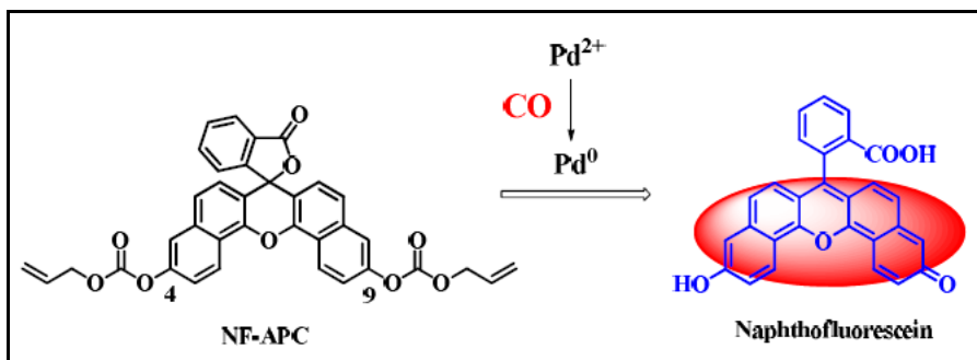
Figure 2.24. Sensing mechanism of the probe (Source: Yan et al., 2016).
