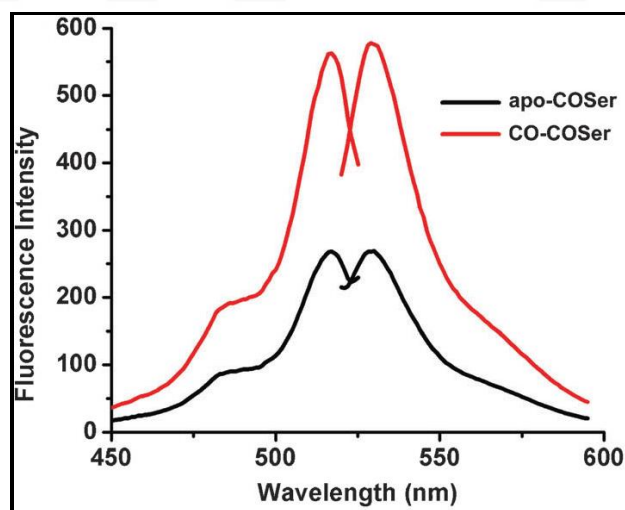
Figure 2.18. Fluorescence emission of the probe before and after CO addition (Source: Wang et al., 2012).
