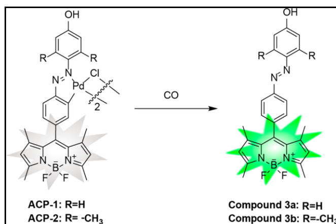
Figure 2.33. Sensing mechanism of the probes towards CO (Source: Li et al., 2016).
