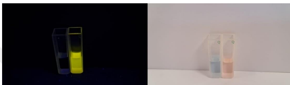
Figure 4.62. 1e photographs in UV (left) and daylight (right) in the absence (left ones) and presence (right ones) of CORM-2.
