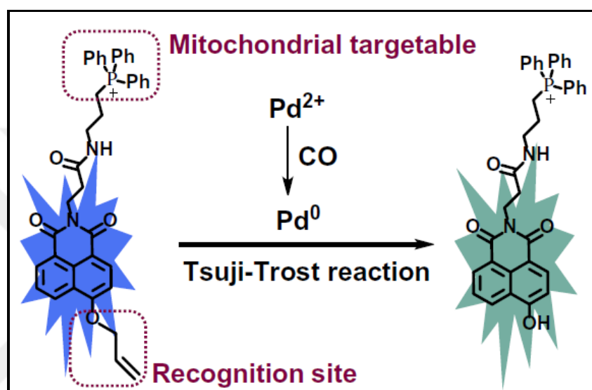
Figure 2.28. The ratiometric sensing mechanism of the probe (Source: Du et al., 2021).
