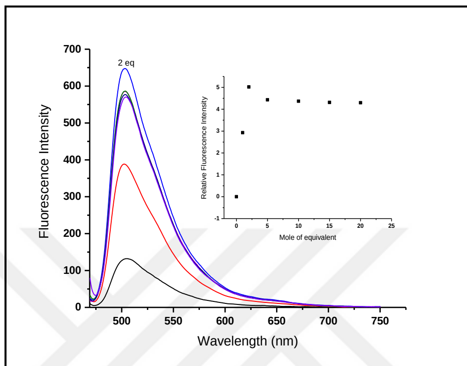
Figure 4.43. Fluorescence spectra of 1d (5 \mu M) in the presence of the increasing amount of CORM-2 (0-25 eq) in 0.01 M PBS/EtOH (pH 7.4, v/v,9:1), ( \lambda_{\text{ex}} : 460 nm).
