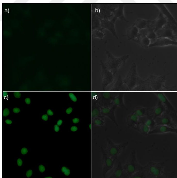
Figure 4.24. Fluorescence images of A549 cells. (a) fluorescence image of cells treated with only 1b (1 \mu M) (control); (b) bright field image of cells treated with 1b (1 \mu M) in CO environment; (c) fluorescence image of cells treated with 1b (1 \mu M) in CO environment; (d) merged images of frames (b and c). ( \lambda_{ex} :500 nm), scale bar: 100 \mu m.
