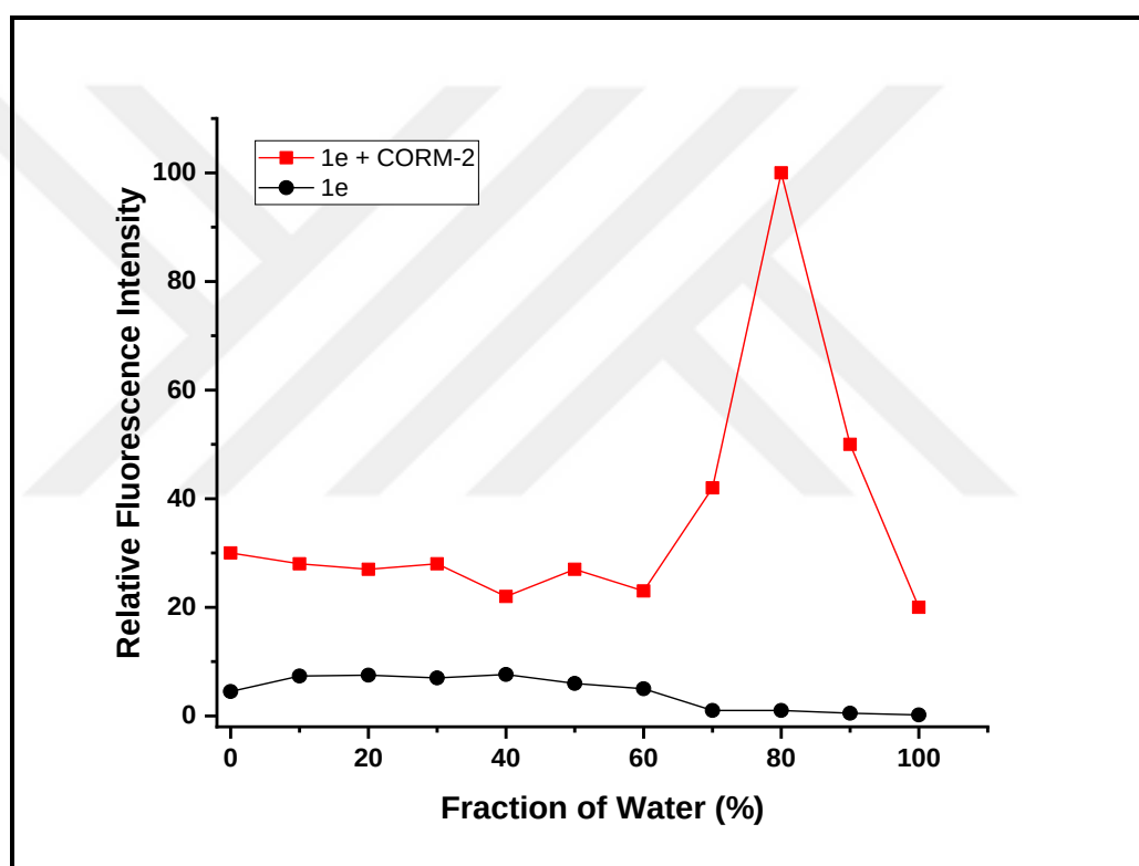
Figure 4.53. Effect of the fraction of water on the interaction of 1e (5 \mu M) with CORM-2 (50 \mu M) in 0.01M PBS/DMF (pH 7.4), ( \lambda_{\text{ex}} : 520 nm).
