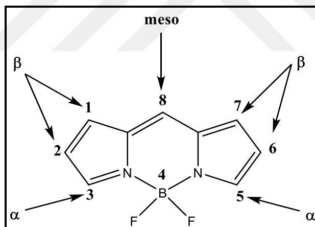
Figure 1.1. Structure of BODIPY
