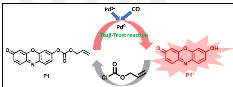
Figure 2.27. Proposed sensing mechanism of the probe (Source: Biswas et al., 2019).
