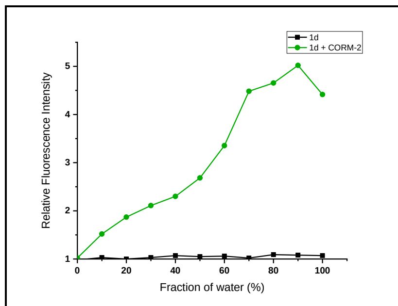
Figure 4.41. Effect of water fraction on fluorescence intensity of 1d (5 \mu M) in the presence and absence of CORM-2 (2 eq.) in 0.01 M PBS/EtOH (pH 7.4, v/v, 9:1), ( \lambda_{\text{ex}} : 460 nm).
