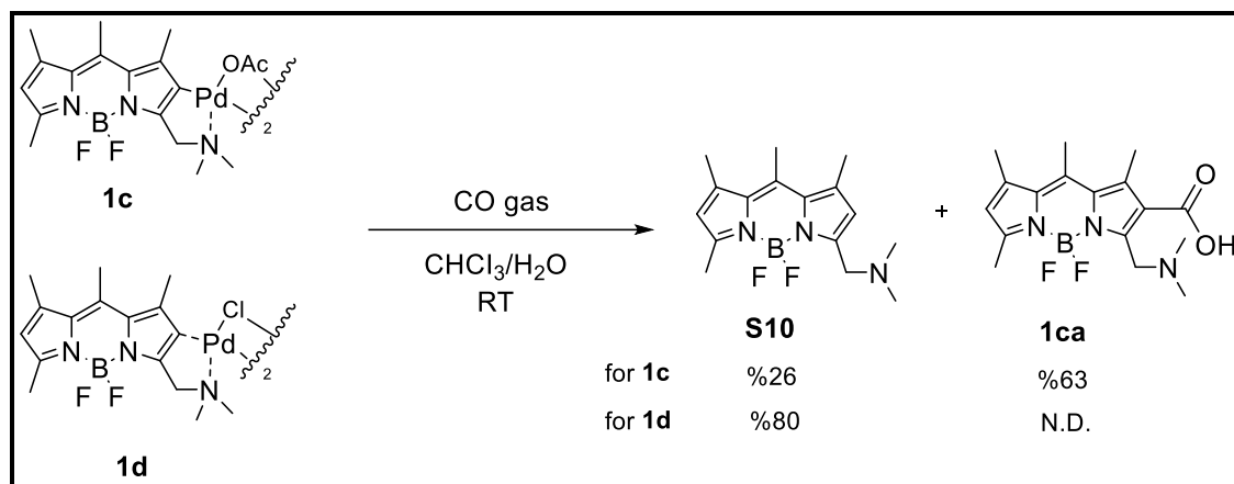
Figure 4.3. Reaction with carbon monoxide gas of the probe 1c and 1d .
