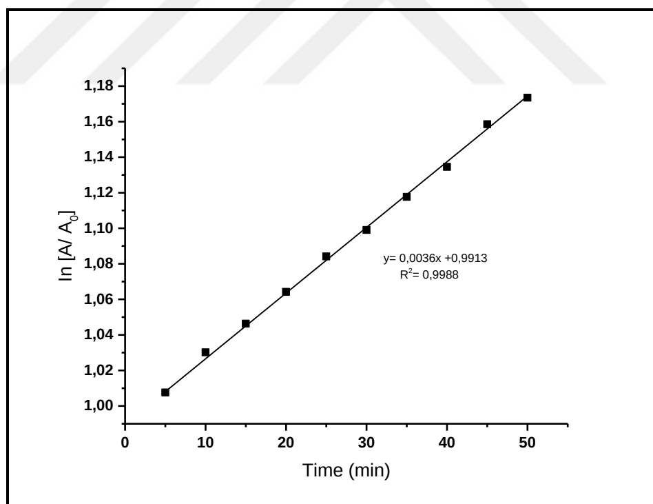
Figure 4.66. \ln (A_t/A_0) /time graphic of 1e .
