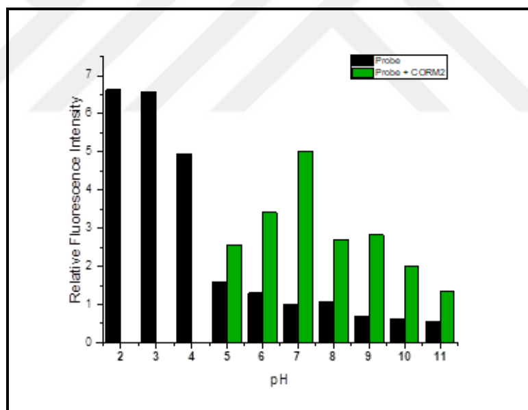
Figure 4.42. Effect of pH on 1d (5 \mu M) in the presence and absence of CORM-2 (2 eq.) in 0.01 M PBS/EtOH (pH 7.4, v/v, 9:1), ( \lambda_{\text{ex}} : 460 nm).
