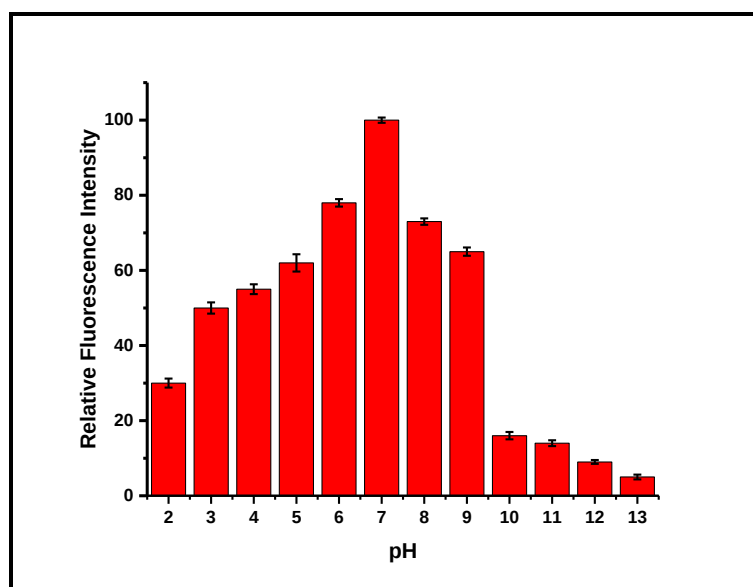
Figure 4.56. Effect of pH on the response of 1e (5 \mu M) toward CORM-2 (250 \mu M, 50 eq.) in 0.01 M PBS/DMF (pH 7.4, v/v, 8:2), ( \lambda_{\text{ex}} : 520 nm).
