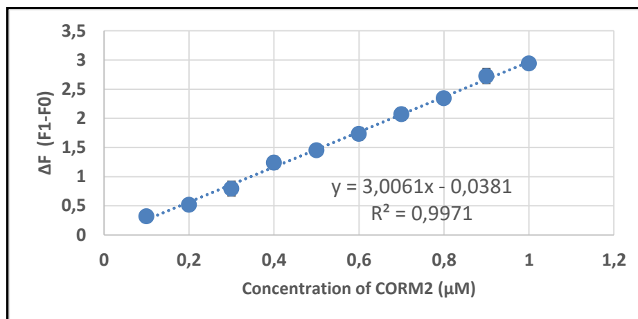
Figure 4.21. Fluorescence changes of 1b with the addition of CORM-2 at increasing concentrations in 0.01 M PBS/EtOH (pH 7.4, v/v, 1:1), ( \lambda_{\text{ex}} : 500 nm).
