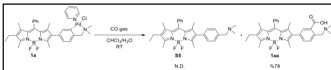
Figure 4.1. Reaction with carbon monoxide gas of the probe 1a .
