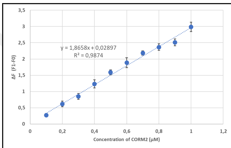
Figure 4.59. Fluorescence changes of 1e (5 \mu\text{M} ) upon the addition of CORM-2 (0.1 to 1 \mu\text{M} ) in 0.01 M PBS/DMF (pH 7.4, v/v, 8:2), ( \lambda_{\text{ex}} : 520 nm).
