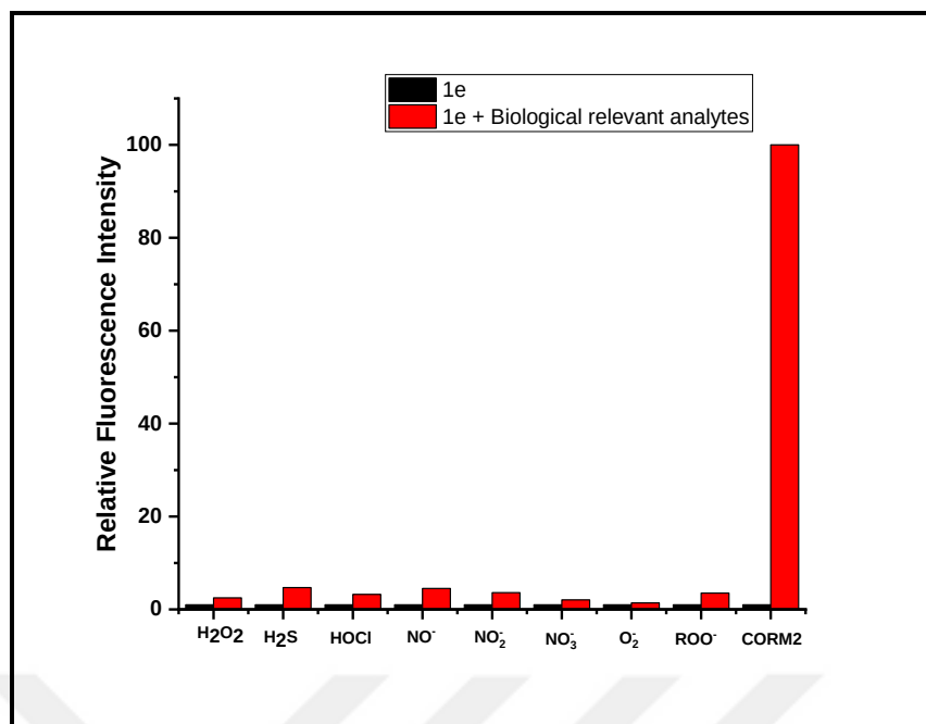
Figure 4.60. Bar graph notation of fluorescence intensities of 1e (5 \mu M) with reactive oxygen species and CORM-2 (250 \mu M, 50 eq.) in 0.01M PBS/DMF (pH 7.4, v/v, 8:2), ( \lambda_{\text{ex}} : 520 nm).
