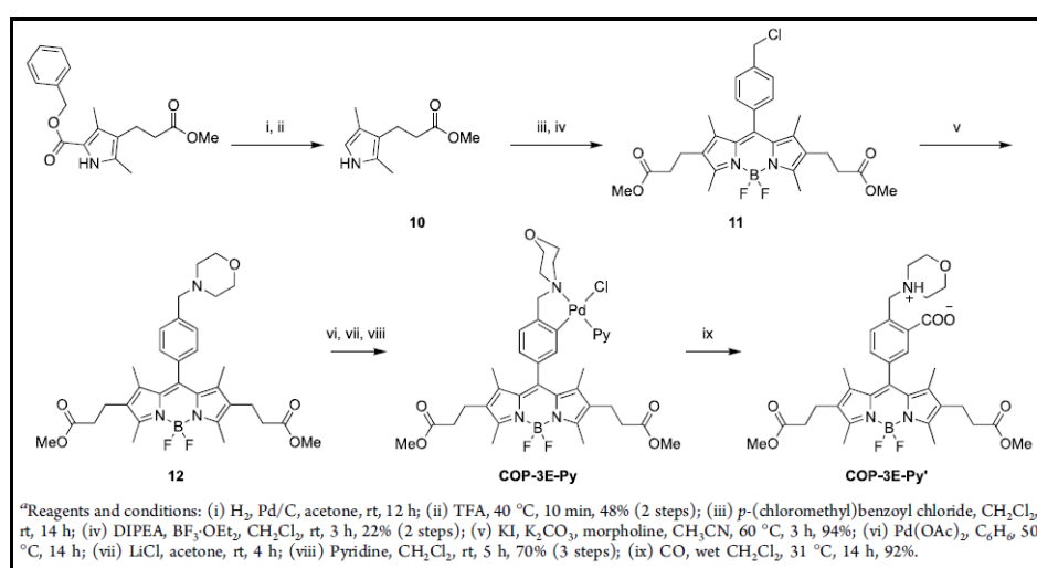
Figure 2.35. Synthetic route of the COP-3E-Py and reaction with CO (Source: Morstein et al., 2020).
