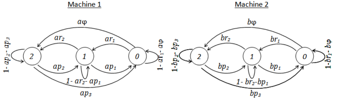
Figure 2 : State Transitions of Machine 1 and Machine 2
