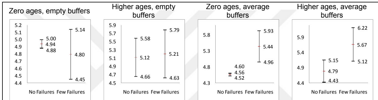
Figure 4 : Impact of Initial Machine Failures on Bottleneck Status of Dash under Different Initial Conditions
