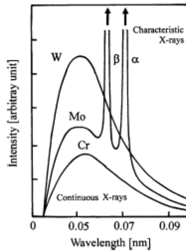
Figure 2.2: Schematic representation of X-ray spectrum [110]
