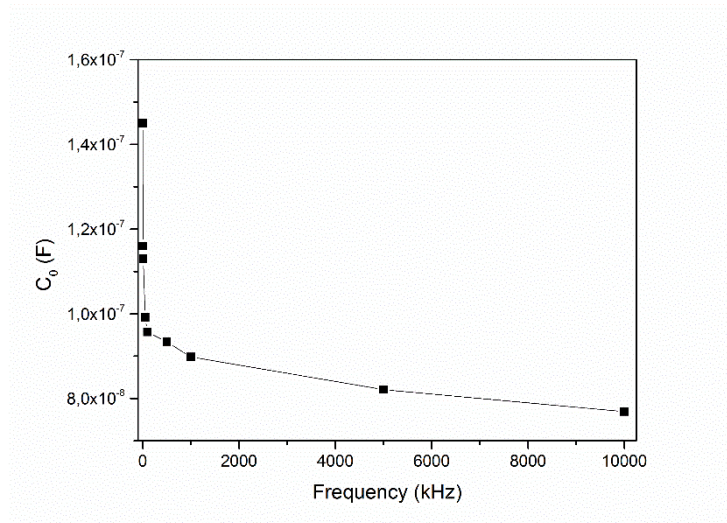
Figure 5.30: The variation of capacitance at zero bias with frequency in the p-CAIS/n-Si device
