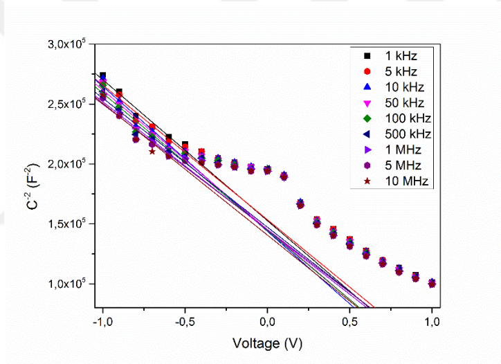
Figure 6.14: The variation of C^{-2} with voltage for the n-ZIS/p-CAIS device at different frequencies
