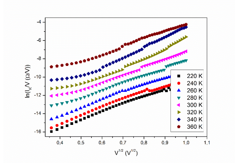
Figure 6.12: Plot of \ln(I_R/V) versus (V)^{1/2} for the n-ZIS/p-CAIS device.
