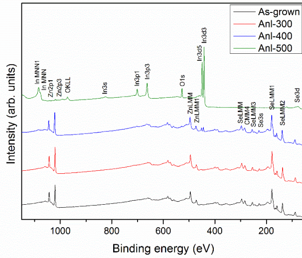
Figure 4.6: The XPS spectra of the as-grown and annealed ZIS thin films at different temperatures after first sputtering
