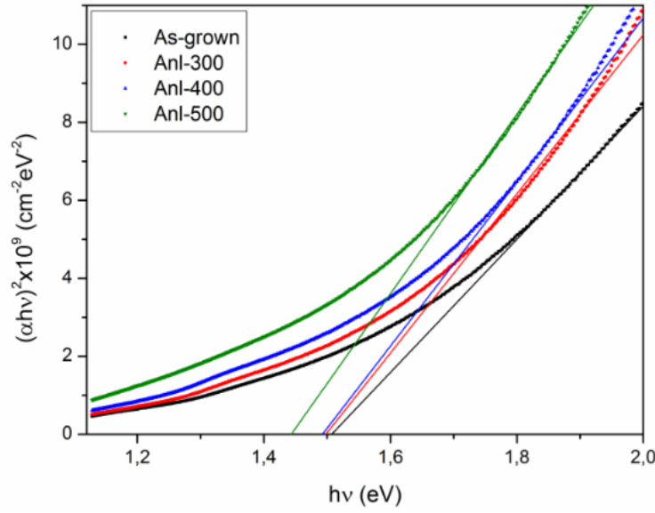
Figure 5.12: The variation of (\alpha h\nu)^2 with the photon energy for CAIS samples
