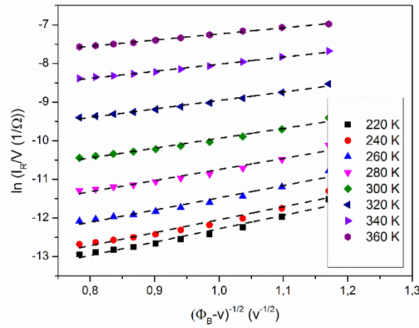
Figure 5.27: Plot of \ln(I_R/V) versus (\Phi_b - V)^{-1/2} for the p-CAIS/n-Si device.
