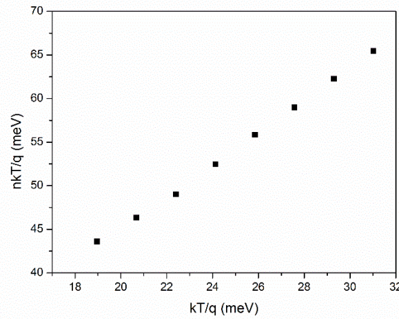
Figure 6.7: Plot of nkT/q versus kT/q for the n-ZIS/p-CAIS device.
