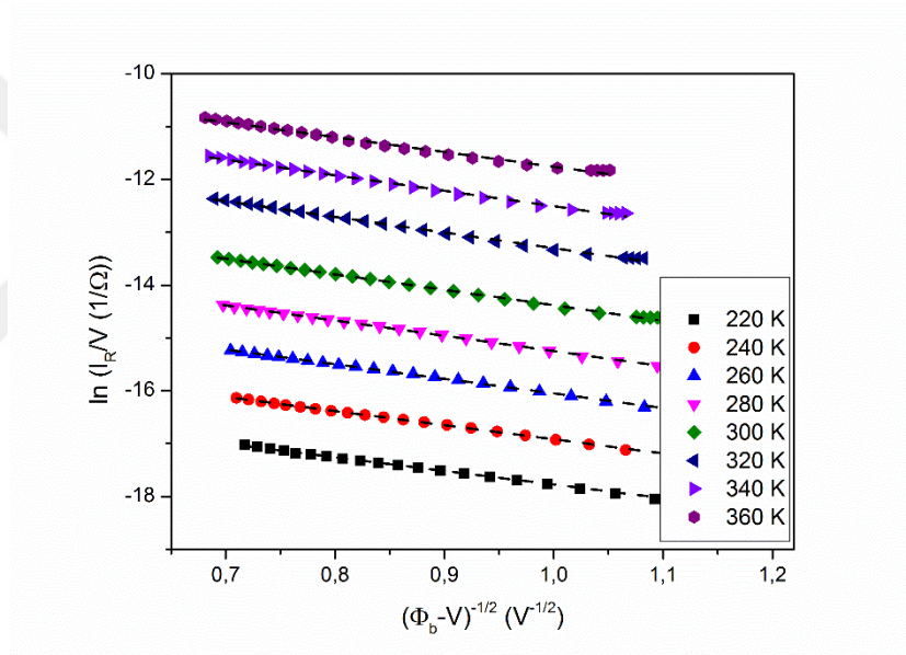
Figure 4.36: Plot of \ln(I_R/V) versus (\Phi_b - V)^{-1/2} for the n-ZIS/p-Si device.
