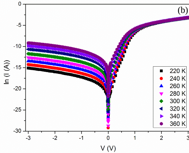
Figure 4.26: (a) Linear and (b) semi-logarithmic I-V plots of n-ZIS/p-Si hetero-junction at different ambient temperatures.
