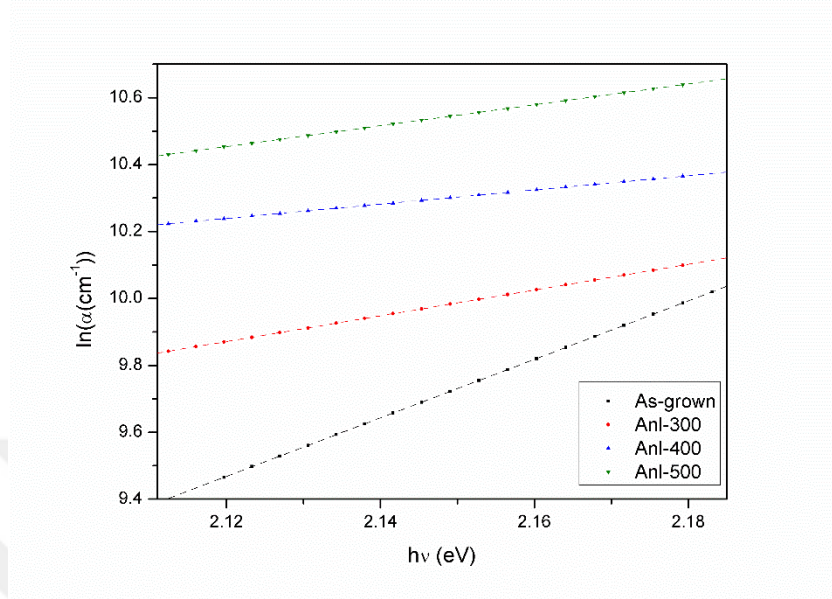
Figure 4.18: Plots of \ln(\alpha) versus h\nu for ZIS samples
