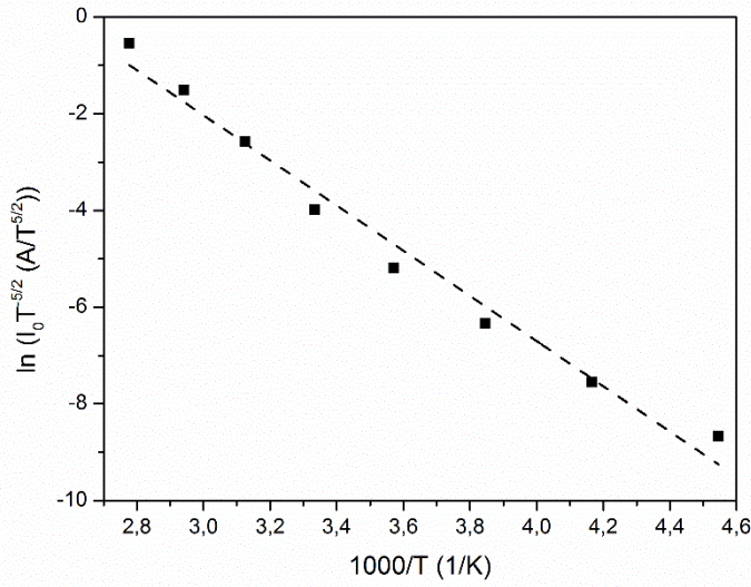
Figure 4.31: Plot of \ln(I_0 T^{-5/2}) versus 1000/T for the n-ZIS/p-Si device.
