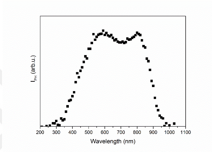
Figure 6.18: Photo-current versus wavelength plot of the n-ZIS/p-CAIS device.
