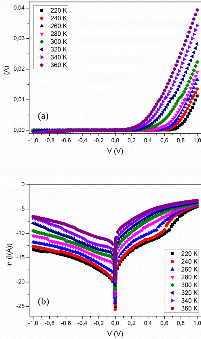
Figure 6.1: (a) Linear and (b) semi-logarithmic I-V plots of n-ZIS/p-CAIS hetero-junction at different ambient temperatures.
