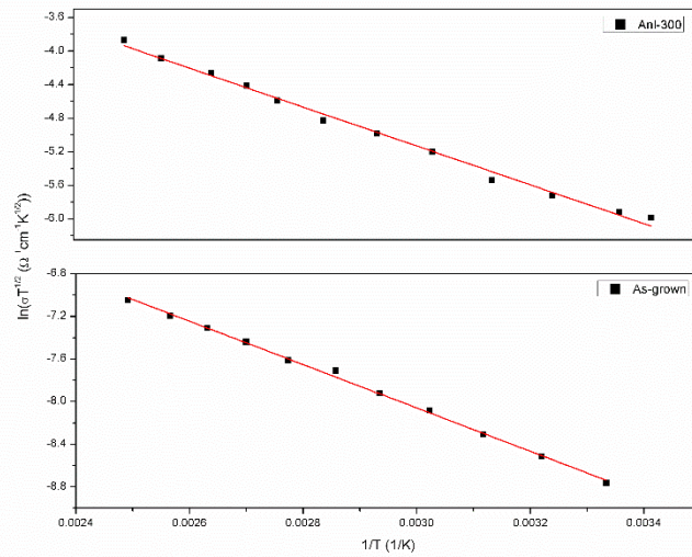
Figure 4.20: Plots of \ln(\sigma T^{1/2}) versus T^{-1} in the high-temperature region for the ZIS film in as-grown form and annealed at 300 °C. Solid lines are the best fit lines according to Eq. 4.21
