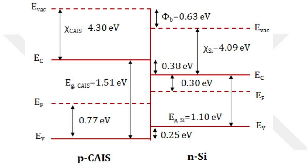
Figure 5.31: The band diagram of the p-CAIS/n-Si device
