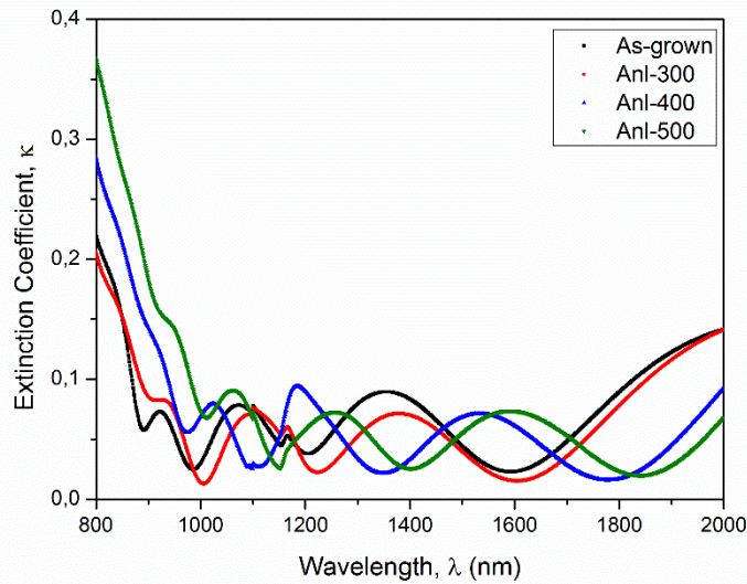
Figure 4.14: Calculated extinction coefficients for the ZIS samples
