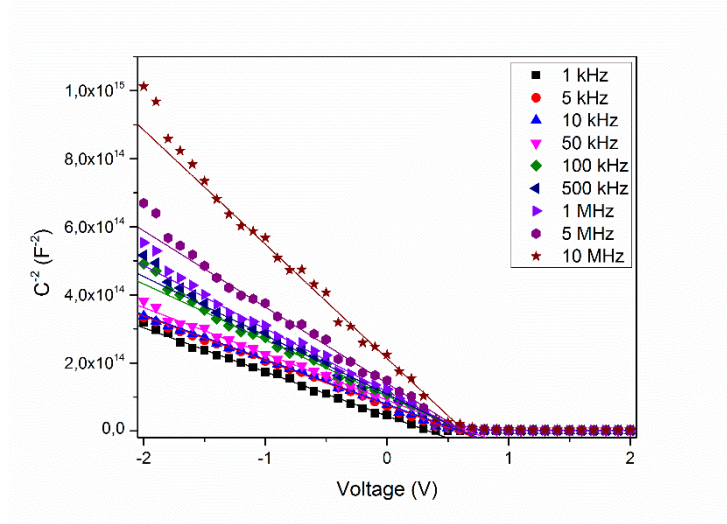
Figure 5.29: The variation of C^2 with voltage for the p-CAIS/n-Si device under different frequencies
