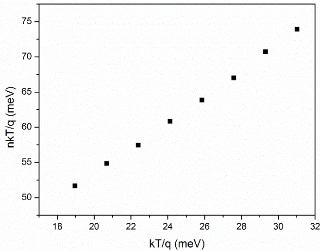
Figure 4.32: Plot of nkT/q versus kT/q for the n-ZIS/p-Si device.
