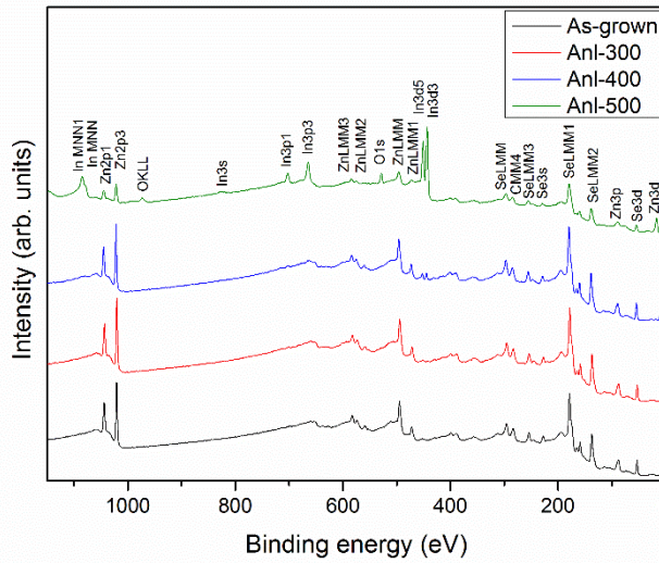
Figure 4.7: The XPS spectra of the as-grown and annealed ZIS thin films at different temperatures after second sputtering
