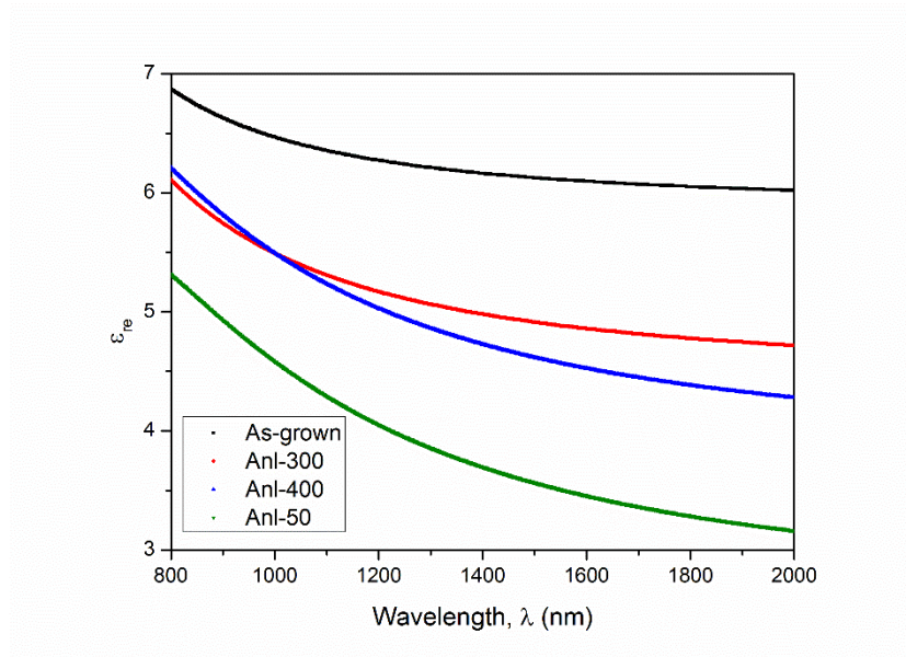
Figure 4.15: Real part of the dielectric constants for the ZIS samples
