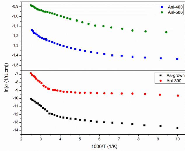
Figure 4.19: Temperature dependent electrical conductivity of as-grown and annealed ZIS films
