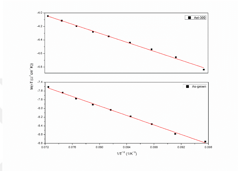
Figure 4.22: Plots of \ln(\sigma T) versus T^{-1/2} in the high-temperature region for the ZIS film in as-grown form and annealed at 300 °C. Solid lines are the best fit lines according to Eq. 4.27
