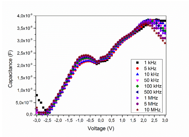
Figure 6.13: Room temperature C-V plots of the n-ZIS/p-CAIS device at different frequencies
