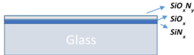
Figure 65: Substrate with buffer layer stack
