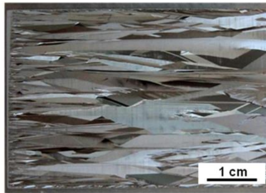
Figure 63: 10 \mu\text{m} silicon layer crystallized by cw-diode laser [135]
