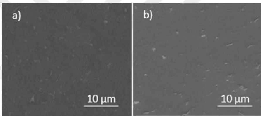
Figure 45: Scanning electron micrographs taken from the seed layer annealed at 450°C (a), and the absorber grown on this layer following 600°C annealing (b). The surface features visible on both images are thought to be discontinuities in film thickness where two crystals coalesced during the AIC process. Similar features being present in both surfaces is indicative that the epitaxial growth occurred in the absorber layer.
