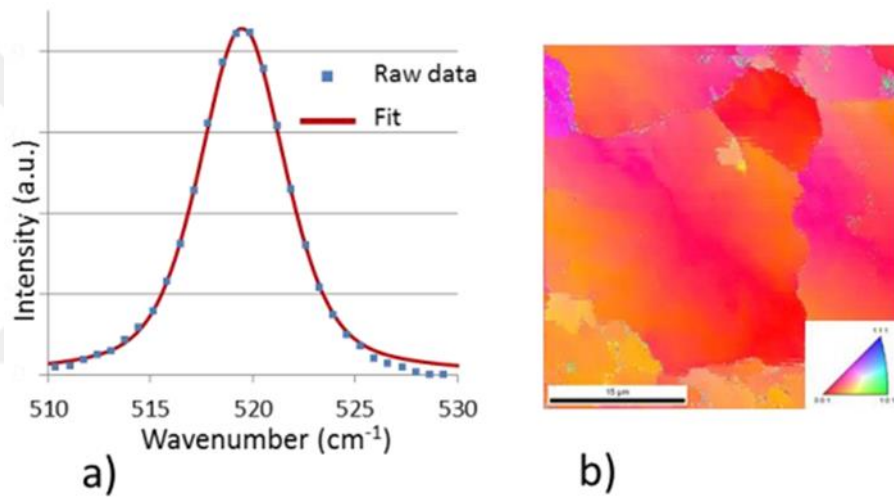
Figure 47: Structure of the SPE absorber layer (Al etch prior to absorber deposition), a) Raman peak with a Lorentzian/Gaussian fit, and b) EBSD image.
