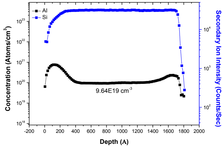
Figure 39: SIMS profile of standard AIC poly-Si film
