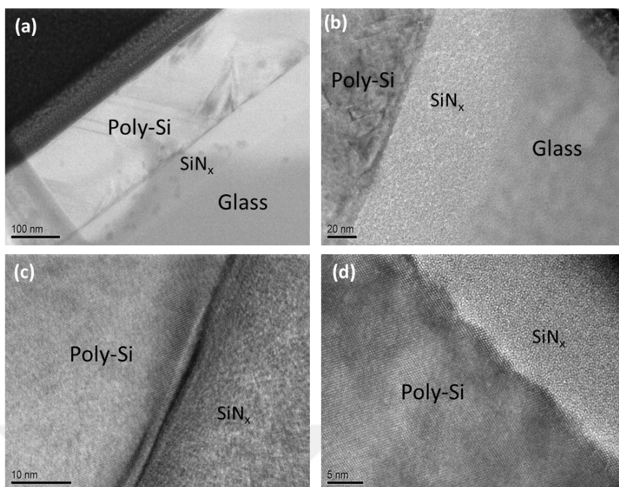
Figure 40: TEM images of standard AIC poly-Si film
