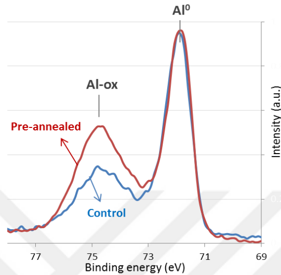
Figure 52: Comparison of the normalized photoelectron spectra showing the highest Al-oxide peak for the control and pre-annealed samples.
