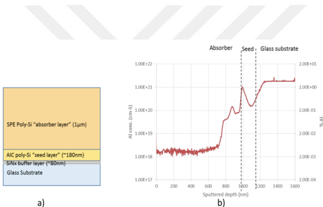
Figure 46: SPE absorber a) a sketch showing the consecutive layers, and b) SIMS depth profile of after annealing at 550°C at 48hrs (w/out Al etch prior to absorber deposition).
