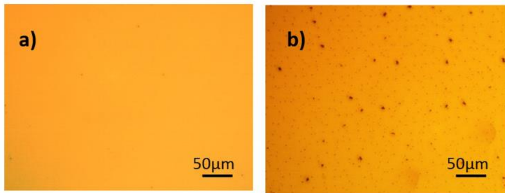
Figure 57: Optical micrographs from the a-Si / Al interface taken from samples from batches a) E-RT, and b) E-HT. The interface for the E-RT sample appears featureless, while small crystal nuclei are visible for the E-HT sample.
