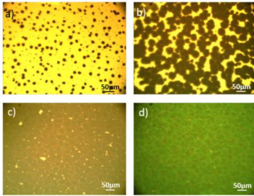
Figure 49: Optical micrographs taken from control samples annealed at 420 °C for varying durations: (a) 40, (b) 65, (c) 90, and (d) 120 min.
