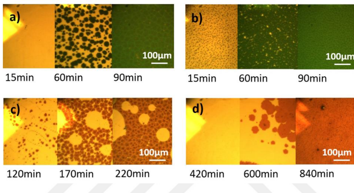
Figure 58: Optical micrographs taken from the a-Si / Al interface of samples annealed at 420 °C at varying annealing times (as given in the lower left corner insert for each micrograph), a) E-RT, b) E-HT, c) P-9, d) P-29.
