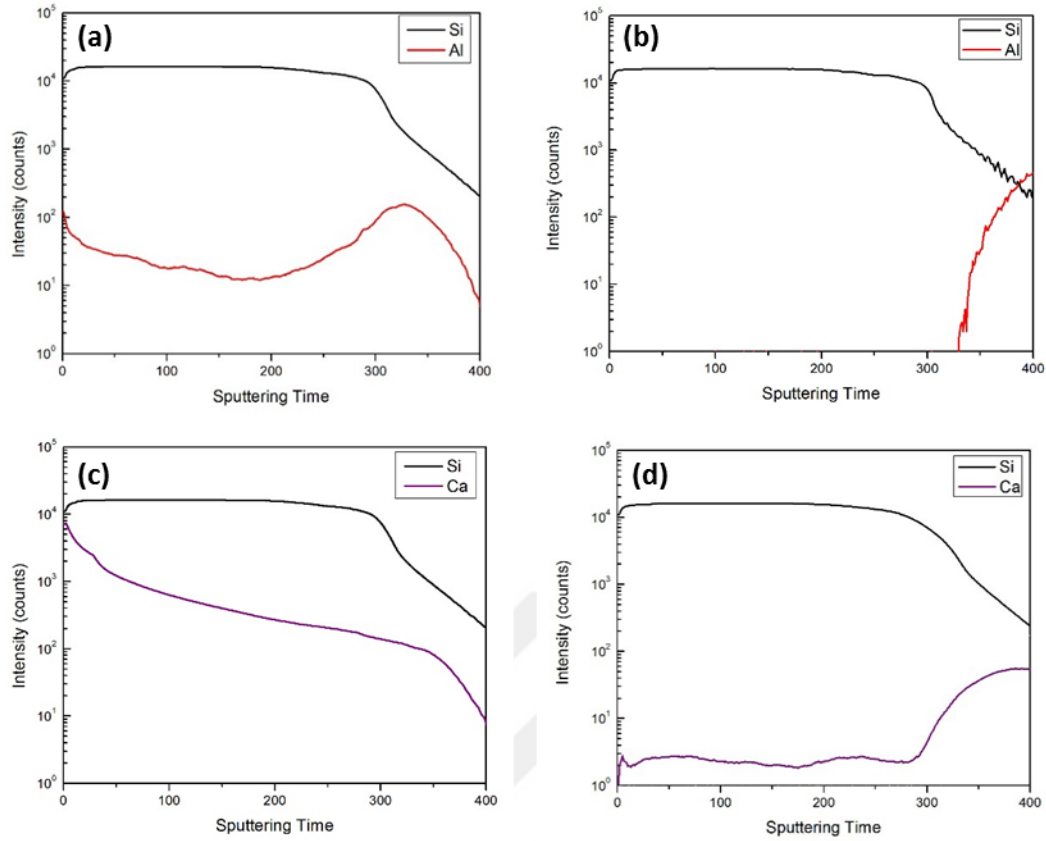
Figure 19: SIMS measurements of Si thin film on glass without (a, c) and with (b, d) SiN x buffer layer [99].
