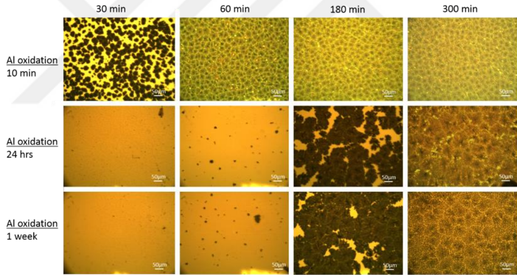
Figure 41: Optical micrographs taken at various durations of annealing at 500°C of AIC samples with different Al-oxidation conditions.
