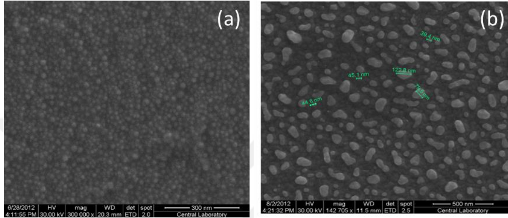
Figure 10: SEM image of AuNPs on AZO film after 1h of annealing at 500 °C by 5 nm Au film (a) and 15 nm Au film.
