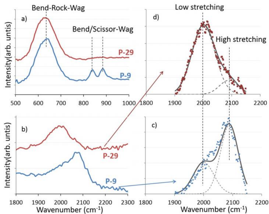
Figure 62: Normalized FTIR spectra taken from the as-deposited a-Si films from batches P-9 and P-29: a) Bend modes, b) stretch modes, c) Gaussian
