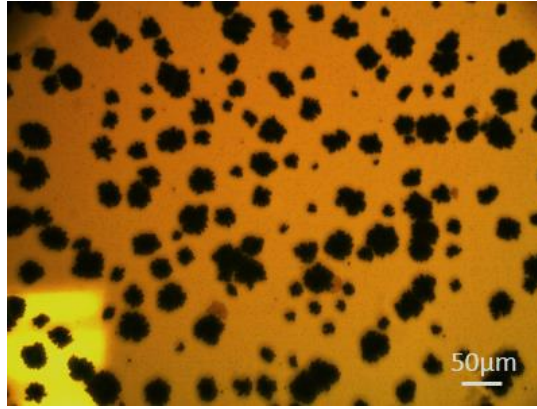
Figure 26: Optical micrograph taken from a-Si/Al/SiN x /glass sample annealed at 475°C for 2 hrs. Image was taken in reflection mode through the glass substrate.
