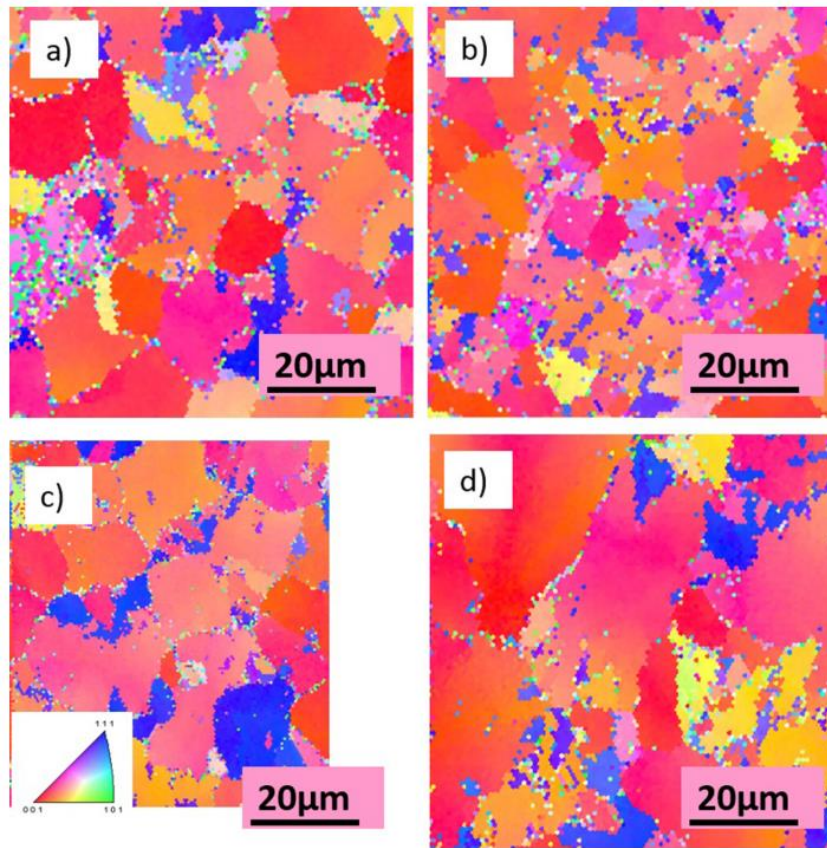
Figure 60: EBSD images taken from fully crystallized samples annealed at 450 °C, a) E-RT, b) E-HT, c) P-9, and d) P-29. The colors represents the orientation of grains according to the color code given in the lower left corner inset.
