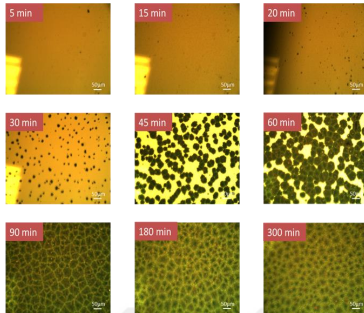
Figure 30: Optical micrographs taken from samples annealed at 500°C at varying annealing times (given in the upper left corner inset for each micrograph).
