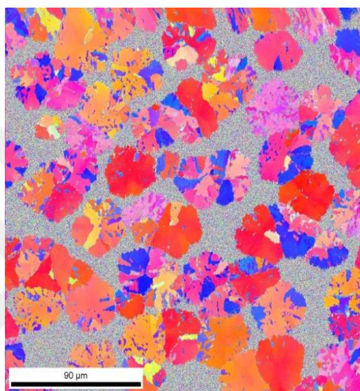
Figure 34: EBSD images taken from partially crystallized samples annealed at 500°C. The grainy (predominantly grey colored) background is Al, whereas the solid colored features are the Si grains. Some of the features consist of only one color (single crystal), while others have multiple colors (multi-crystalline).
