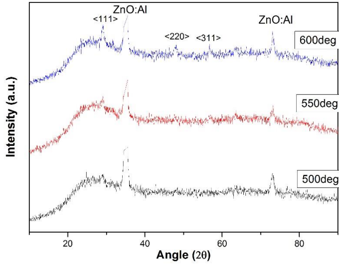
Figure 13: XRD measurements of samples with annealed for 12 h at 500 °C, 550 °C and 600 °C.
