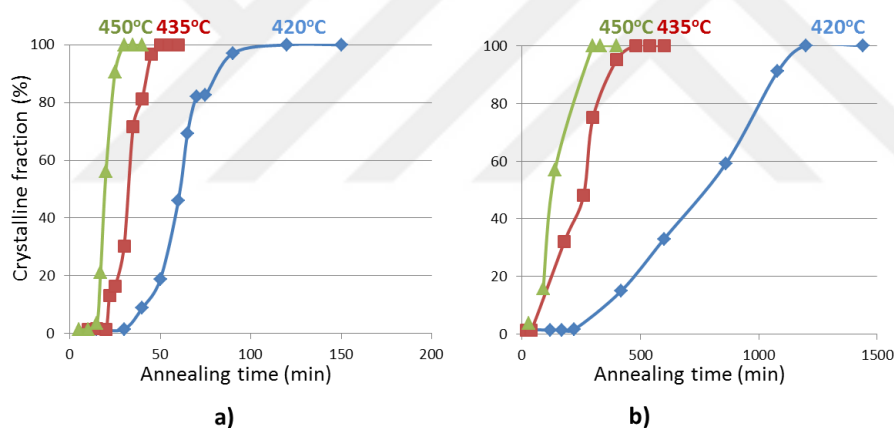
Figure 56: Crystallization percentage versus annealing time at 420, 435, and 450 °C: (a) control sample and (b) pre-annealed sample.
