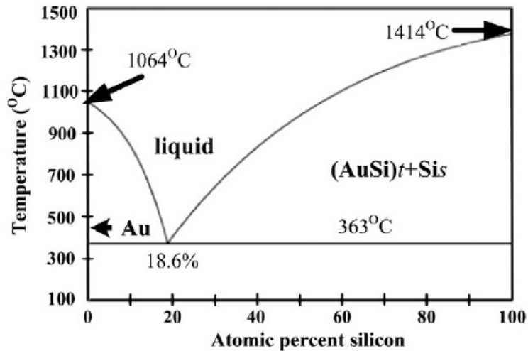
Figure 9: Au-Si equilibrium phase diagram [71].
