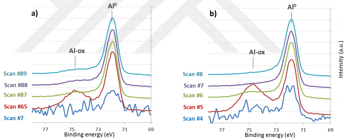
Figure 51: Selected XPS spectra taken from a-Si/Al/SiN x /glass stacks: (a) control sample and (b) pre-annealed sample. All spectra are normalized with respect to their maxima.
