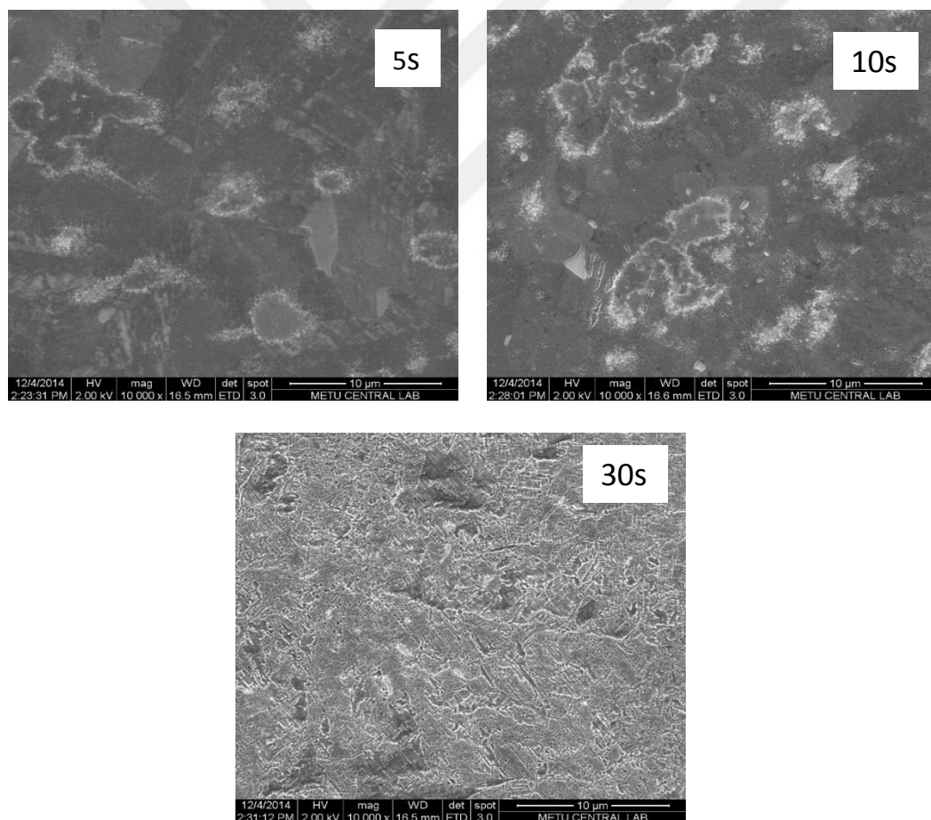
Figure 43: SEM images of \text{HNO}_3\text{:HF} solution etching
