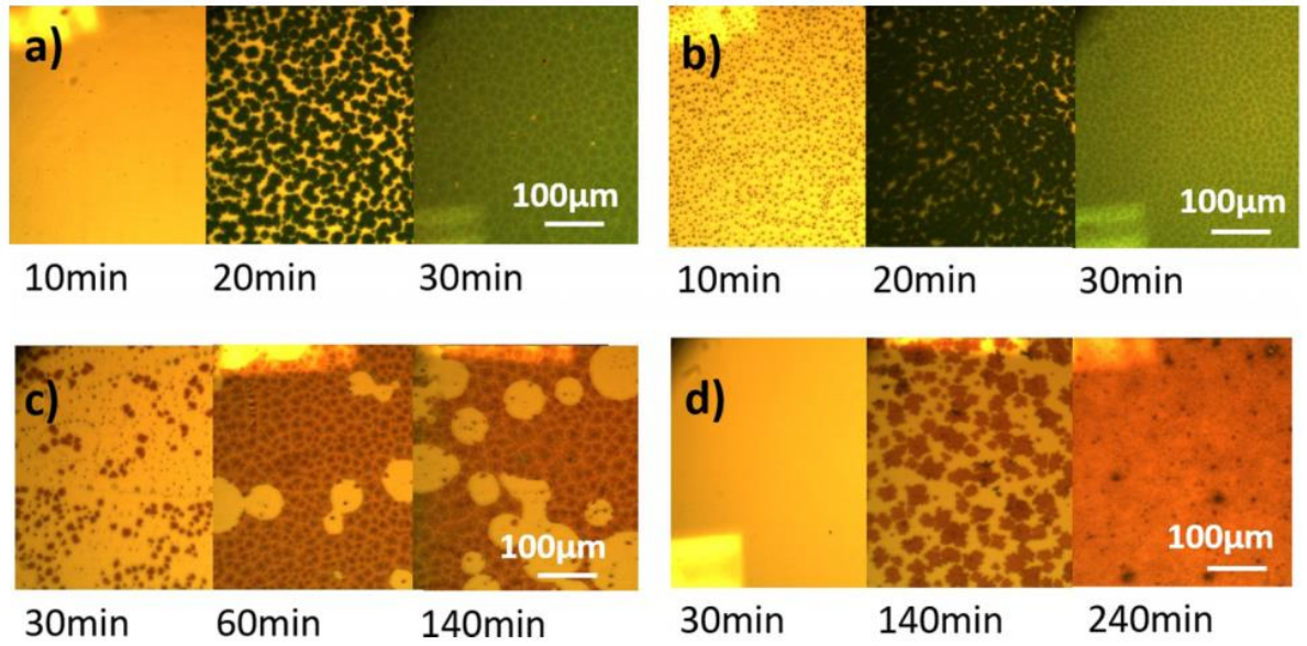
Figure 59: Optical micrographs taken from the a-Si / Al interface of samples annealed at 450°C at varying annealing times (as given in the lower left corner insert for each micrograph), a) E-RT, b) E-HT, c) P-9, d) P-29.
