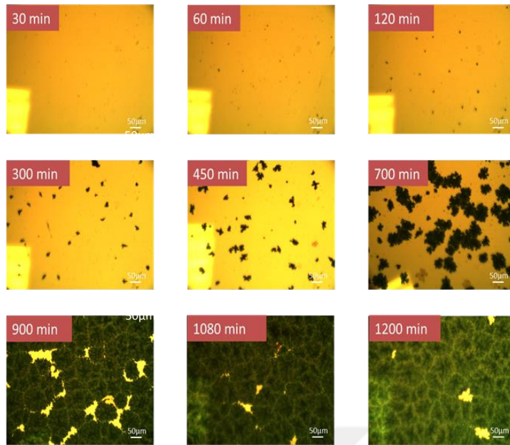
Figure 28: Optical micrographs taken from samples annealed at 450°C at varying annealing times (given in the upper left corner inset for each micrograph).
