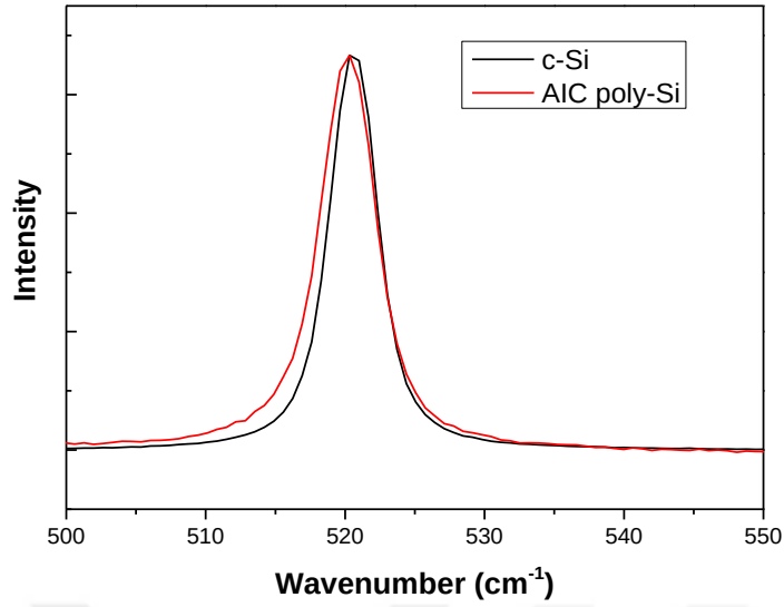
Figure 18: Raman spectroscopy of monocrystalline silicon and AIC poly-Si
