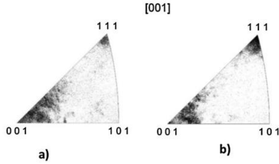
Figure 55: EBSD inverse pole figures showing the orientation distribution of poly-Si films in the direction normal to the surface: (a) control sample and (b) pre-annealed sample
