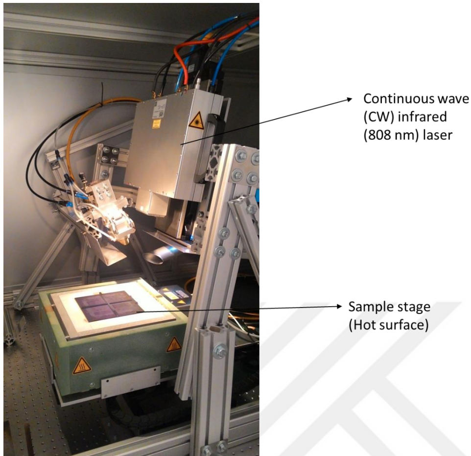
Figure 64: cw-diode laser system used at HZB, Germany
