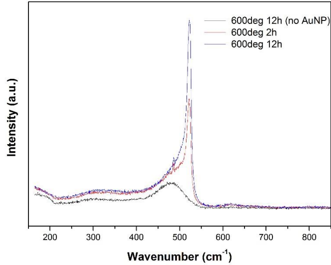
Figure 14: Raman measurements of the samples with and without AuNPs annealed at 600 °C
