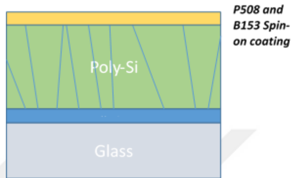
Figure 68: Spin-on dopant coating
