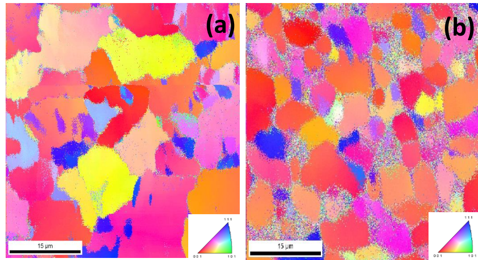
Figure 25: EBSD analysis of samples (a) “d” and (b) “f”.
