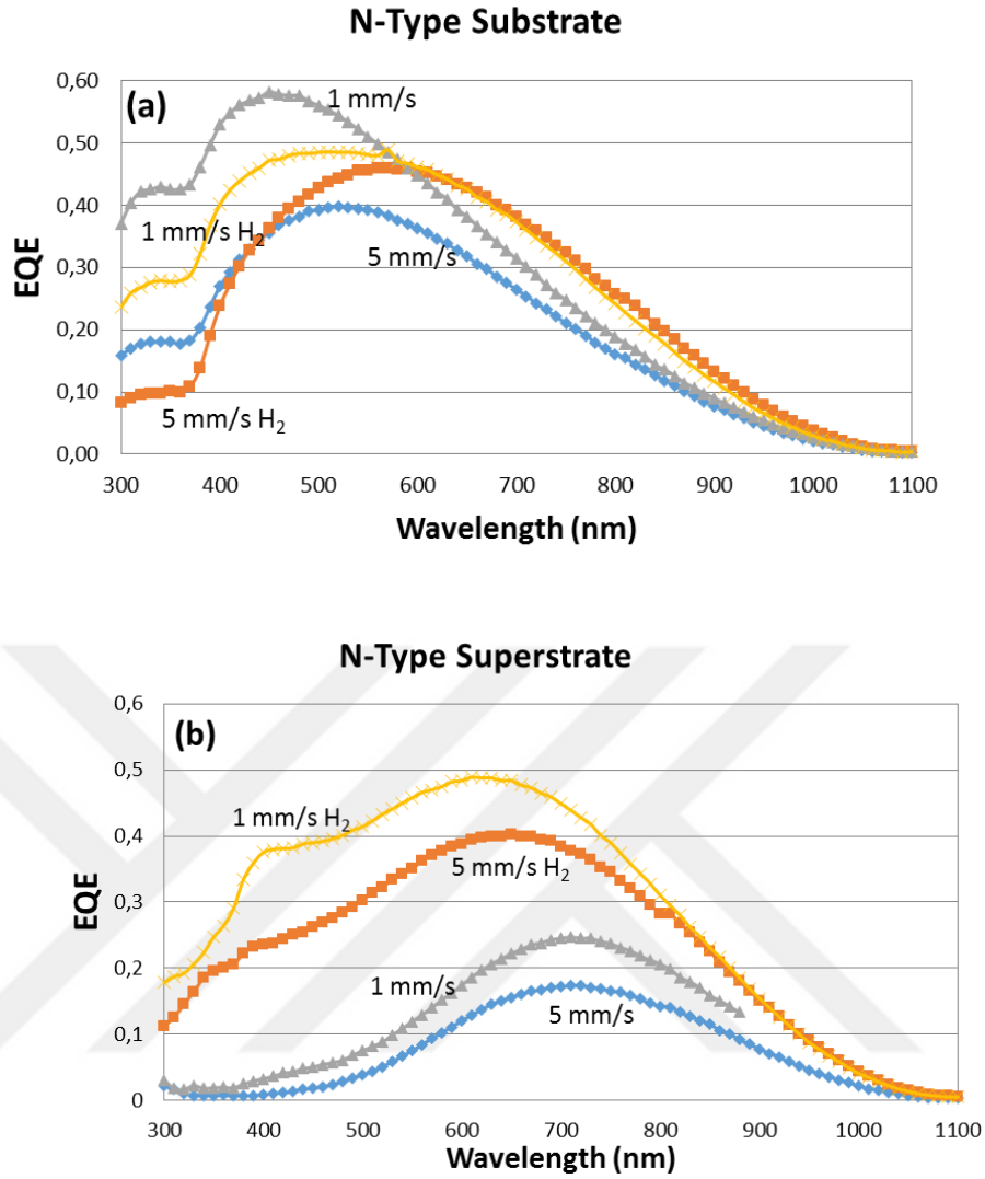
Figure 78: External Quantum Efficiency (EQE) measurement of n-type samples both in substrate (a) and superstrate (b) configurations
