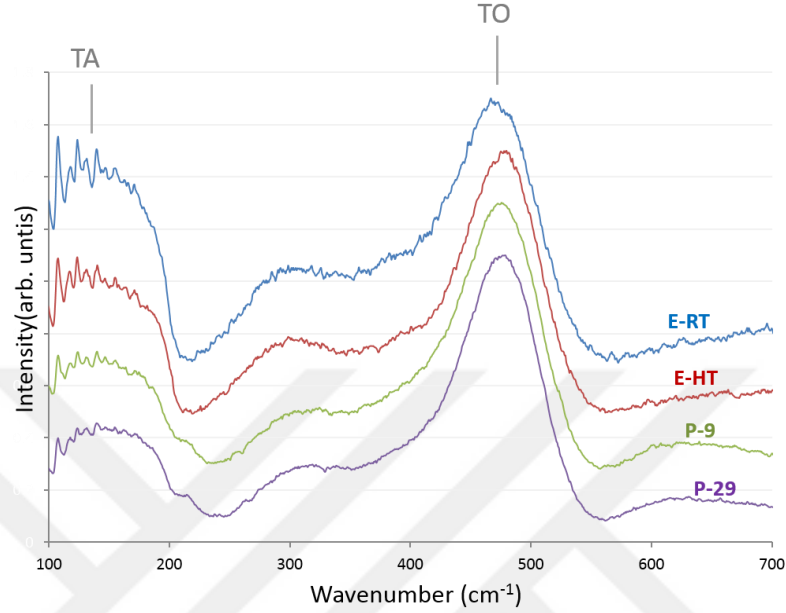
Figure 61: Normalized Raman spectra taken from the as-deposited a-Si films from batches E-RT, E-HT, P-9 and P-29. Spectra are stacked on the same graph (with varying intensity off sets) for ease of comparison. Approximate positions of the transverse acoustic (TA) and transverse optical (TO) peaks are indicated on the graph.
