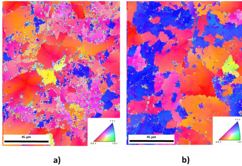
Figure 54: EBSD images taken from final poly-Si layers: (a) control sample and (b) pre-annealed sample. Grain colors correspond to crystal axes normal to the surface of poly-Si films as represented in the color codes given in the lower right inset.
