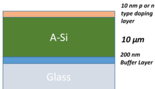
Figure 66: a-Si:H and doping layer depositions
