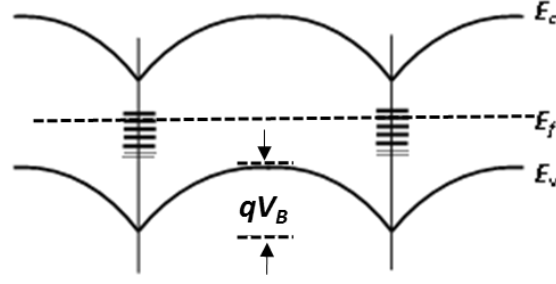
Figure 6: Grain boundary modelling of polycrystalline silicon with high dopant concentration
