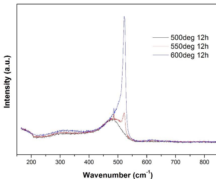
Figure 12: Raman measurements of samples annealed for 12 h at 500 °C, 550 °C and 600 °C.
