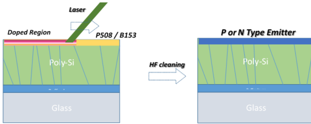
Figure 69: Laser doping process of P508 and B153 spin-on dopants.
