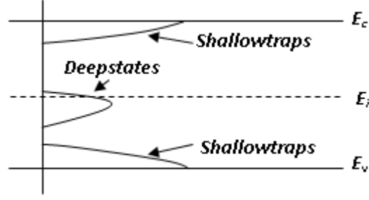
Figure 4: The effect of dangling bonds and defects
