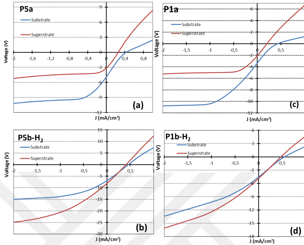
Figure 74: Solar simulator results of the selected cells on p-type samples 5 mm/s doped (a), (b) and 1 mm/s doped (c), (d)
