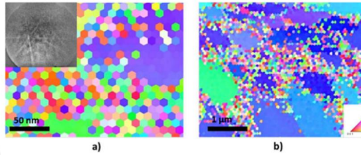
Figure 53: EBSD images taken from Al layers: (a) control sample (inset showing the Kikuchi pattern) and (b) pre-annealed sample.
