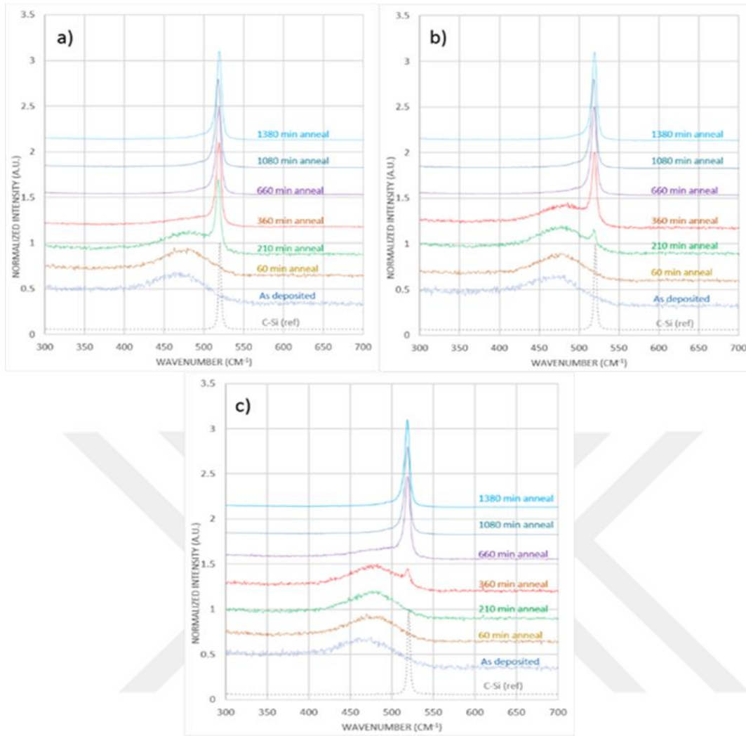
Figure 44: Raman spectroscopy taken from absorber layers before and after 600°C SPE annealing steps; grown on AIC seed layers annealed at: a) 450°C, b) 500°C, and c) 525°C.
