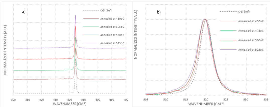
Figure 38: Raman spectroscopy taken from fully crystallized samples annealed at varying temperatures: a) wide wavenumber range, b) near c-Si peak (background subtracted).
