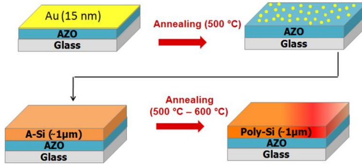
Figure 11: Fabrication process of Au induced a-Si crystallization
