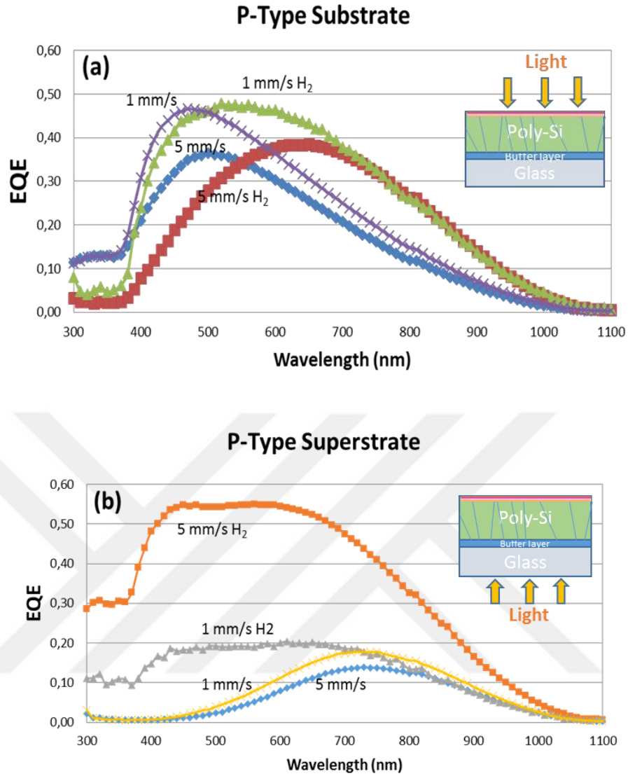
Figure 77: External Quantum Efficiency (EQE) measurement of p-type samples both in substrate (a) and superstrate (b) configurations
