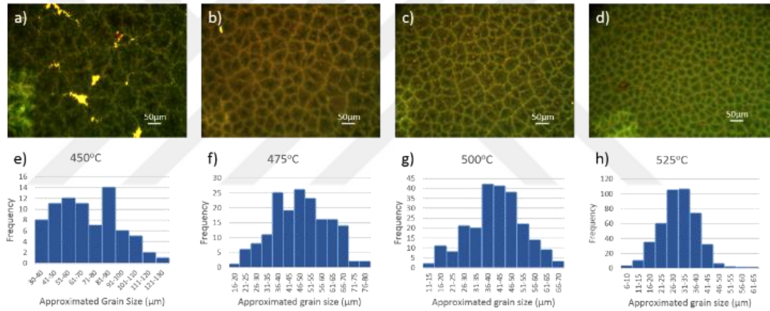
Figure 35: Effect of annealing temperature on poly-Si grain size: optical micrographs taken from fully crystallized samples annealed between 450 and 525°C (a through d), distribution of approximated grain size for fully crystallized samples annealed between 450 and 525 °C (e through h)
