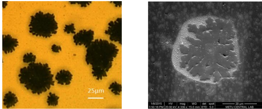
Figure 27: Micrographs taken from a-Si/Al/SiN x /glass sample annealed at 475°C for 2.5 h showing the formation of depletion regions, a) optical micrograph of large grains shown, a depletion region around them where no nuclei formation is present can be seen; b) scanning electron micrograph of a crystalline Si cluster where the sample was polished partially to expose the Si particle yet leave some of the surrounding Al-Si matrix. A high contrast region surrounding the Si grain is visible, indicating the Si-free (depletion) region
