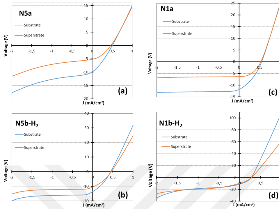
Figure 75: Solar sim results of the selected cells on n-type samples 5 mm/s doped (a), (b) and 1 mm/s doped (c), (d)
