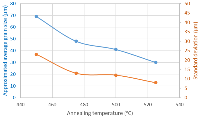
Figure 36: Annealing temperature vs. approximated average grain size and standard deviation. The referred grains do not necessarily represent a single crystal.
