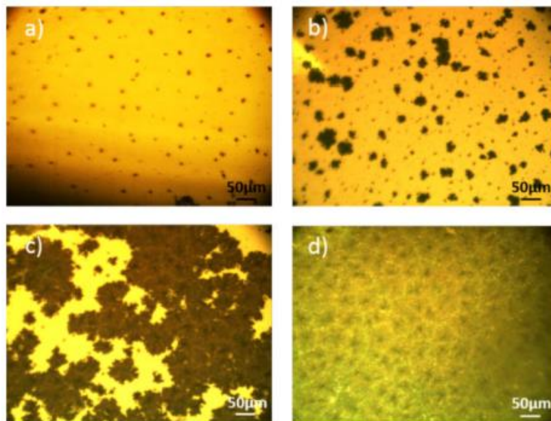
Figure 50: Optical micrographs taken from pre-annealed samples annealed at 420 °C for varying durations: (a) 220, (b) 420, (c) 1080, and (d) 1200 min.
