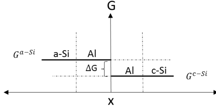
Figure 16: Schematic of Gibbs free energies of a-Si/Al and c-Si/Al systems [83]
