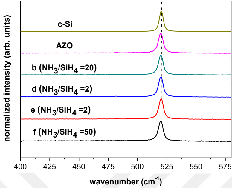
Figure 22: The Raman analysis of reference c-Si and poly-Si films produced by AIC technique on different SiN x and AZO coated glass
