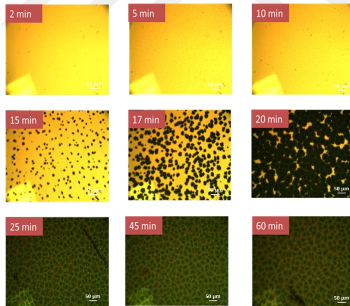
Figure 31: Optical micrographs taken from samples annealed at 525°C at varying annealing times (given in the upper left corner inset for each micrograph).
