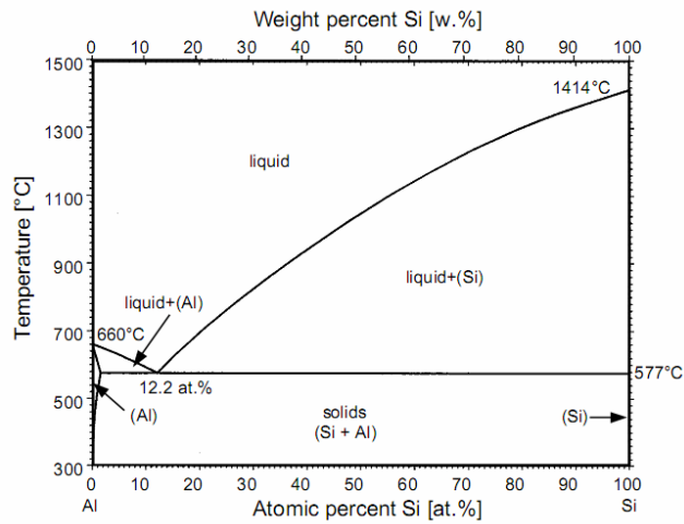
Figure 15: Al-Si equilibrium phase diagram [92]
