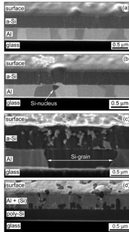
Figure 17: FIB images of ALILE process. (a) before annealing, (b) after annealing at 500°C for 5min, (c) annealing at 500°C 10min annealing; (d) 60min annealing at 500°C as a result of glass/poly-Si/Al+Si [83].
