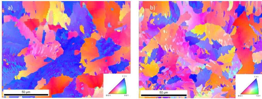
Figure 37: EBSD images taken from fully crystallized samples annealed at a) 450°C and b) 525°C. The colors represents the orientation of grains according to the color code given in the lower right corner inset.
