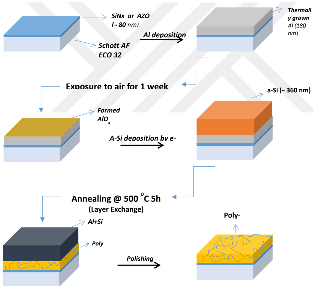
Figure 21: AIC poly-Si formation steps on SiN x or AZO buffer layer
