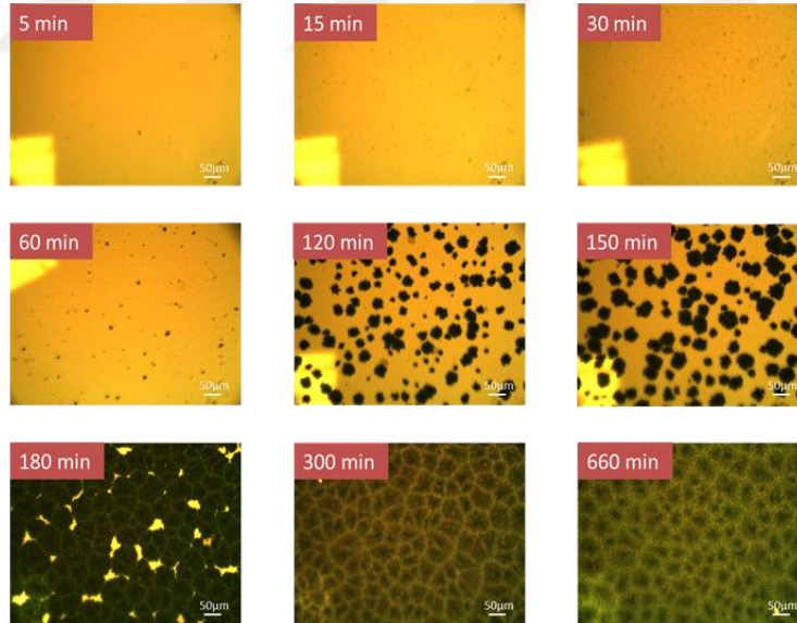
Figure 29: Optical micrographs taken from samples annealed at 475°C at varying annealing times (given in the upper left corner inset for each micrograph).
