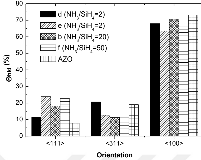
Figure 23: The calculated preferential orientation factor of poly-Si films by XRD measurements.
