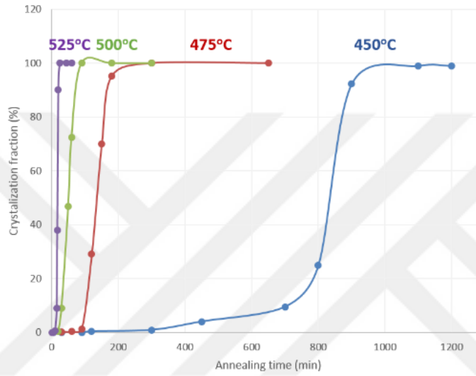
Figure 32: Percent crystallization vs annealing time curves for AIC experiments carried out at 450, 475, 500, and 525°C.
