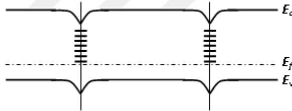
Figure 7: Modelling of polycrystalline silicon with completely filled trap states at the grain boundary
