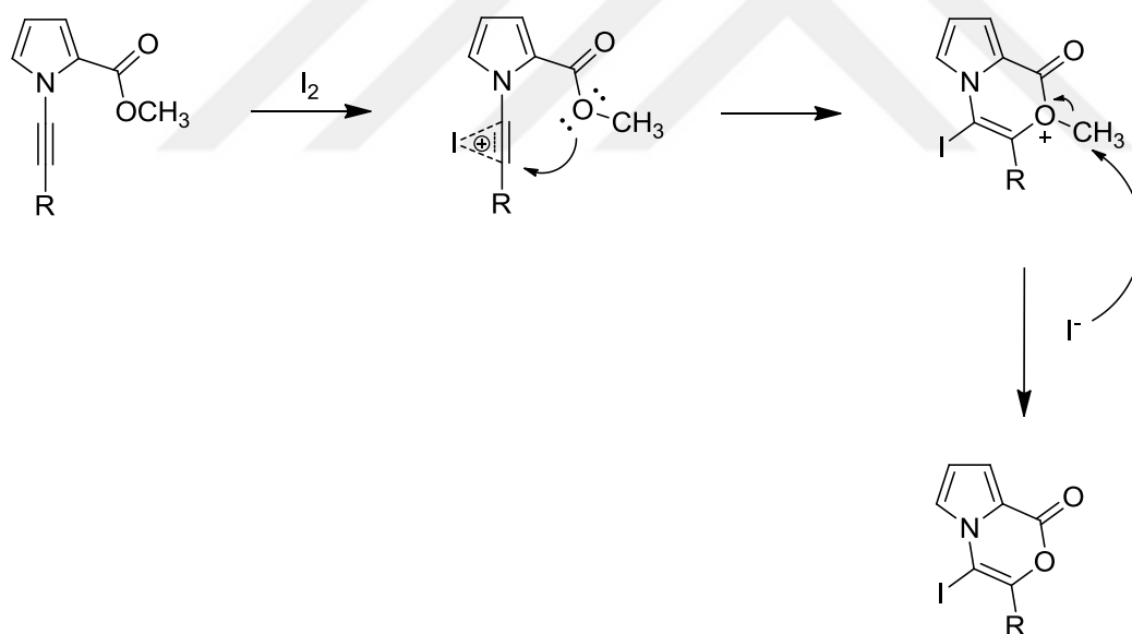
Scheme 29. Proposed reaction mechanism of electrophilic cyclization reaction
