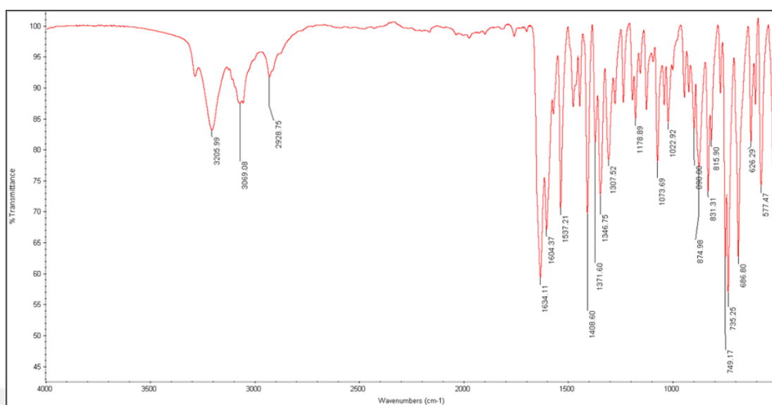
Figure 58 IR Spectrum of Compound 80
