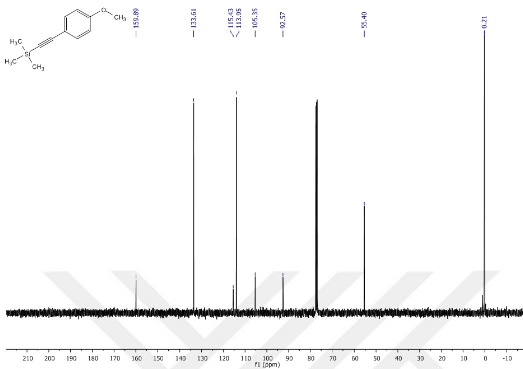
Figure 20 13 C-NMR Spectrum of Compound 62 in CDCl 3
