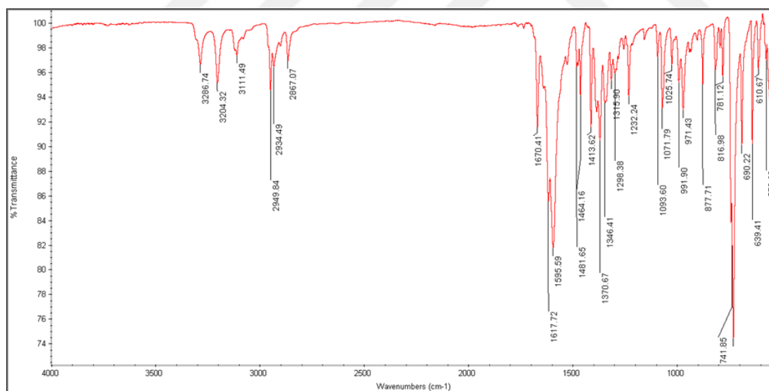
Figure 61 IR Spectrum of Compound 81
