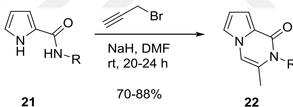
Scheme 3. Synthesis of pyrrolopyrazinone derivative 22
