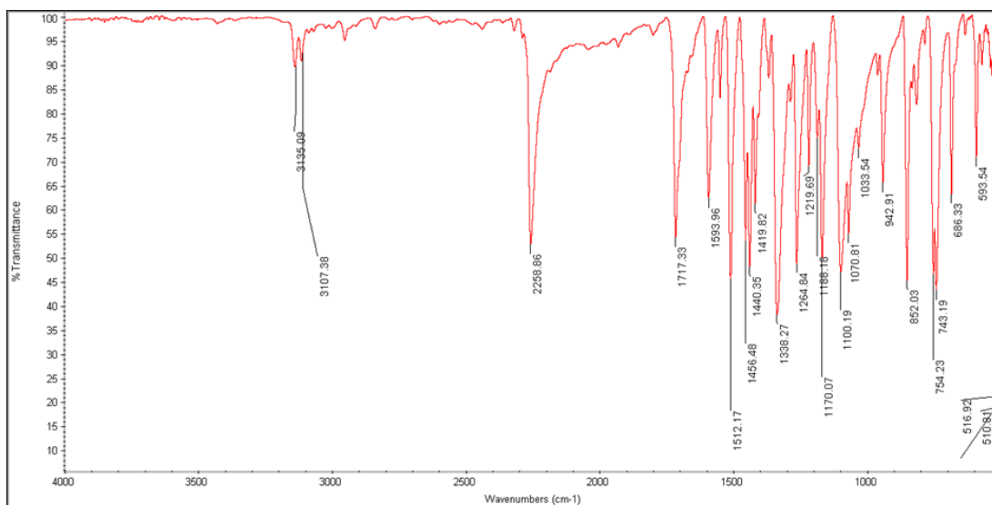
Figure 44 IR Spectrum of Compound 75
