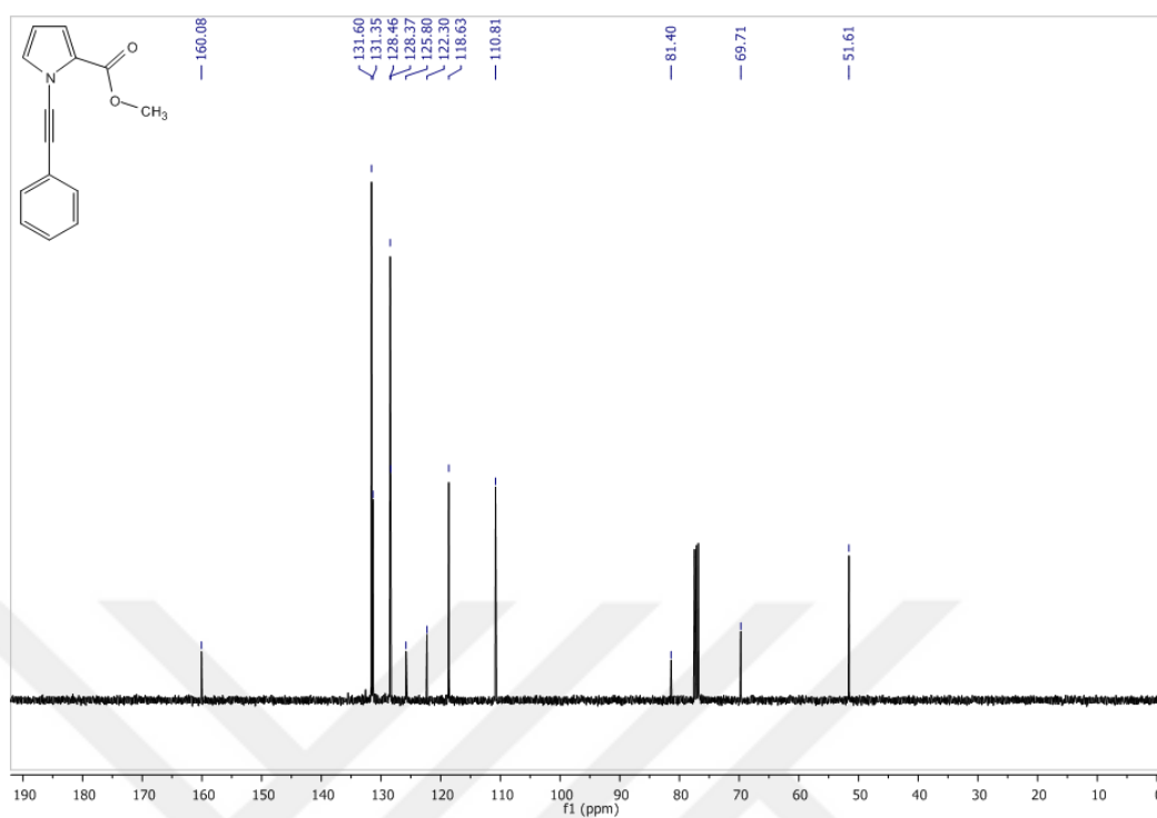
Figure 34 13 C-NMR Spectrum of Compound 72 in CDCl 3
