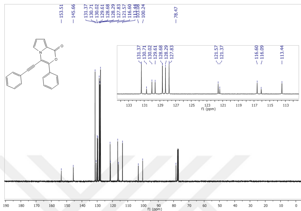
Figure 14 13 C-NMR spectrum of compound 93 in CDCl 3
