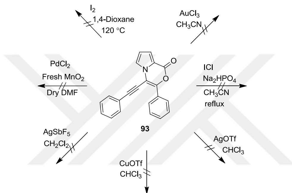
Scheme 32. Attempts to cyclize compound 93
