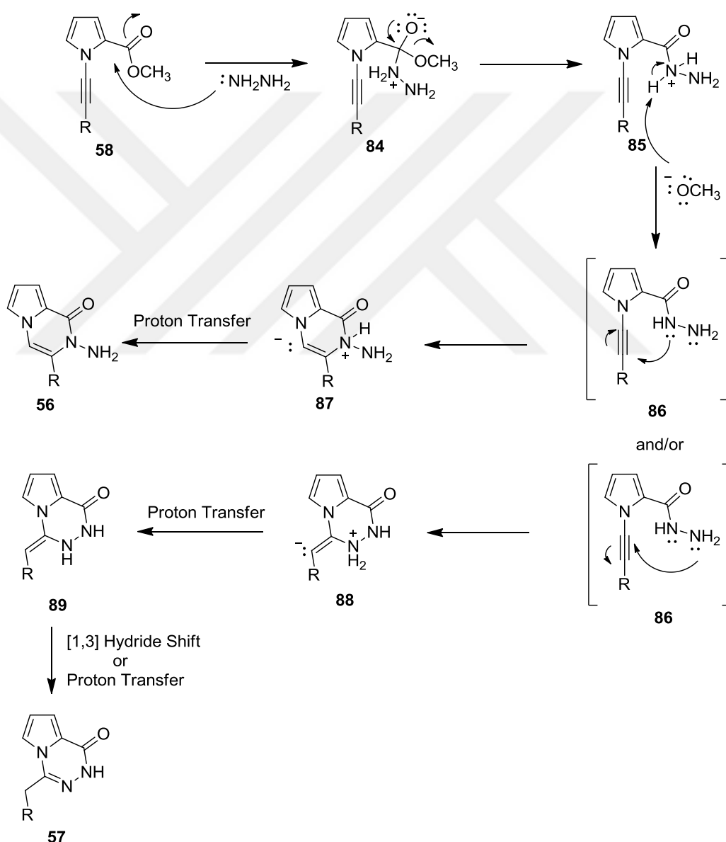
Scheme 27. Proposed reaction mechanism of nucleophilic cyclization reaction
