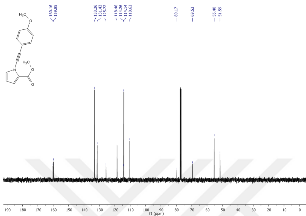
Figure 40 13 C-NMR Spectrum of Compound 74 in CDCl 3
