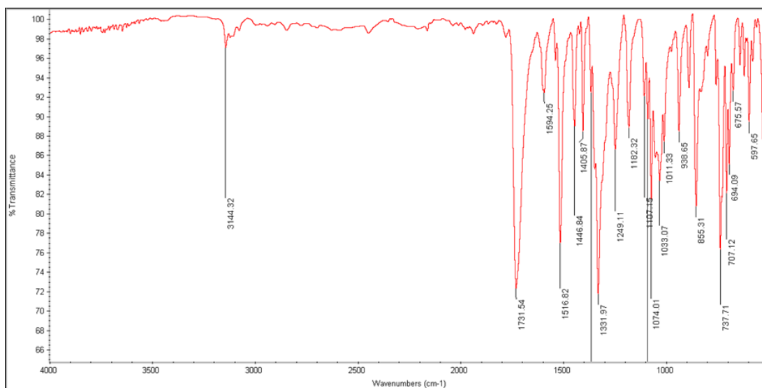
Figure 76 IR Spectrum of Compound 92
