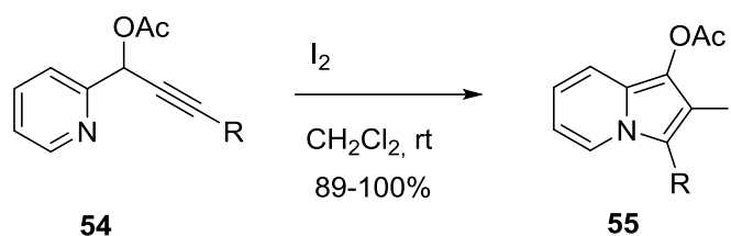
Scheme 11. Cyclization reaction of compound 54 via iodine
