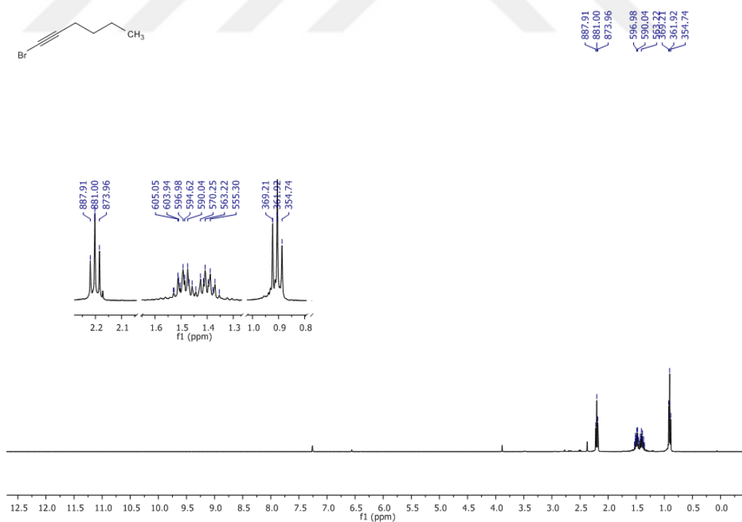
Figure 27 ^1\text{H} -NMR Spectrum of Compound 69 in \text{CDCl}_3
