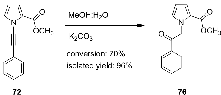
Scheme 23. Attempt to hydrolyze compound 72
