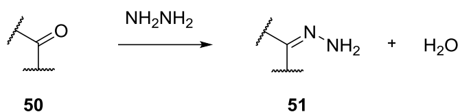
Scheme 8. Hydrazone formation of carbonyl groups
