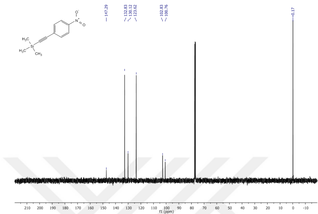
Figure 22 13 C-NMR Spectrum of Compound 64 in CDCl 3
