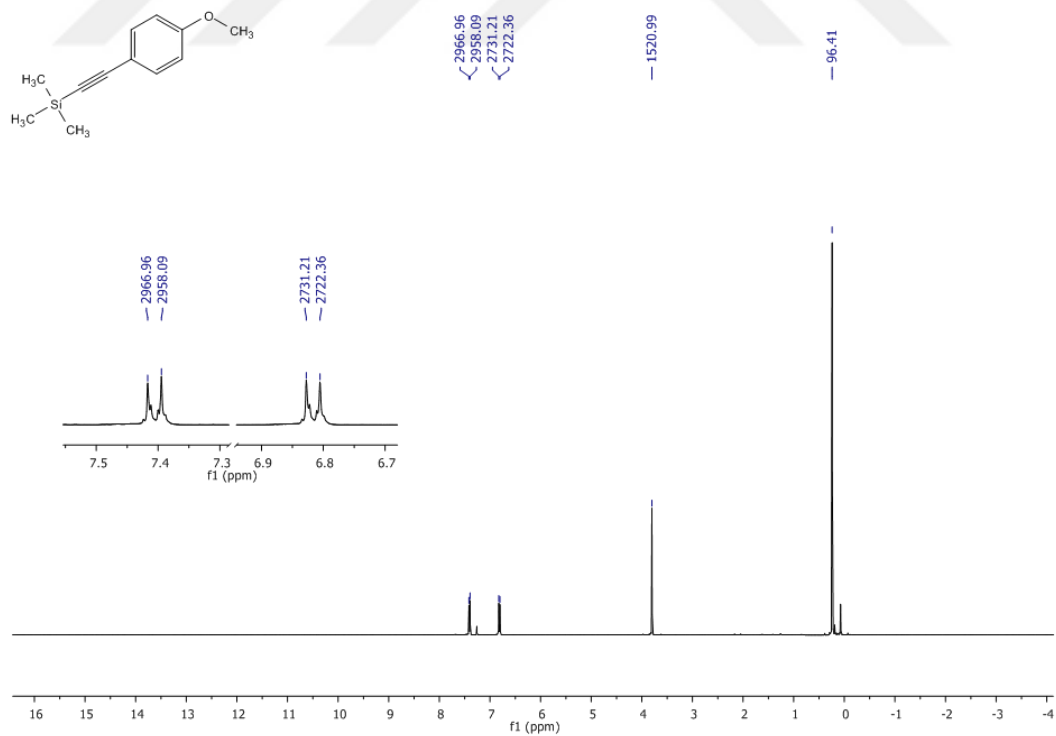
Figure 19 ^1\text{H} -NMR Spectrum of Compound 62 in \text{CDCl}_3
