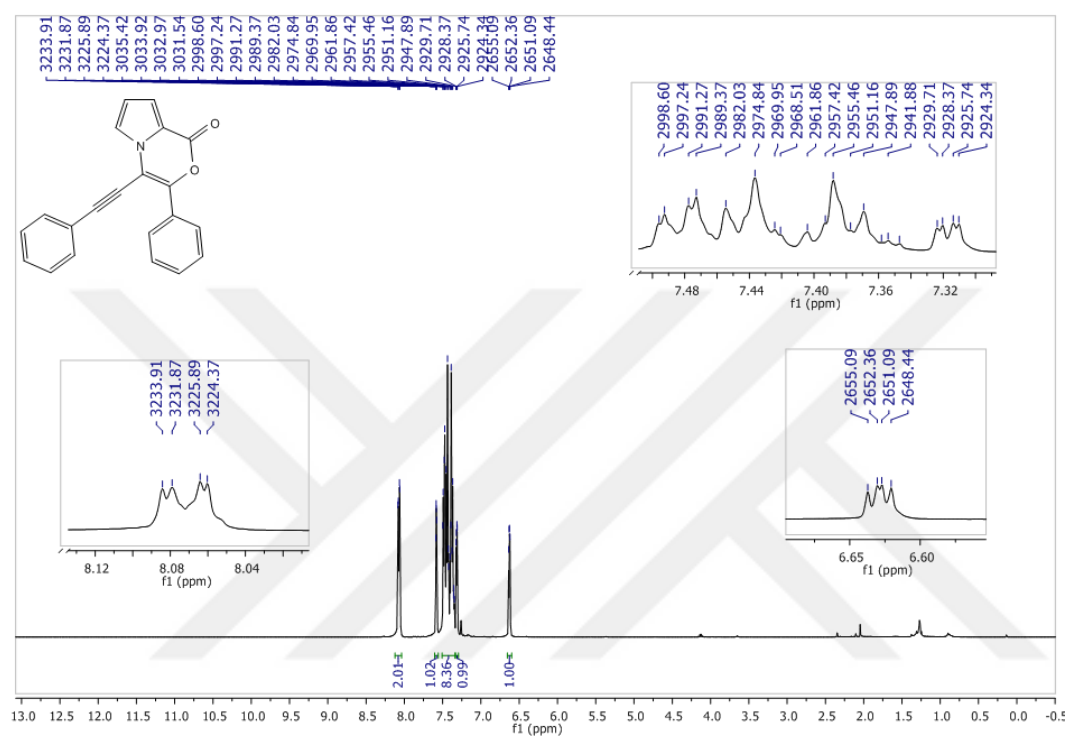
Figure 13 ^1\text{H} -NMR spectrum of compound 93 in CDCl 3
