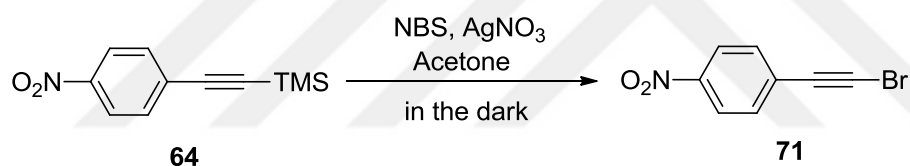
Scheme 20. Synthesis of 1-(bromoethynyl)-4-nitrobenzene ( 71 )
