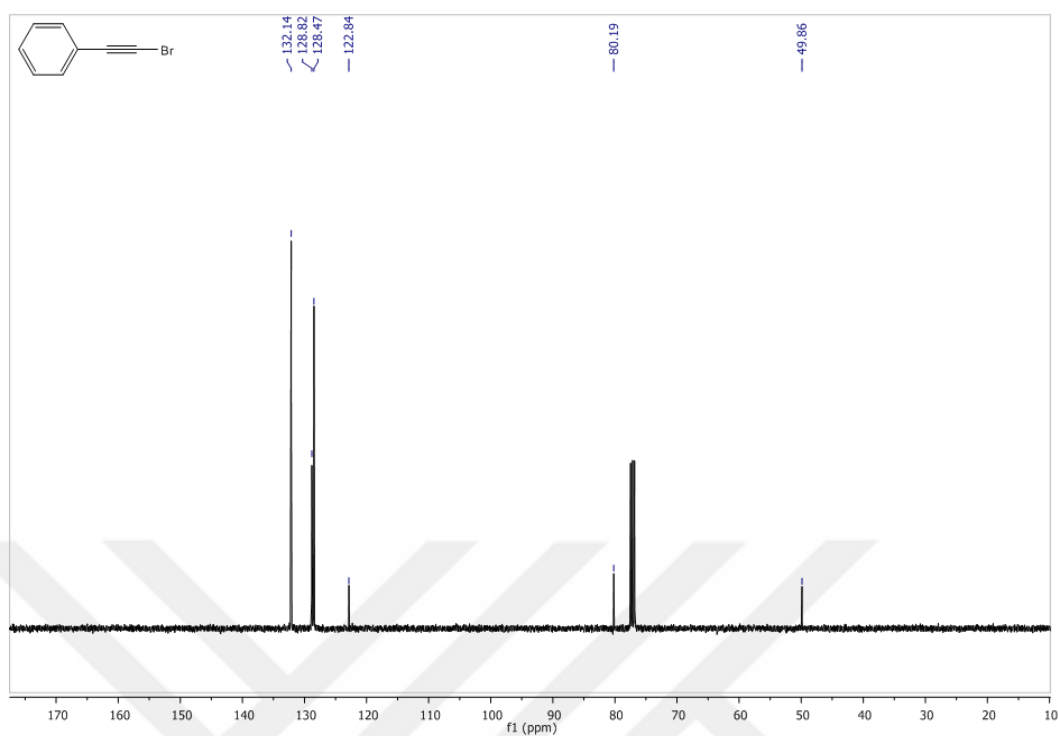
Figure 26 ^{13}\text{C} -NMR Spectrum of Compound 67 in \text{CDCl}_3
