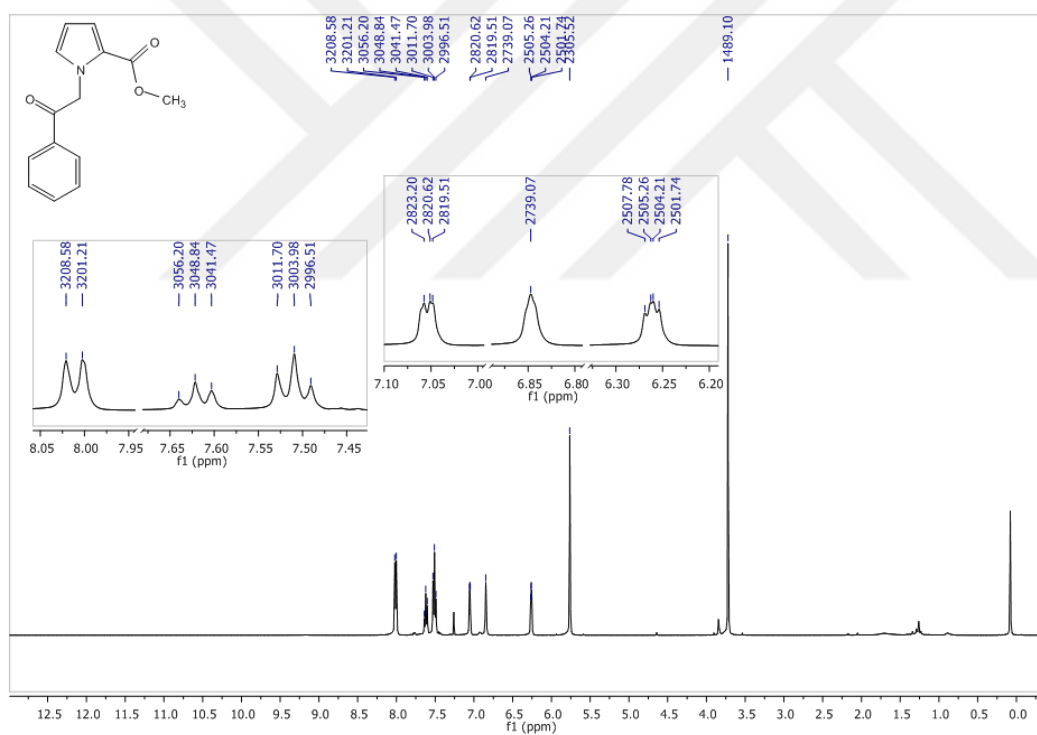
Figure 45 1 H-NMR Spectrum of Compound 76 in CDCl 3
