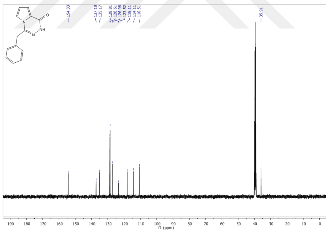
Figure 51 ^{13}\text{C} -NMR Spectrum of Compound 78 in DMSO- \text{d}_6
