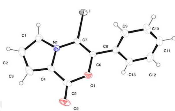
Figure 12 X-ray analysis of compound 90
