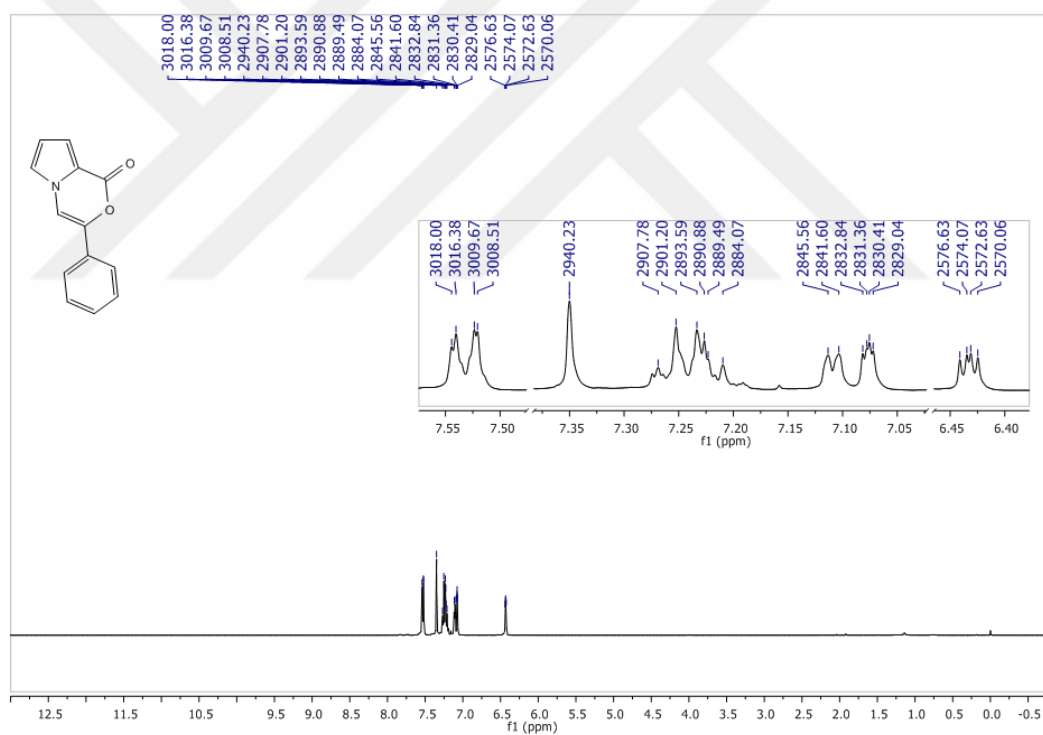
Figure 83 1 H-NMR Spectrum of Compound 95 in CDCl 3
