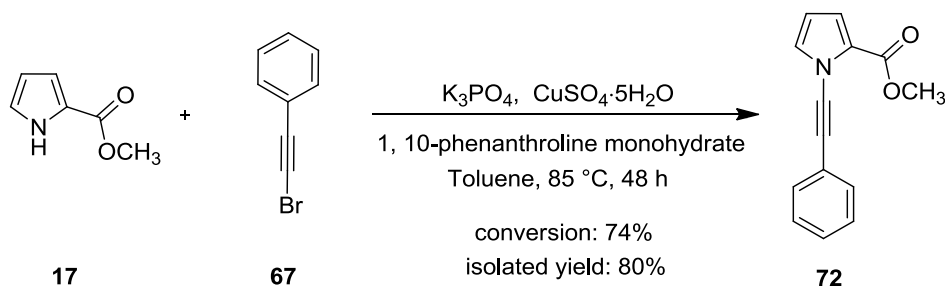
Scheme 22. Proper N -alkynylation reaction conditions
