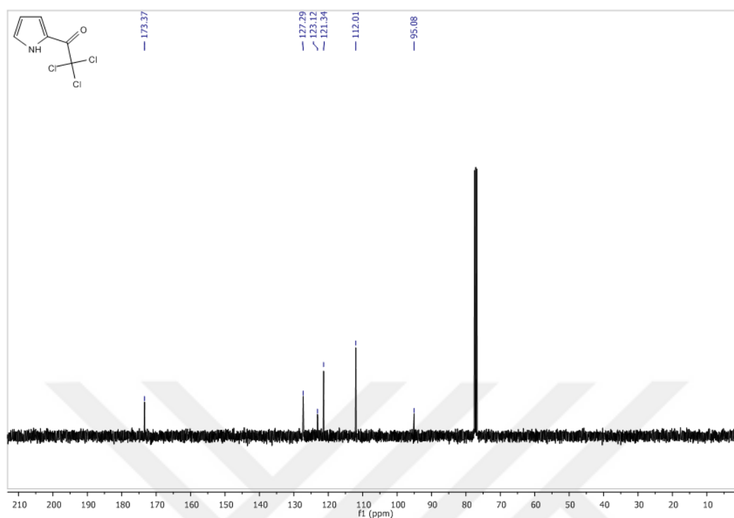
Figure 16 13 C-NMR Spectrum of Compound 60 in CDCl 3
