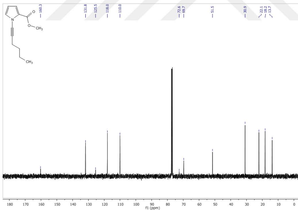
Figure 37 13 C-NMR Spectrum of Compound 73 in CDCl 3
