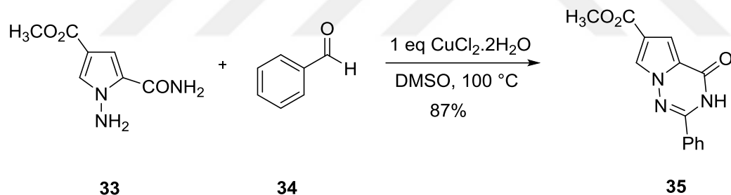
Scheme 5. Synthesis of pyrrolotriazinone derivative 35
