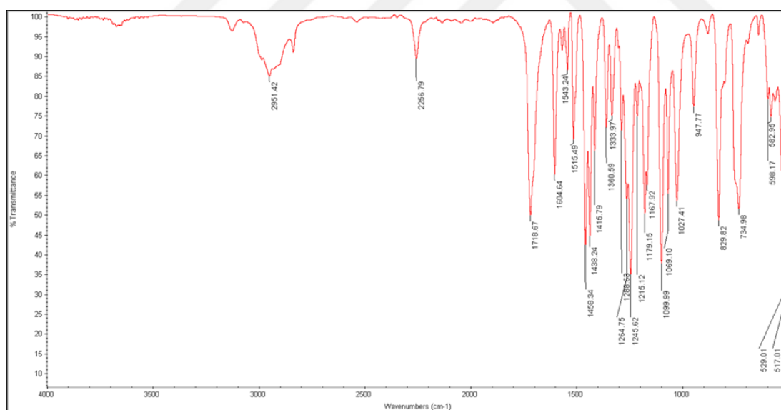
Figure 41 IR Spectrum of Compound 74
