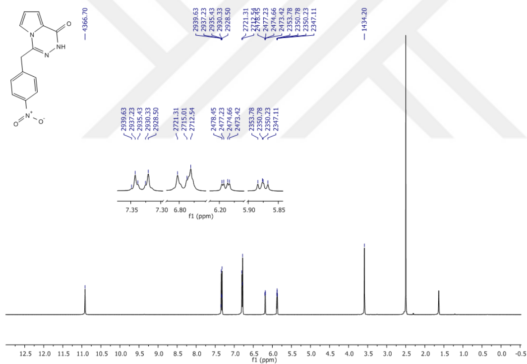
Figure 65 1 H-NMR Spectrum of Compound 83 in DMSO-d 6
