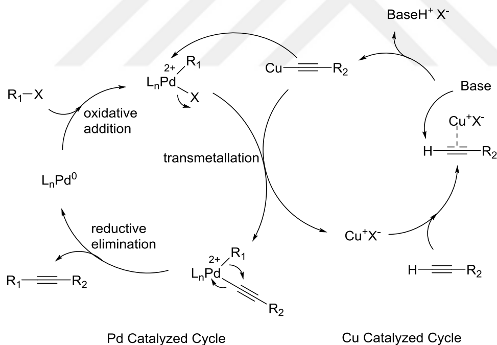
Scheme 16. Mechanism of Sonogashira coupling reaction
