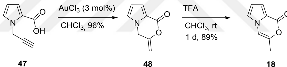
Scheme 7. Synthesis of pyrrolooxazinone derivative 18
