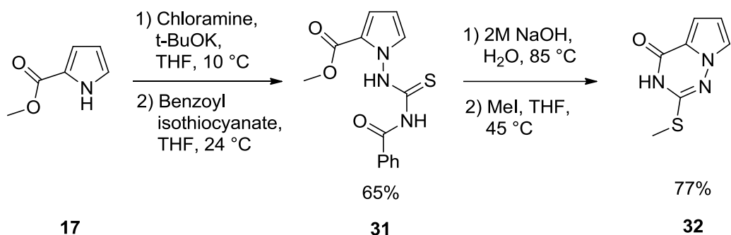
Scheme 4. Synthesis of pyrrolotriazinone derivative 32
