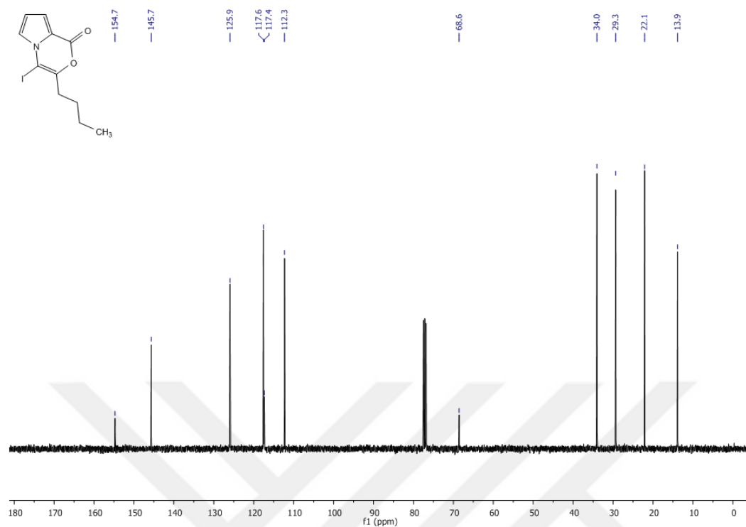
Figure 72 13 C-NMR Spectrum of Compound 91 in CDCl 3
