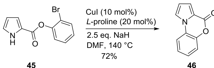
Scheme 6. Synthesis of pyrrolooxazinone derivative 46
