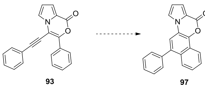
Scheme 31. The idea of further cyclization
