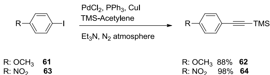
Scheme 17. Synthesis of arylalkyne derivatives 62 and 64
