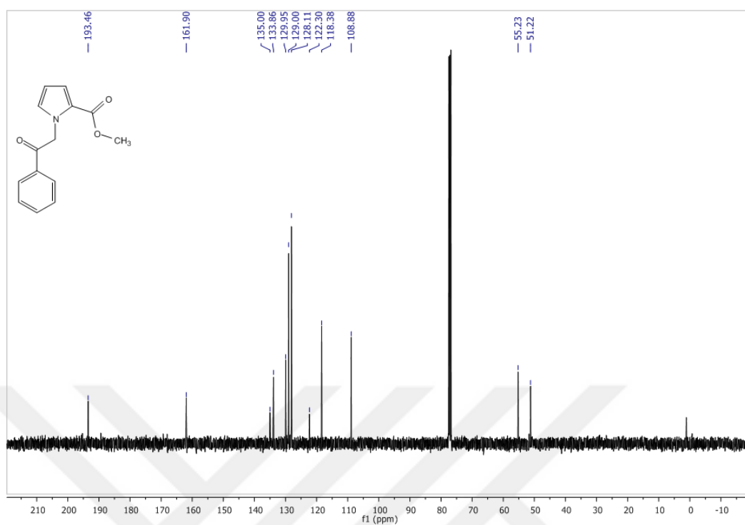
Figure 46 13 C-NMR Spectrum of Compound 76 in CDCl 3
