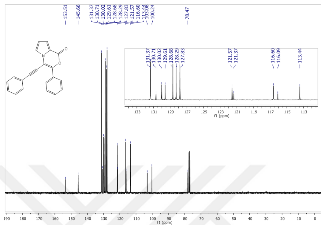
Figure 78 13 C-NMR Spectrum of Compound 93 in CDCl 3
