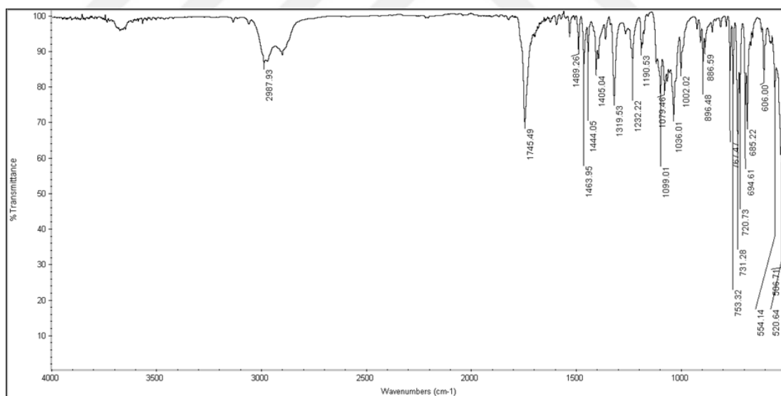
Figure 79 IR Spectrum of Compound 93
