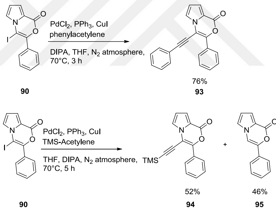
Scheme 30. Sonogashira coupling reactions of 4-iodo-3-phenyl-1 H -pyrrolo[2,1- c ][1,4]oxazin-1-one ( 90 )
