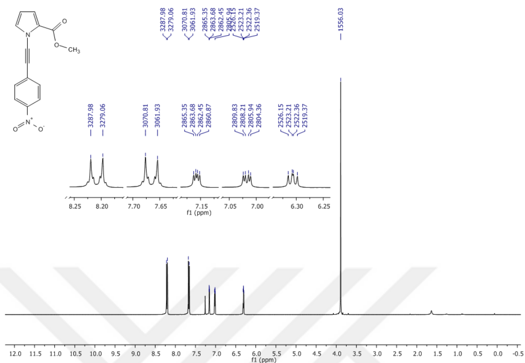
Figure 42 1 H-NMR Spectrum of Compound 75 in CDCl 3
