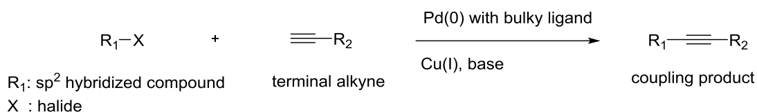
Scheme 15. Sonogashira coupling reaction
