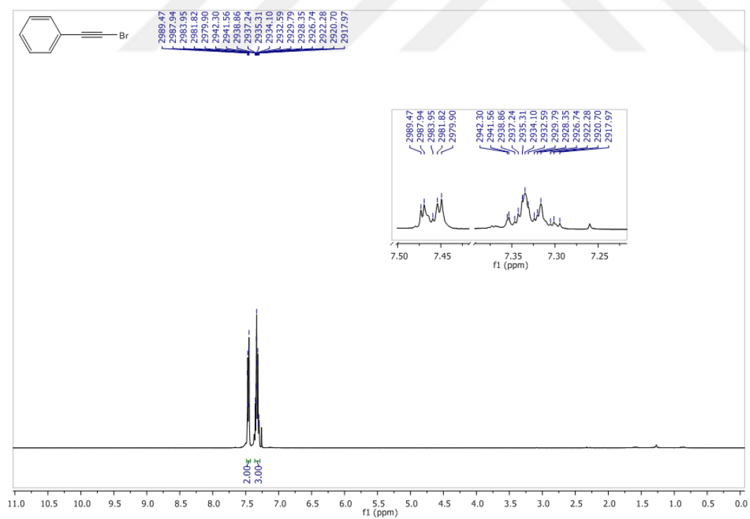
Figure 25 1 H-NMR Spectrum of Compound 67 in CDCl 3
