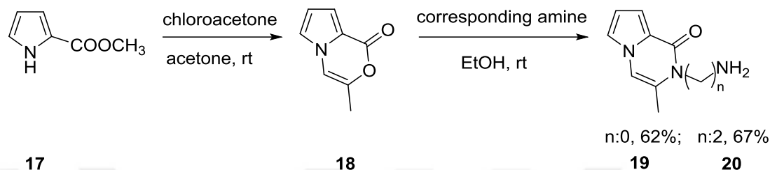
Scheme 2. Synthesis of pyrrolopyrazinone derivatives 19 and 20
