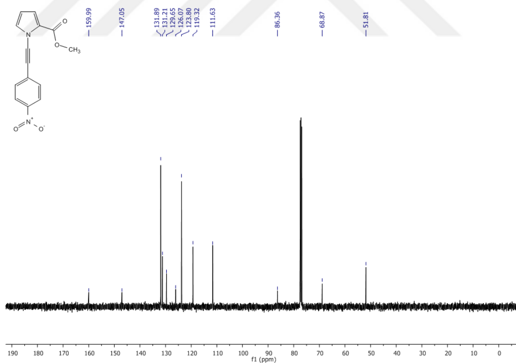
Figure 43 13 C-NMR Spectrum of Compound 75 in CDCl 3
