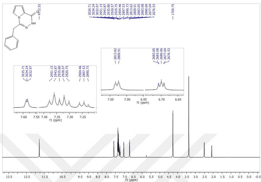
Figure 50 ^1\text{H} -NMR Spectrum of Compound 78 in DMSO- \text{d}_6
