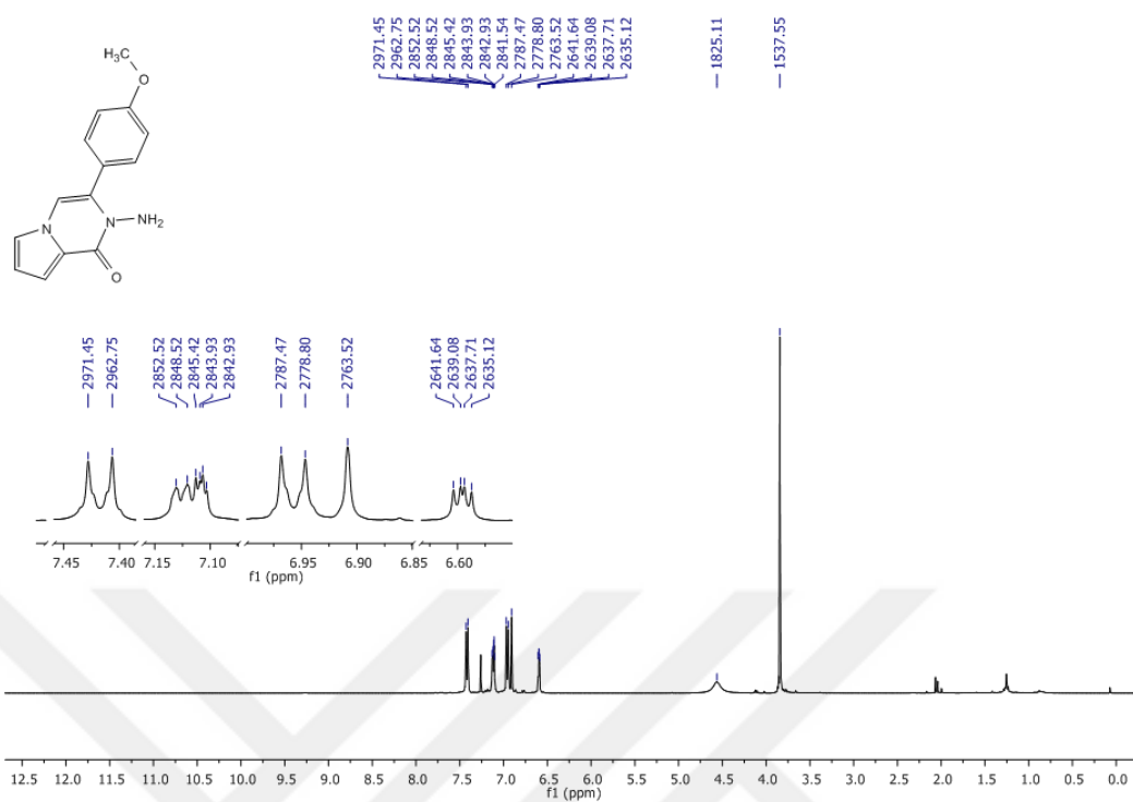
Figure 62 1 H-NMR Spectrum of Compound 82 in CDCl 3
