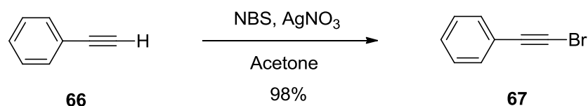
Scheme 19. Synthesis of (bromoethynyl)benzene ( 67 )
