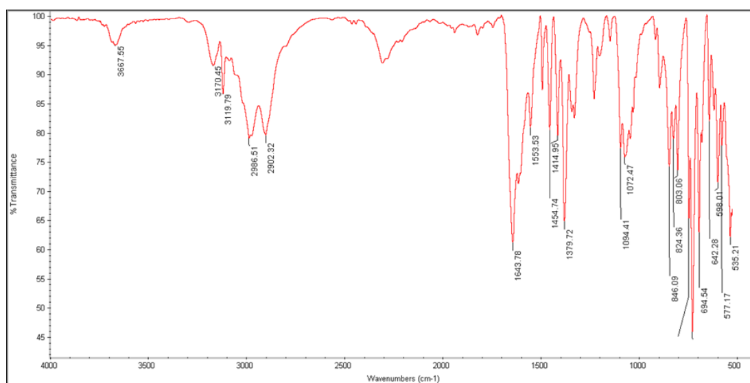
Figure 52 IR Spectrum of Compound 78
