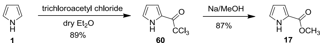
Scheme 14. Synthesis of methyl 1 H -pyrrole-2-carboxylate ( 17 )
