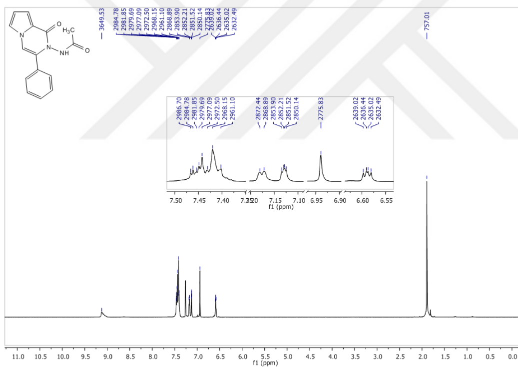
Figure 53 1 H-NMR Spectrum of Compound 79 in CDCl 3
