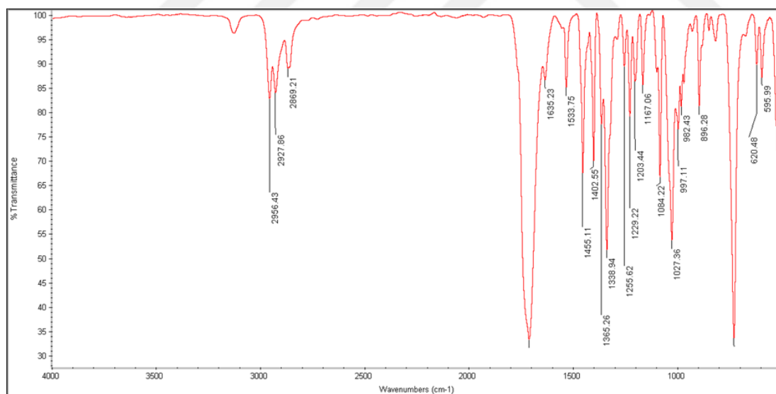
Figure 73 IR Spectrum of Compound 91
