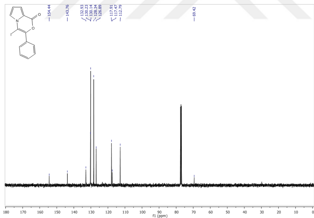
Figure 69 13 C NMR Spectrum of Compound 90 in CDCl 3
