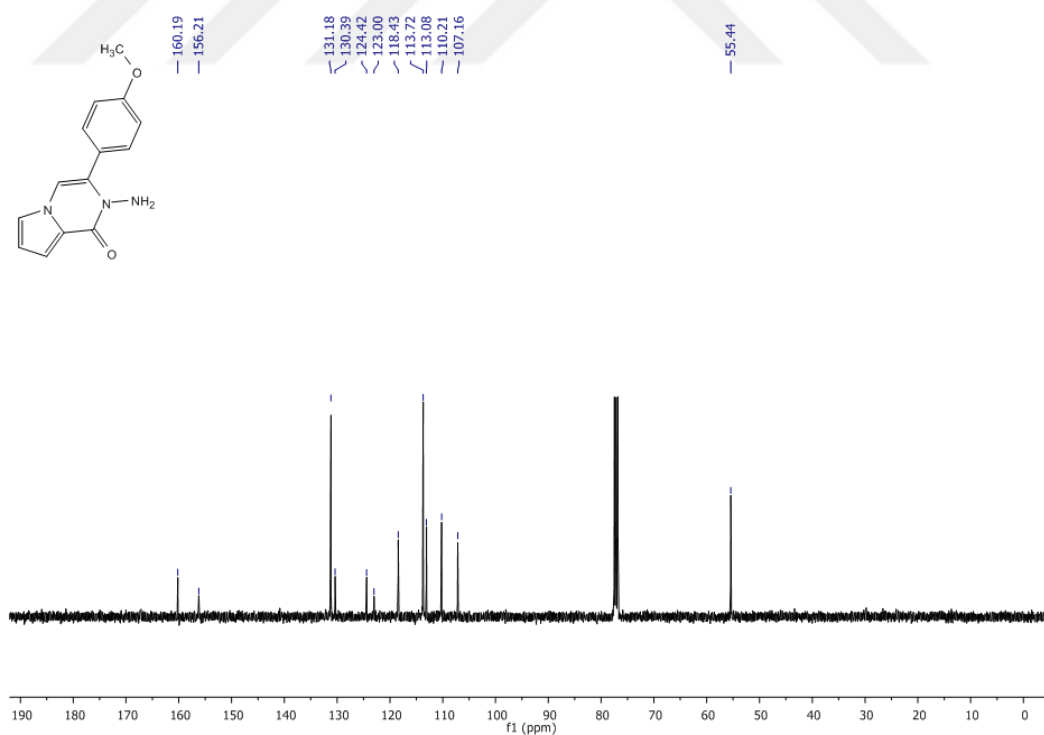
Figure 63 13 C-NMR Spectrum of Compound 82 in CDCl 3
