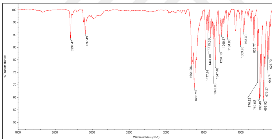
Figure 49 IR Spectrum of Compound 77
