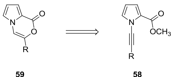
Scheme 13. Pathway to synthesis pyrrolooxazinone skeleton
