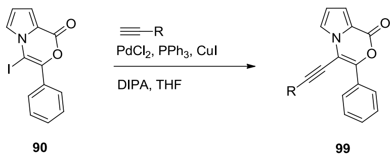
Scheme 35. Further functionalizations of compound 90
