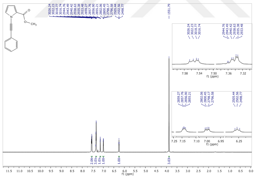
Figure 33 1 H-NMR Spectrum of Compound 72 in CDCl 3
