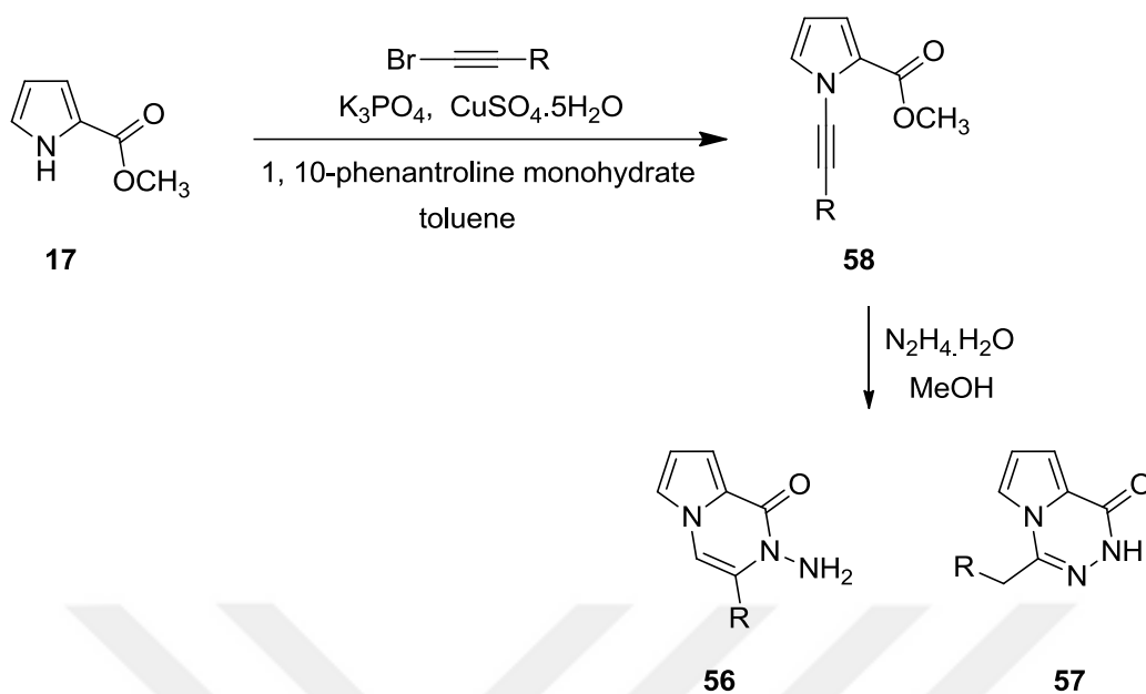
Scheme 33. Nucleophilic cyclization reaction via hydrazine monohydrate
