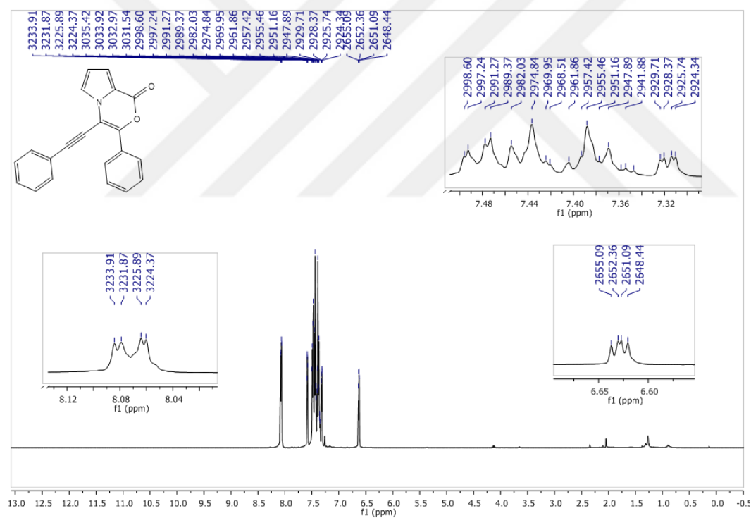
Figure 77 1 H-NMR Spectrum of Compound 93 in CDCl 3
