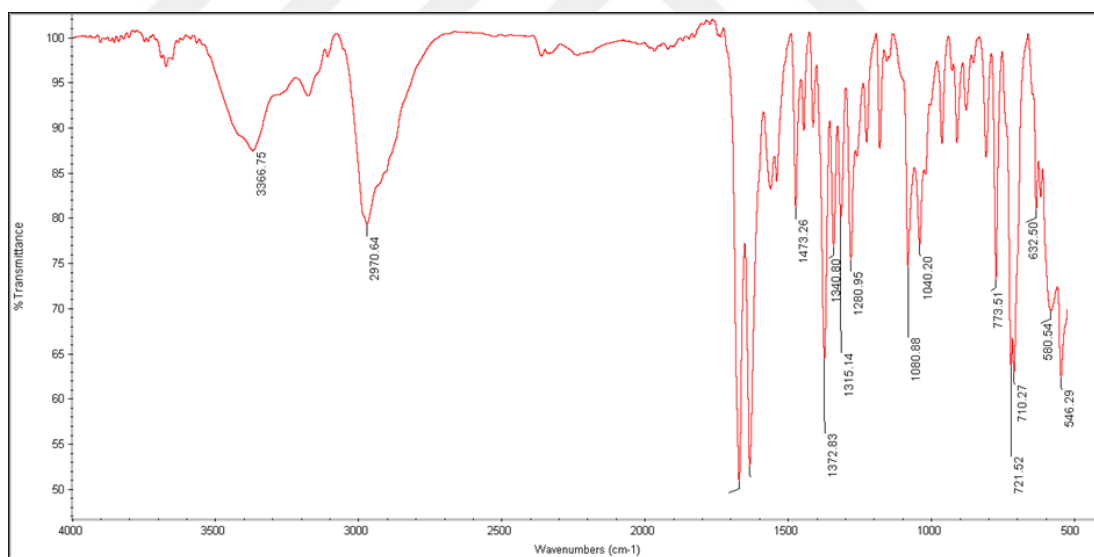
Figure 55 IR Spectrum of Compound 79
