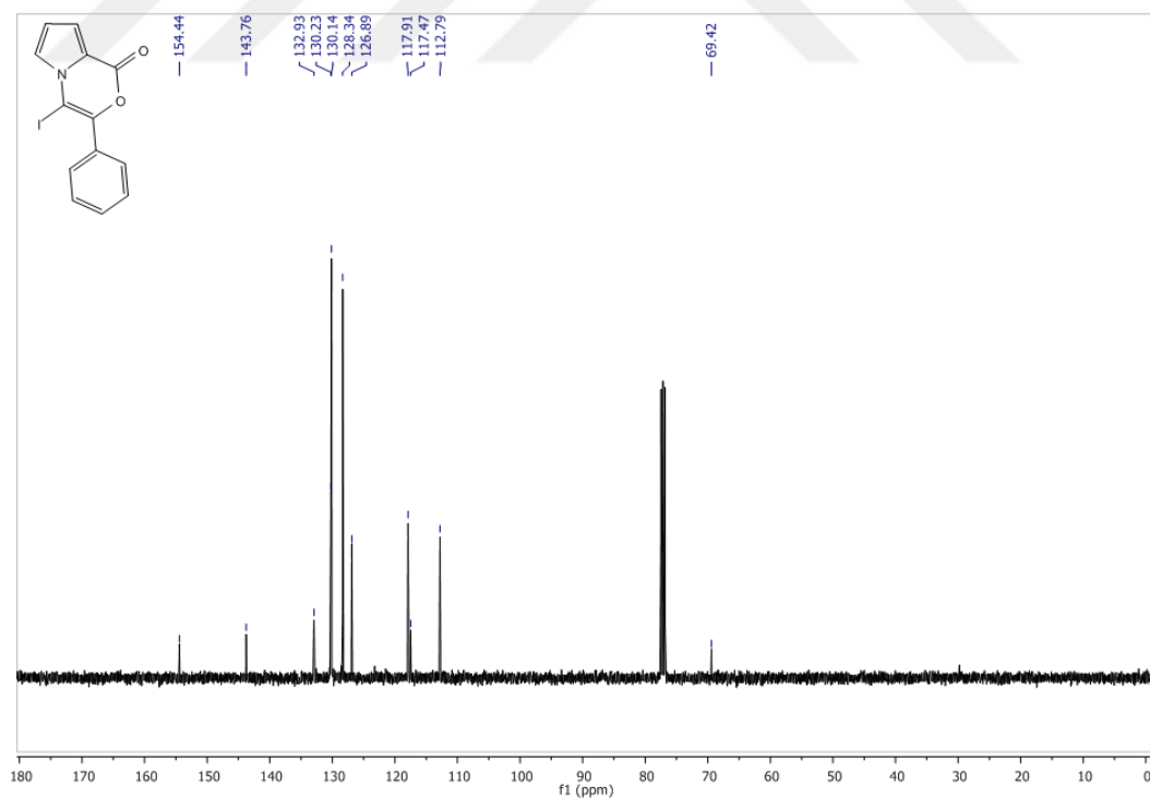
Figure 11 13 C-NMR spectrum of compound 90 in CDCl 3
