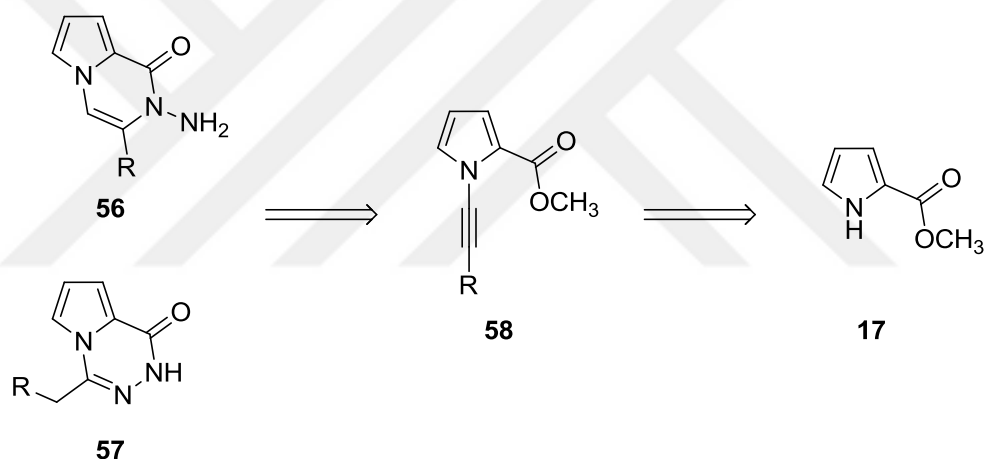
Scheme 12. Pathway to synthesize pyrrolopyrazinone and triazinone skeletons
