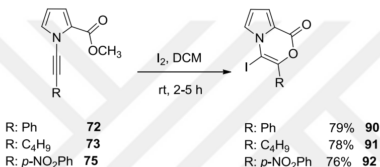
Scheme 28. Electrophilic cyclization reactions of key compounds 72 , 73 , 75
