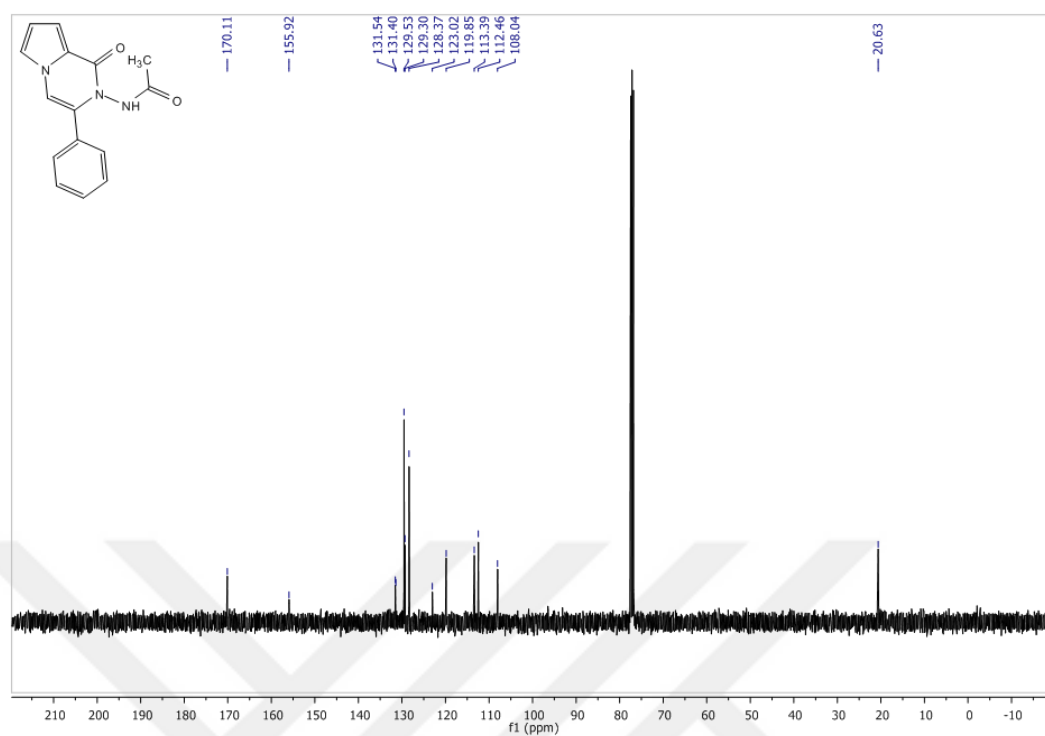
Figure 54 13 C-NMR Spectrum of Compound 79 in CDCl 3
