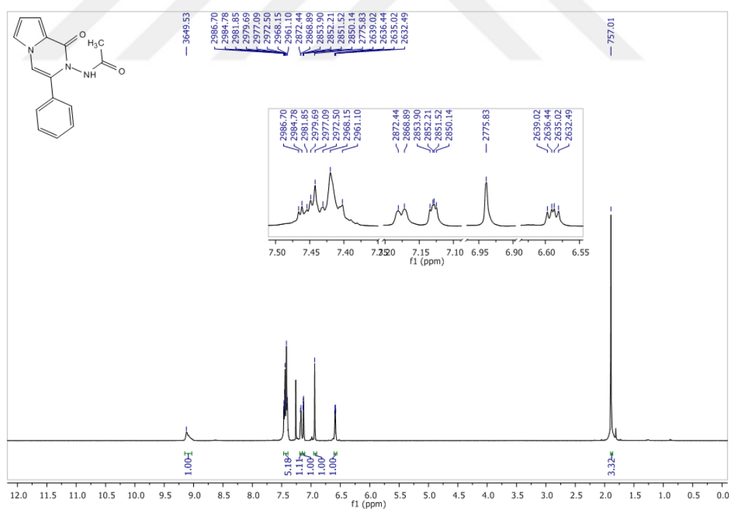
Figure 5 1 H-NMR spectrum of compound 79 in CDCl 3
