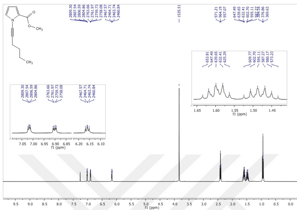
Figure 36 1 H-NMR Spectrum of Compound 73 in CDCl 3
