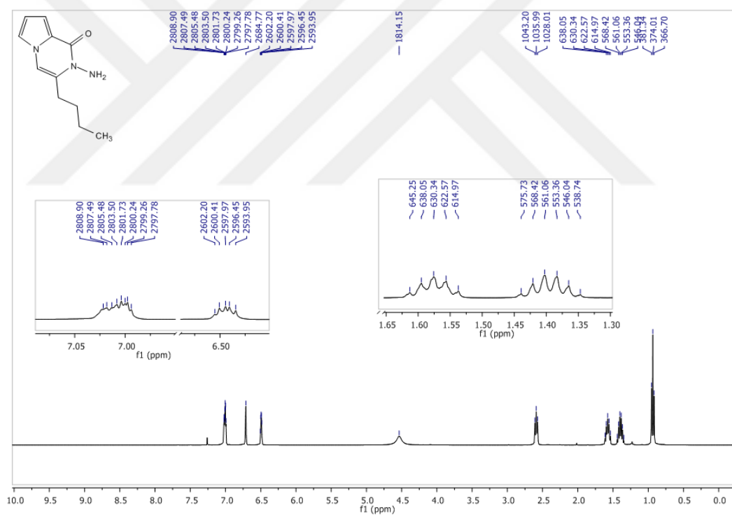
Figure 59 1 H-NMR Spectrum of Compound 81 in CDCl 3
