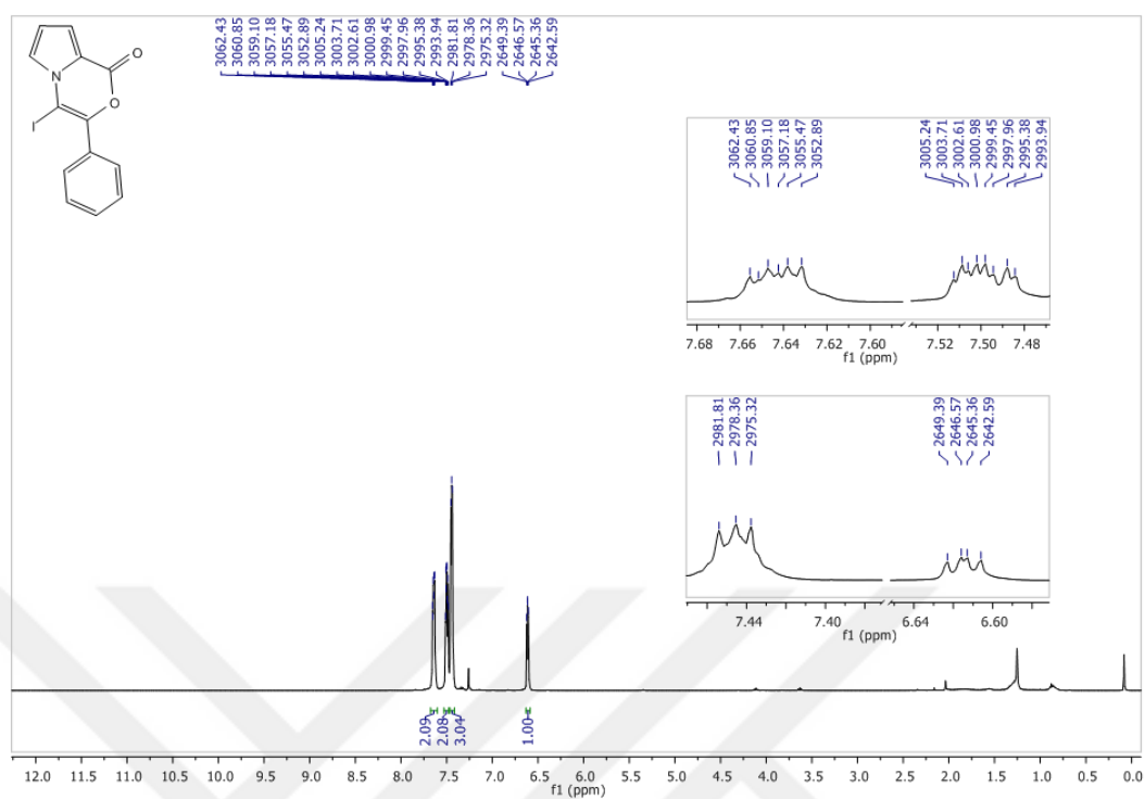
Figure 10 1 H-NMR spectrum of compound 90 in CDCl 3
