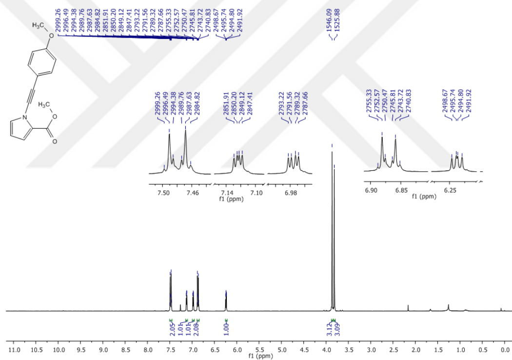
Figure 39 1 H-NMR Spectrum of Compound 74 in CDCl 3
