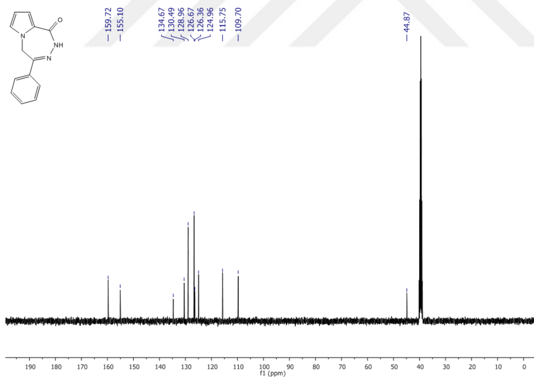
Figure 57 13 C-NMR Spectrum of Compound 80 in DMSO-d 6
