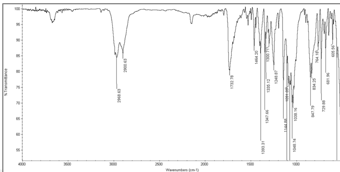
Figure 82 IR Spectrum of Compound 94
