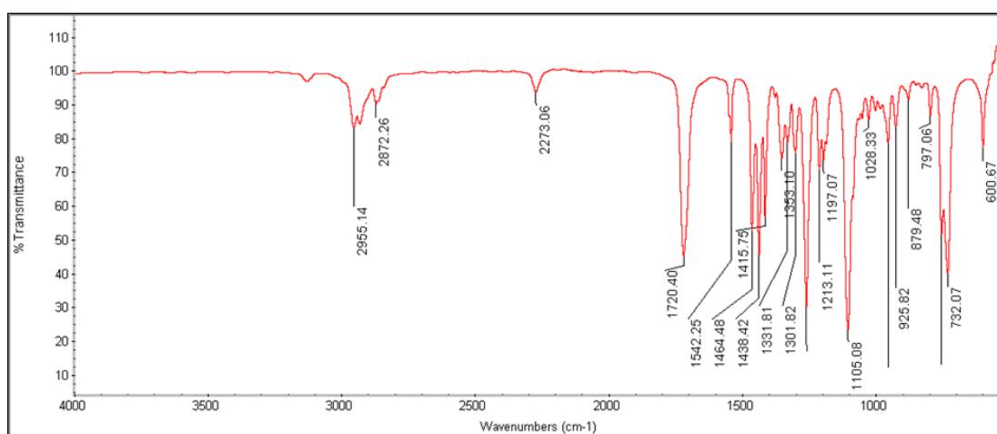
Figure 38 IR Spectrum of Compound 73
