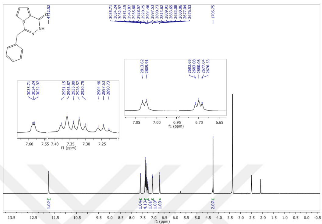
Figure 7 1 H-NMR spectrum of compound 78 in DMSO-d 6
