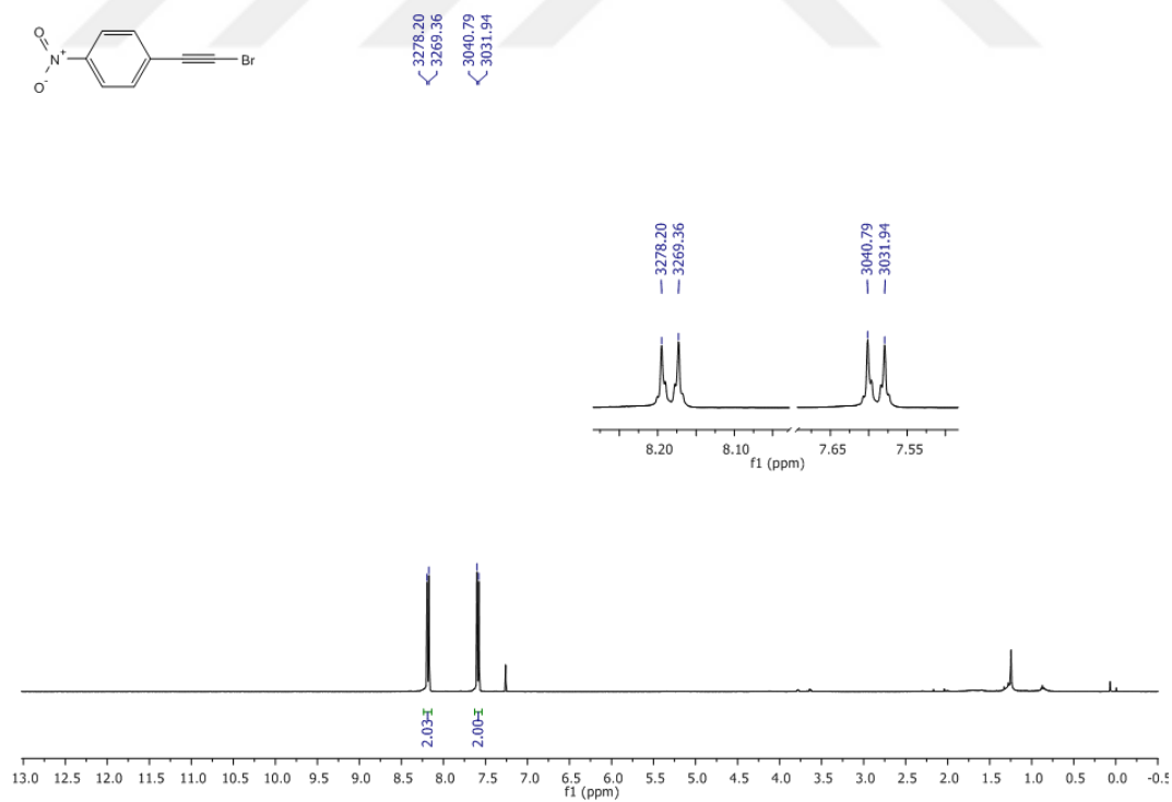
Figure 31 ^1\text{H} -NMR Spectrum of Compound 71 in \text{CDCl}_3
