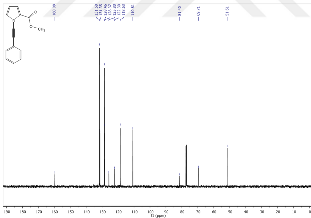
Figure 2 13 C-NMR spectrum of compound 72 in CDCl 3
