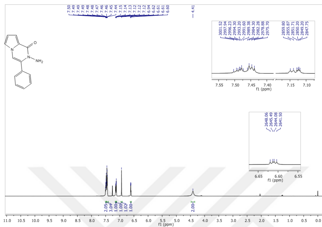
Figure 3 1 H-NMR spectrum of compound 77 in CDCl 3
