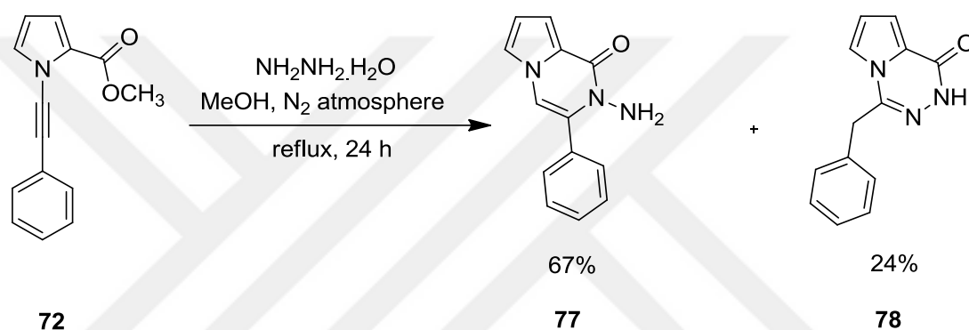
Scheme 24. Nucleophilic cyclization reaction of compound 72
