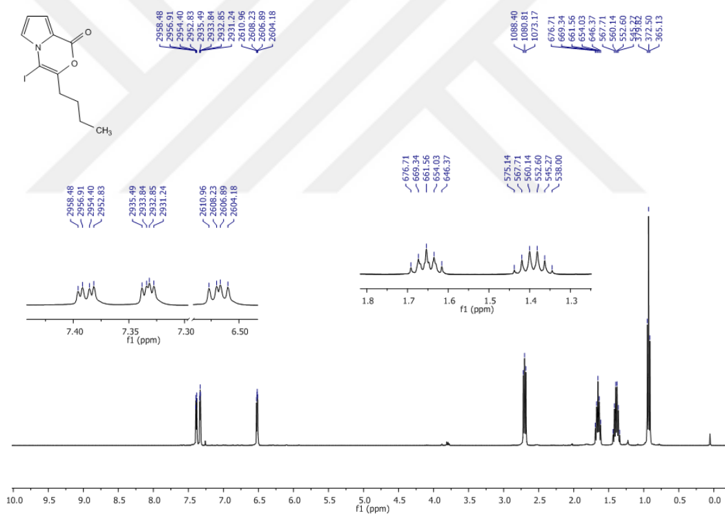
Figure 71 1 H-NMR Spectrum of Compound 91 in CDCl 3
