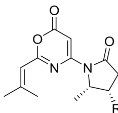
R:OH, Salinazinone A;
