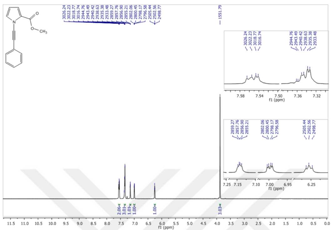
Figure 1 1 H-NMR spectrum of compound 72 in CDCl 3
