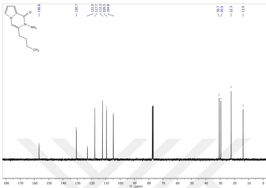
Figure 60 13 C-NMR Spectrum of Compound 81 in CDCl 3
