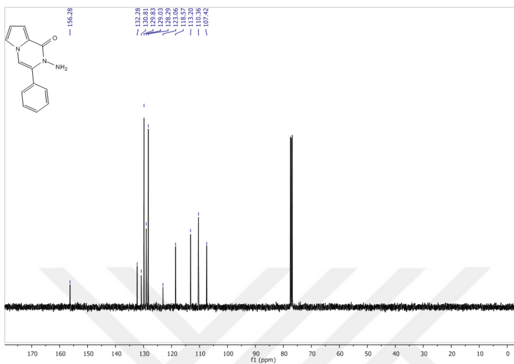
Figure 48 13 C-NMR Spectrum of Compound 77 in CDCl 3
