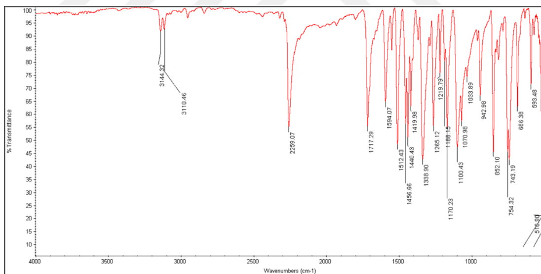
Figure 67 IR Spectrum of Compound 83
