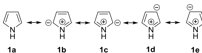
Scheme 1. Resonance structures of pyrrole
