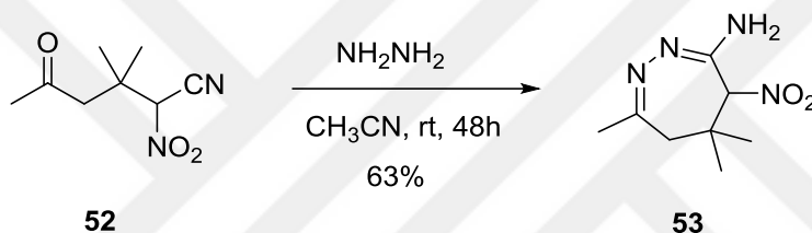
Scheme 9. Cyclization reaction of compound 52 via hydrazine
