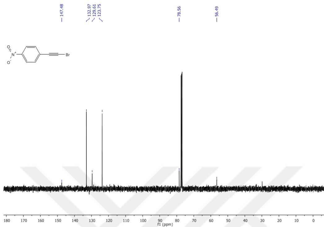
Figure 32 13 C-NMR Spectrum of Compound 71 in CDCl 3
