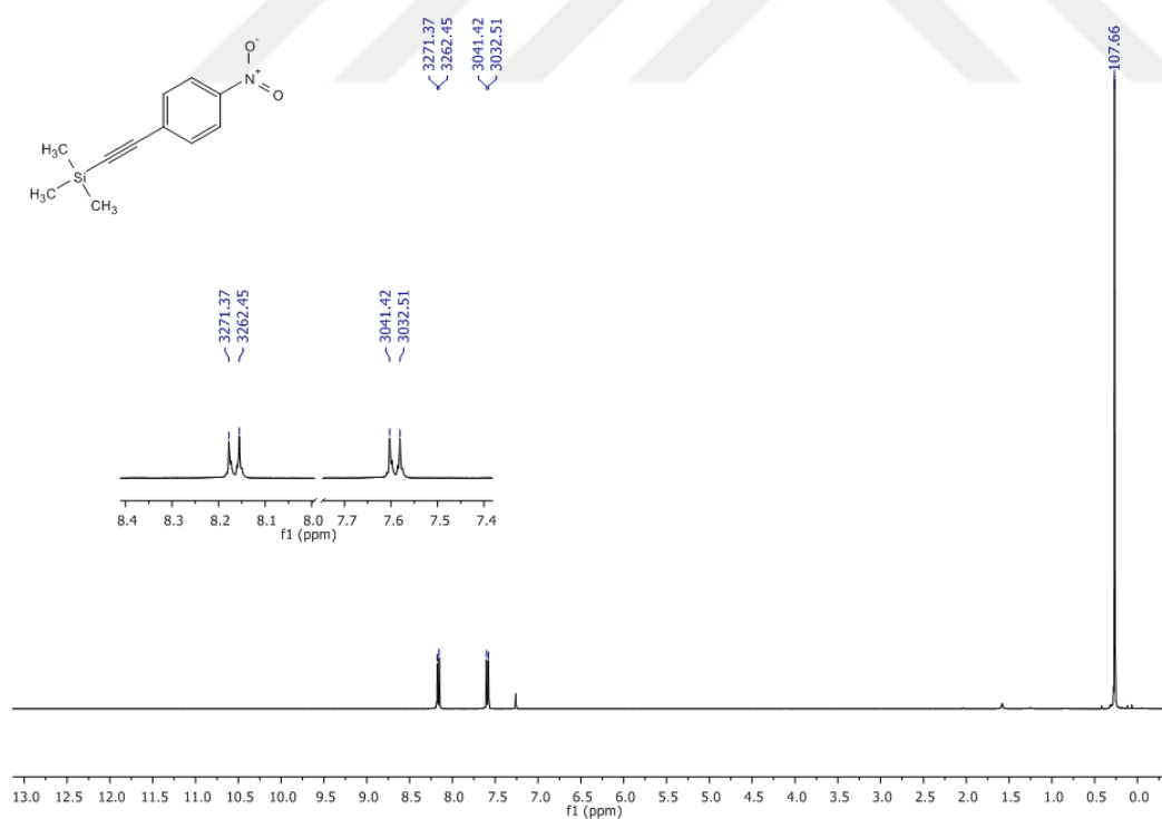
Figure 21 1 H-NMR Spectrum of Compound 64 in CDCl 3
