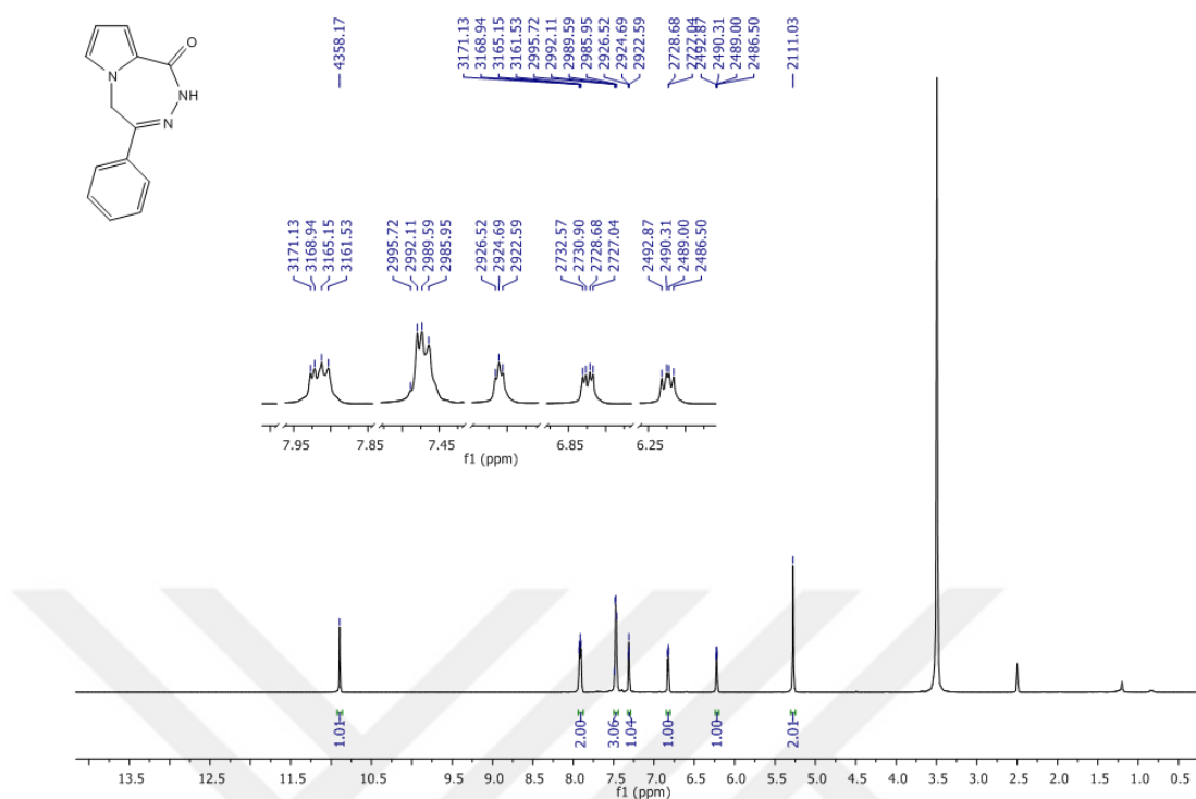
Figure 9 ^1\text{H} -NMR spectrum of compound 80 in \text{DMSO-d}_6
