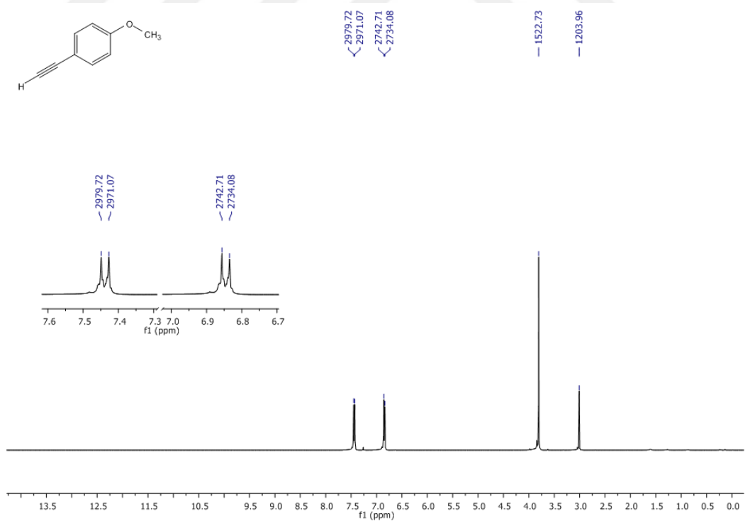
Figure 23 1 H-NMR Spectrum of Compound 65 in CDCl 3
