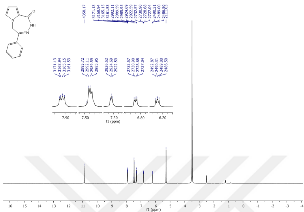
Figure 56 1 H-NMR Spectrum of Compound 80 in DMSO-d 6
