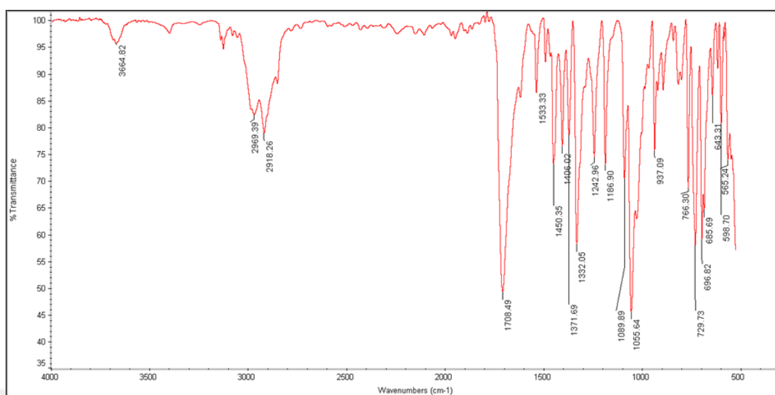
Figure 70 IR Spectrum of Compound 90
