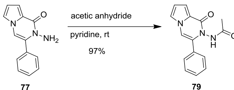
Scheme 25. Acetylation reaction of compound 77 .
