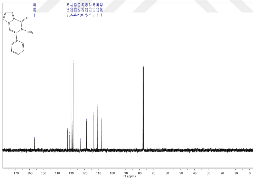
Figure 4 13 C-NMR spectrum of compound 77 in CDCl 3
