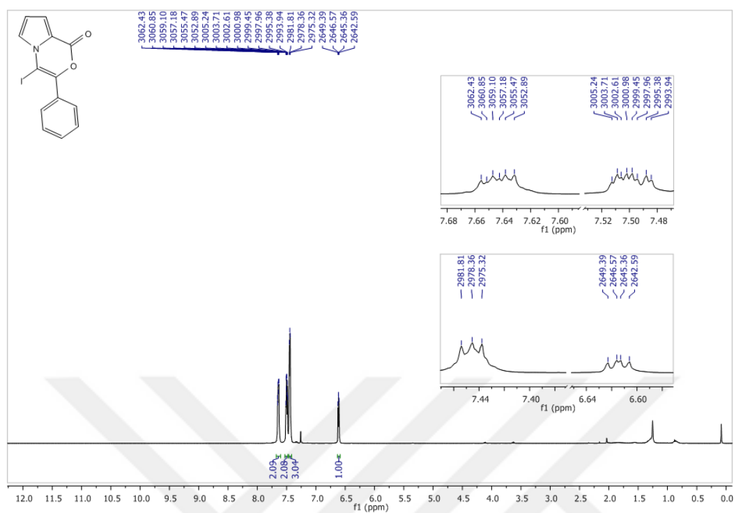
Figure 68 1 H-NMR Spectrum of Compound 90 in CDCl 3
