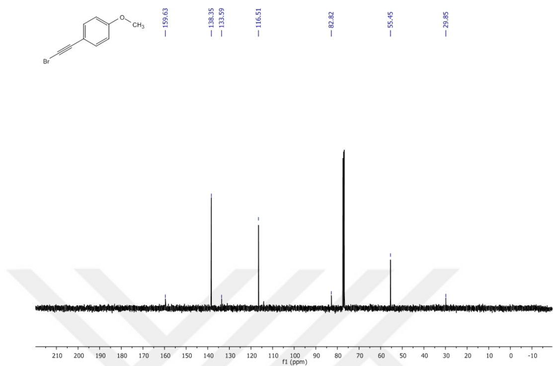
Figure 30 ^{13}\text{C} -NMR Spectrum of Compound 70 in \text{CDCl}_3
