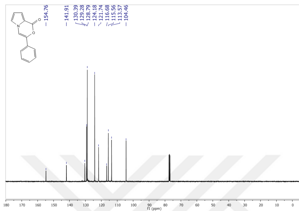
Figure 84 ^{13}\text{C} -NMR Spectrum of Compound 95 in \text{CDCl}_3
