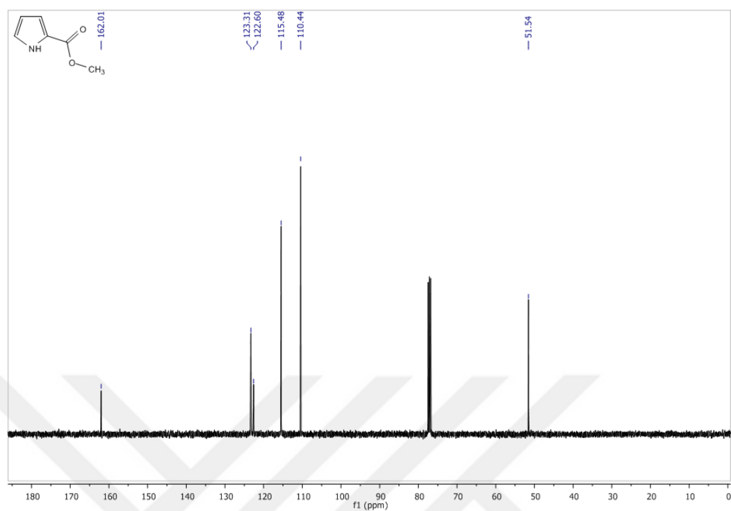
Figure 18 ^{13}\text{C} -NMR Spectrum of Compound 17 in \text{CDCl}_3
