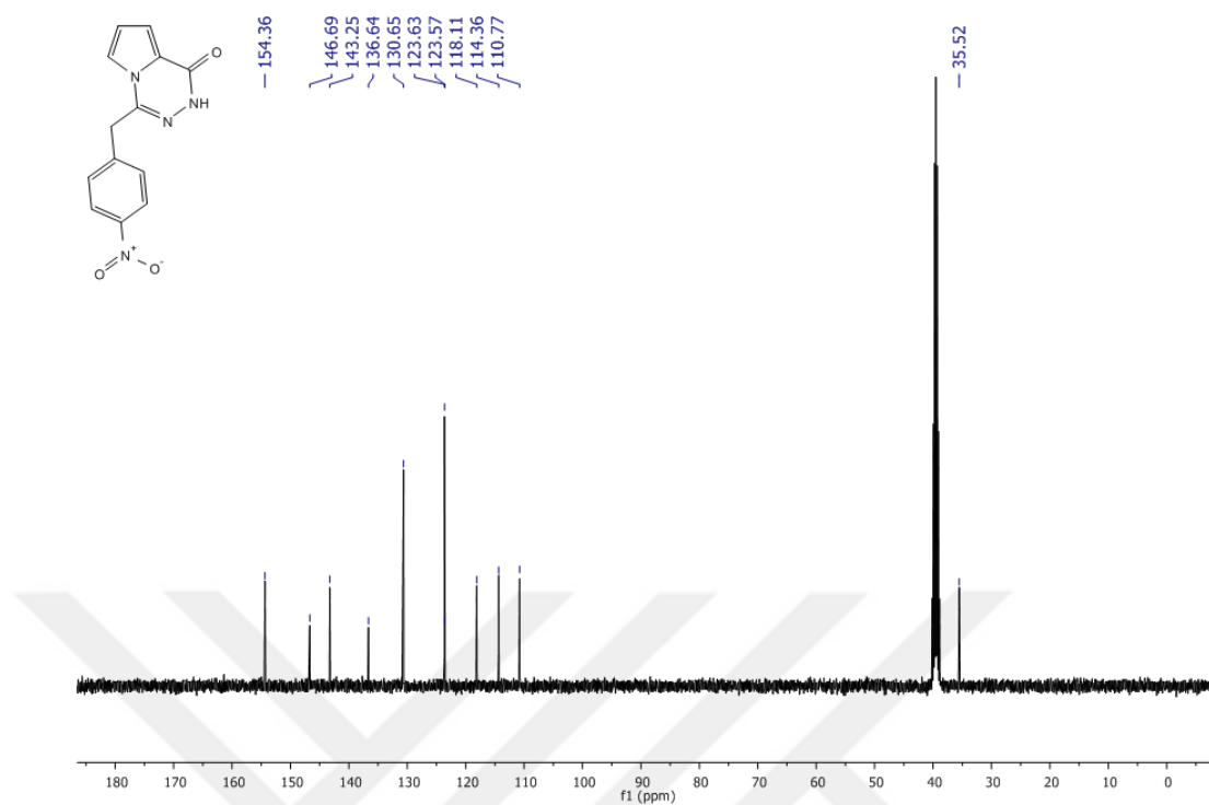
Figure 66 13 C-NMR Spectrum of Compound 83 in DMSO-d 6
