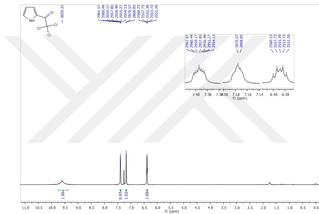
Figure 15 1 H-NMR Spectrum of Compound 60 in CDCl 3
