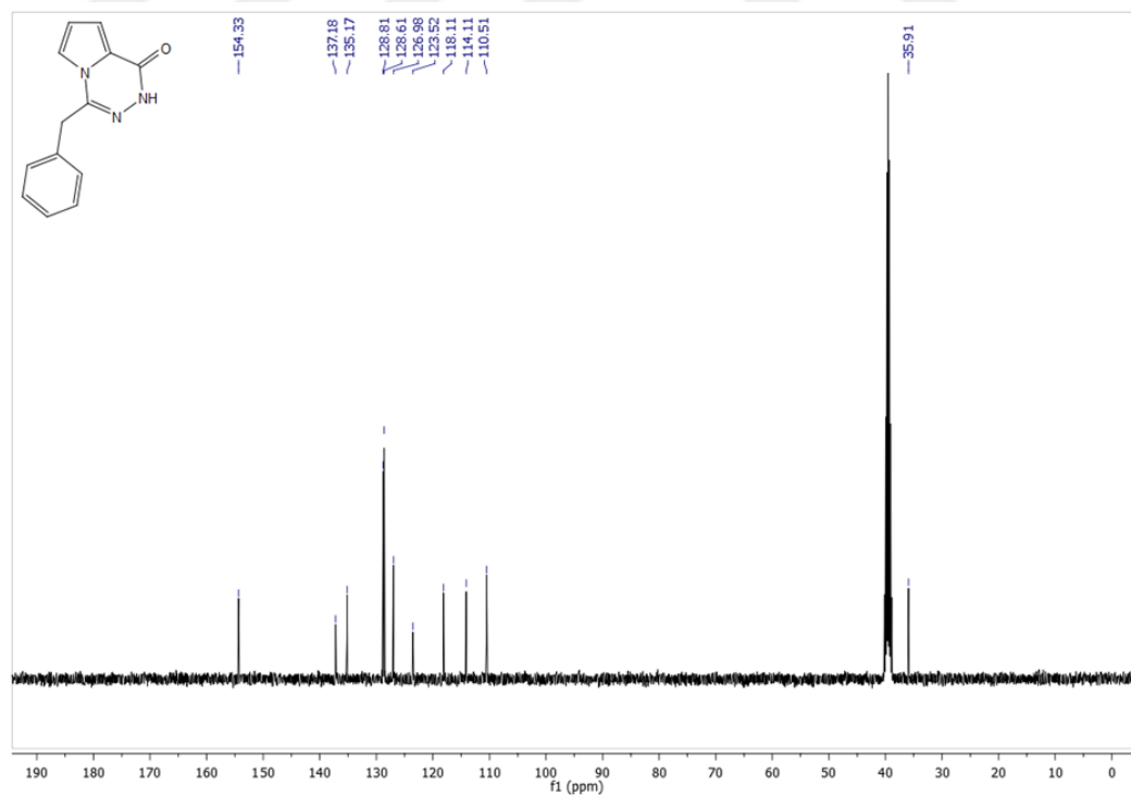
Figure 8 13 C-NMR spectrum of compound 78 in DMSO-d 6
