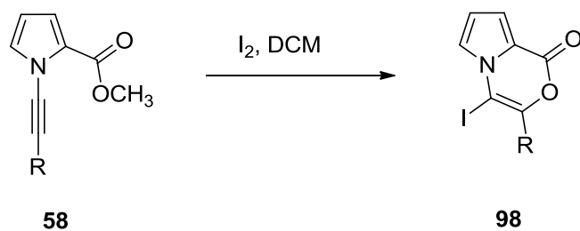
Scheme 34. Electrophilic cyclization reaction via iodine
