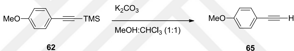
Scheme 18. Hydrolysis of compound 62
