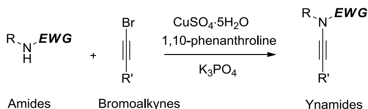
Scheme 21. Copper catalyzed cross-coupling reaction to afford ynamides
