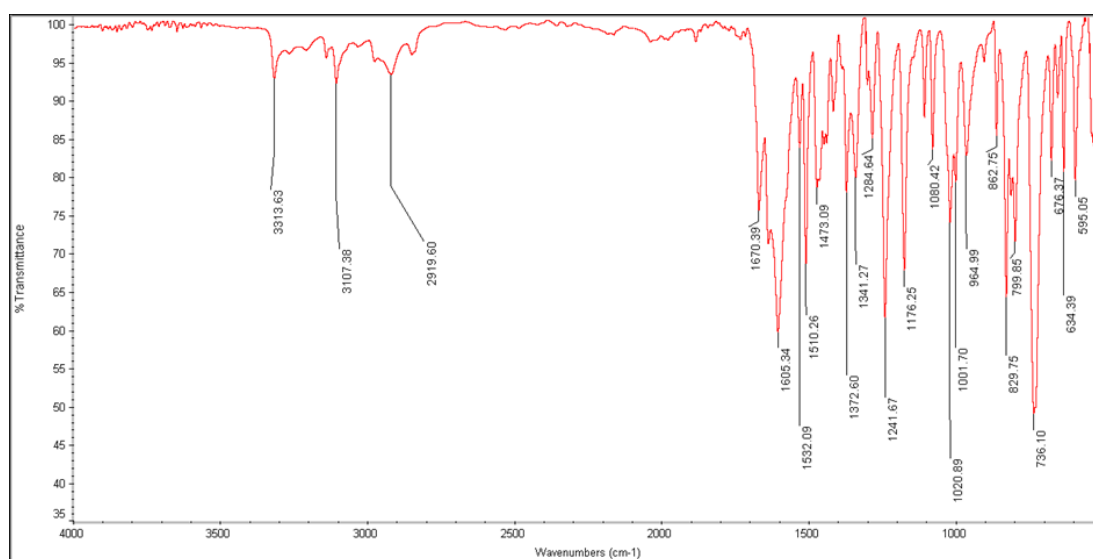
Figure 64 IR Spectrum of Compound 82
