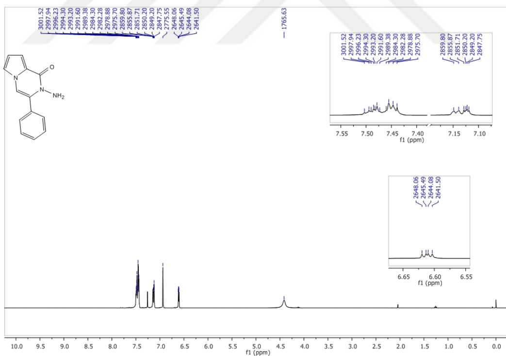
Figure 47 1 H-NMR Spectrum of Compound 77 in CDCl 3
