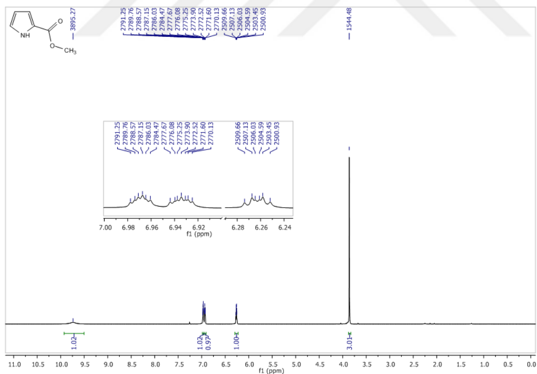
Figure 17 1 H-NMR Spectrum of Compound 17 in CDCl 3
