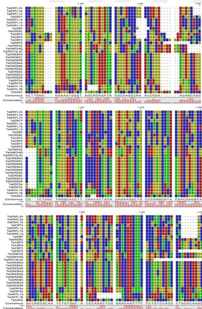
Figure 3.9. Graphical illustration of conserved regions in AP2 containing TF gene family
