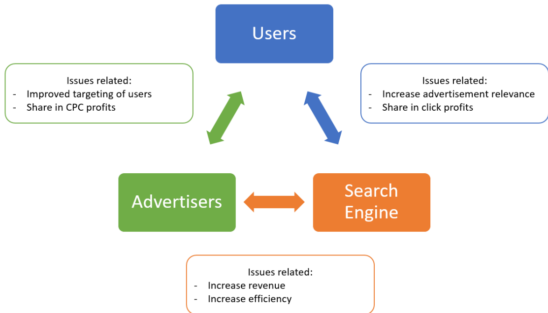
Figure 3.1: Actors
