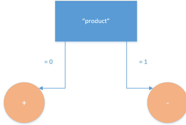
Figure 4.1: Decision Tree
