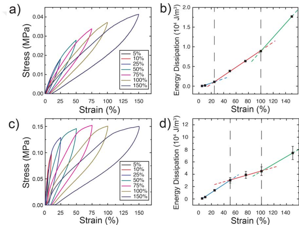
Figure 4.4 a) Stress/strain cycling curves and b) average energy dissipation values and corresponding linear fits for pure SIS fiber mats. c) Stress strain cycling curves and d) average energy dissipation values and corresponding linear fits for elastic conductors fabricated with 25% (wt/vol) STFA solutions. Linear correlations relating energy dissipation to strain describe different regions of strain induced structural changes (blue, red, and green lines).
