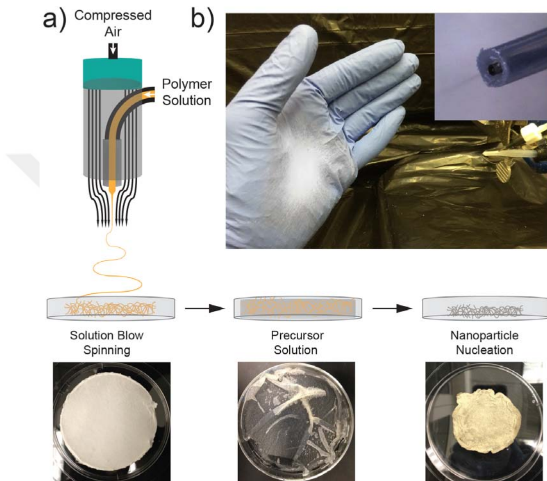
Figure 4.1 a) Schematic illustration of poly(styrene-block-isoprene-block-styrene) (SIS) block copolymer solution blow spun fiber network fabrication and images of the as spun fiber network, fiber mat swollen with silver nanoparticle precursor solution, and conductive polymer-nanoparticle composite after nanoparticle nucleation. b) Image of the direct deposition of SIS fibers onto a gloved hand (solution blow spinning nozzle in use-inset).
