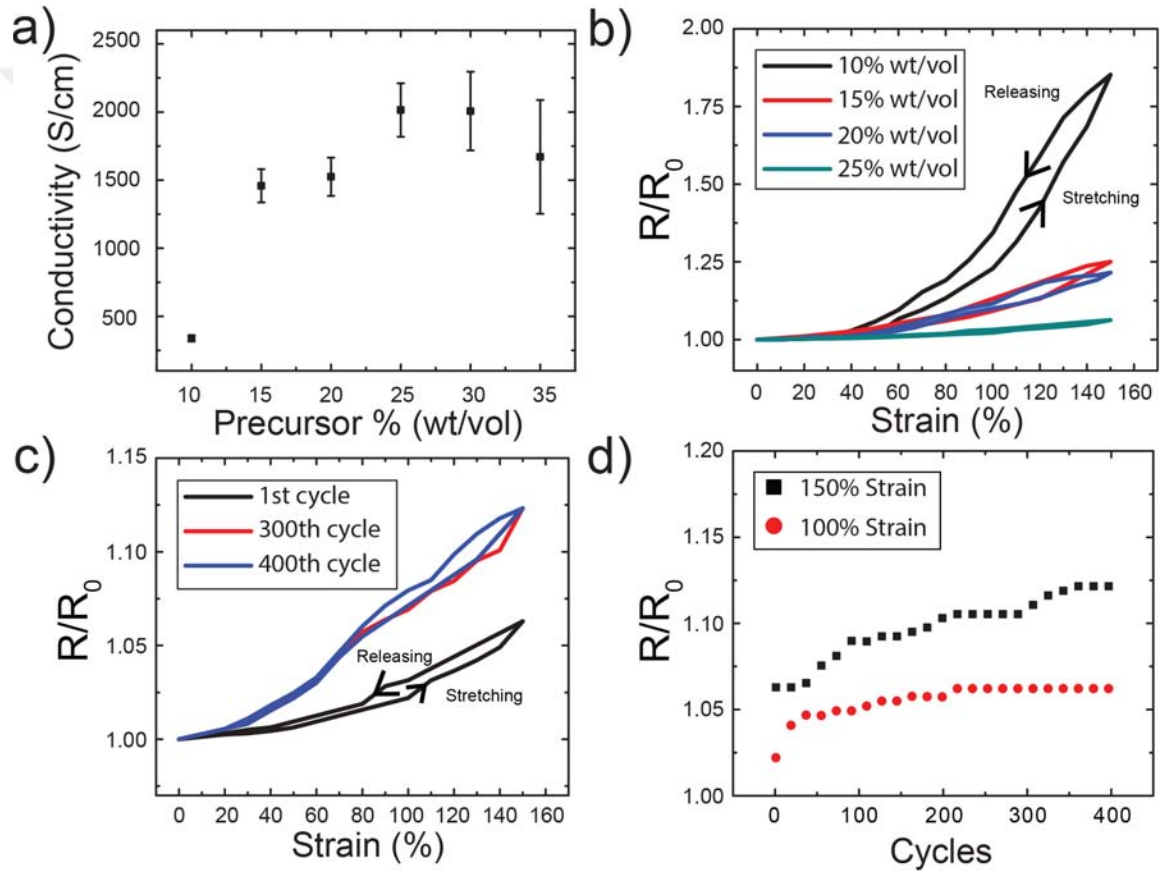
Figure 4.3 a) Average electrical conductivity of stretchable conductors as a function of STF concentration. b) Normalized resistance values as a function of uniaxial tensile strain for various STF concentrations. c,d) Normalized resistance values as a function of uniaxial tensile strain and cycle number.
