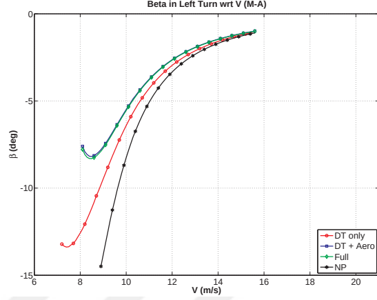
Figure 3.9. Different sources effect on sideslip with respect to V in left turn.
