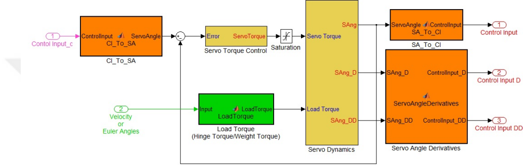
Figure 2.1. Simulink diagram for actuator dynamics.
