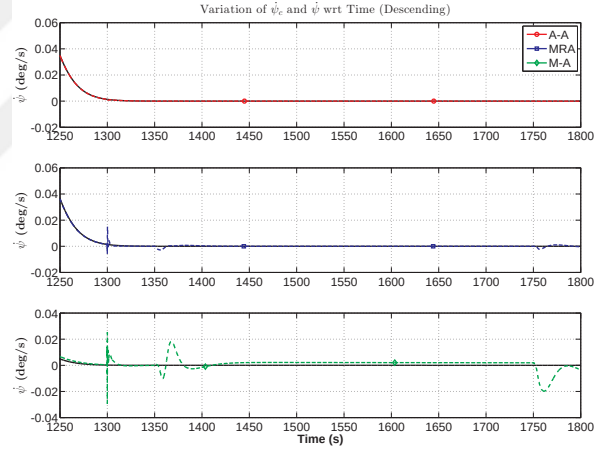
Figure 6.47. Variation of \psi and \psi_c with time in descending.
