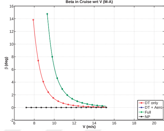
Figure 3.3. Different sources effect on sideslip with respect to V in cruise.
