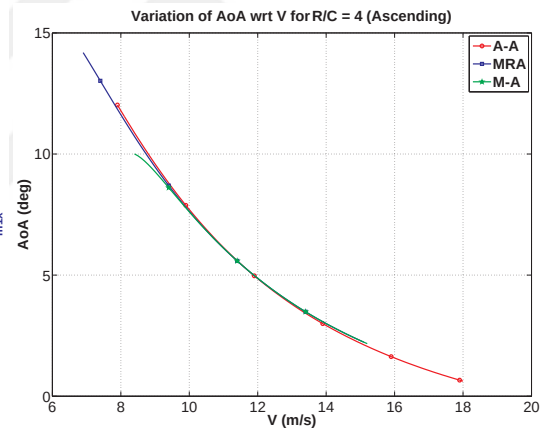
Figure 4.66. Angle of attack variation with speed in ascending.
