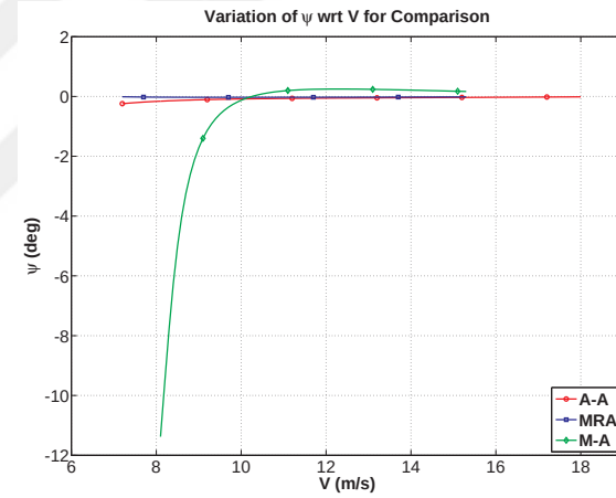
Figure 4.31. Yaw angle variation with speed in cruise.
