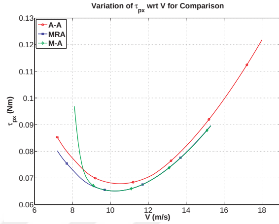
Figure 4.33. Required torque variation with speed in cruise.
