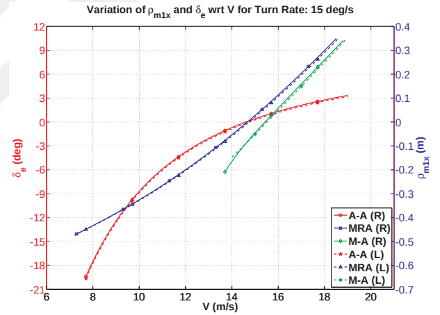
Figure 4.40. Position of long-mass and elevator variation with speed for \dot{\psi} = 15 deg/s.
