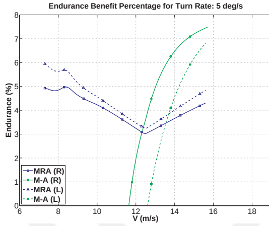
Figure 4.53. Percent increase in endurance as compared to that of A-A aircraft for \dot{\psi} = 5 deg/s.
