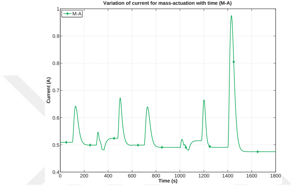
Figure 3.22. Variation of current for mass-actuation with time in mission-1.
