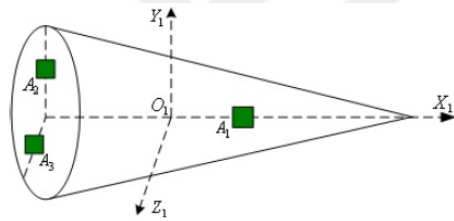
Figure 1.7. Missile with internal mass mechanism [7].
