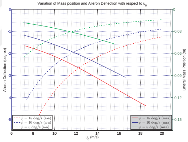
Figure A.22. Comparison between \rho_{m_{2y}} and \delta_a with respect to u_0 .
