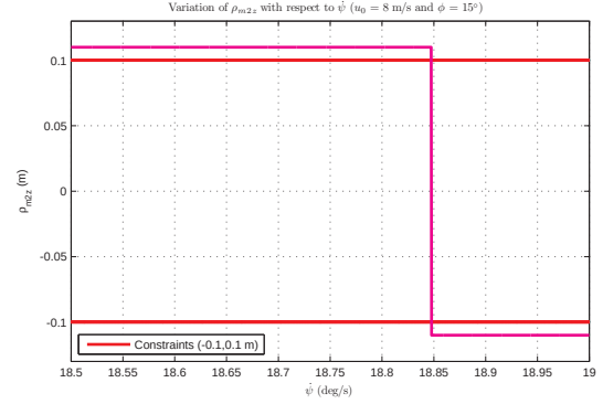
Figure A.5. \rho_{m2z} when u_0 = 8 \text{ m/s} and \phi = 15^\circ .
