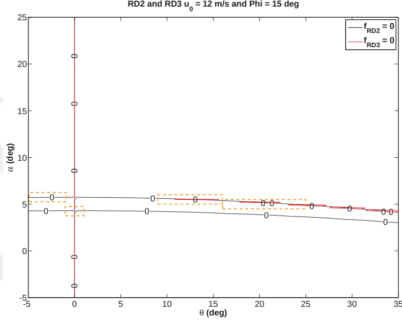
Figure A.6. The zero level curves in terms of u_0 = 12 \text{ m/s} and \phi = 15^\circ .
