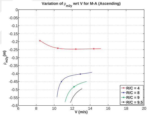
Figure 4.58. \rho_{m2y} variation with speed for M-A aircraft.
