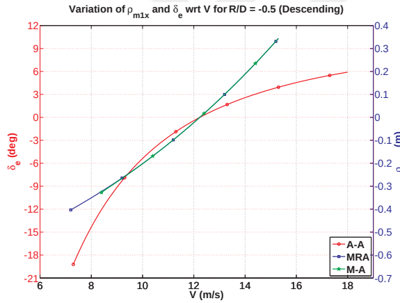
Figure 4.75. \rho_{m1x} and \delta_e variation with speed in descending.
