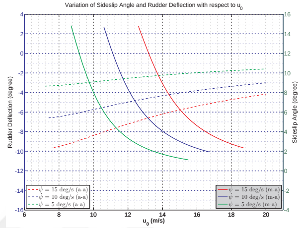
Figure A.16. Comparison between \beta and \delta_r with respect to u_0 .
