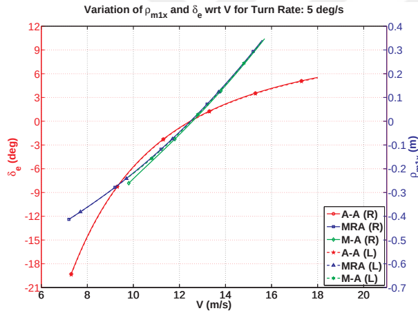
Figure 4.39. Position of long-mass and elevator variation with speed for \dot{\psi} = 5 deg/s.
