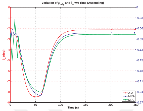
Figure 6.52. Variation of \rho_{m2y} and \delta_a with time in ascending.
