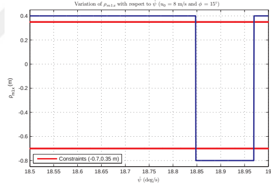
Figure A.3. \rho_{m_{1x}} when u_0 = 8 \text{ m/s} and \phi = 15^\circ .
