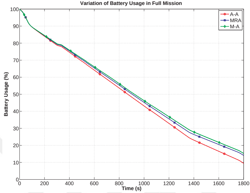
Figure 6.60. Battery usage of airplanes in full mission.
