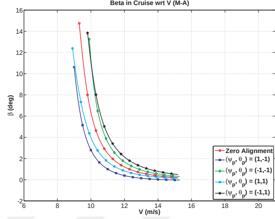
Figure 3.11. Alignment effect on sideslip with respect to V in cruise.
