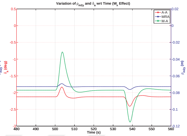
Figure 6.37. Effect of W_x on \rho_{m2y} and \delta_a with time.
