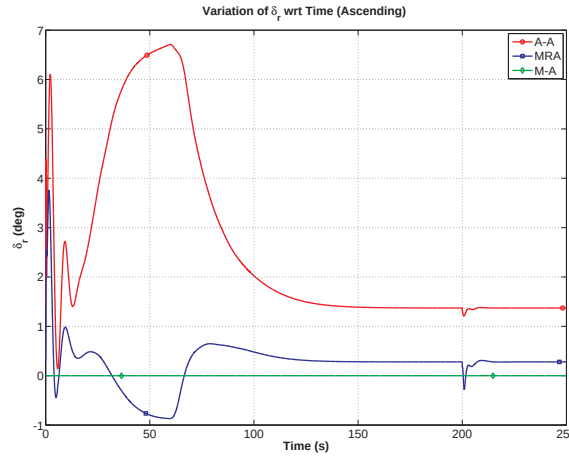
Figure 6.54. Variation of \delta_r with time in ascending.
