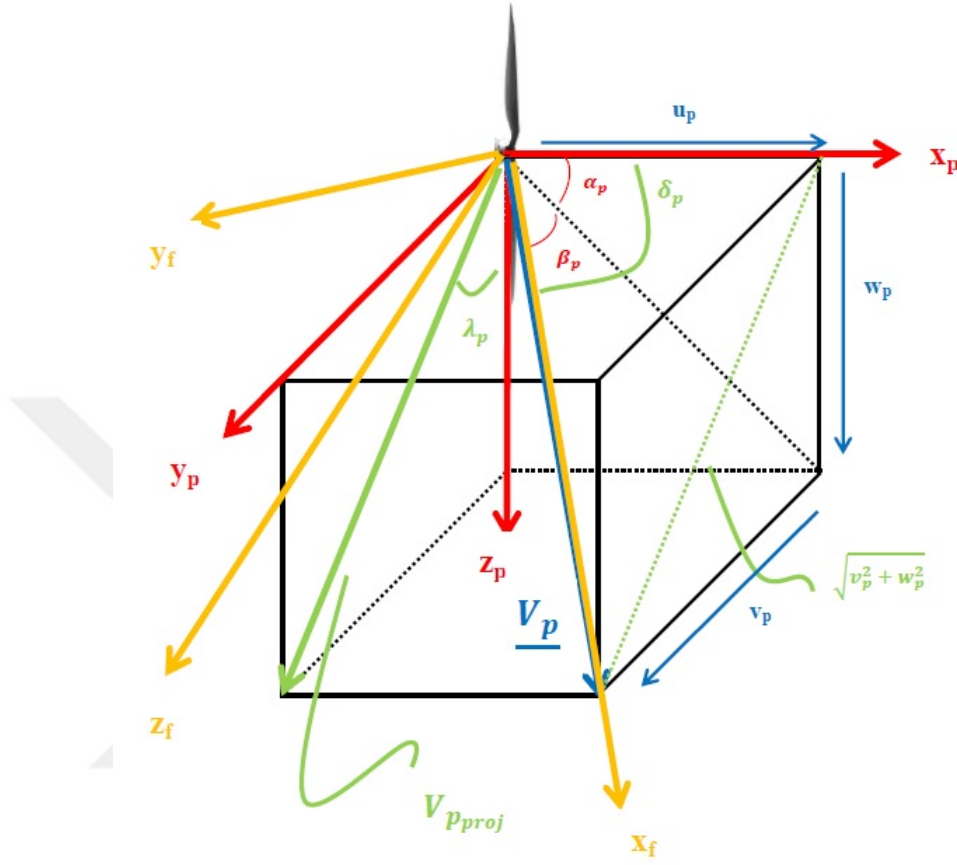
Figure 2.4. Propeller and flow frame.
