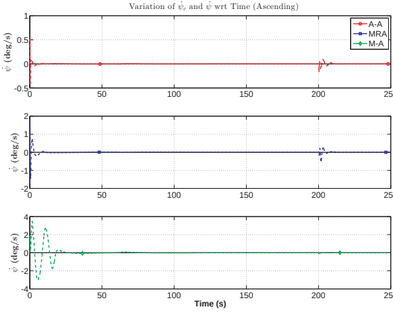
Figure 6.46. Variation of \psi and \psi_c with time in ascending.
