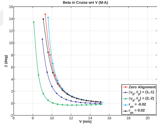
Figure 3.15. Placement effect on sideslip with respect to V in cruise.
