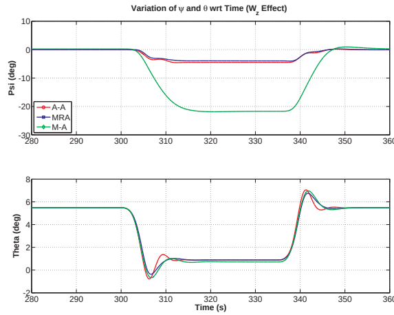
Figure 6.42. Effect of W_z on \psi and \theta with time.
