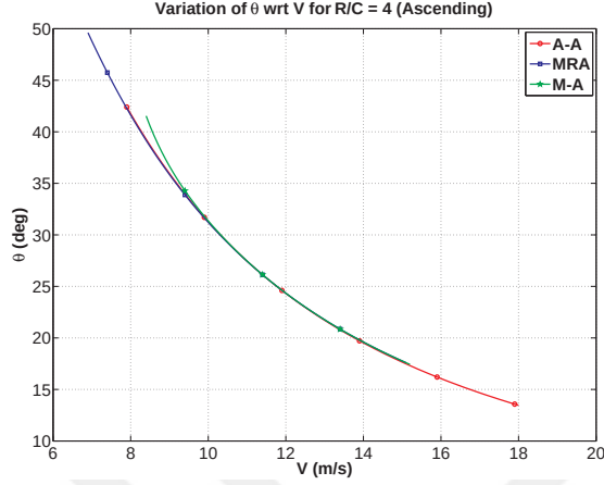
Figure 4.67. Pitch angle variation with speed in ascending.
