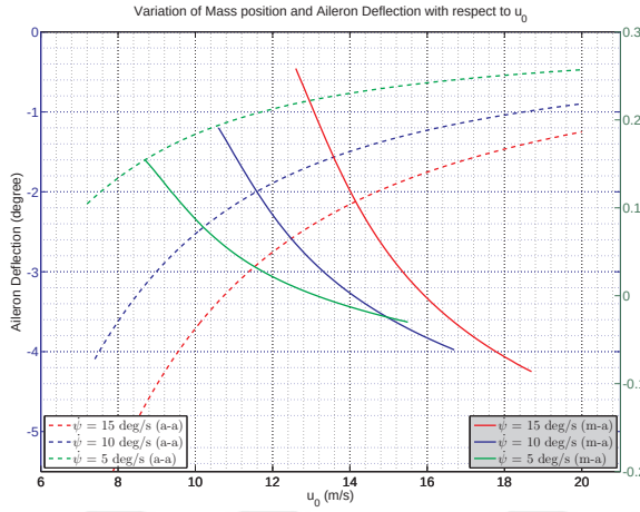
Figure A.15. Comparison between \rho_{m_{2y}} and \delta_a with respect to u_0 .
