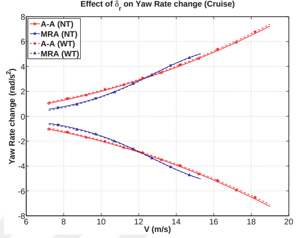
Figure 5.16. Effect of \delta_r on yaw rate change, \Delta\dot{r} , in cruise.
