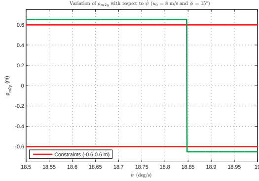
Figure A.4. \rho_{m2y} when u_0 = 8 \text{ m/s} and \phi = 15^\circ .
