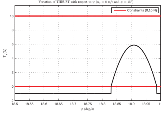
Figure A.2. Required thrust when u_0 = 8 \text{ m/s} and \phi = 15^\circ .
