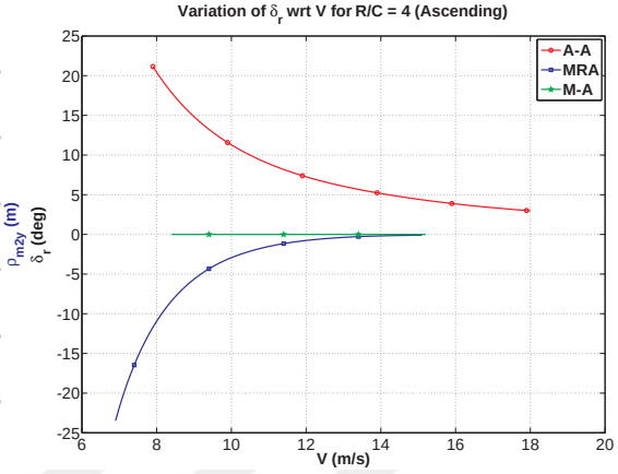
Figure 4.64. \delta_r variation with speed in ascending.
