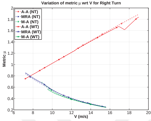
Figure 5.2. Metric \mu variation with speed in right turn.
