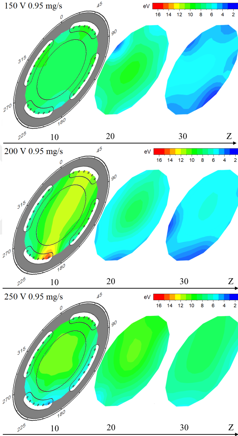
Figure 4.A.2.2 Electron temperature distributions at different axial distances for cathode position of \theta = 0^\circ .
