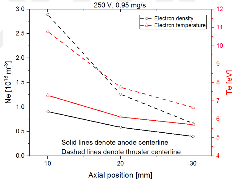
Figure 4.17 Electron density and electron temperature profiles experimentally measured in the axial direction for 250 V - 0.95 mg/s. Anode centerline means the line passing through the midpoints between the inner and outer edges of the anode disc.
