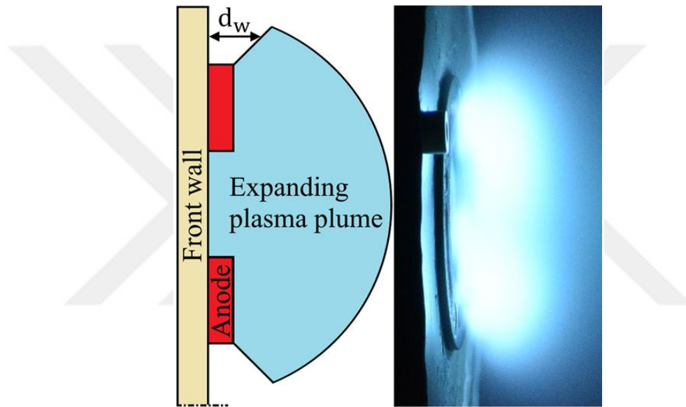
Figure 5.6 A schematic of expanding plasma plume of the XPT (left) and a side view photo of a thruster firing taken during experiments (right). d_w shows the distance between the front wall and the edge of the expanding plasma plume.
