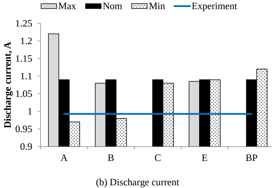
Figure 3.4 Summary of the one-at-a-time sensitivity analysis results of UT-62 Hall thruster for thrust and discharge current. Note the “nom” nominal condition is displaying the same result for all cases.
