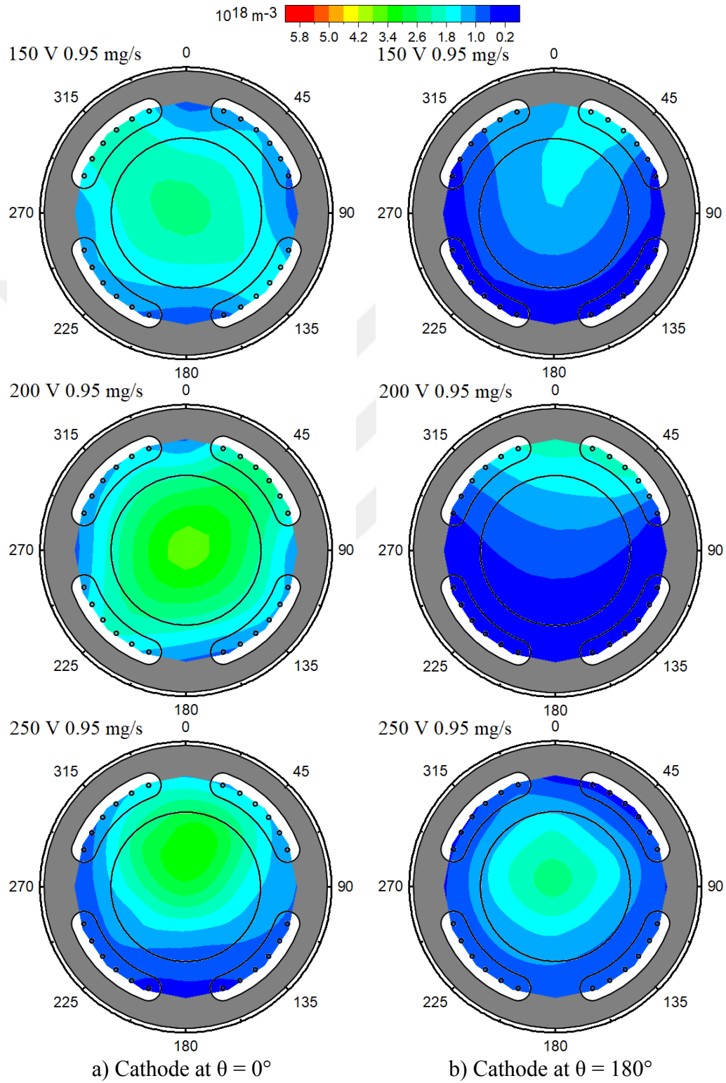
Figure 4.A.1.4 Electron density distributions for 0.95 mg/s.
