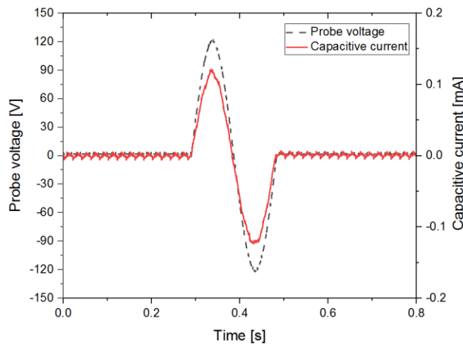
Figure 4.8 Capacitive current of the electrical circuit.
