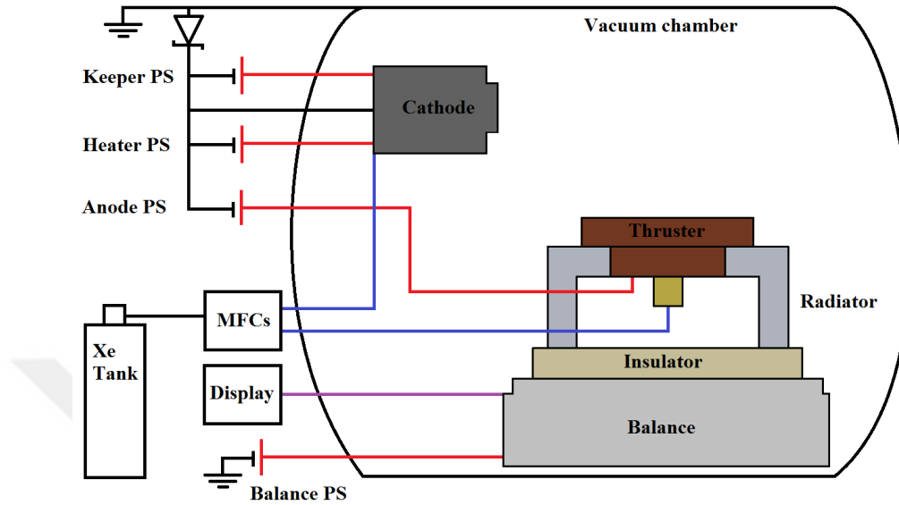
Figure 4.A.3.2 Electrical diagram of the experimental setup.
