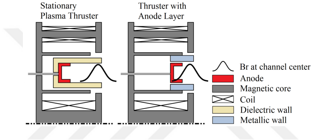
Figure 1.1 Comparison of SPT and TAL.
