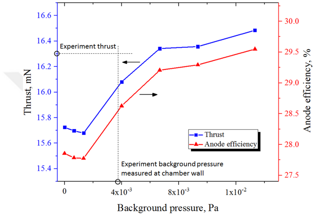
Figure 3.7 Simulated thrust and anode efficiency of UT-62 Hall thruster under different background pressure conditions.
