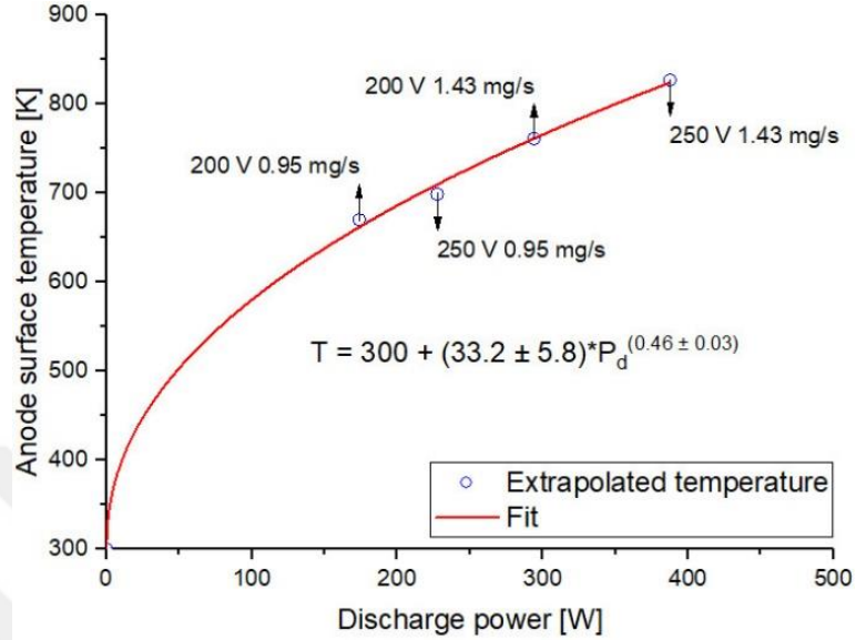
Figure 4.21 Experimentally measured anode surface temperatures against discharge power.
