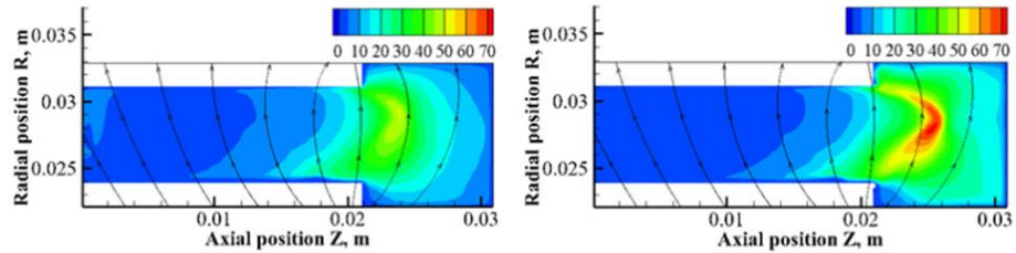
(e) Electron temperature (eV)
