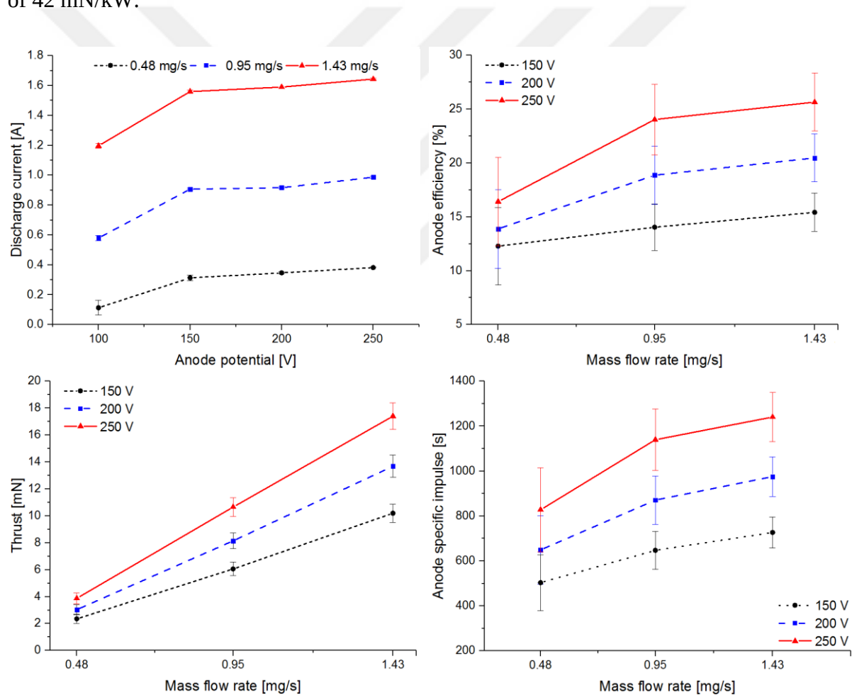
Figure 4.12 Experimental performance characteristics. Error bars represents 1-sigma standard deviation of the total error.
