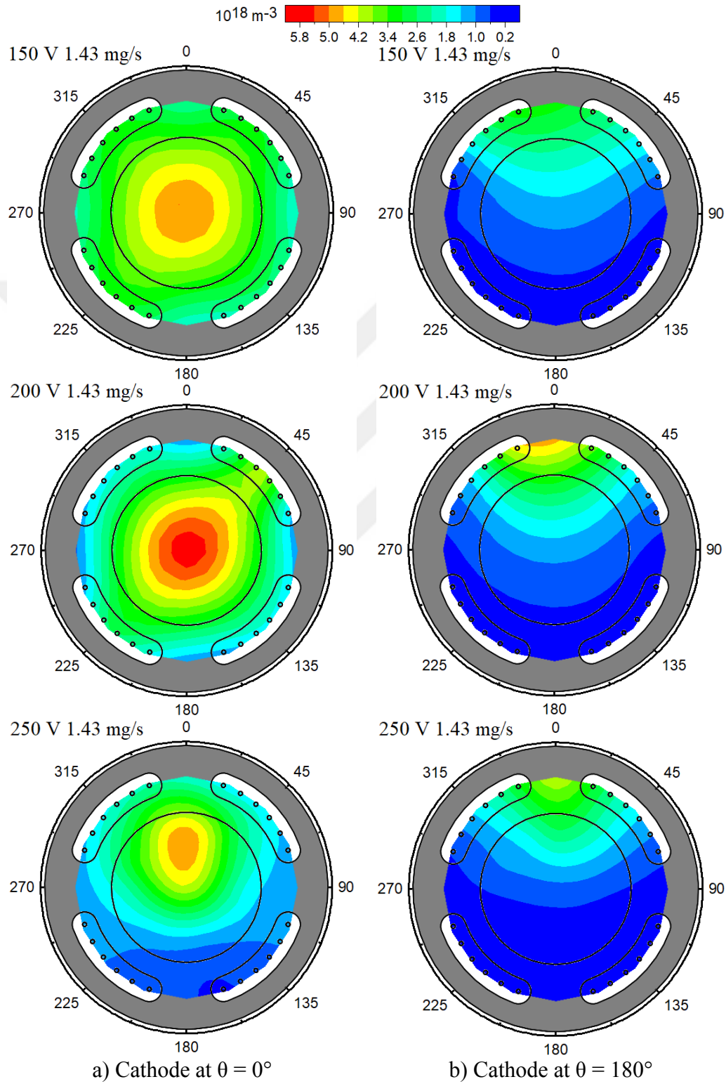
Figure 4.A.1.3 Electron density distributions for 1.43 mg/s.
