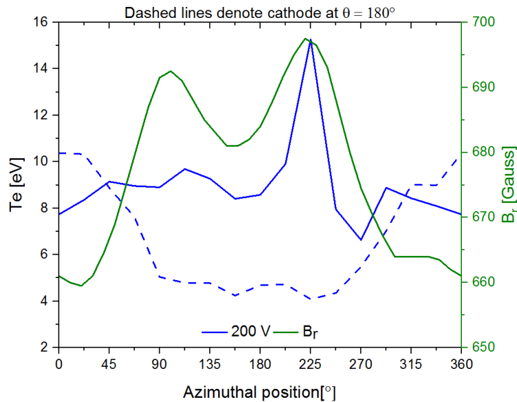
Figure 4.19 Distribution of electron temperature experimentally measured in the azimuthal direction along the anode centerline for 200 V - 1.43 mg/s.
