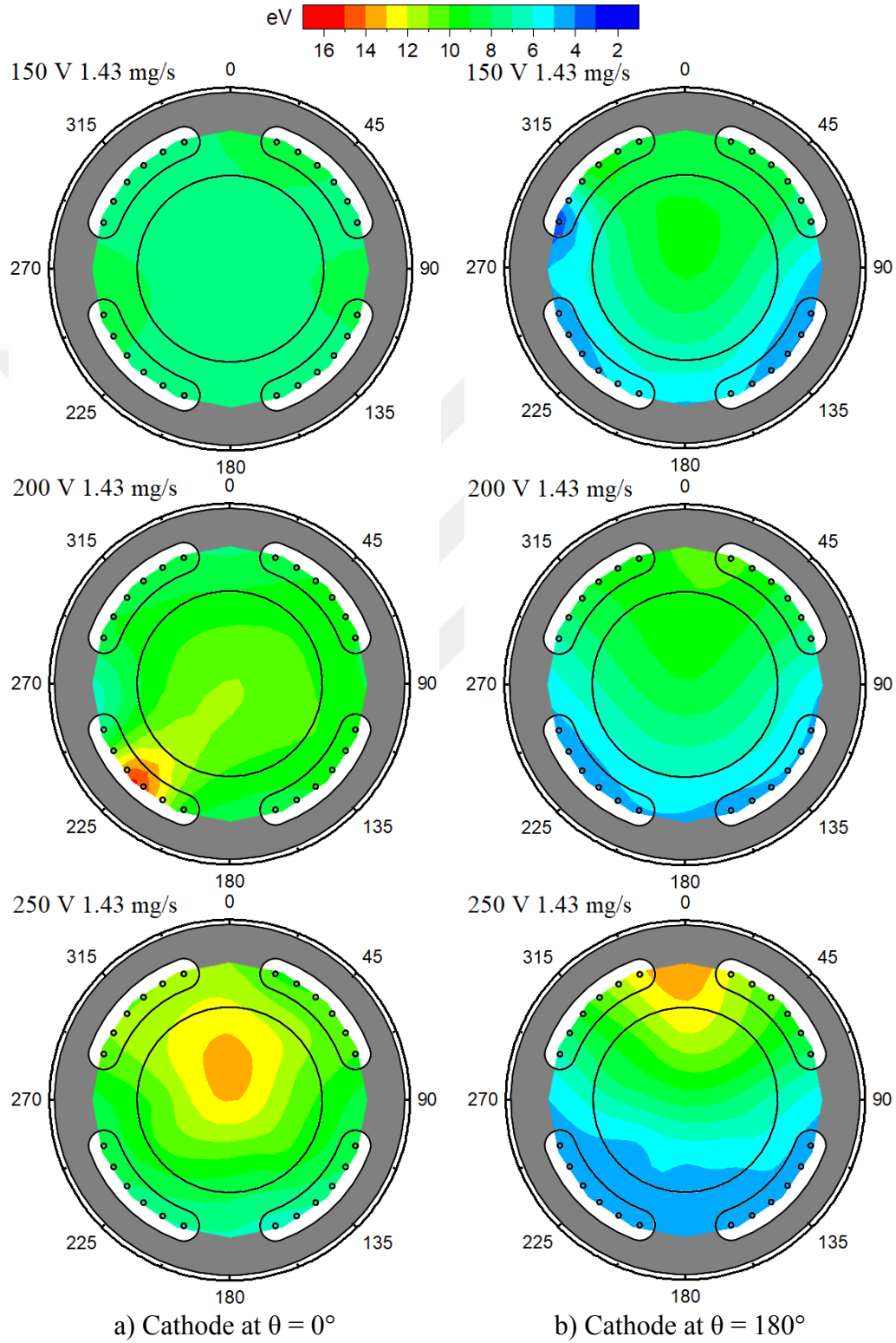
Figure 4.A.2.3 Electron temperature distributions for 1.43 mg/s.
