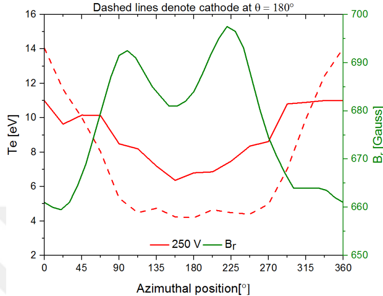
Figure 4.20 Distribution of electron temperature experimentally measured in the azimuthal direction along the anode centerline for 250 V - 1.43 mg/s.
