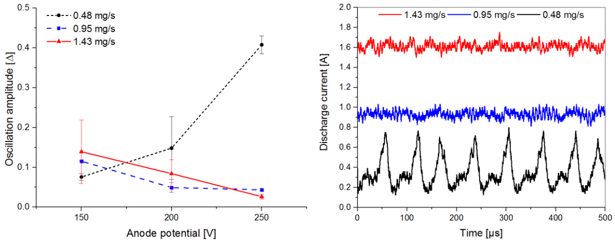
Figure 4.13 Experimental oscillation amplitudes and discharge current wave forms at 250 V.
