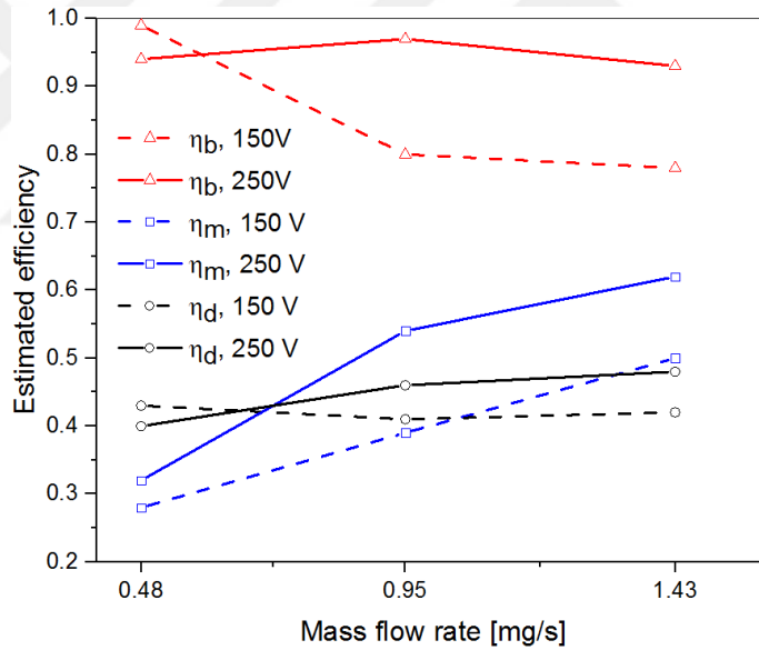
Figure 4.15 Anode efficiency components estimated at the thruster exit ( 0x D_A ) using experimental data. \eta_b , \eta_m and \eta_d shows efficiencies related to current utilization, mass utilization and plume divergence respectively
