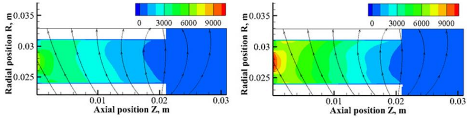
(a) Neutral density distribution ( 10^{16} \text{ m}^{-3} )
