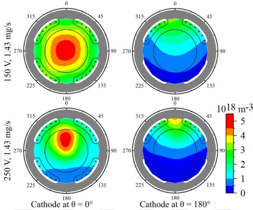
Figure 4.16 2D electron density maps experimentally measured for 150 V - and 250 V - 1.43 mg/s at z = 10 mm.
