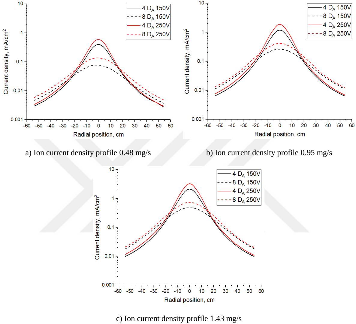
Figure 4.14 Experimental ion current density profiles plotted on logarithmic scale. D A means anode diameter.
