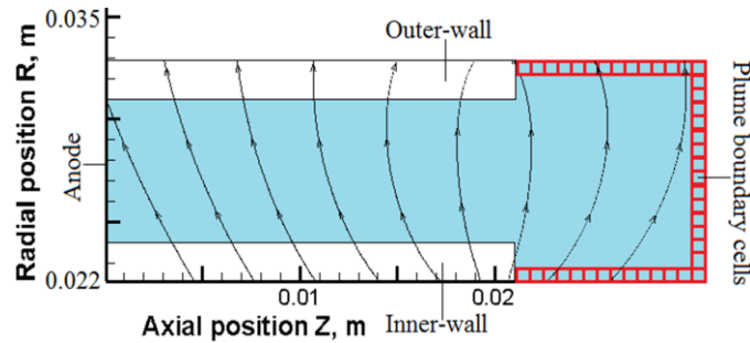
(b) Close-up view of computational domain. Lines with arrows represent the magnetic field applied.
