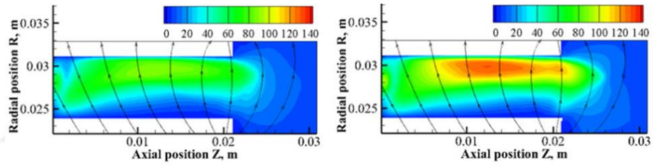
(c) Plasma ion density distribution ( 10^{16} \text{ m}^{-3} )
