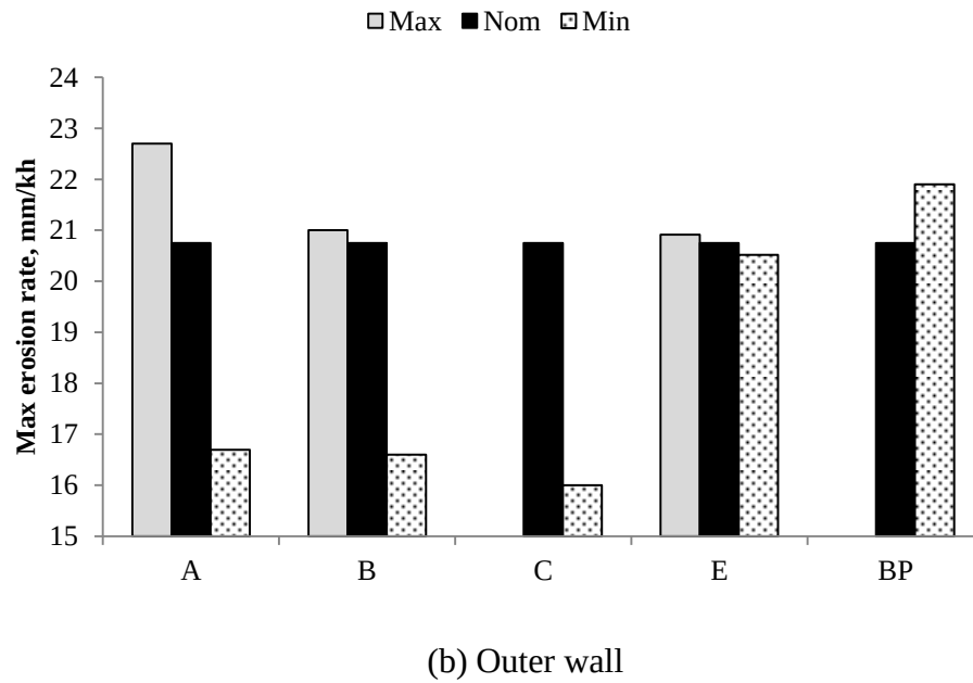
Figure 3.9 Summary of the one-at-a-time sensitivity analysis results of UT-62 Hall thruster for the maximum channel-wall erosion rate.
