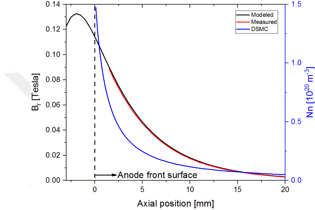
Figure 2.7 Br Nn distributions of the XPT thruster head. Br and Nn are along the anode centerline.
