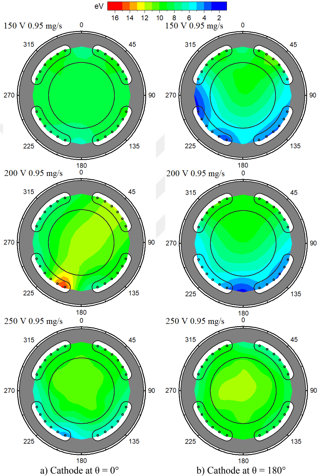
Figure 4.A.2.4 Electron temperature distributions for 0.95 mg/s.
