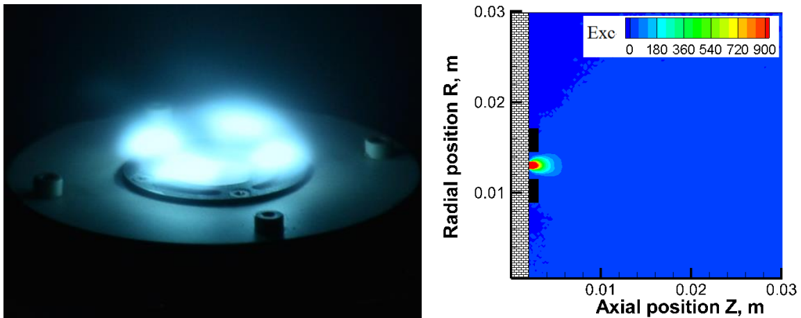
Figure 4.24 Anode dark space photo taken during experiments (left) and simulated excitation collisions (right).
