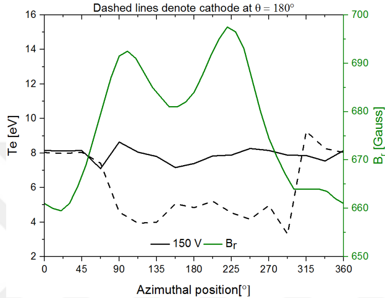
Figure 4.18 Distribution of electron temperature experimentally measured in the azimuthal direction along the anode centerline for 150 V - 1.43 mg/s.
