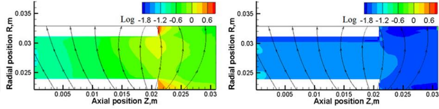
(b) Neutral temperature (eV)
