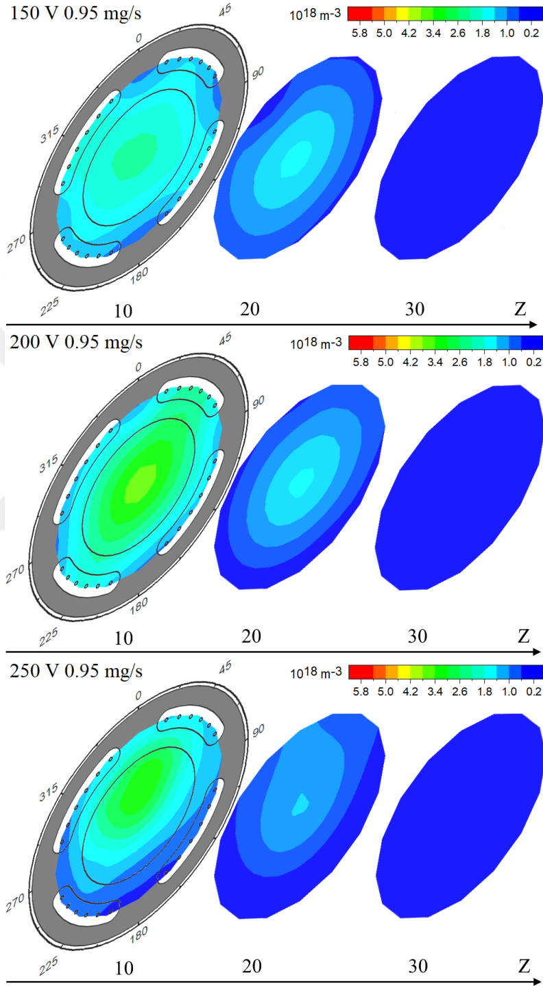
Figure 4.A.1.2 Electron density distributions at different axial distances for cathode position of \theta = 0^\circ .
