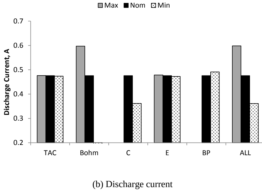
Figure 3.12 Summary of the one-at-a-time sensitivity analysis results of the XPT for thrust and discharge current. Note the “nom” nominal condition is displaying the same result for all cases.
