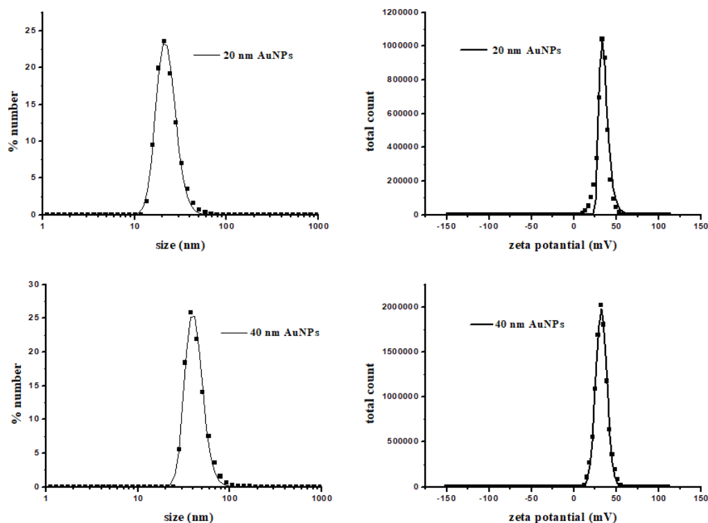
Figure 3.5. Size and zeta potentials of 20 nm and 40 nm non conjugated AuNPs. Size and zeta potential distribution was obtained by using DLS
