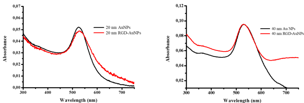
Figure 3.4. UV-vis spectrum of 20 nm non conjugated and RGD conjugated AuNPs (left) and 40 nm non conjugated and RGD conjugated AuNPs (right)
