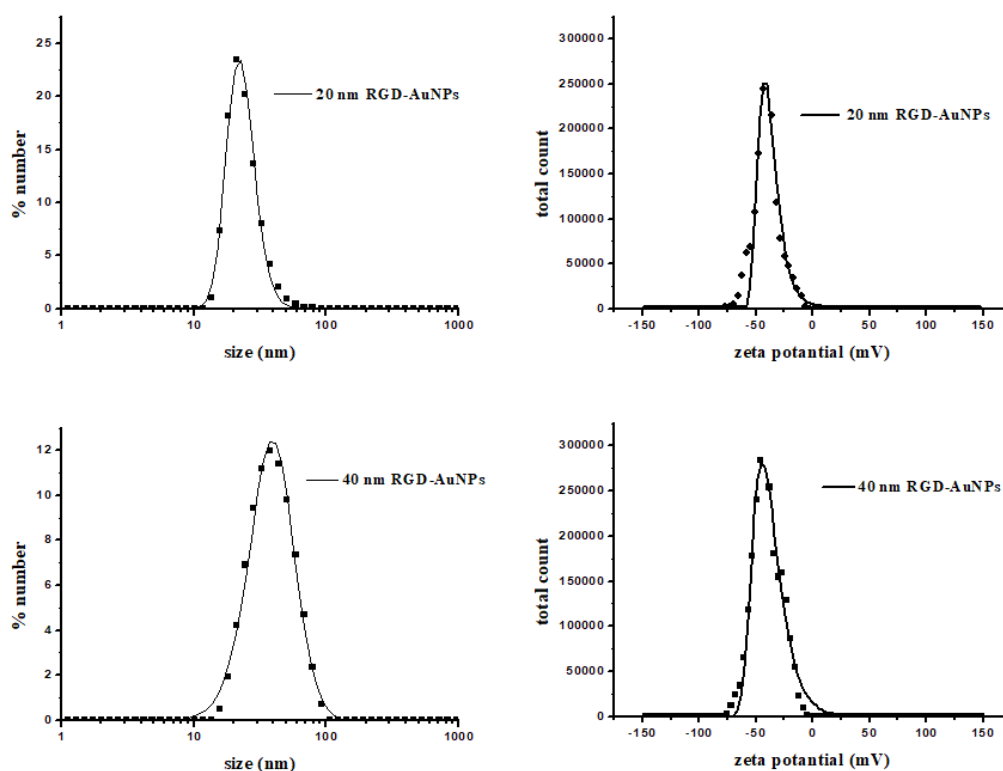
Figure 3.6. Measurements of particle size and zeta potentials of 20 nm and 40 nm RGD conjugated AuNPs. Size and zeta potential distribution was obtained by using DLS.
