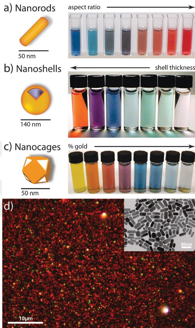
Figure 1.1. a) Gold nanorods, (b) silica–gold core–shell nanoparticles, and (c) gold nanocages. The intense color of these nanoparticles arises from the collective excitation of their conduction electrons, or surface plasmon resonance modes, which results in photon absorption at wavelengths, which varies with (a) aspect ratio, (b) shell thickness, and/or (c) galvanic displacement by gold. (d) Optical dark-field scattering micrograph of gold nanorods (electron micrograph in the inset) showing resonant scattering from their transverse (short-axis) plasmon mode (green) and their lower energy, longitudinal (long-axis) plasmon mode (red)). (Source: Dreaden et al. 2012)
