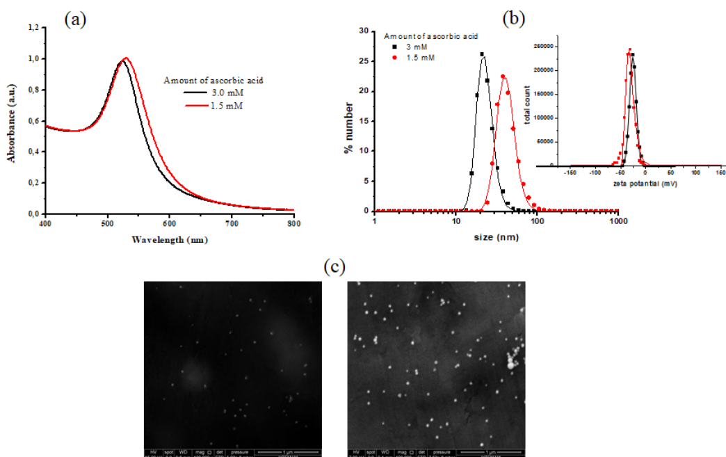
Figure 2.5. Characterizations of synthesized 20 nm and 40 nm gold nanoparticles. UV-vis spectrum (a), size distribution (b) and insert graph shows the zeta potential distributions of gold nanoparticles obtained from DLS measurements. SEM images (c) of AuNPs of size 20 nm (left) and 40 nm (right).
