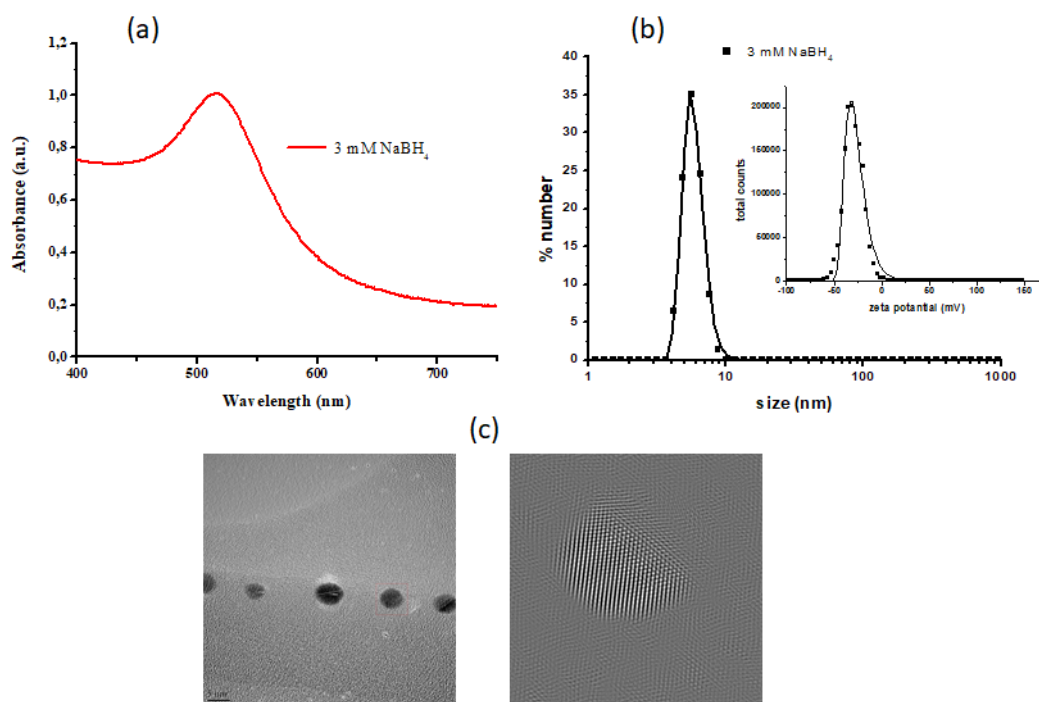
Figure 2.4. Characterizations of 5 nm gold nanoparticles UV-Vis spectrum (a) and TEM images (c) of AuNP. Right graph shows the size distribution and insert graph shows the zeta potential distributions of gold nanoparticles obtained from DLS measurements (b).
