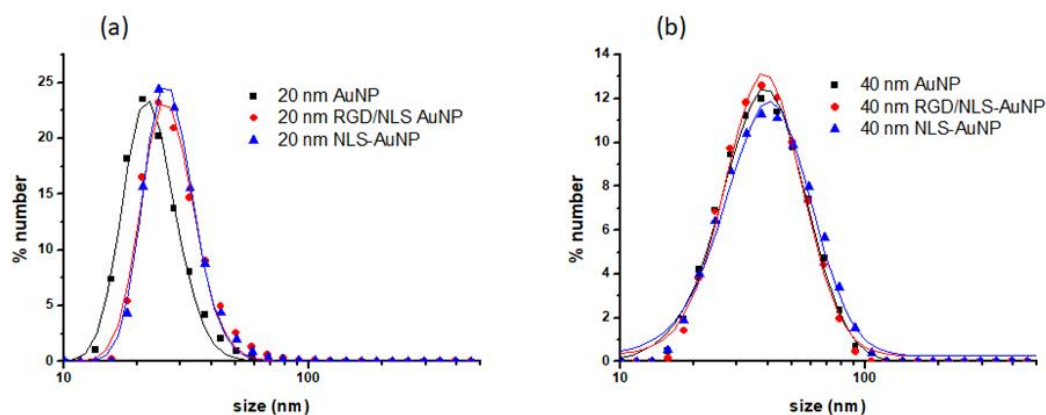
Figure 4.4. Size distribution of non conjugated and conjugated 20 nm (a) and 40 nm (b) AuNPs nanoparticles results obtained by using DLS.
