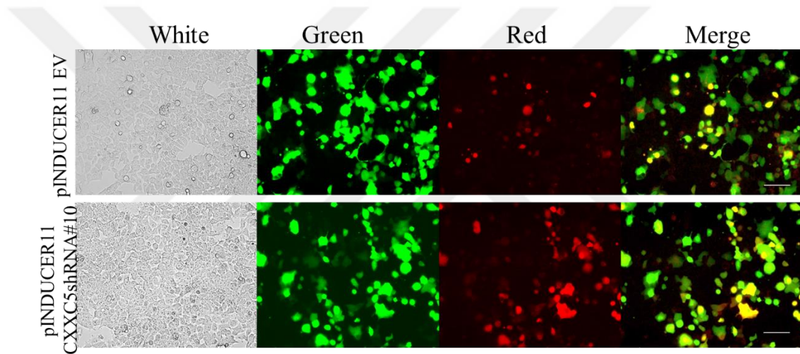
Figure 11 Transfection with pINDUCER11 and packaging elements
