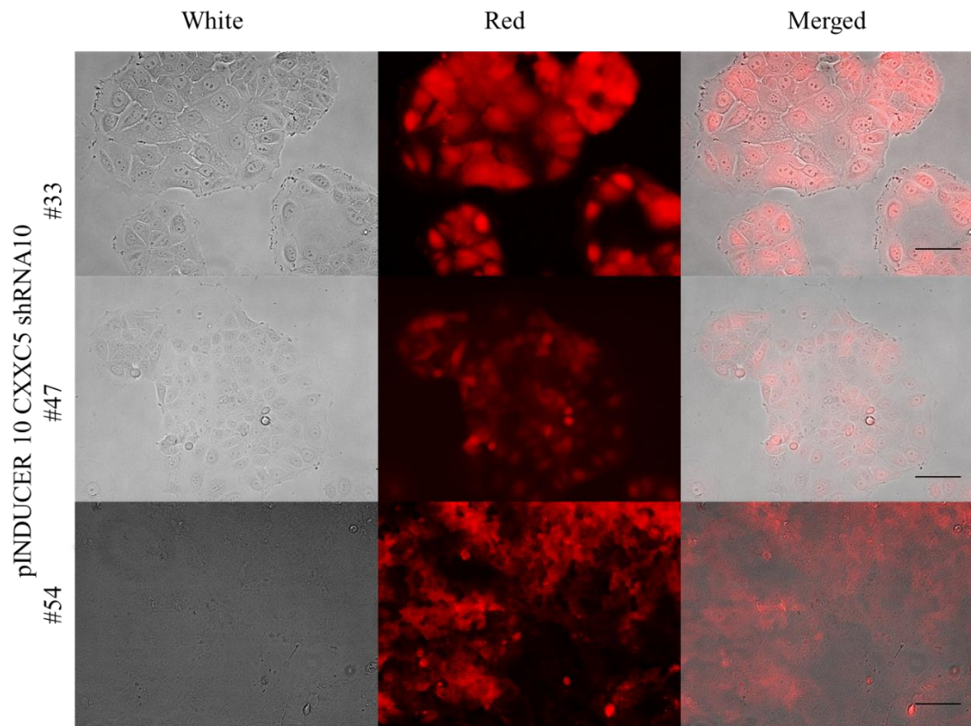
Figure 14 Induction control of pINDUCER10 CXXC5-shRNA#10 colony 33, 47, 54
