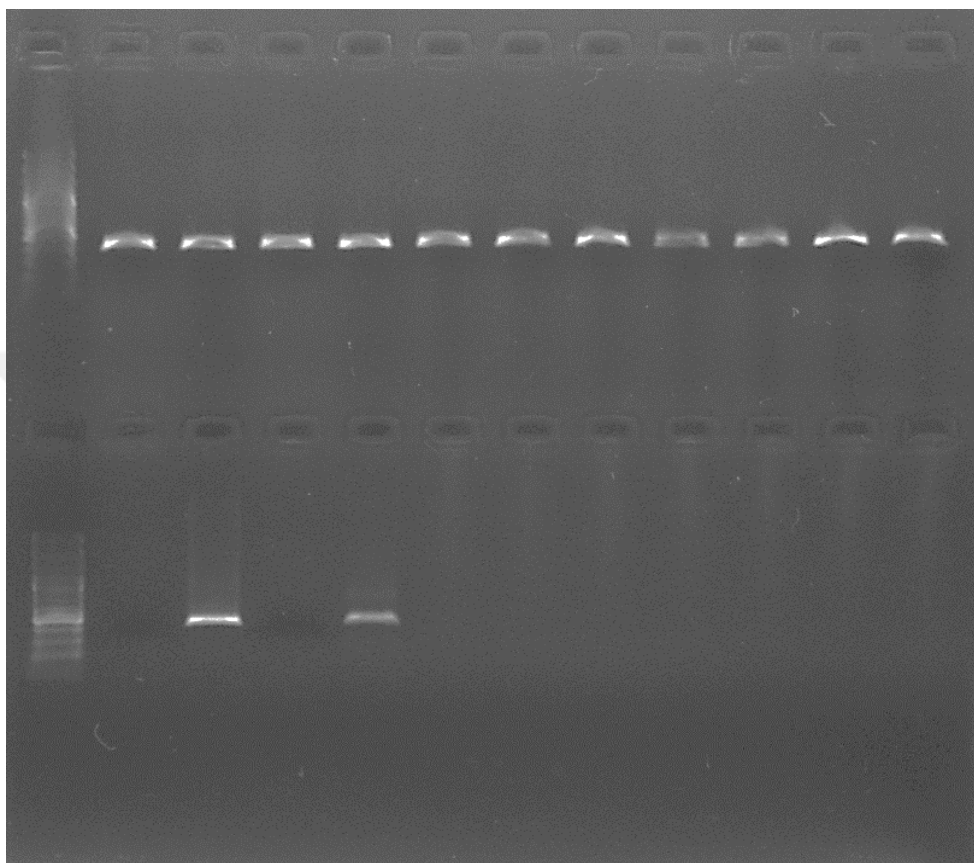
Figure 22 cDNA conversion control PCR with GAPDH cDNA and gDNA positive controls
