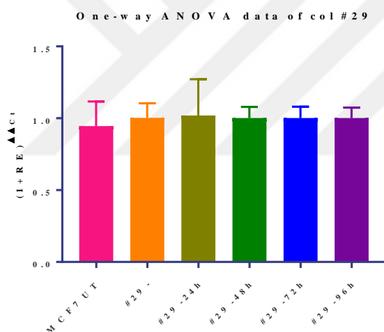
Figure 20 Graphical representation of RT-qPCR results of time course experiment of colony #29
