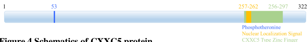
Figure 4 Schematics of CXXC5 protein
