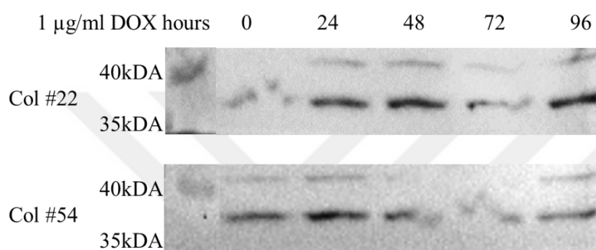
Figure 19 Time course experiment for clones; #22 and #54
