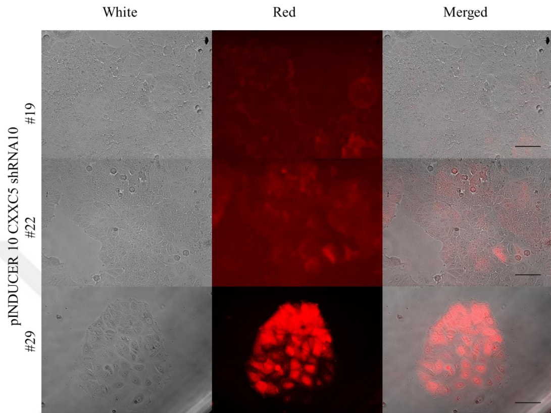
Figure 13 Induction control of pINDUCER10 CXXC5-shRNA#10 colony 19, 22, 29
