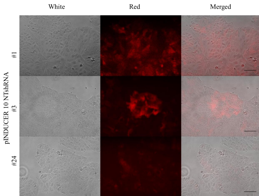
Figure 15 Induction control of pINDUCER10 NTshRNA colony 1, 3, 24
