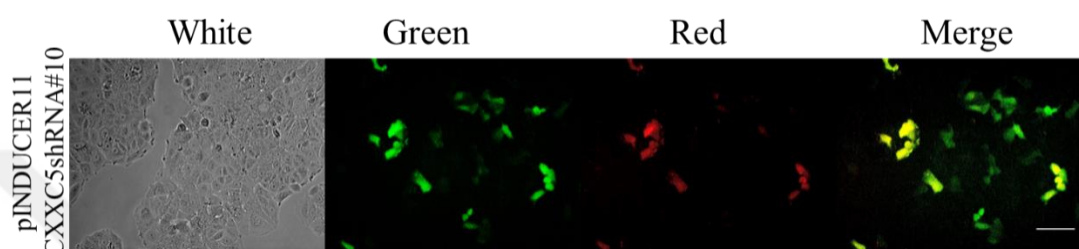
Figure 12 pINDUCER11 CXXC5 shRNA#10 infected MCF7
