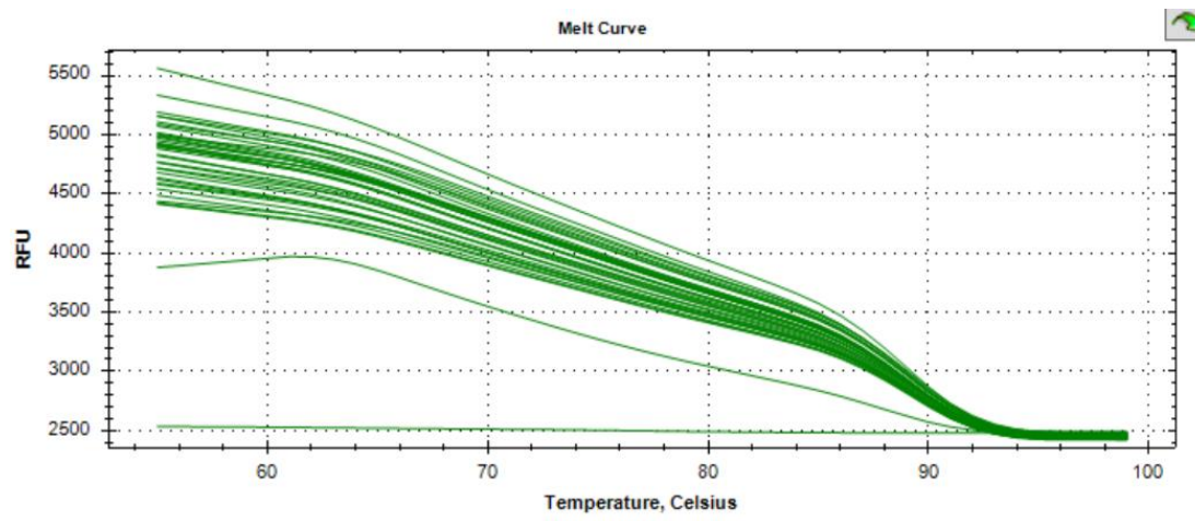
Figure 28 Sample melt curve
