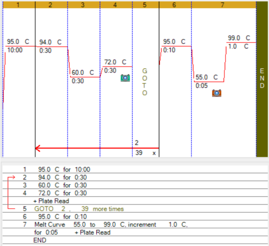
Figure 23 RT-qPCR cycling conditions
