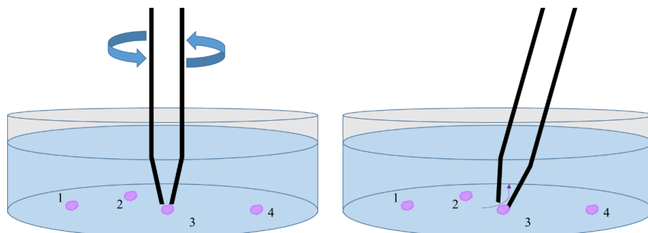
Figure 6 Monoclonal selection
