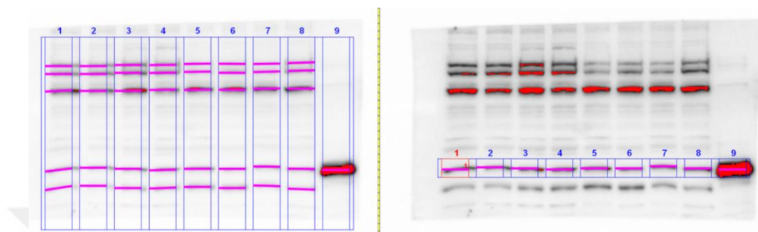
Figure 32 Normalization of the WB data using ImageLab
