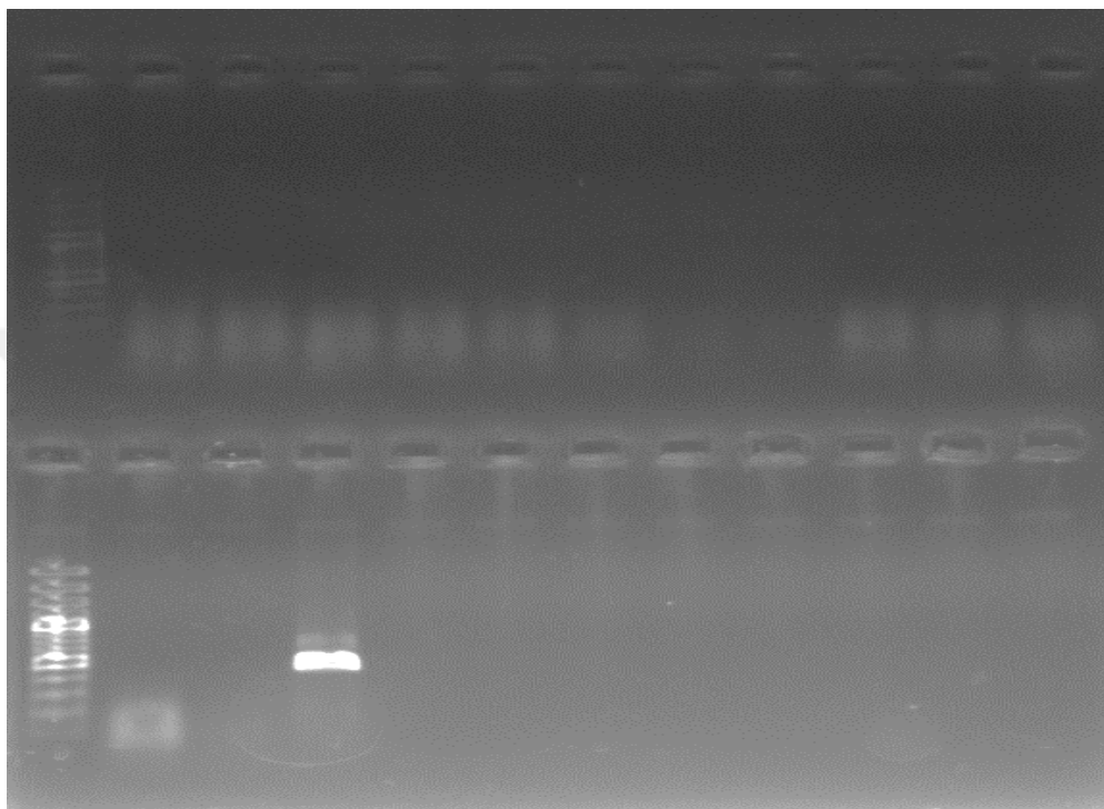
Figure 21 Genomic DNA contamination control PCR with gDNA positive control
