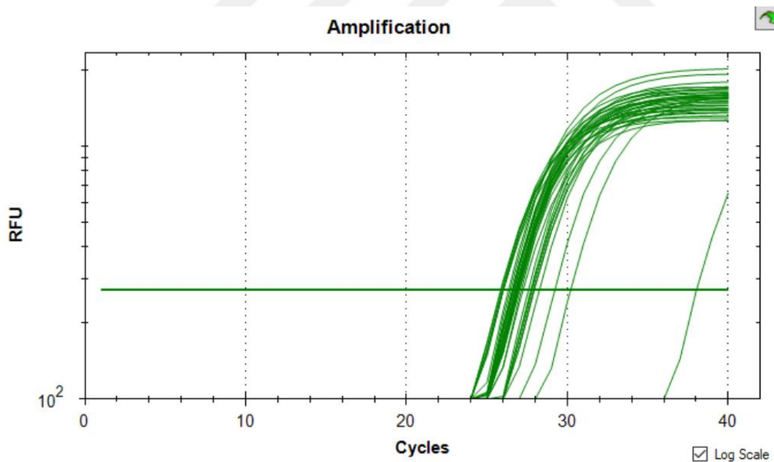
Figure 25 Sample amplification curve for qPCR
