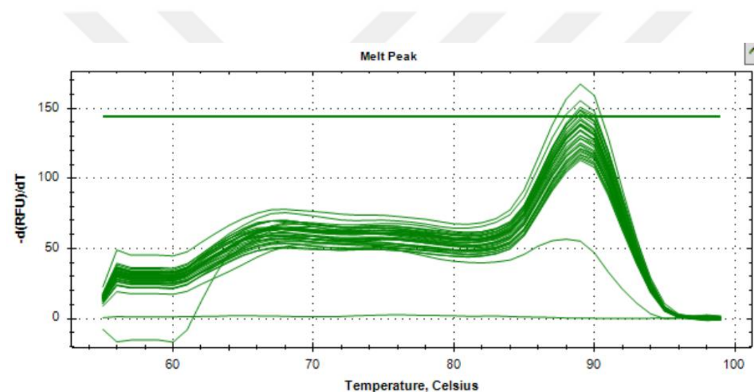
Figure 29 Sample melt peak
