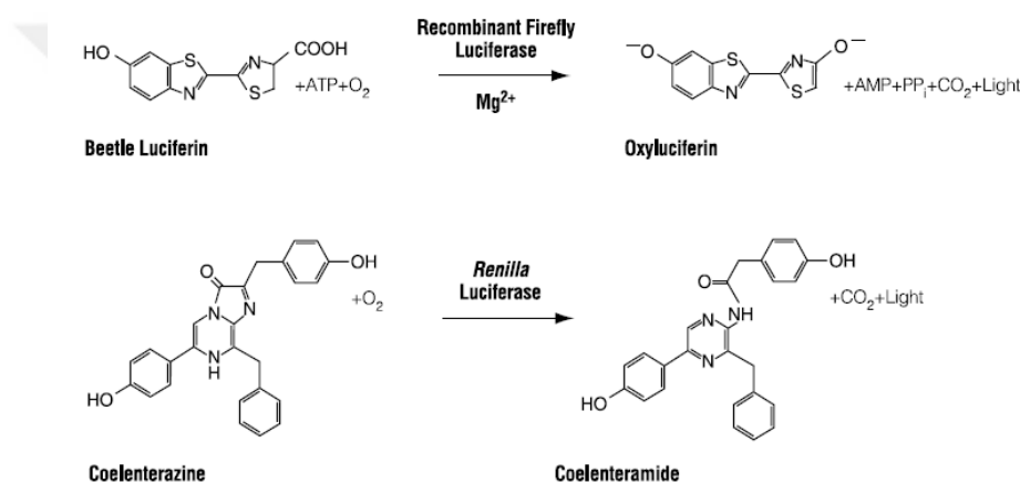
Figure 5 Chemical reaction of firefly luciferase and Renilla luciferase in the presence of their substrate
