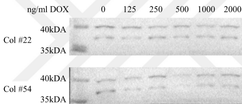
Figure 18 Dose response experiment for colonies; 22 and 54
