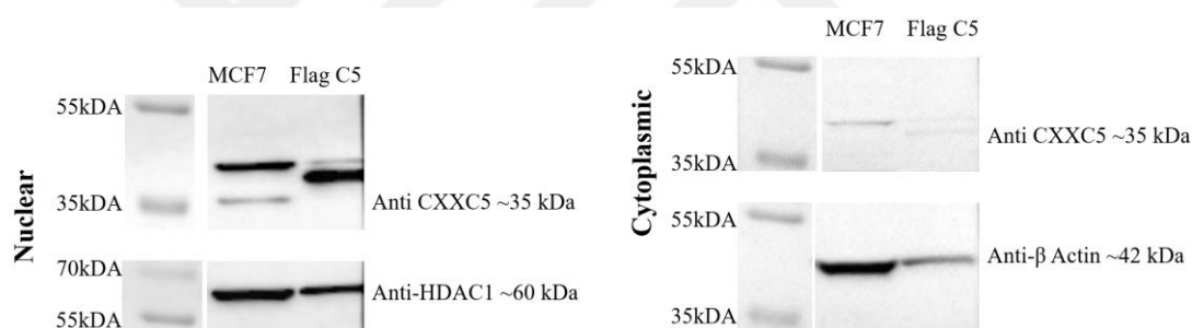
Figure 16 Nuclear vs cytoplasmic expression of CXXC5 in MCF7 cells
