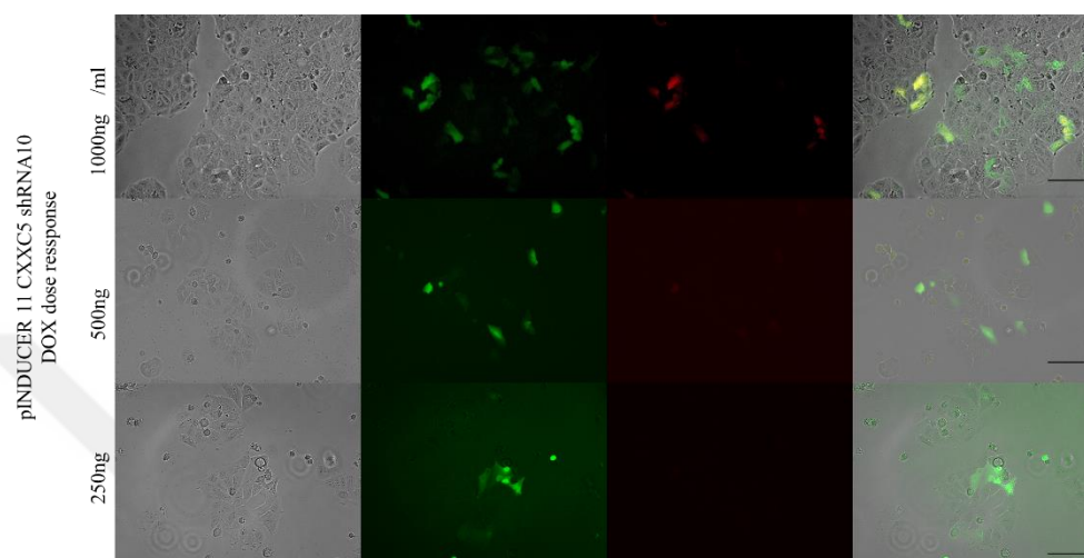
Figure 31 pINDUCER11 CXXC5 shRNA#10 infected MCF7 dose response for Doxycycline
