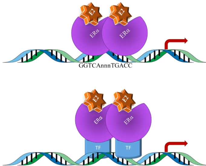
Figure 2 Schematic representation of ERE-dependent and ERE-independent signaling pathways
