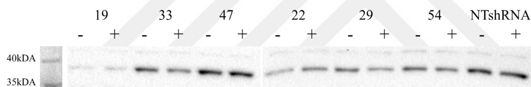
Figure 17 CXXC5 expression in nuclear extracts of stable cell lines generated with MCF7
