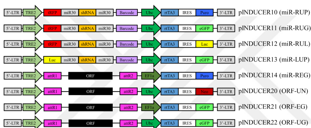
Figure 9 Diagrams of the pINDUCER vector series.
