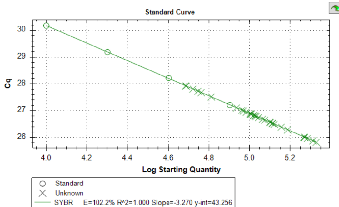
Figure 24 Sample standard curve of qPCR reaction
