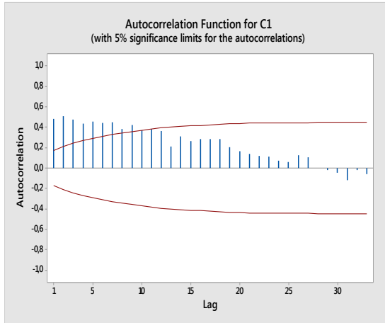
Figure 5.7.a. Autocorrelation function for all accident numbers
