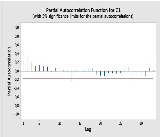
Figure 5.7.b. Partial autocorrelation function for all accident numbers
