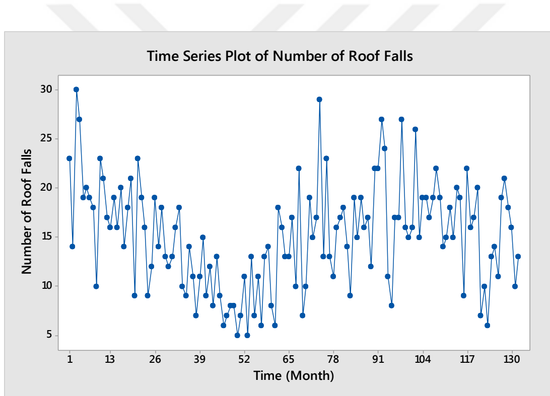
Figure 5.15 Time series plot for roof fall accidents
