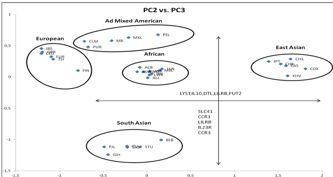
Figure 3.2. Separation of 1000 Genome populations along PC2 vs. PC3. Genes with the largest contributions on the respective PCs are listed on the axes.
