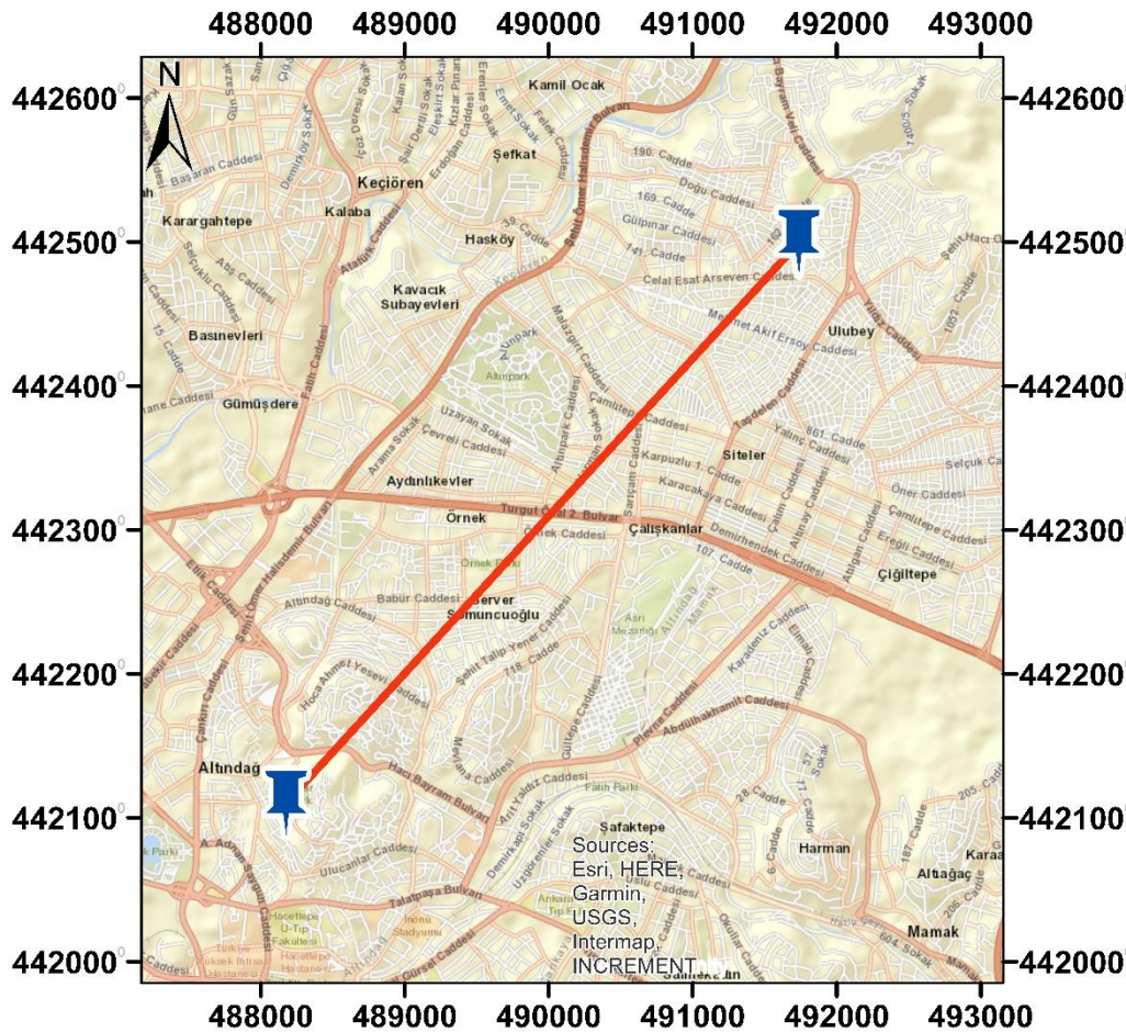
Figure 3.17: Euclidean distance.
