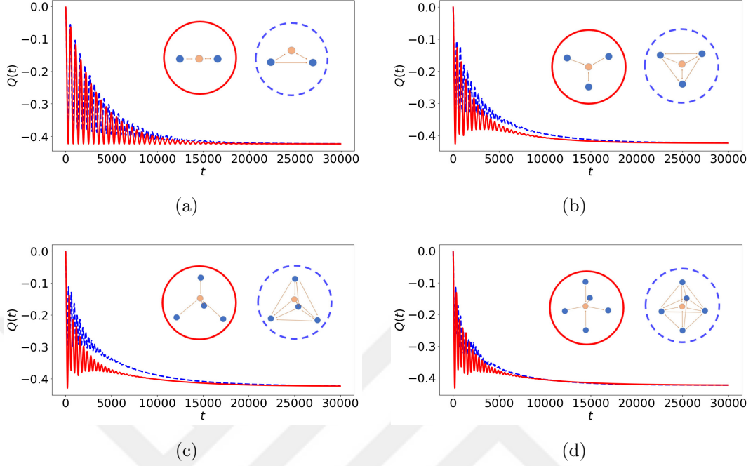
Figure 2.5: Heat current as defined in Eq. (2.23) with respect to dimensionless time t . The solid red curve corresponds to the case in which there is no coupling between the buffer spins. The dotted blue curve illustrates the case with coupling between buffer spins. (a) Two buffer spin network. (b) Three buffer spin network. (c) Four buffer spin network. (d) Five buffer spin network.
