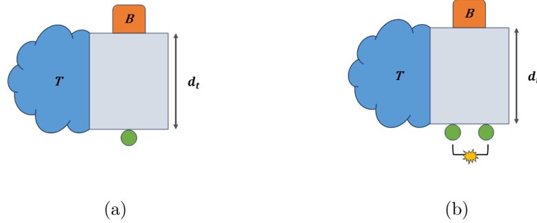
Figure 3.9: Schematic representation of the experimental setup: the blue cloud represents the biological system at temperature T , the gray box signifies the hydrogel with a thickness of d_t , the orange box denotes the static magnetic source B , and the green disc represents the NV center. (a) Configuration for a single NV center. (b) Configuration for two entangled NV centers, with entanglement symbolized by the yellow star.
