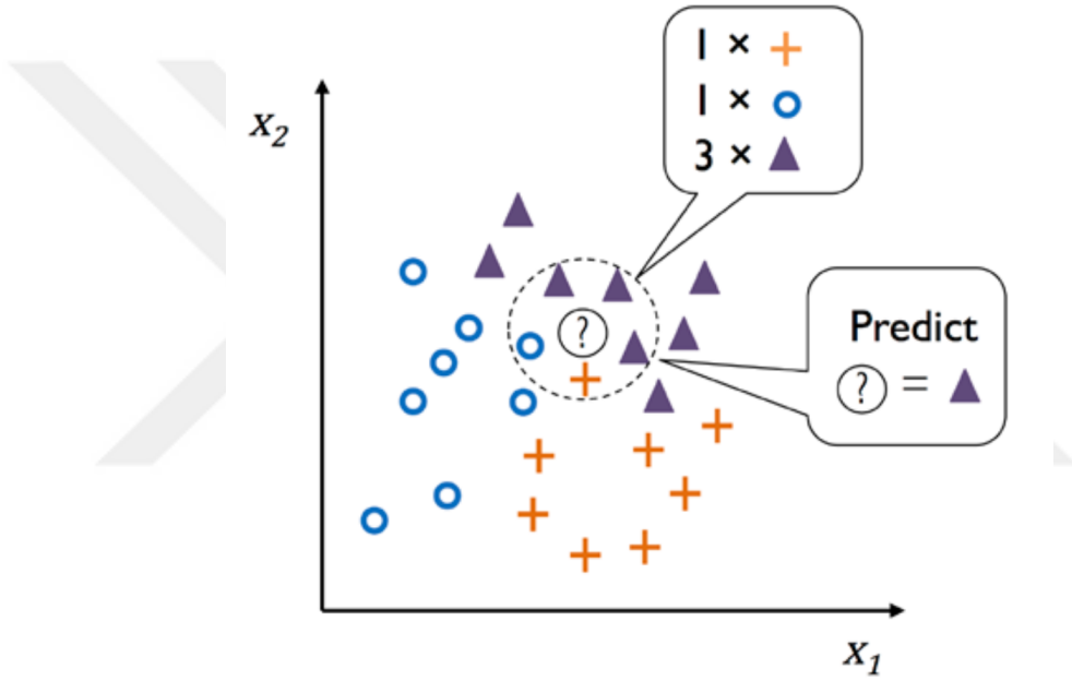
Figure 2.14: KNN with two features[79]
