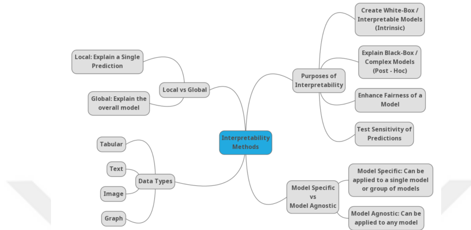
Figure 2.19: The classification of interpretability techniques[56]
