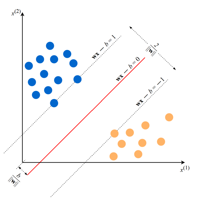
Figure 2.15: SVM[15]
