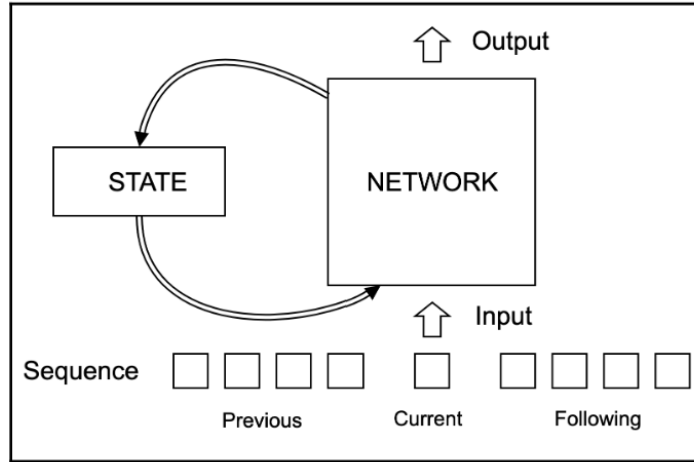
Figure 2.17: RNNs structure[95]
