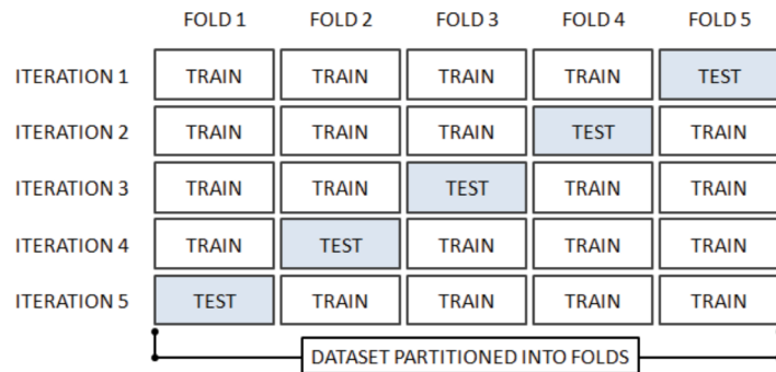
Figure 3.6: KFCV Process[69]
