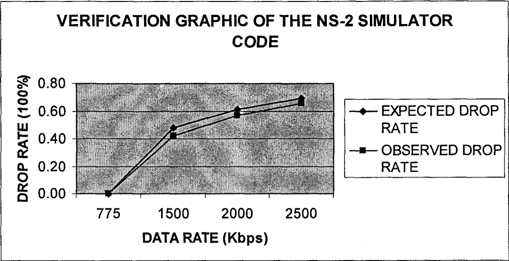
Figure 5-3 Verification Graphic of Ns-2 Simulator
