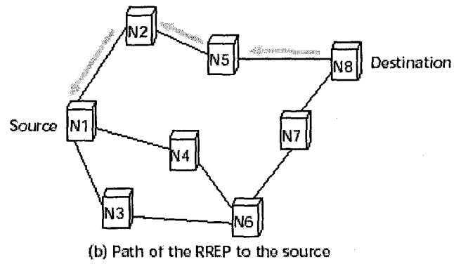
Figure 4-5 AODV Route Discovery [20]
