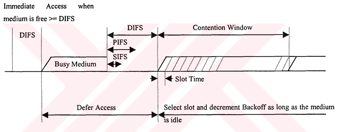
Figure 3-2 Inter Frame Space Time
