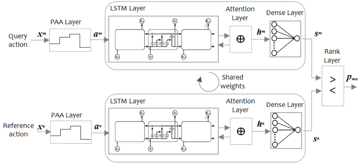
Figure 1. General framework for pairwise ranking of actions.
