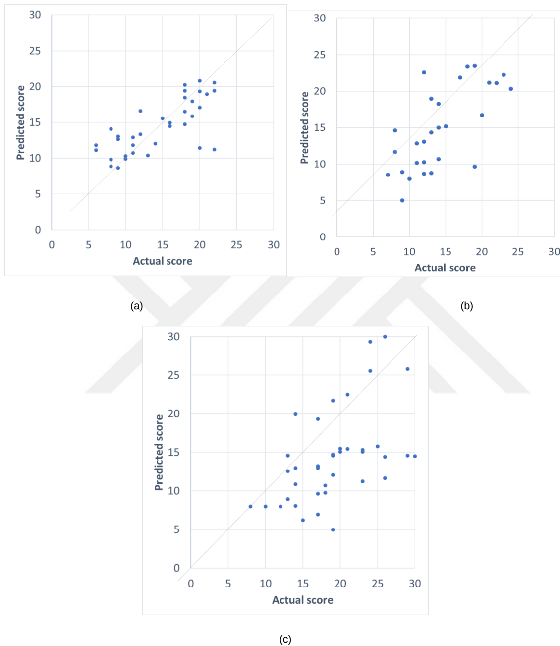
Figure 12. Scatter plots for predicted skill scores vs actual scores for the tasks of (a) knot tying, (b) needle passing, and (c) suturing
