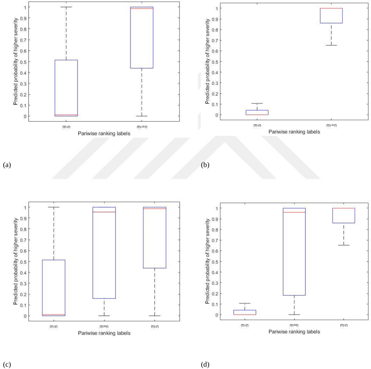
Figure 7. Boxplots of predicted probabilities against pairwise ranking labels for (a) binary ranking without attention, (b) binary ranking with attention, (c) ternary ranking without attention, and (d) ternary ranking with attention.
