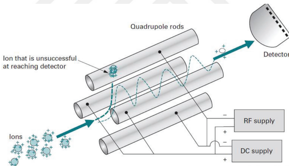
Figure 2.5. Quadrupole Mechanism 19
