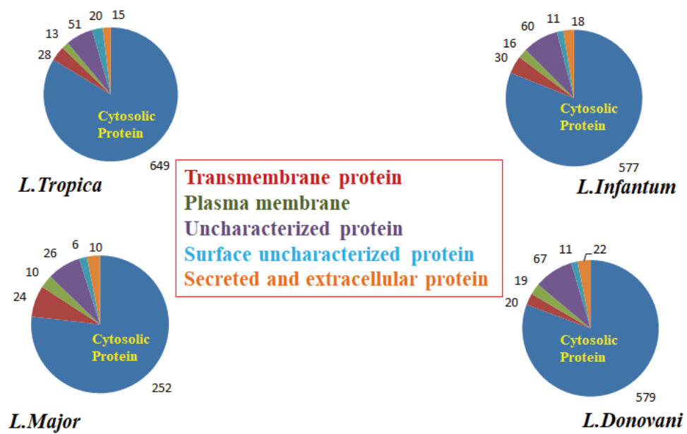
Figure 4.6. Protein Distribution
