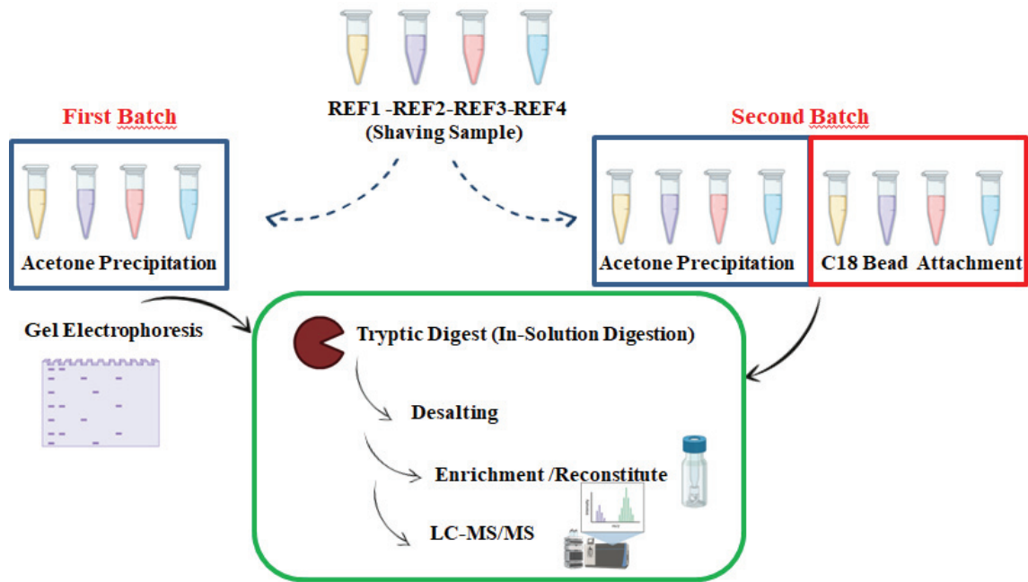
Figure 3.1. Experimental Workflow
