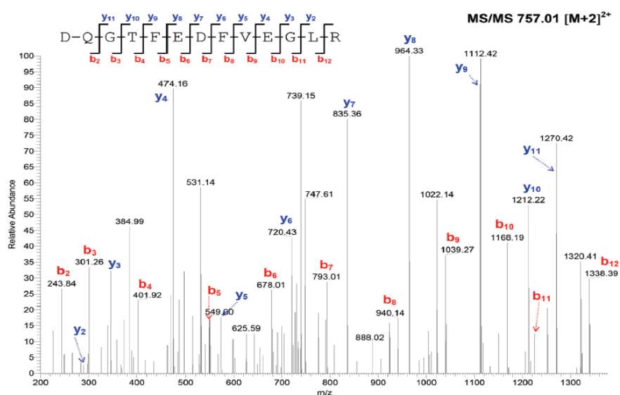
Figure 2.11. MS/MS spectrum 45
