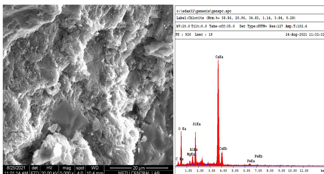
Figure 4. 10. SEM/EDX analysis of the reference specimen of the cement paste
