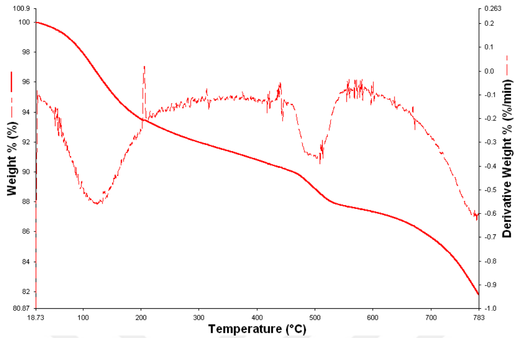
Figure 4. 20. TGA analysis of reference specimen
