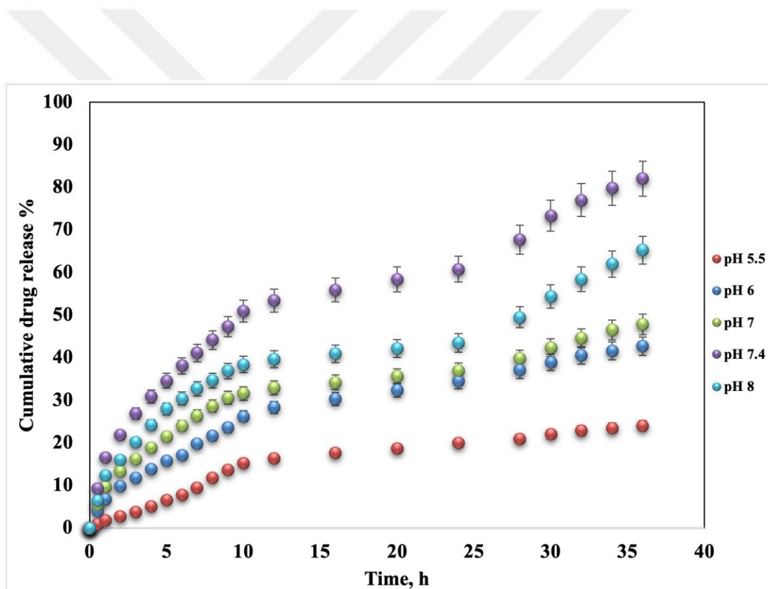
Figure 4.36. Carboxyl-activated CTX release from MIP1 was studied at pH: 5.5,6,7,7.4 and 8; 37°C.
