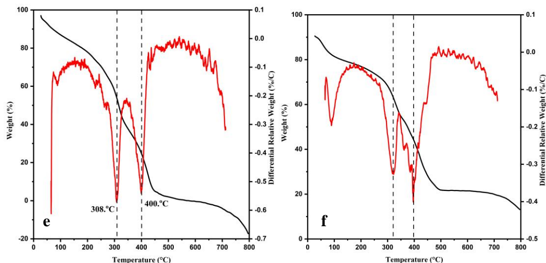
Figure 4.21. a: TGA/DTG curve of BC, b: TGA/DTG curve of M-BC, c: TGA/DTG curve of MIP1, d: TGA/DTG curve of MIP2, e: TGA/DTG curve of MIP3, f: TGA/DTG curve of NIP.
