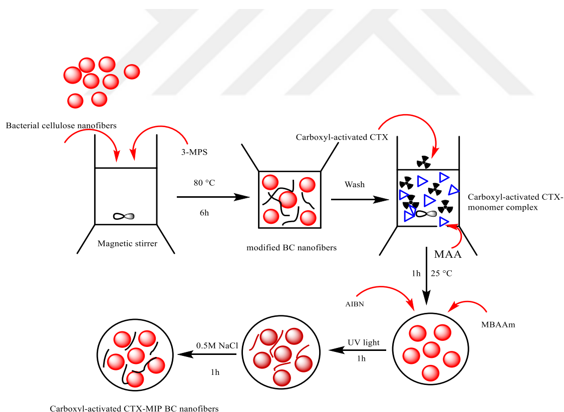
Figure 3.4. Schematic illustration of the carboxyl-activated CTX-MIPs/BC nanofibers' synthesis.
