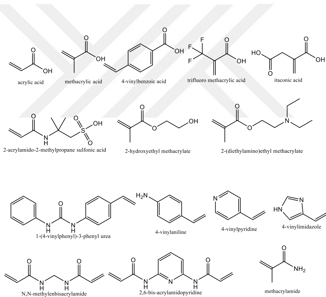
Figure 2.8. Scheme of commonly used monomers [125].
