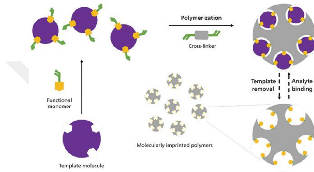
Figure 2.7. Schematic illustration of the molecularly imprinted process [118].
