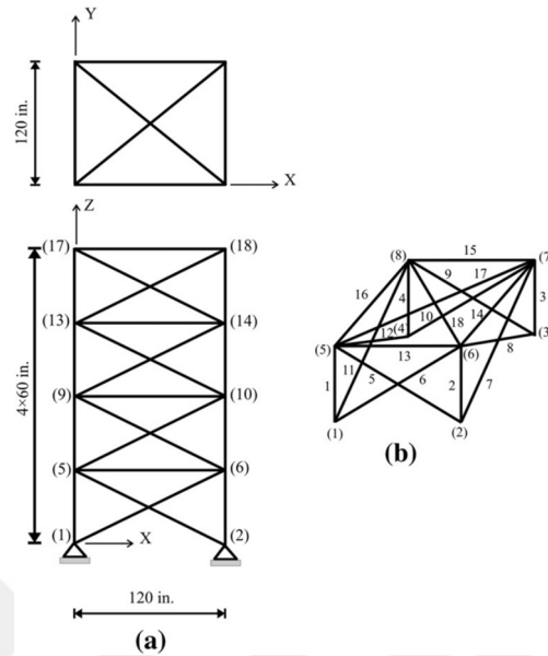
Figure 5.13. 72-member truss tower
