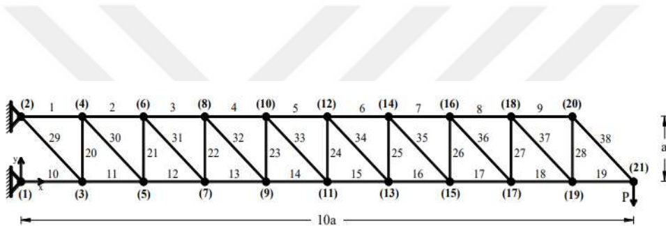
Figure 5.7. 38-member cantilever truss
