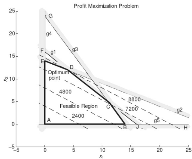
Figure 1.5. An illustration of the graphical method (Arora, 2004)
