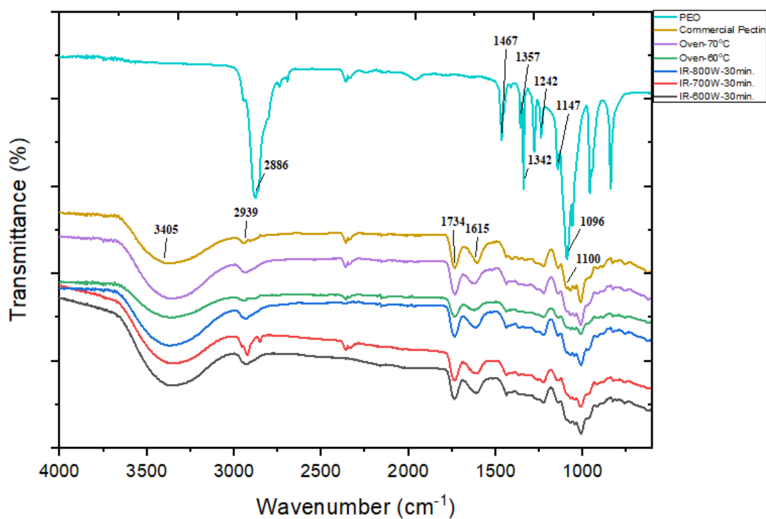
Figure 14. FTIR spectra of PEO and pectin powders
