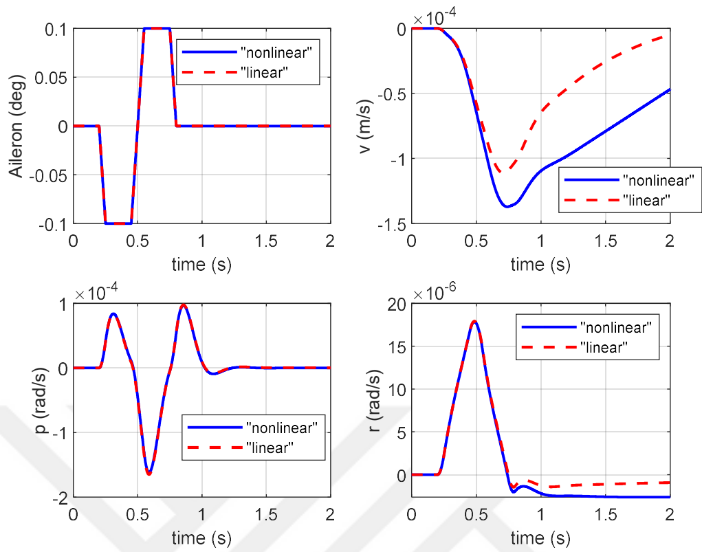
Figure 4.4 Linear model comparison for aileron inputs
