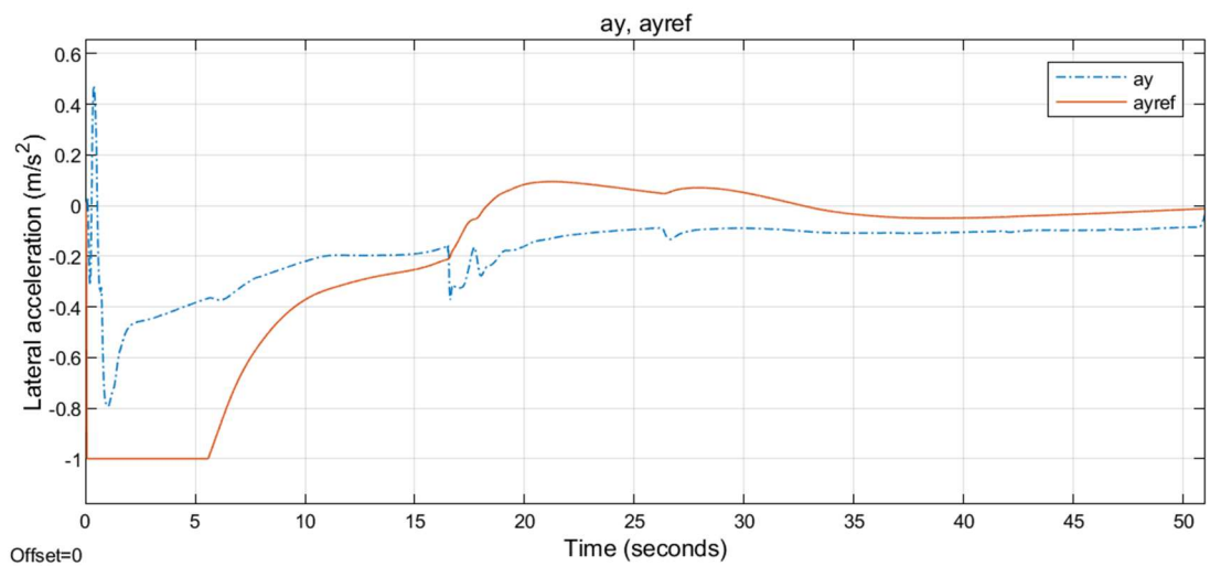
Figure 9.8 Lateral acceleration for the first simulation condition with SMC
