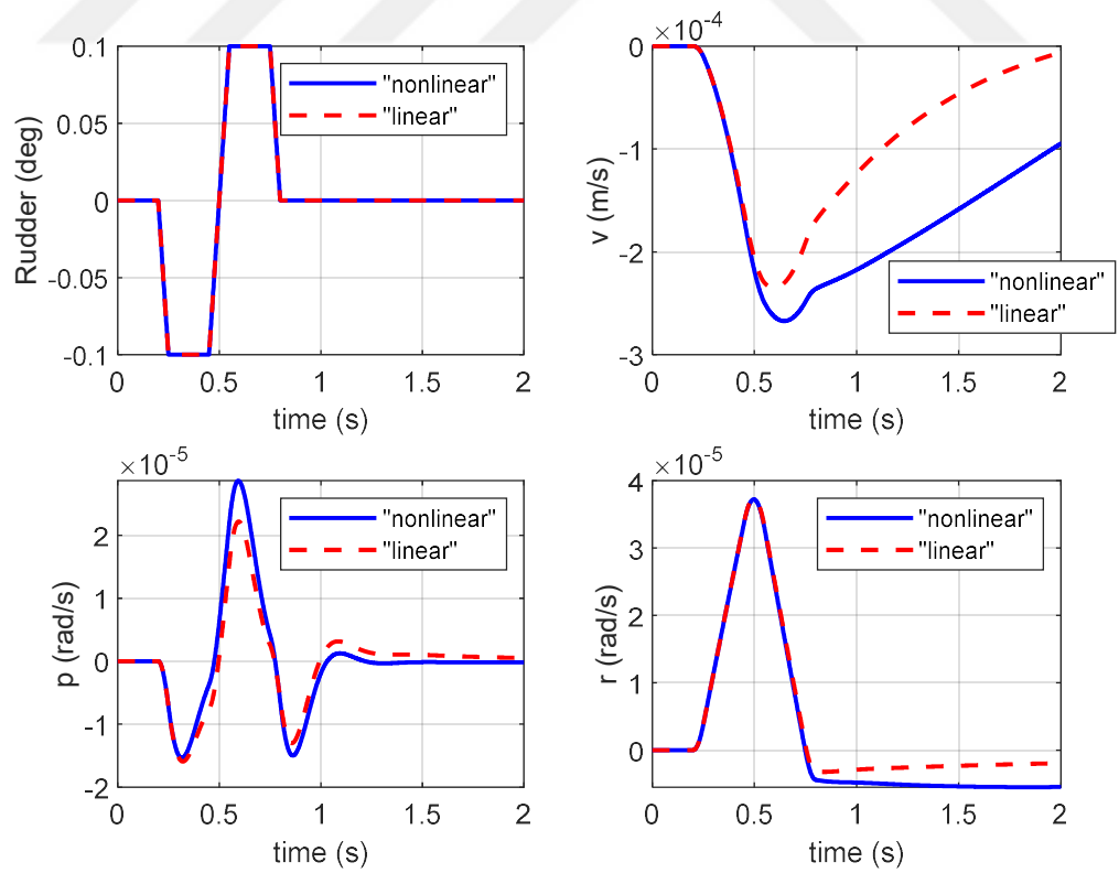
Figure 4.5 Linear model comparison for rudder inputs
