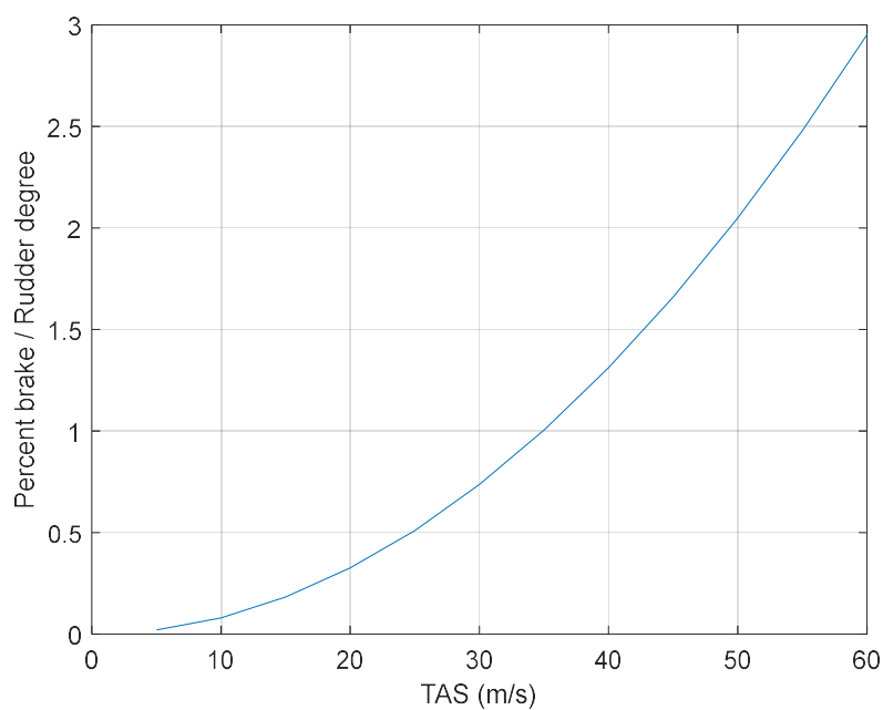
Figure 5.2 Relationship between differential brake and rudder with respect to speed of the aircraft
