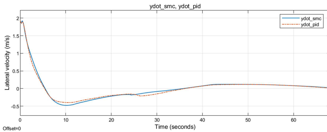
Figure 9.92 Lateral velocity with respect to runway midline for the sixth simulation condition
