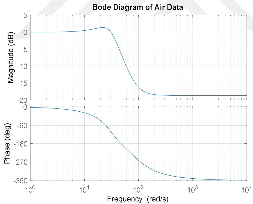
Figure 2.10 Bode Diagram of Air Data Sensors
