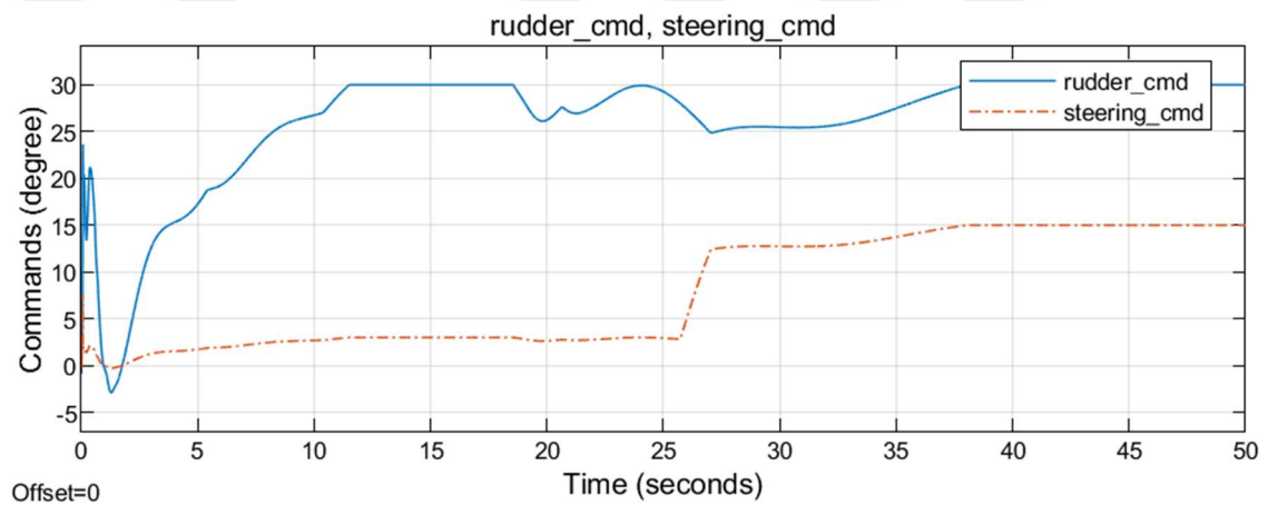
Figure 9.140 Rudder and steering commands for the eighth simulation condition with SMC
