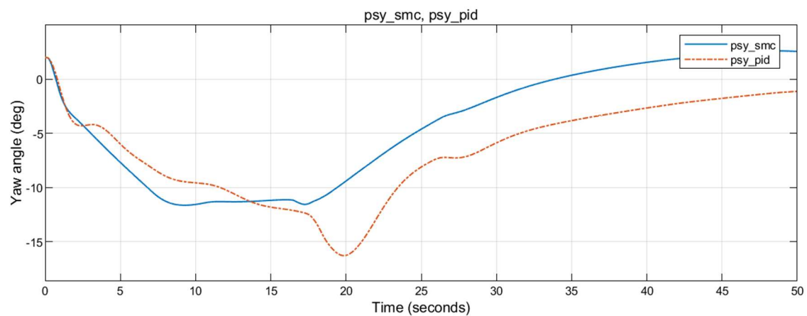
Figure 9.162 Yaw angle for the ninth simulation condition
