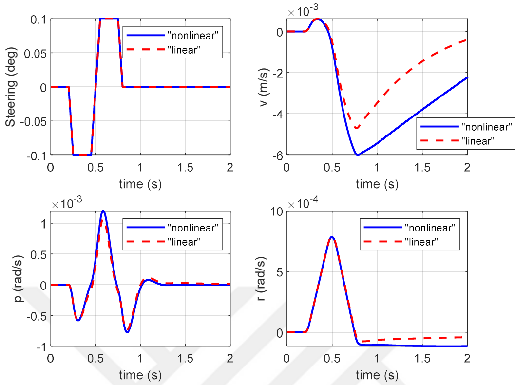
Figure 4.6 Linear model comparison for steering inputs
