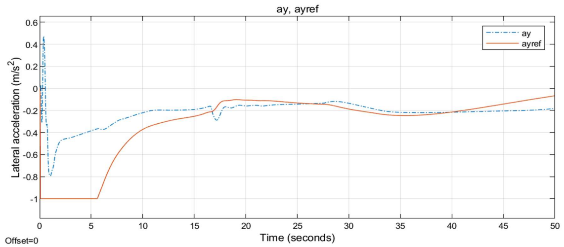
Figure 9.134 Lateral acceleration for the eighth simulation condition with SMC
