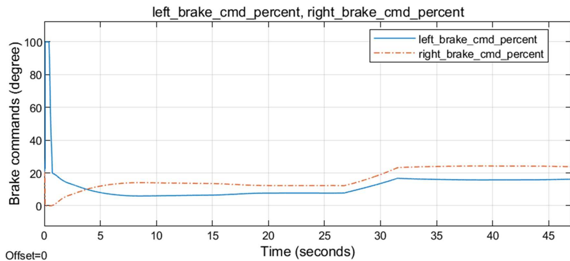
Figure 9.34 Left and right brake commands for the second simulation condition with SMC
