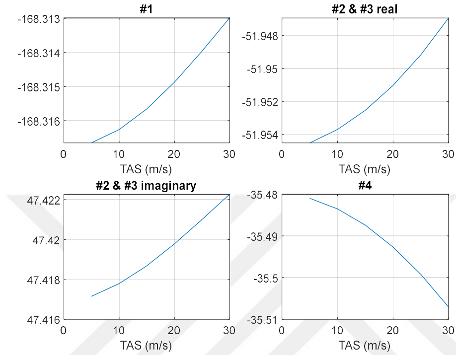
Figure 13.68 Longitudinal poles of 3 tires on the ground aircraft
