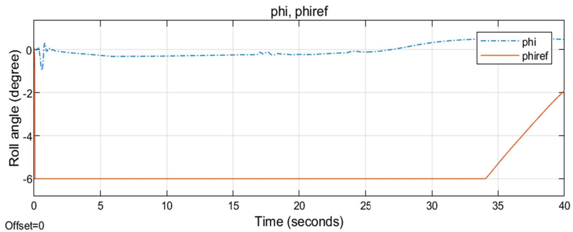
Figure 9.46 Roll angle for the third simulation condition with SMC
