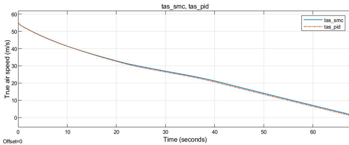
Figure 9.93 True airspeed for the sixth simulation condition
