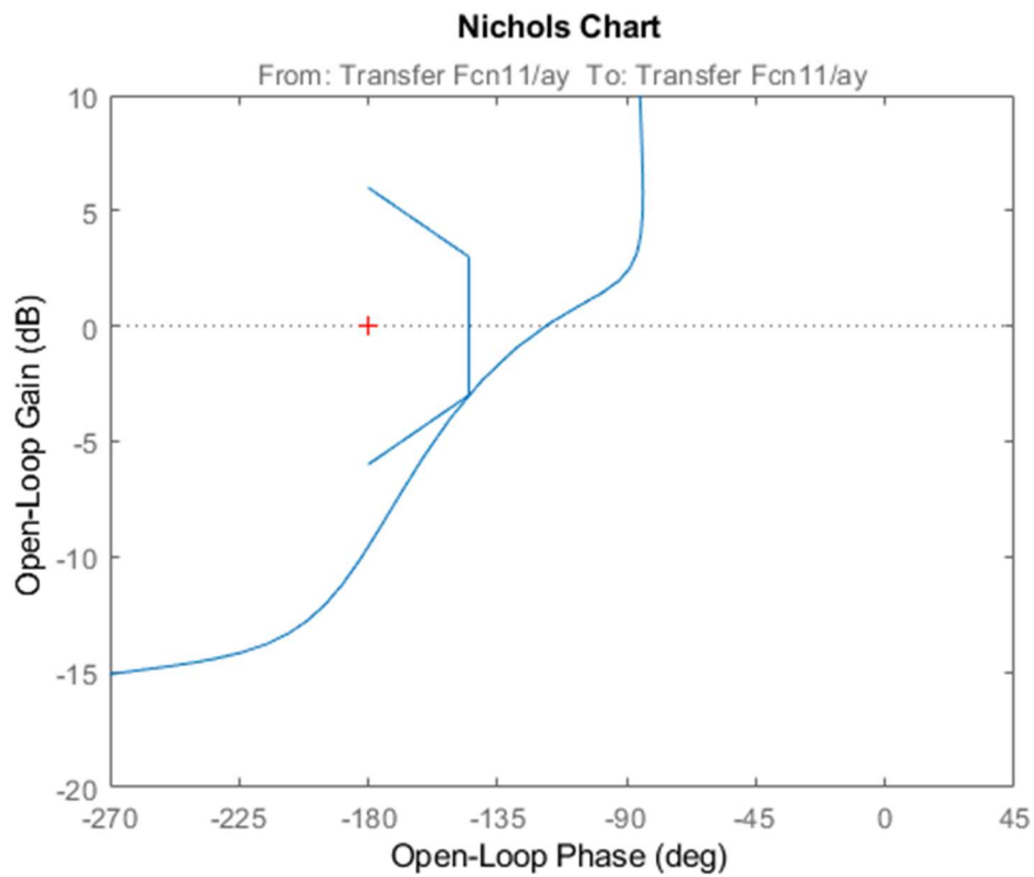
Figure 13.62 ay loop for lateral PID controller
