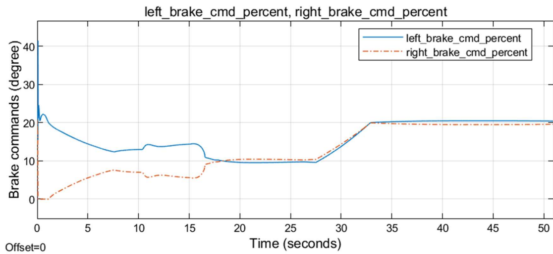
Figure 9.16 Left and right brake commands for the first simulation condition with SMC
