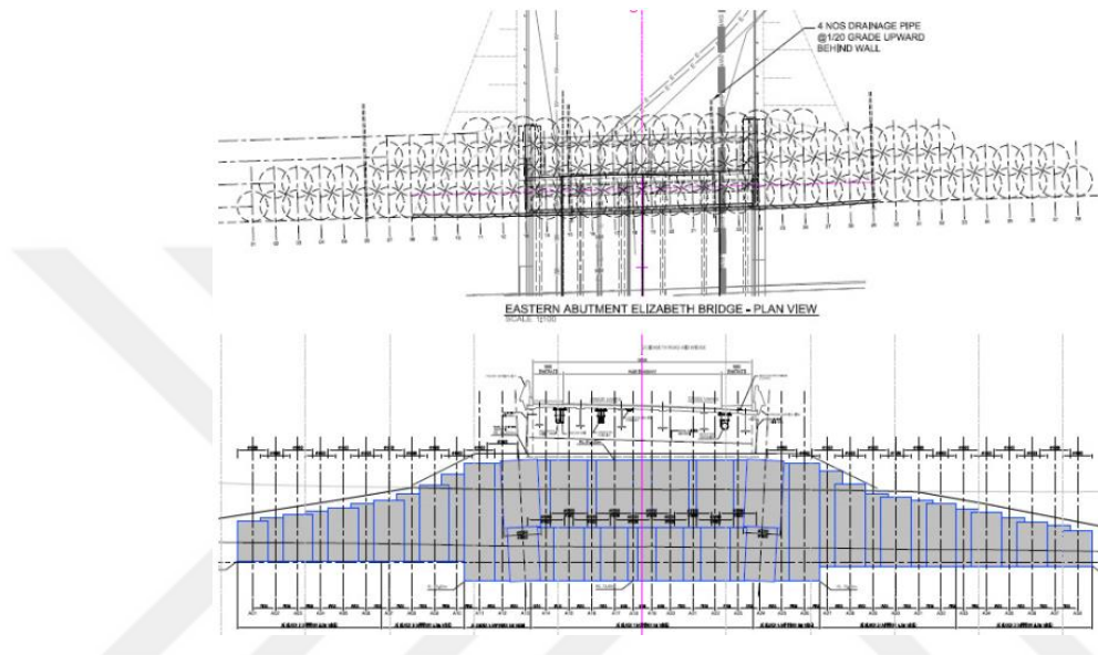
Figure 3.18. Jet grouted mass gravity wall: (a) plan view and (b) elevation (Vincent et al. 2014)
