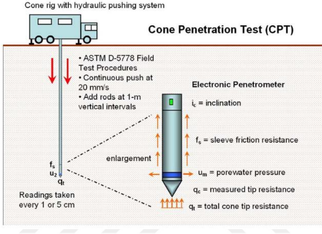
Figure 2.9. Overview of the Cone Penetration Test (CPT) Per ASTM D 5778 Procedures (Source: NCHRP Project 20-05 Final Report, 2007)
