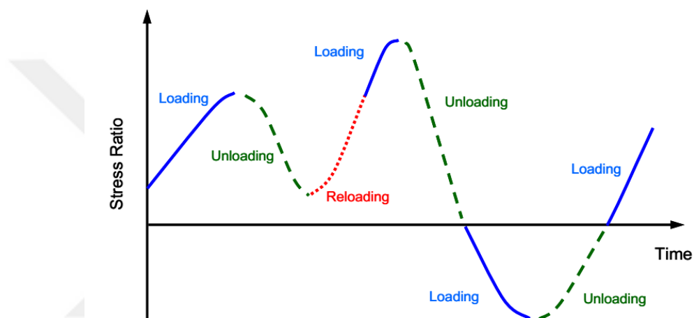
Figure 5.8. Stress ratio history showing loading, unloading, and reloading (Source: Byrne and Beaty 2011).
