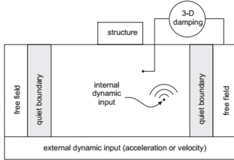
Figure 5.4. The rigid base type of dynamic loading boundary conditions available in Flac (Source: Flac, 2008).
