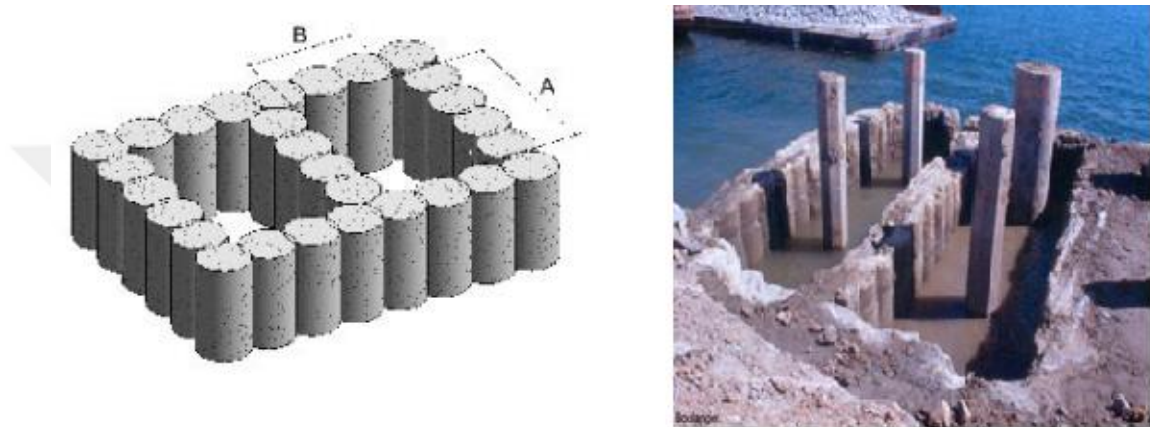
Figure 3.20. Cellular design of jet grout columns (a): plan dimension of cell, (b): an example application near the sea(Source Bolunger., 2012).
