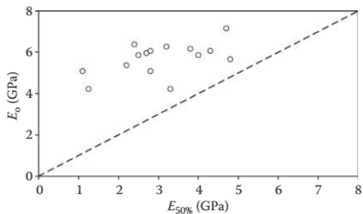
Figure 3.15. Elasticity for large strains modulus E_{50\%} values change small strain Elasticity for small strains modulus E_0 of jet grout (Croce et al. 2014 ).
