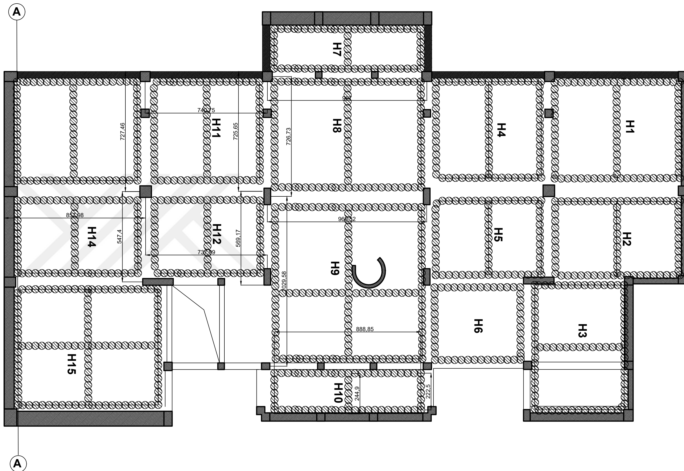
Figure B.1 Application plan of H Block
