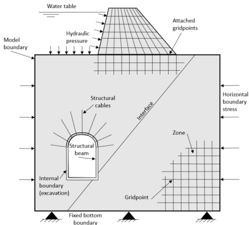
Figure 5.1. Elements of a FLAC model(Source: Flac, 2008).
