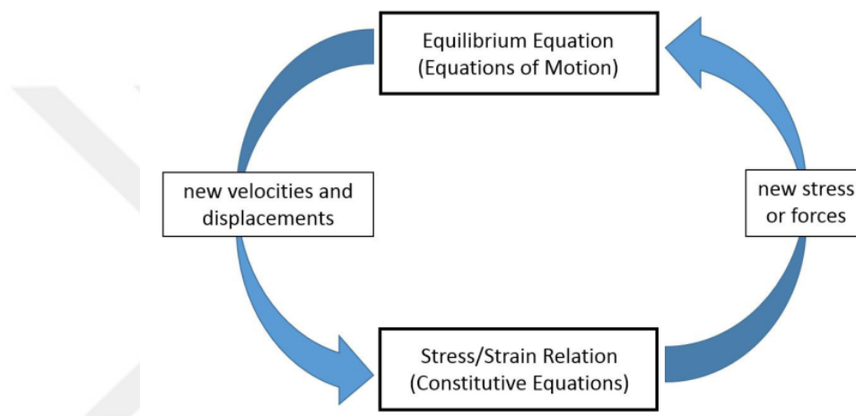
Figure 5.2. Basic explicit calculation cycle.
