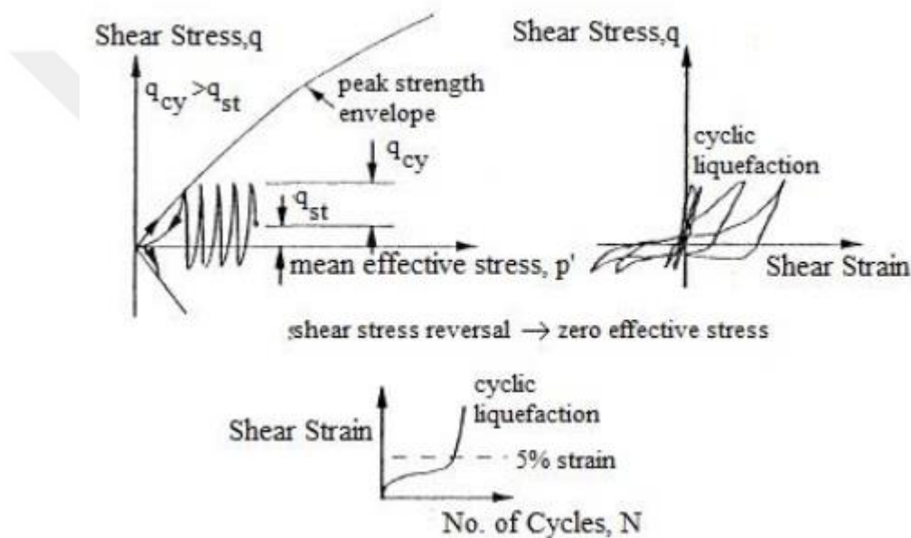
Figure 2.4. Cyclic liquefaction. (Source: Kramer, 1996)
