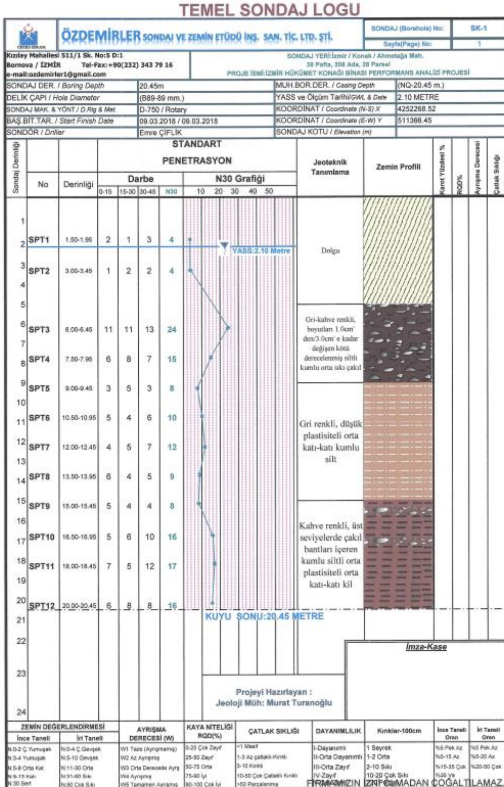
Figure A.1. Borehole log-1 (Özdemirler 2018).
