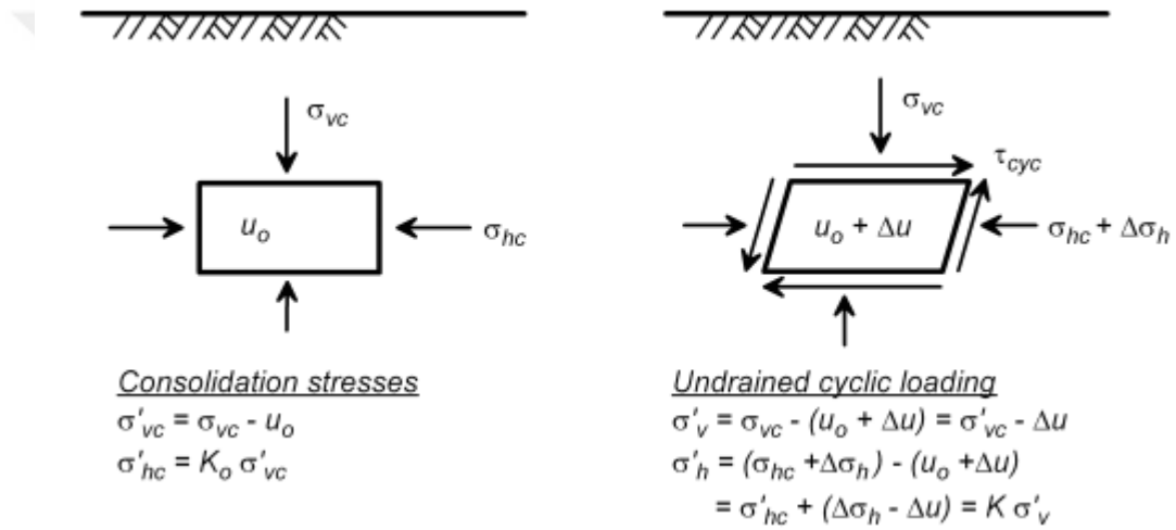
Figure 2.7. Cyclic stresses on a soil element beneath level ground during horizontal shaking (Idriss and Boulanger, 2008).
