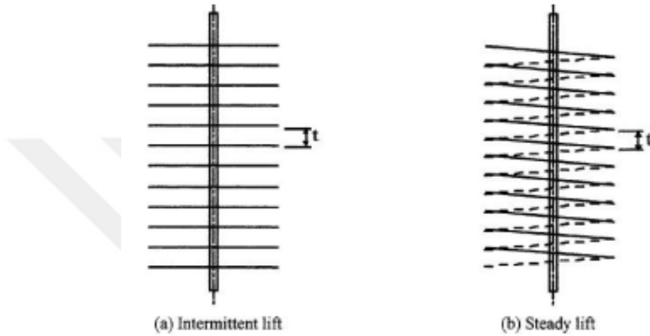
Figure 3.8. Lifting methods of drilling rods (Source: Croce et al. 2014)
