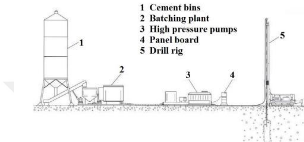
Figure 3.4. The Equipments of jet grouting application(Source:Croce et al. 2014).
